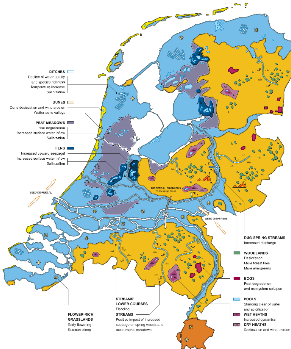
Fig. 5. Ecohydrological sketch map showing the ecohydrological impact of climate change in the Netherlands. Climate change, through its impact on the water cycle, will alter the diversity of plant species and plant communities. These alterations will in turn have an effect on habitat factors that are essential for plant growth such as salt levels, acidity, and the availability of moisture, oxygen and nutrients. The map indicates ecohydrological effects in 2050 under two climate change scenarios: W and W+. Both scenarios include a global temperature rise of 2 °C, increased winter rainfall, drier summers (especially W+) and more intensive rainfall events.
