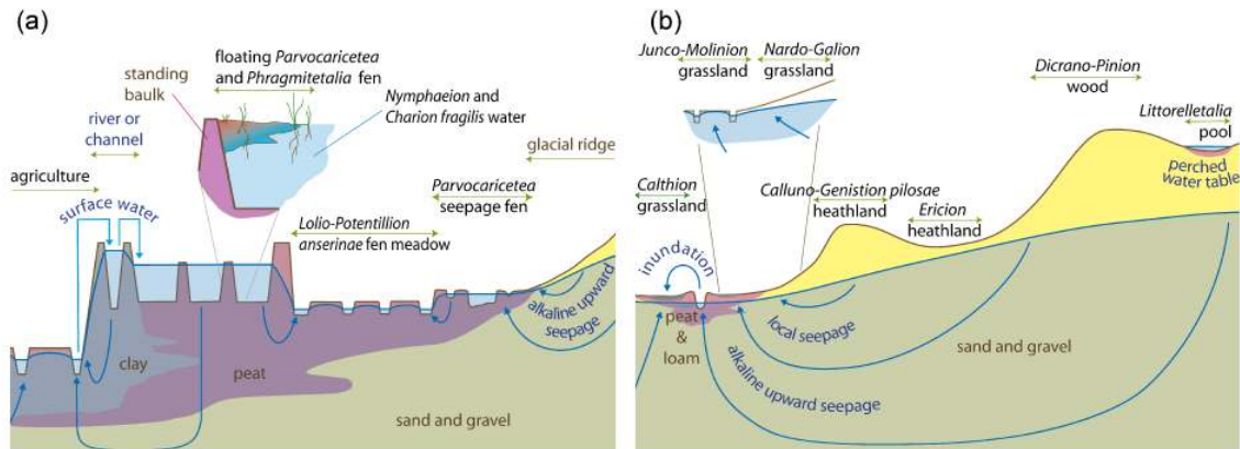
Fig. 1. Schematized ecohydrological cross sections, measuring ca. 10 km in width and 10 m in height, of (a) a fen landscape and (b) a cover-sand landscape. These landscapes occur in the “low” and “high” part of the Netherlands, respectively. Some characteristic vegetation types at the level of alliances and orders are indicated in italics (nomenclature according to Schaminée et al., 1995).
