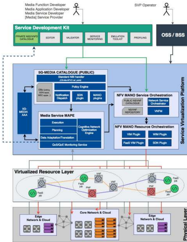
Fig. 1. High-level architecture.
