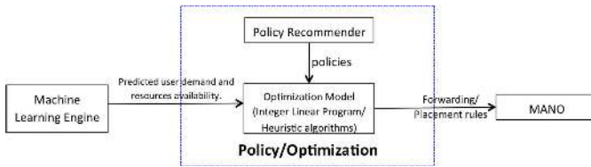
Fig. 4. Policy/optimization component.
