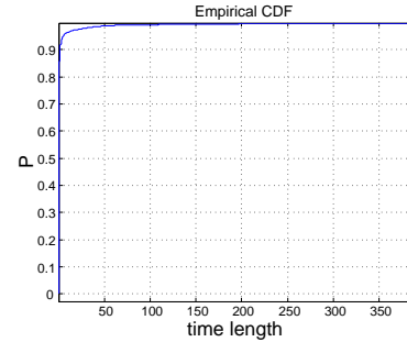
Fig. 6. Cumulative distribution formula of time length.
