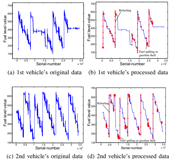
Fig. 14. Comparison between processed fuel level data and original data.
