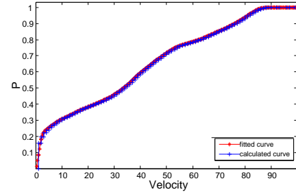
Fig. 9. The cumulative probability distribution of velocity. The solid line with stars represents the fitted curve. The solid line with pluses represents the calculated curve.
