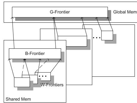
Figure 3: Hierarchical frontiers
