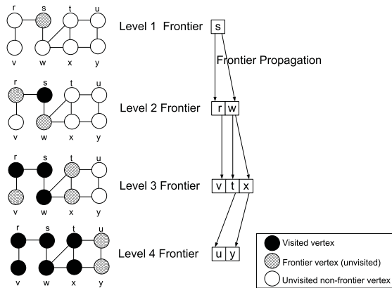
Figure 2: The operation of BFS
