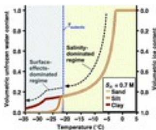
Figure 3. Schematic illustration of the two-regime division assumed in estimating ice saturations. Sand, silt, and clay are approximated using quartz grains of descending diameters ( 700, 40, \text{ and } 3\mu\text{m} , respectively). Pore water is an NaCl- \text{H}_2\text{O} solution with salinity of 0.7\text{M} ( =42\text{ppt} ): T_{\text{eutectic}} , eutectic point ( -21^\circ\text{C} ); S_n , pore-water salinity.
