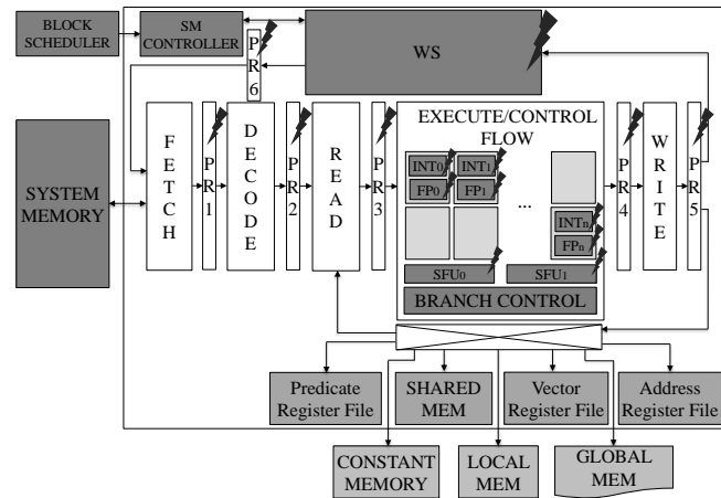
Fig. 2. A general scheme of the microarchitectural organization of the FlexGripPlus model and the internal modules targeted for the experiments. The SFU controllers are not shown in the scheme.
