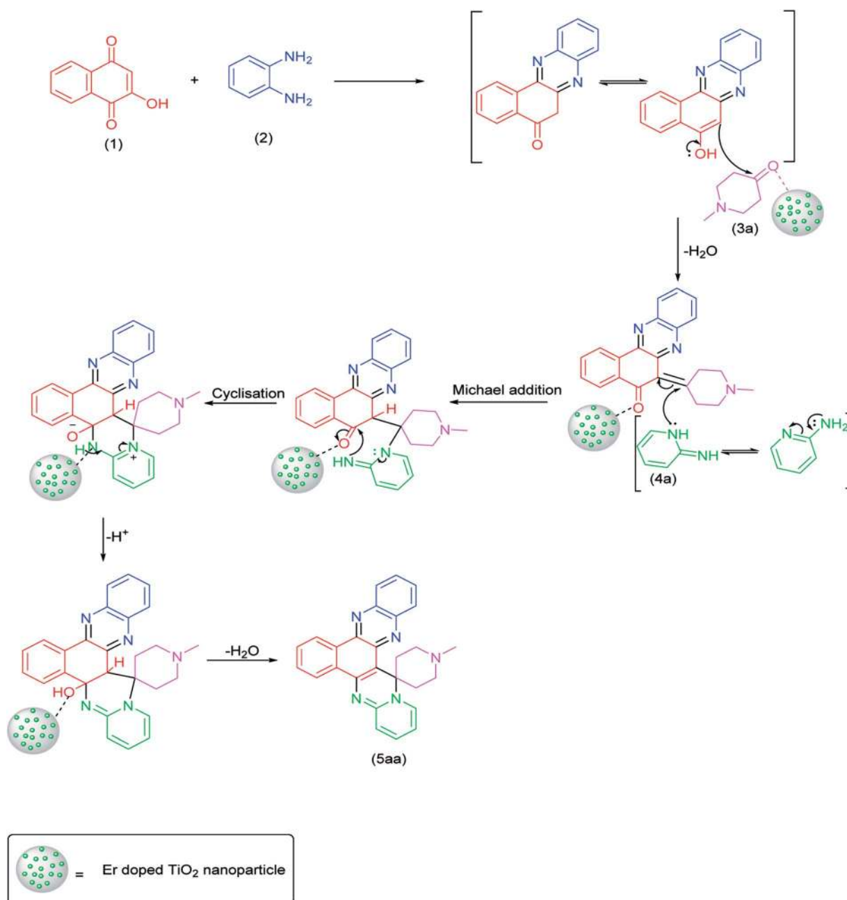
Scheme 2 Proposed mechanism.
