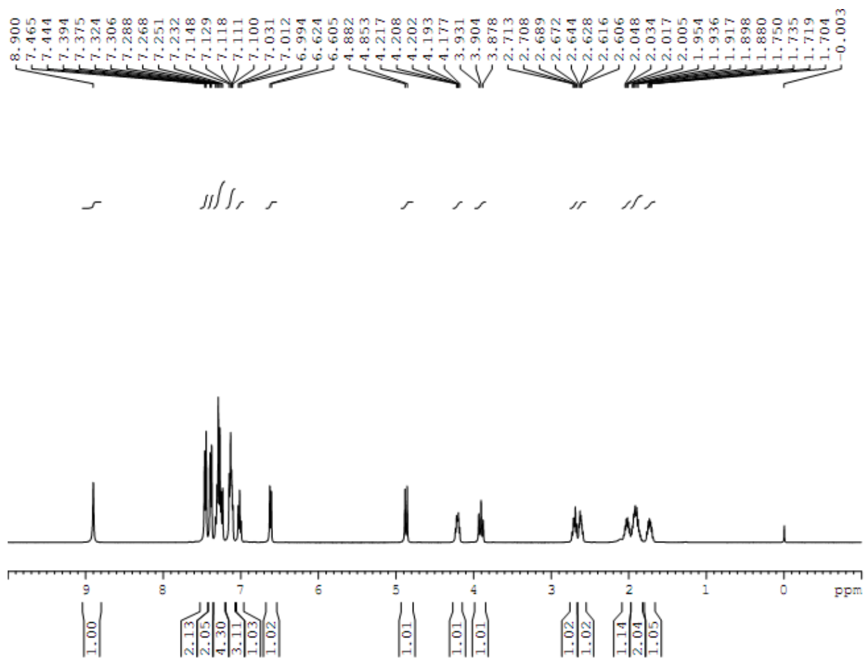
^1\text{H} NMR Spectrum of 6B
