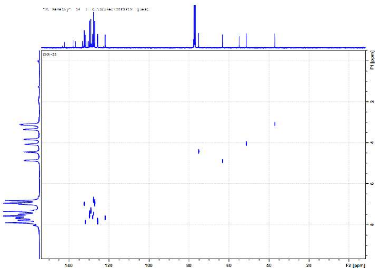
1 H- 13 C COSY spectrum of compound 10d
