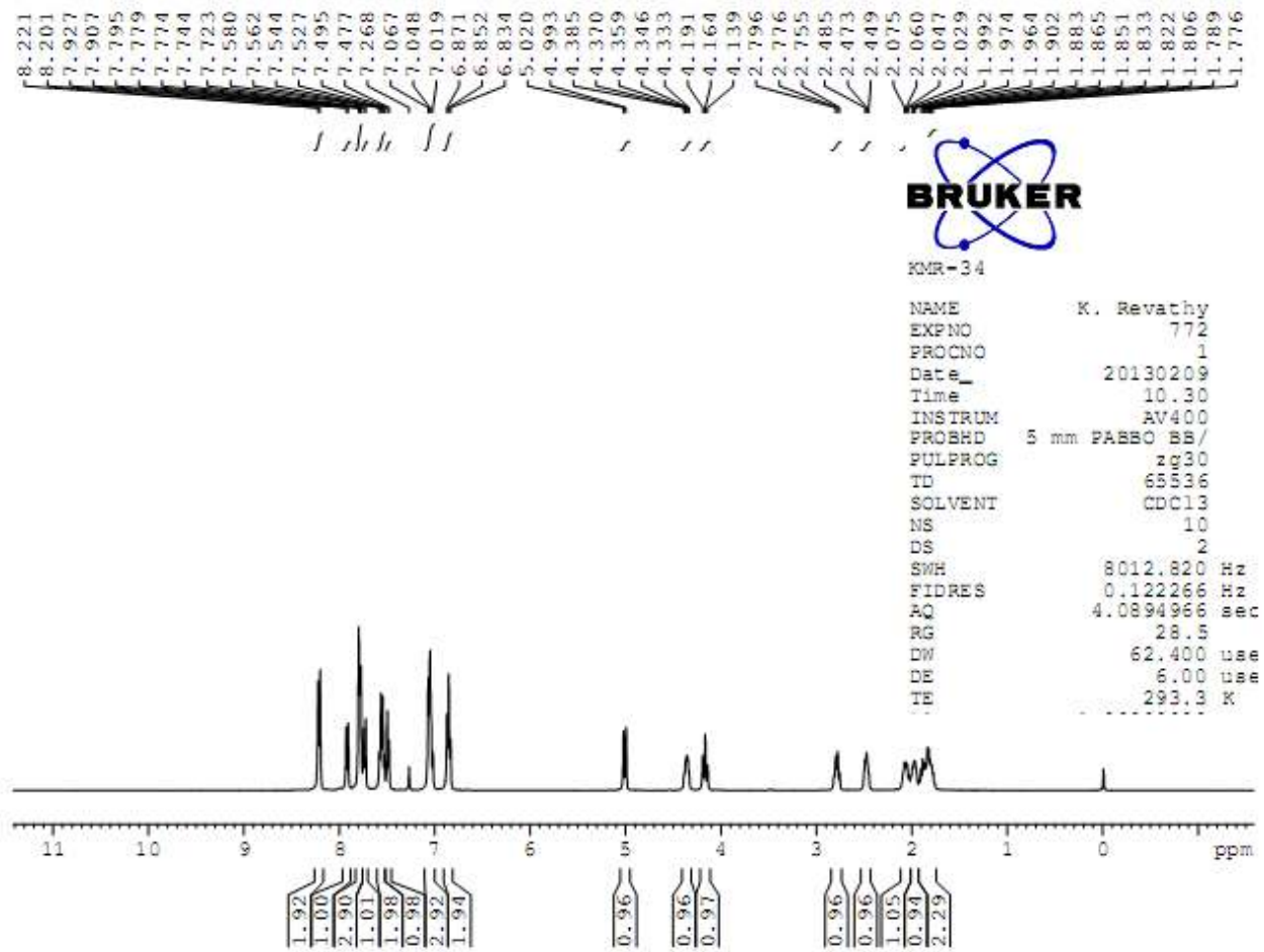
1 H NMR Spectrum of 10c
