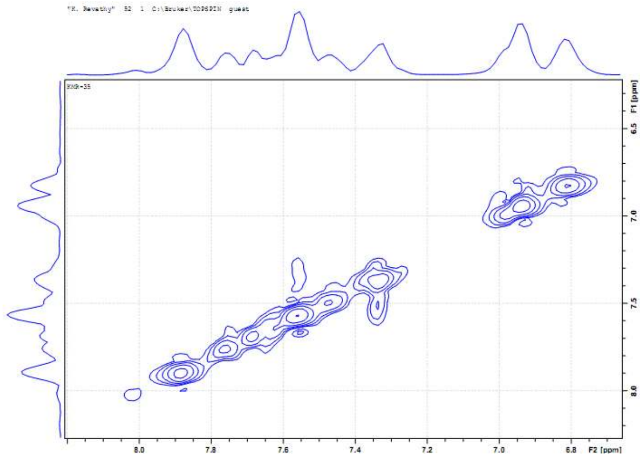
Expanded ^1\text{H} - ^1\text{H} COSY spectrum of compound 10d
