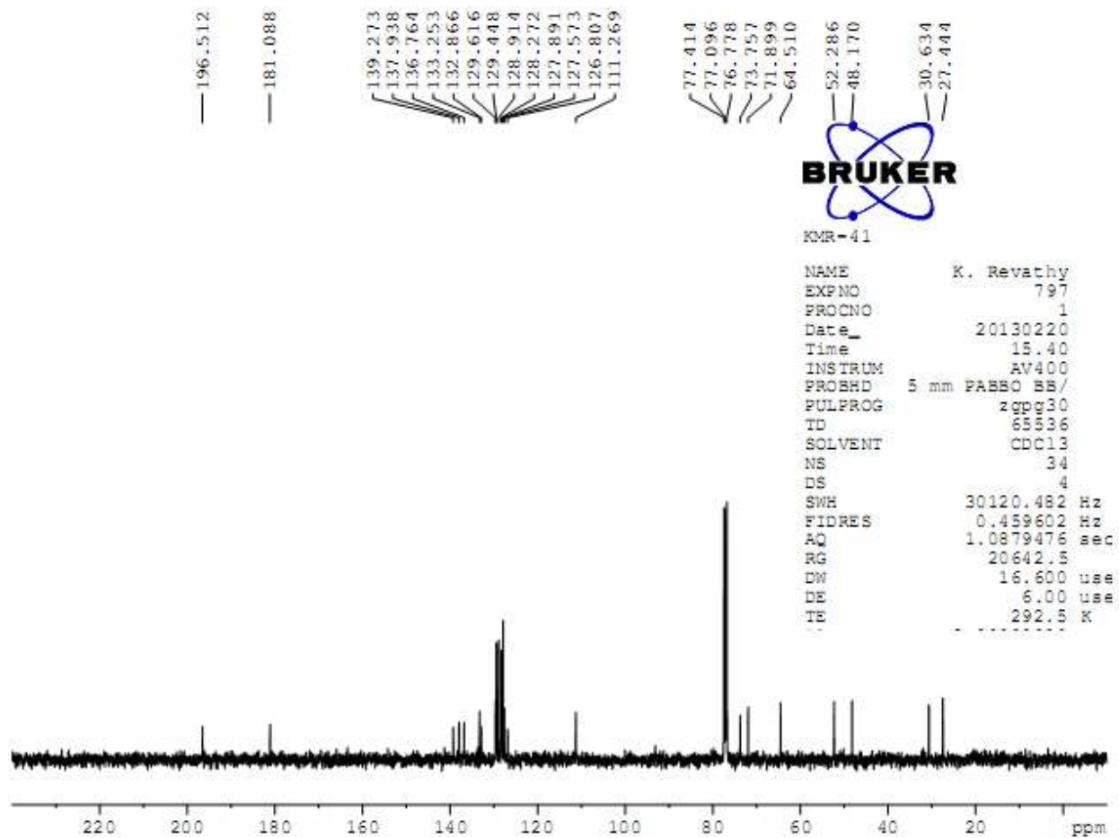
13 C NMR Spectrum of 6i
