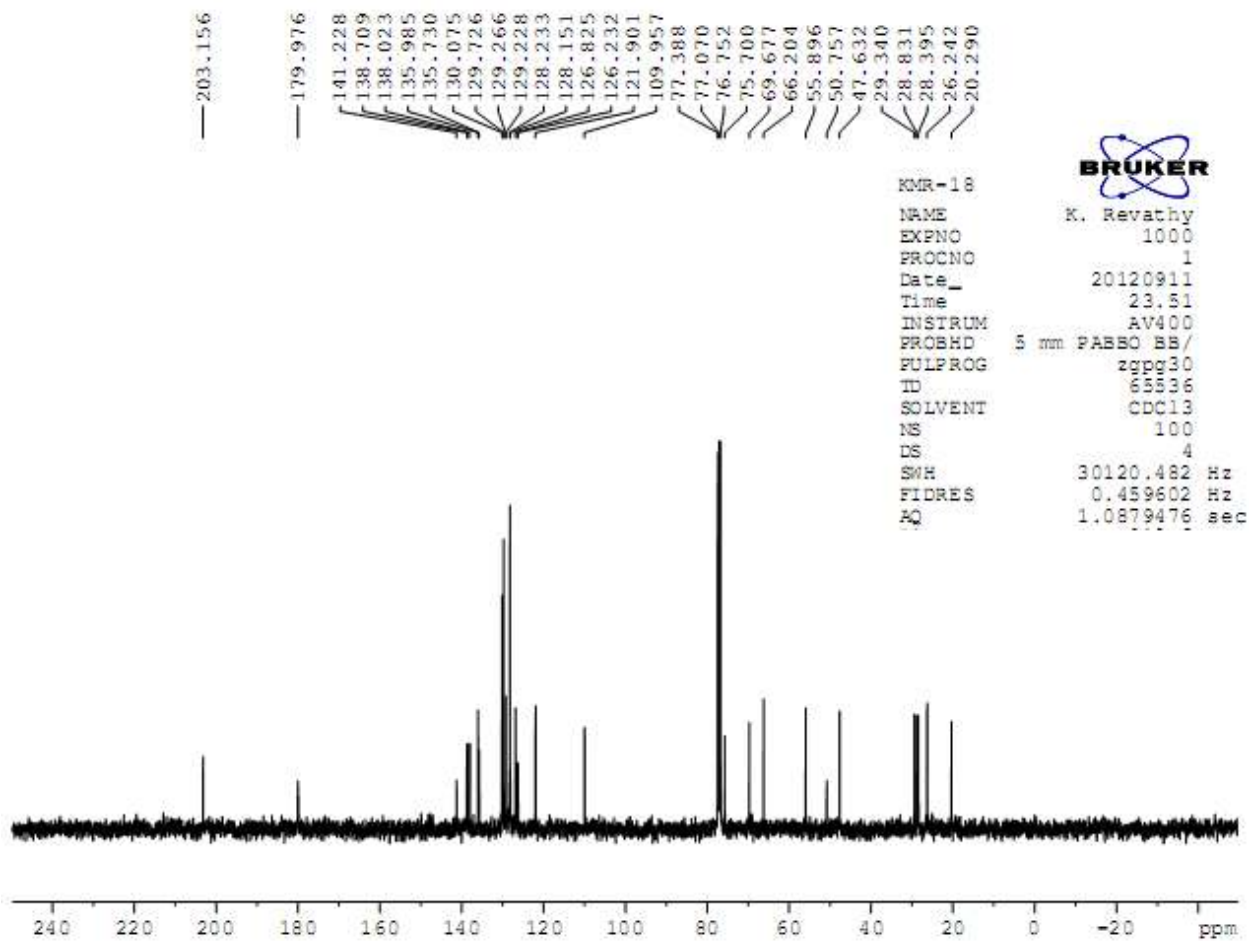
13 C NMR Spectrum of 8a
