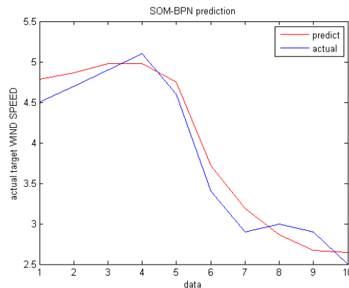
Fig. 2: Predicted/actual output wave form
