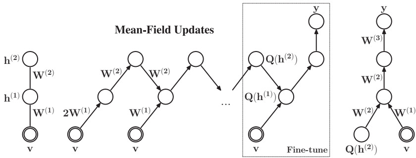
Figure 6: (Left) A two-hidden-layer Boltzmann machine. (Right) After learning, the DBM model is used to initialize a multilayer neural network. The marginals of approximate posterior q(h_j^{(2)} = 1|\mathbf{v}) are used as additional inputs. The network is fine-tuned by backpropagation.
