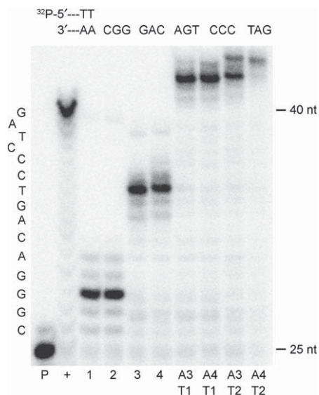
Figure 2. Primer extension in the presence of two functionalized dNTPs. 5 32 P end labeled primer template (sequences as indicated in the figure) were incubated with double substituted combinations of functionalized dNTPs. P: Radiolabeled Primer; +: natural dNTPs; 1: A3 , dCTP, dGTP; 2: A4 , dCTP, dGTP; 3: T1 , dCTP, dGTP; 4: T2 , dCTP, dGTP; A3T1: A3 , T1 , dCTP, dGTP; A4T1: A4 , T1 , dCTP, dGTP; A3T2: A3 , T2 , dCTP, dGTP; A4T2: A4 , T2 , dCTP, dGTP.
