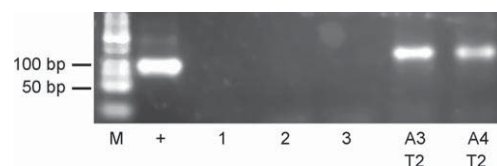
Figure 4. Generation of functionalized DNA duplexes in the presence of two modified dNTPs. M: Marker; +: natural dNTPs; 1: A3 , dCTP, dGTP; 2: A4 , dCTP, dGTP; 3: T2 , dCTP, dGTP; A3T2: A3 , T2 , dCTP, dGTP; A4T2: A4 , T2 , dCTP, dGTP.
