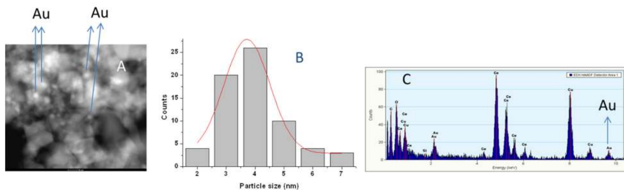
Figure 1. STEM image of (A) Au/nCeO 2 (Scale is 10 nm) (B) Particle size distribution (C) Representative XEDS spectrum for an individual Au particle.
