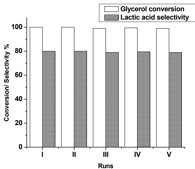
Figure 5. Recycle experiments for Au-Pt nCeO 2 (conditions for each experiment: 0.17 M glycerol, NaOH to glycerol mol ratio of 4, glycerol to metal mol ratio of 680, 100°C, P (O 2 ) = 5 bar, 30 min)
