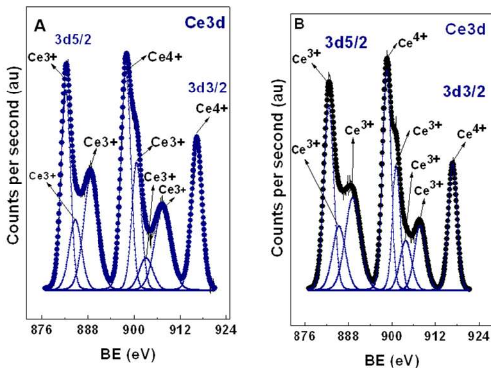
Figure 4. XPS spectra showing the Ce 3d core level of Au/nCeO 2 (A) and Au-Pt/nCeO 2 (B)
