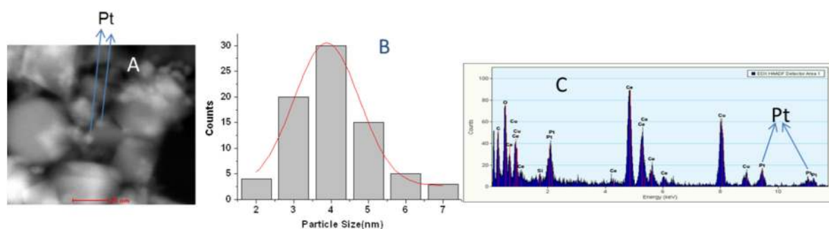
Figure 2. STEM image of (A) Pt/nCeO 2 (Scale is 20 nm) (B) Particle size distribution (C) Representative XEDS spectrum for an individual Pt particle.
