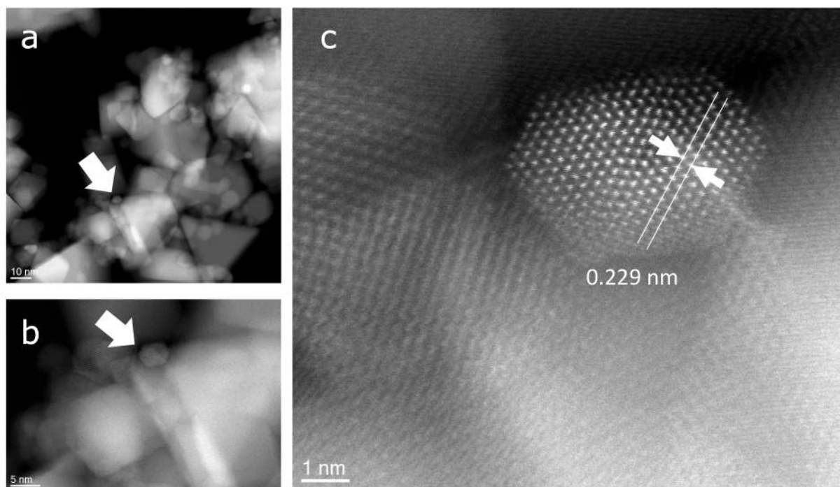
Figure 4. High-resolution TEM at different magnifications ( a , b ) showing the ceria and Au/Pt particles and ( c ) Atomic-resolution TEM image of a bimetallic cluster indicating the lattice spacing.
