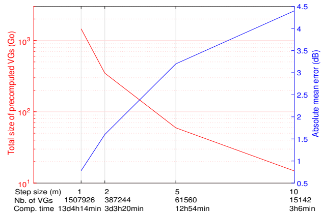
FIGURE 12. Absolute mean error and storage size vs step size, and the corresponding number of VGs and computation time.
