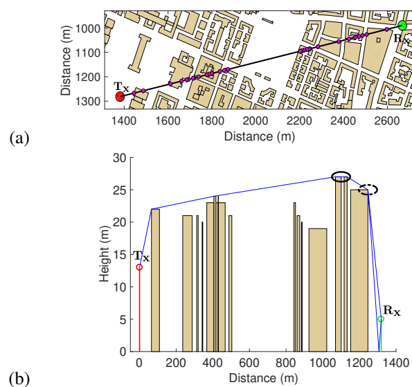
FIGURE 14. (a) Considered link in Munich, (b) extracted vertical profile.
