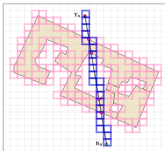
FIGURE 13. Principle of vertical profile extraction.
