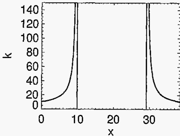
Figure C1. The number of iterations, k , needed for \zeta to change from \zeta_{\max} to \zeta_{\min} , as a function of x . The vertical lines indicate the break-points, between which \zeta = \zeta_{\max} . The number of steps required for the solution to reach steady state is given approximately by the largest value of k at the gridpoints nearest the break-points, about 140 in this case.
