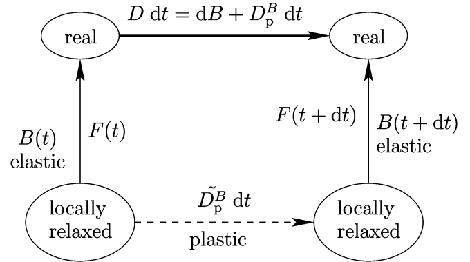
Fig. 12. Incompressibility and plasticity. The incompressible evolution \tilde{D}_p^B of the relaxed conformation implies the usual property \text{tr}(\tilde{D}_p^B) = 0 . Despite this, the corresponding flow D_p^B in real space is not traceless in general ( \text{tr}(D_p^B) \neq 0 ): it is related to \tilde{D}_p^B through a finite transformation B , see equation (38) for details.
