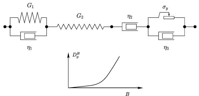
Fig. 26. Combined Bingham-Burger model: schematic diagramme (top) and plot (bottom) of plastic flow as a function of tensor B , in the stationary regime. In a combined Bingham-Burger model, the plastic flow would increase weakly with the applied stress at low stresses, and more strongly above the yield stress. We believe it would mimic the rheological behaviour of a foam quite adequately.
