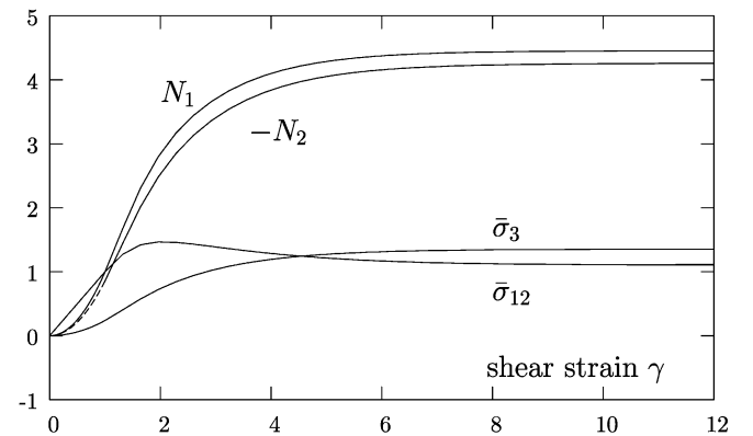
Fig. 20. Shear stress \bar{\sigma}_{12} , deviatoric stress \bar{\sigma}_3 in the vorticity direction and normal stress differences N_1 and N_2 in the course of an experiment as a function of the shear deformation \gamma , for \dot{\gamma} = 8 .
