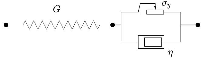
Fig. 5. With the Bingham model, from which we develop a fully tensorial model in the present work, the response to weak stresses is elastic (modulus G ); by contrast, the response to large stresses presents both a yield threshold ( \sigma_y ) and a viscous component ( \eta ).
