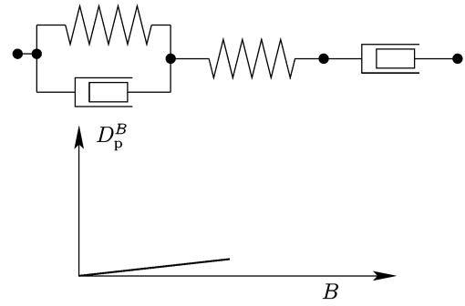
Fig. 24. Burger model: schematic diagramme (top) and plot (bottom) of plastic flow as a function of tensor B , in the stationary regime and under small applied stresses. In Burger's model, suitable for foams under low applied stresses (see Sect. 3.1), the plastic flow increases with the applied stress. If we neglect the short time scale response provided by the Voigt-Kelvin element (spring and viscous element in parallel), then this increase is weak and linear, as determined by the viscous element in series.
