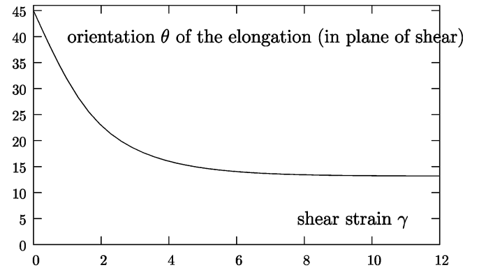
Fig. 19. Orientation of the stored elastic deformation in the course of an experiment as a function of the shear deformation \gamma . The applied shear rate is \dot{\gamma} = 8 .
