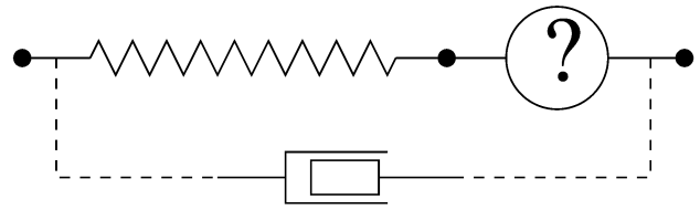
Fig. 3. The considerations of Section 2.4 lead us to the idea of a rheological model consisting in a spring in series with some creeping element yet to be defined. The long, soft spring reflects the fact that creep may trigger at rather large elastic (stored) deformations. Optionnally, an additional “ dilute regime ” viscous element may be added in parallel: in a context of imposed deformation, it will not alter the dynamics of the system.
