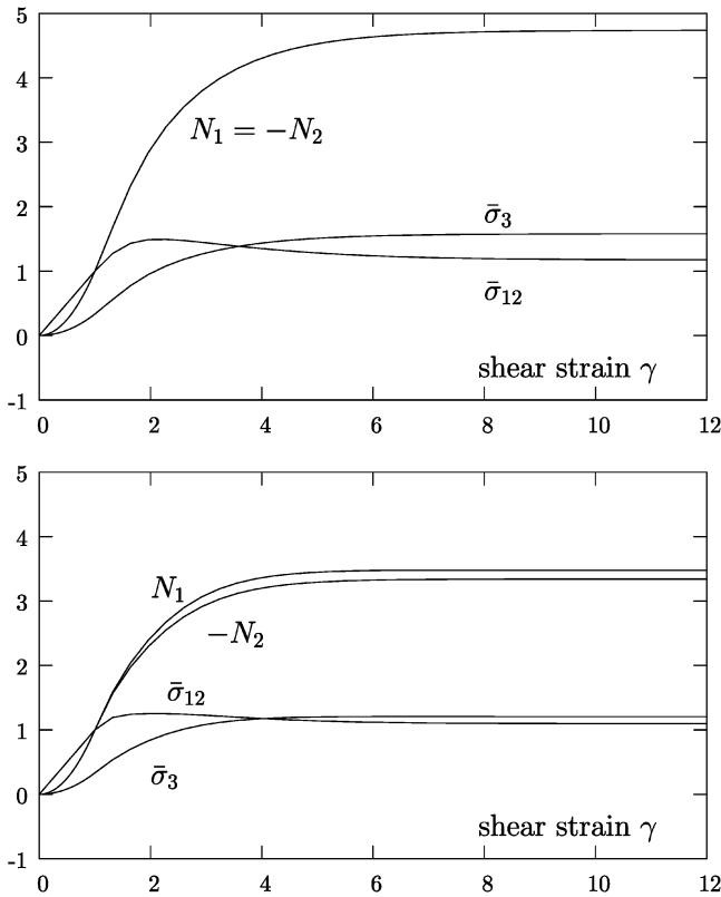
Fig. 23. Impact of plasticity on the stress response. The shear stress \bar{\sigma}_{12} , the deviatoric stress \bar{\sigma}_3 in the vorticity direction and the normal stress differences N_1 and N_2 are plotted as a function of the shear deformation \gamma , for a shear rate \dot{\gamma} = 8 . Mooney-Rivlin elasticity is chosen with k_1 = 0 and k_2 = 1 . The plastic deformation rate is taken as expressed by equation (41) with b_1 = (\text{tr } B - 4)\theta(\text{tr } B - 4) . Parameter b_2 is varied. Top: b_2 = 0 . Bottom: b_2 = b_1 .
