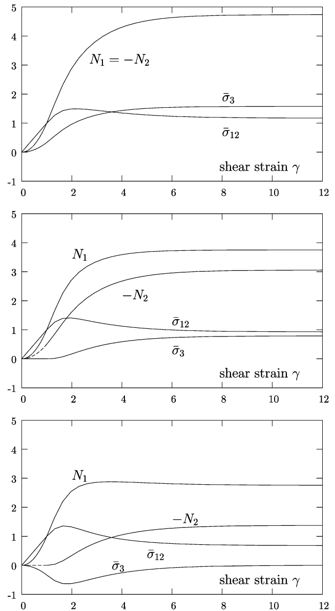
Fig. 22. Impact of elasticity on the stress response. The shear stress \bar{\sigma}_{12} , the deviatoric stress \bar{\sigma}_3 in the vorticity direction and the normal stress differences N_1 and N_2 are plotted as a function of the shear deformation \gamma , for a shear rate \dot{\gamma} = 8 . Mooney-Rivlin elasticity is chosen with different parameter values. Top: k_1 = 0 and k_2 = 1 . Center: k_1 = 1/2 and k_2 = 1/2 . Bottom: k_1 = 1 and k_2 = 0 .
