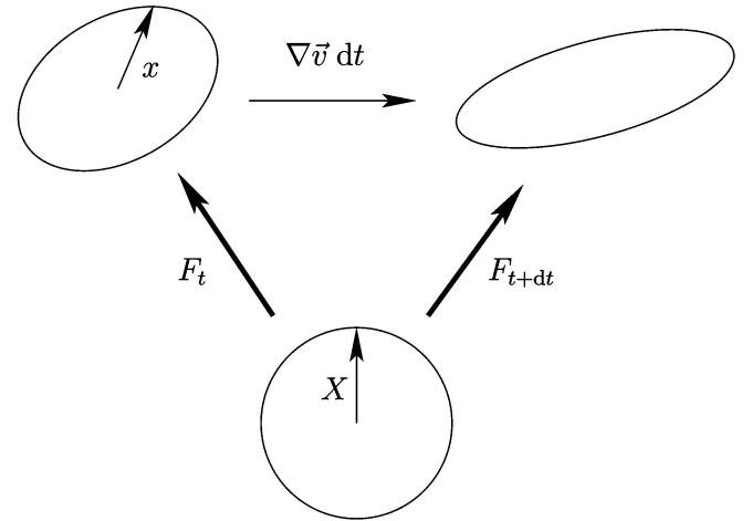
Fig. 9. Variation of the local material stored deformation (see Fig. 2) that corresponds to an infinitesimal displacement field. As described by equation (11), tensor F describes the transformation from the relaxed, reference state (sphere, generic point \bar{X} ) to the current state (ellipsoid, generic point \bar{x} ). F is chosen to be a pure deformation, while \nabla\vec{v} dt may include some rotation. In this example, the evolution of tensor F is purely kinematic (see App. A), as the material is supposed to behave in a reversible, elastic manner here. See Figure 28 for details on the relaxed state.
