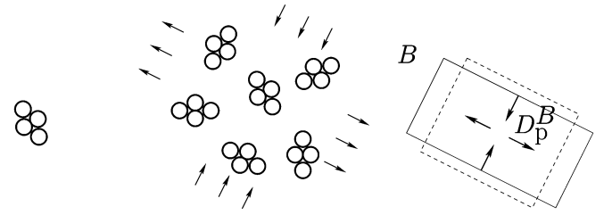
Fig. 11. From T1 process to plastic flow. Left: the stress needed for four bubbles to undergo a T1 process is illustrated in Figure 10. Centre: when a chunk of material contains a number of quadruplets of bubbles with various orientations, it may be postulated that the plasticity threshold corresponds to the most favourably oriented quadruplet (this assumption discards the effects of non-homogeneous deformations, and is discussed in the main text). Right: the rate at which T1 processes occur in the chunk of material when it is subjected to elongation B is expressed in the form of a plastic flow D_p^B , where the material configuration at time t (dashed line) is mapped onto configuration at time t + dt (full line) through infinitesimal deformation D_p^B dt .
