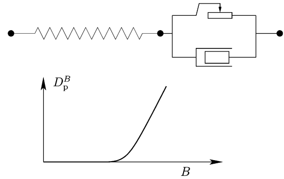
Fig. 25. Bingham model: schematic diagramme (top) and plot (bottom) of plastic flow as a function of tensor B , in the stationary regime. In a model based on Bingham's model, such as that developed in the present work, the plastic flow is zero up to a certain stress (yield stress). Beyond the yield stress, it increases (linearly with the applied stress).
