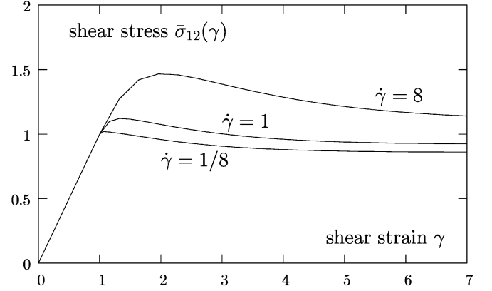
Fig. 13. Shear stress \bar{\sigma}_{12} in the course of a shear experiment, as a function of the shear deformation \gamma , for three different shear rate values \dot{\gamma} . The elasticity and plasticity terms are chosen as described in Section 8.2. The response increases during the initial period of time, when the material deforms purely elastically (as expected, the response is then independent of the shear rate). The increase then levels off once the plasticity threshold has been reached, and saturates at a stationary value. For a plot of the final, stationary value on the applied shear rate, see Figure 15.
