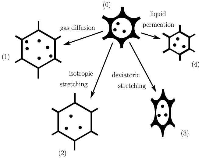
Fig. 7. Four changes in the local structure of a foam. (0) Initial structure. (1) Structure obtained through diffusion of gas from neighbouring regions into the bubble: the number of gas molecules in the bubble (represented by black dots) has increased, while the amount of liquid that surrounds the bubble has not changed. (2) Structure obtained by isotropic stretching: the quantity of gas and the quantity of liquid have not changed. This is not a stress-free conformation. (3) Structure obtained by deviatoric stretching: the volume, the quantity of gas and the quantity of liquid have not changed. This is not a stress-free conformation. (4) Structure obtained by permeation of liquid from the vicinity of the bubble towards other places in the foam: the amount of liquid that surrounds the bubble has decreased, while the number of gas molecules has not changed. In the present work, only changes where both phases are transported simultaneously , such as (0) \rightarrow (2) and (0) \rightarrow (3), are considered.
