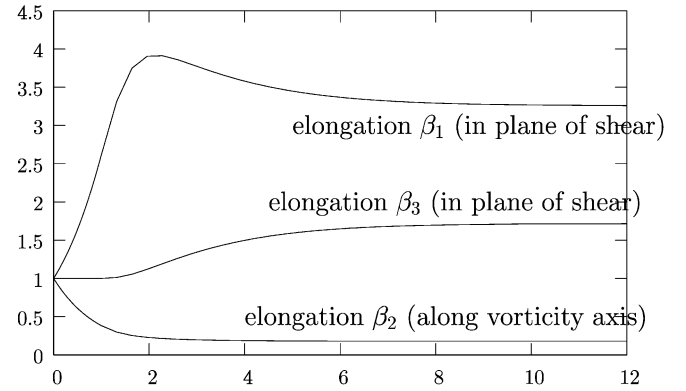
Fig. 18. Eigenvalues of the stored elastic deformation in the course of an experiment as a function of the shear deformation \gamma . The applied shear rate is \dot{\gamma} = 8 .
