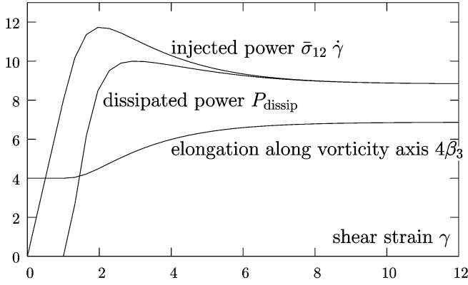
Fig. 14. Dissipation P_{\text{dissip}} per unit volume and injected power \bar{\sigma}_{12} \dot{\gamma} in the course of a shear experiment, as a function of the shear deformation \gamma . The applied shear rate is \dot{\gamma} = 8 . The elasticity and plasticity terms are chosen as described in Section 8.2. Note that there is no dissipation ( P_{\text{dissip}} = 0 ) in the elastic regime, prior to the onset of plasticity. Part of the injected work is not dissipated (non-zero surface area between both curves) and corresponds to the elastic energy stored in the material.
