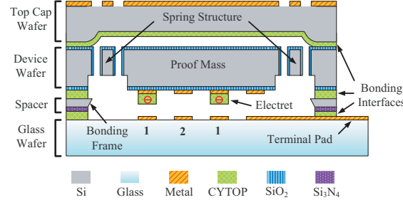
Figure 1. Schematic view of the 4-wafer stack structure for the energy harvesting device. The device is composed of four wafers, namely, Top Cap , Device , Spacer and Glass . The four wafers are bonded together with adhesive polymer in a thermo-compression bonding technique.
