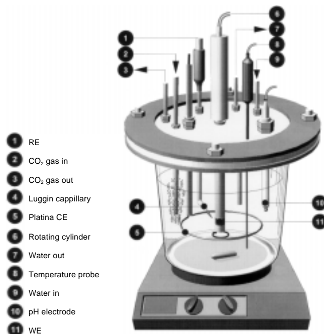
FIGURE 1. Schematic of the experimental cell.
