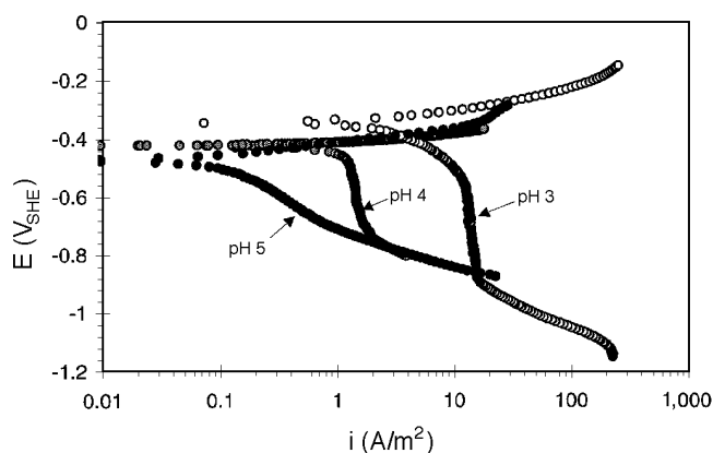
FIGURE 11. pH effect in HCl solution, water + 3% NaCl, P_{\text{N}_2} = 1 bar (100 kPa), t = 20^\circ\text{C} , 1,000 rpm, \tau = 1.7 Pa, \text{Re} = 5,235 , and St52 steel.
