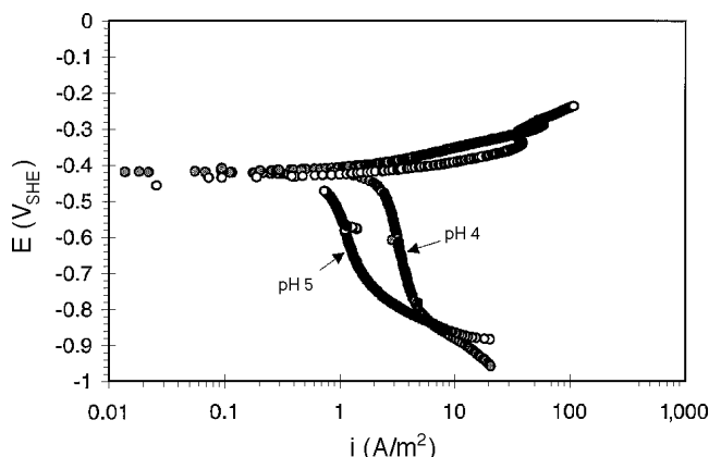
FIGURE 12. pH effect in \text{CO}_2 solution, water + 3% NaCl, P_{\text{CO}_2} = 1 bar (100 kPa), t = 20^\circ\text{C} , 1,000 rpm, \tau = 1.7 Pa, \text{Re} = 5,235 , and St52 steel.
