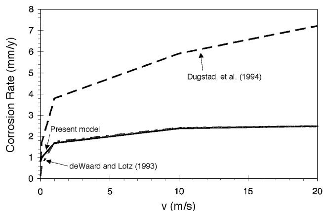
FIGURE 19. Comparison of predicted velocity effects on the corrosion rate for the case of a solution saturated with P_{\text{CO}_2} = 1 bar (100 kPa), pH 4, t = 20^\circ\text{C} , and d_{\text{pipe}} = 25 mm (0.98 in.).
