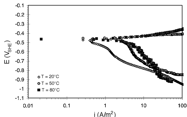
FIGURE 15. Temperature effect in CO 2 solution, water + 1% NaCl, P CO 2 = 1 bar (100 kPa), pH 5, and static using X-65 steel.
