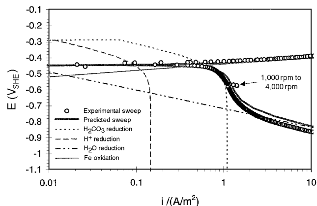
FIGURE 10. Velocity effect in \text{CO}_2 solution at pH 5, water + 3% NaCl, P_{\text{CO}_2} = 1 bar (100 kPa), t = 20^\circ\text{C} , and St52 steel.
