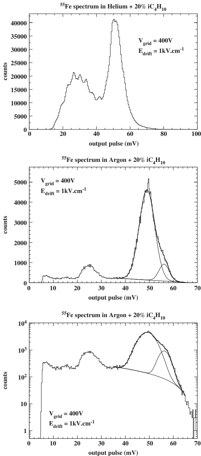
Fig. 5. Measured pulse height from ^{55}\text{Fe} source for a He/isobutane 80/20 mixture (top) and for an Ar/isobutane 80/20 mixture (middle/bottom in linear and logarithmic scale); the curves show the results of the fit to the pulse shape, showing the 5.9 and 6.5 keV lines and their superposition on a linear 'background'.
