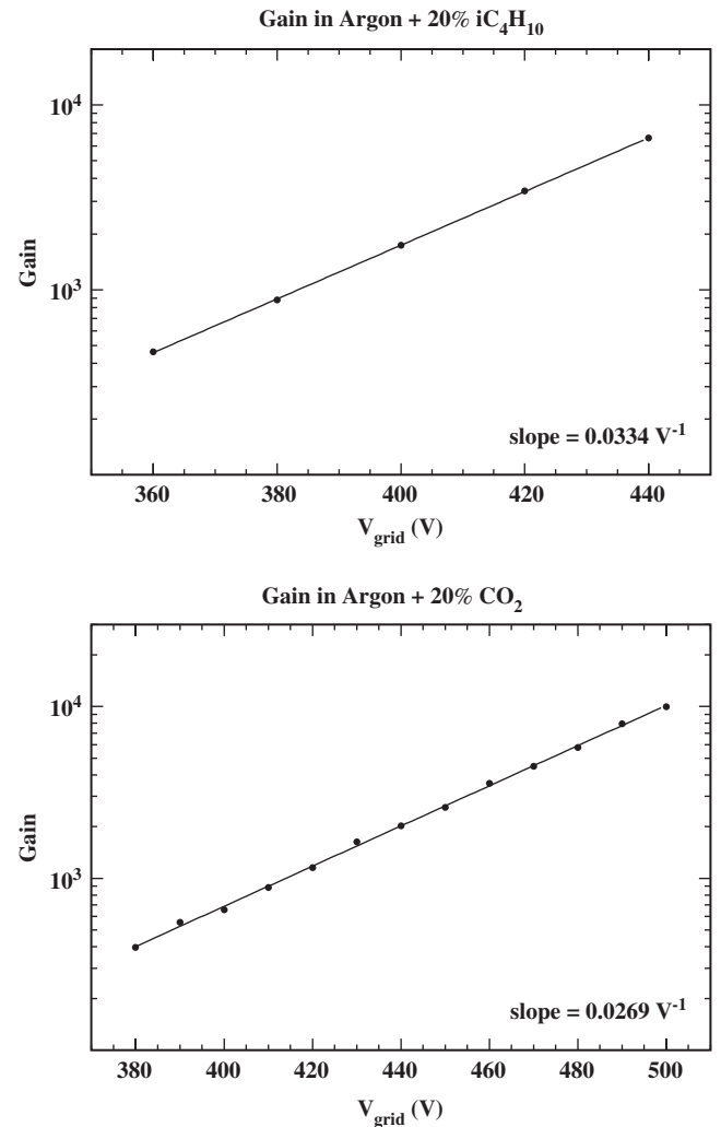
Fig. 6. Measured gas gain vs. grid voltage for Ar/isobutane 80/20 (top) and for Ar/ \text{CO}_2 80/20 (bottom).
