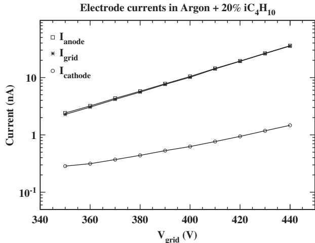
Fig. 7. Measured anode, grid and cathode currents vs. the grid voltage for the Ar/isobutane 80/20 mixture.
