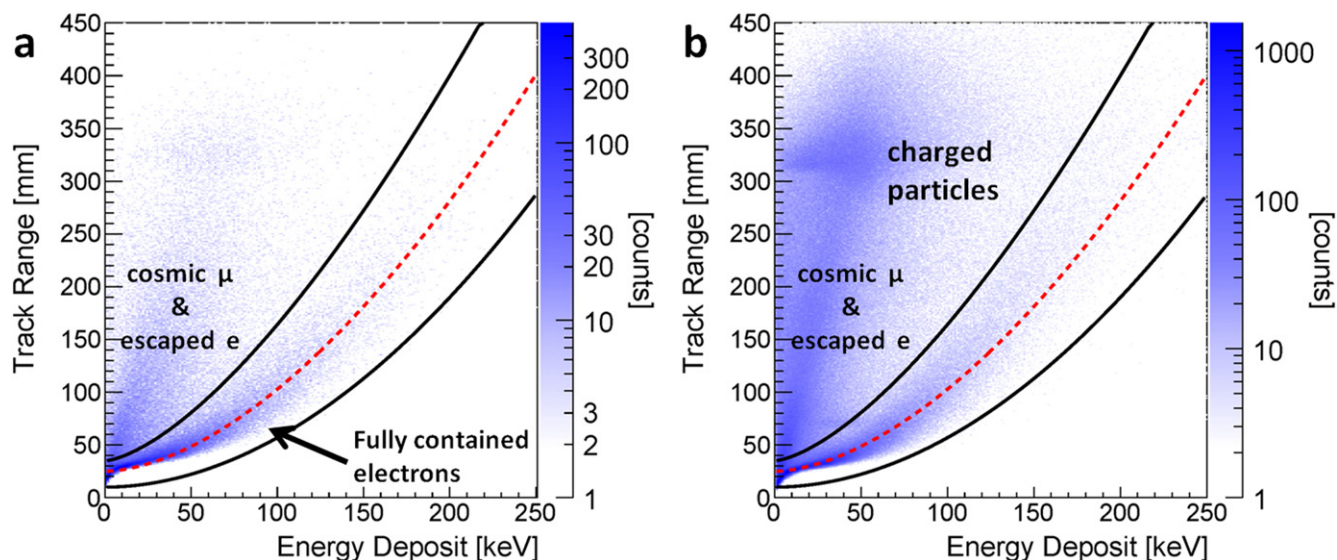
Figure 2. Correlations of the track length and energy deposit in the TPC (a) under the condition of gamma-ray irradiation from ^{137}\text{Cs} (3 MBq) at a distance of 1 m in the laboratory, (b) under the intense radiation generated by a 140 MeV proton beam. In all figures, the fully contained electrons are clearly separated from the minimum ionizing charged particles, e.g., cosmic muons, high-energy electrons, and neutron-recoil events.
