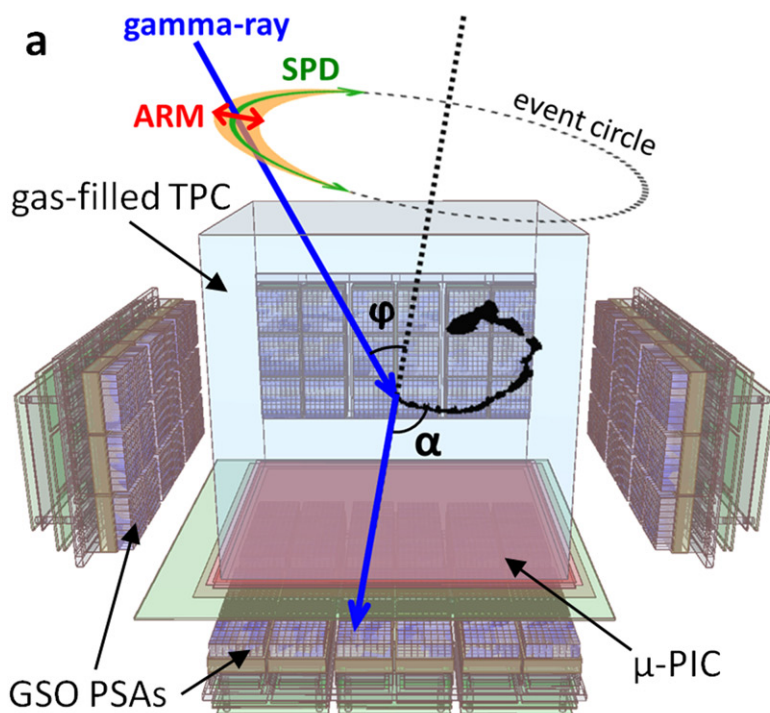
Figure 1. (a) Schematic view of SMILE-II 30 cm-cubic ETCC. A micro-pattern gas detector (MPGD), which consists of 400 \mu\text{m} pitch pixels, is installed at the bottom of the TPC, of which anodes and cathodes are connected via strips to provide the two-dimensional position and charge of the track. One PSA consists of 64 GSO bars (bar size: 6 \times 6 \times 13 \text{ mm}^3 ) with 1 radiation length (R.L.). 36 PSAs are put at the bottom and 18 PSAs are on each side. A typical reconstructed track of a recoil electron is plotted in Figure 1(a), using an improved reconstruction method, where the vertical width of the hit point represents the TOT as a pulse width of each pixel. (b) Photograph of SMILE-II flight model instrument.
