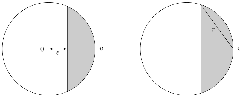
Figure 9. Left: \varepsilon -cap C(\varepsilon, v) about v . Right: cap of radius r about v .
