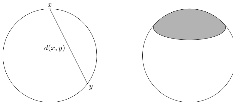
Figure 26. The Euclidean metric on the sphere. A spherical cap (right) is a ball for this metric.
