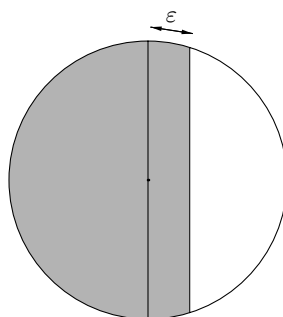
Figure 27. An \varepsilon -neighbourhood of a hemisphere.
