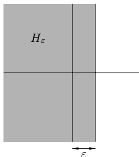
Figure 28. An \varepsilon -neighbourhood of a half-space.
