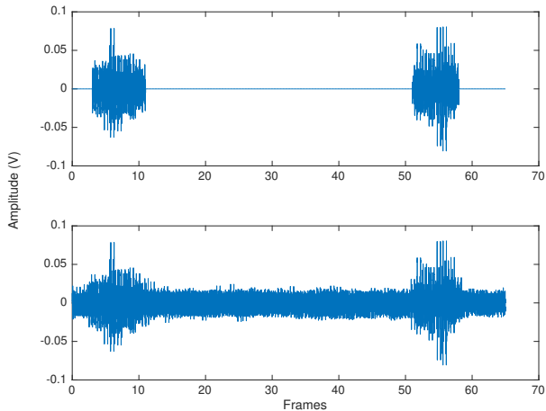
Figure 8: Part of the received sEMG signal before (bottom) and after (top) the contraction detection algorithm.
