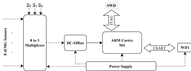
Figure 2: Overall sEMG data acquisition unit block diagram.
