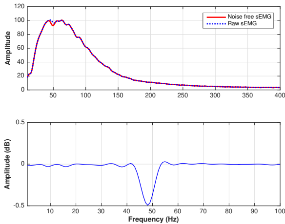
Figure 10: Average contraction frequency spectrum of cleared and raw sEMG signals(above) and the difference of those signals in dB scale (below)
