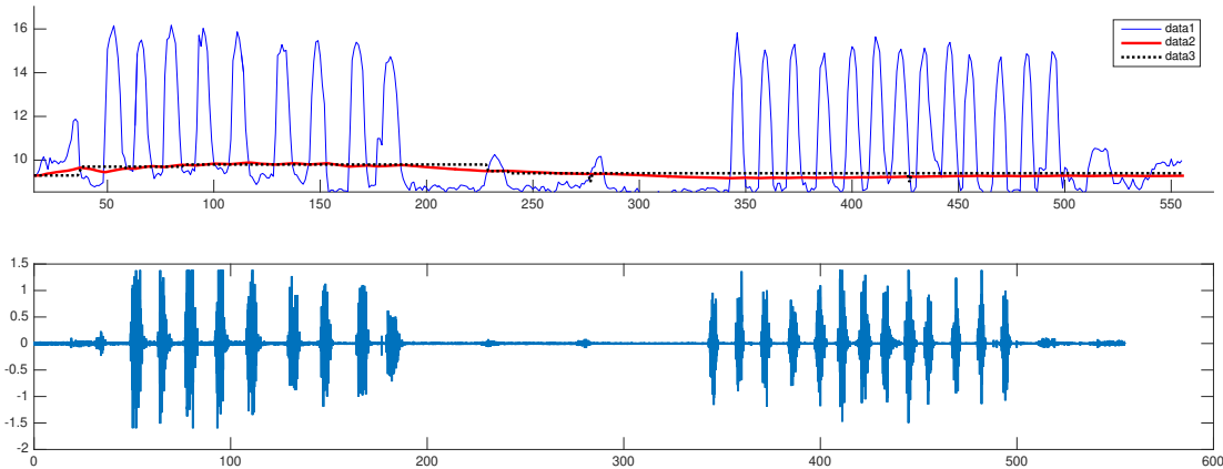
Figure 7: Plots of contraction detection classifier, adaptive threshold and true threshold of subject S7 (above) and plot of recorded sEMG signal (below)
