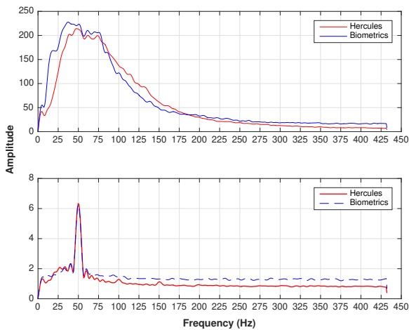
Figure 6: Average frequency Spectrum comparisons of contraction (top) and relaxation (bottom) frames of Biometrics and Hercules.
