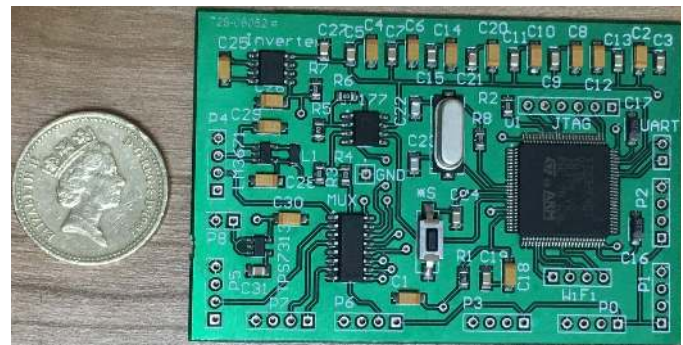
Figure 3: Photo of the eight channel sEMG data acquisition unit (DAU) PCB.
