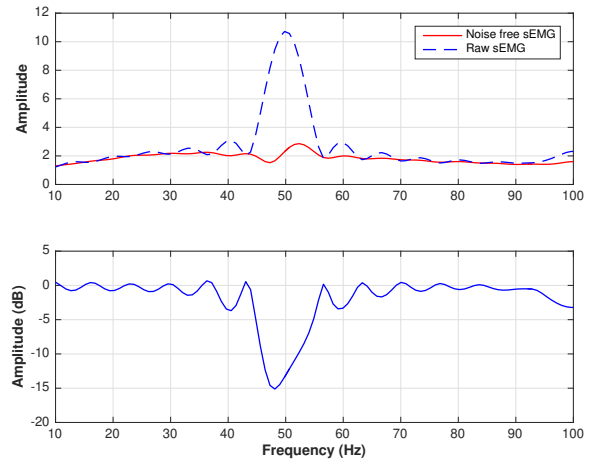
Figure 9: Average noise frequency spectrum of cleared and raw sEMG signals (above) and the difference of those signals in dB scale (below)
