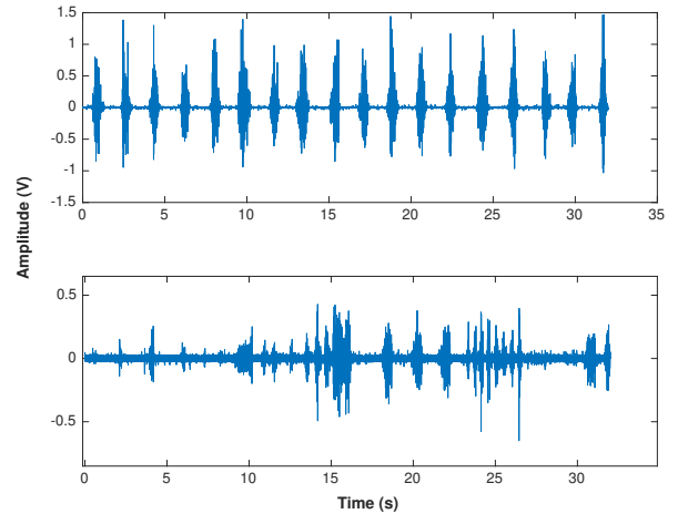
Figure 5: Plots of the selections of the sEMG signal stream of S2 from the group 1 (top) and S9 from the group 2 (bottom)
