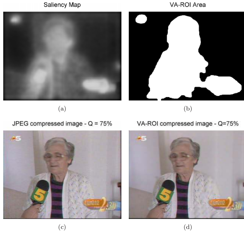
Fig. 5. An example of the visually salient areas identified using the proposed algorithm.
