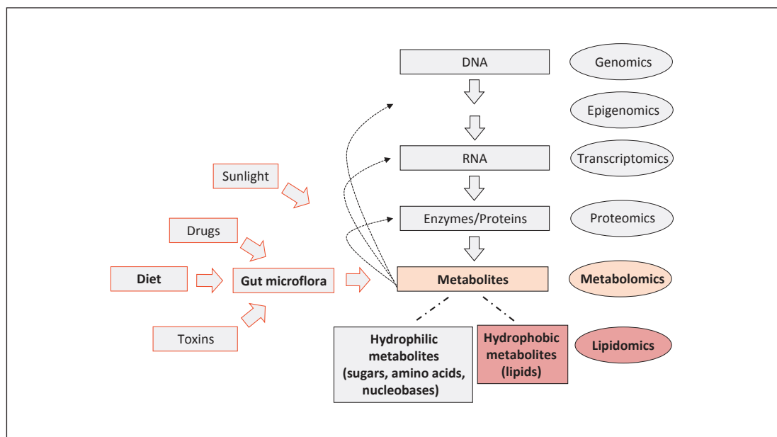
Fig. 3. Metabolomics in systems biology. Genes (DNA) encode mRNAs that, in turn, encode proteins that collectively, and together with environmental factors (e.g., diet), lead to the metabolite inventory of a cell, tissue, or body fluid. Metabolites, in turn, can regulate gene expression, enzymatic activities, and protein functions. Among the metabolites are lipids. Novel approaches now allow for qualitative and quantitative measurements at each level on global scales (genomics, epigenomics, proteomics, and metabolomics). Lipidomics can be viewed as a subdiscipline of metabolomics under the umbrella of systems biology.
