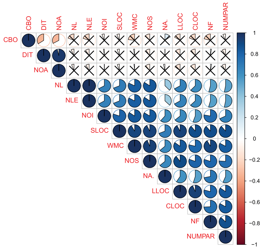
FIGURE 6 Correlation matrix for the source code metrics of the sampled contracts (insignificant correlations [i.e., < 0.01] are crossed out). CBO, coupling between objects; CLOC, comment lines of code; DIT, depth of inheritance tree; LCOM, lack of cohesion in method; LLOC, logical lines of code; McCC, McCabe’s cyclomatic complexity; NA, number of attributes or states; NF, number of functions; NL, nesting level; NLE, nesting level without else-if; NOA, number of ancestors; NOC, number of children; NOD, number of dependencies; NOI, number of outgoing invocation; NOS, number of statement; NUMPAR, number of parameter; OO, objective-oriented; SLOC, source lines of code; WMC, weighted methods per class
