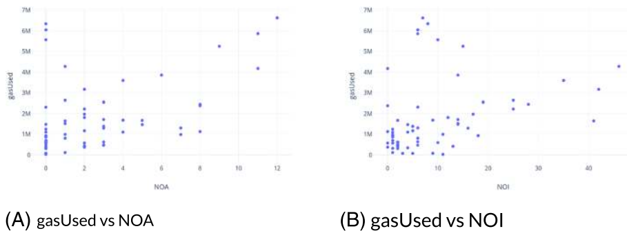
FIGURE 8 Spearman's rank correlation plots for source code metrics ((A) gasUsed vs. NOA and (B) gasUsed vs. NOI) that show the strongest and statistically significant correlations with the gasUsed metric (post-deployment). NOA, number of ancestor; NOI, number of outgoing invocation
