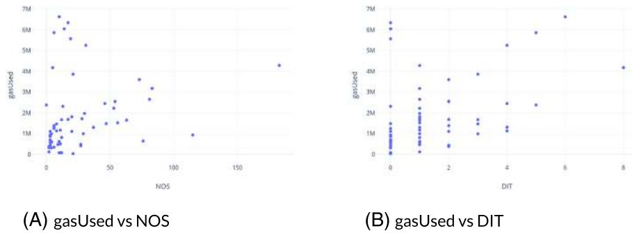
FIGURE 7 Spearman's rank correlation plots for source code metrics ((A) gasUsed vs. NOS and DIT) that show the strongest and statistically significant correlations with the gasUsed metric (post-deployment). DIT, depth of inheritance tree; NOS, number of statement
