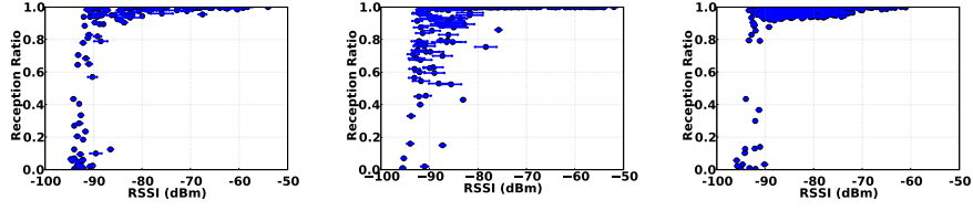
(a) Mirage, IPI = 50ms, Channel 26. (b) Lake, IPI = 50ms, Channel 26. (c) University, IPI = 50ms, Channel 26.
