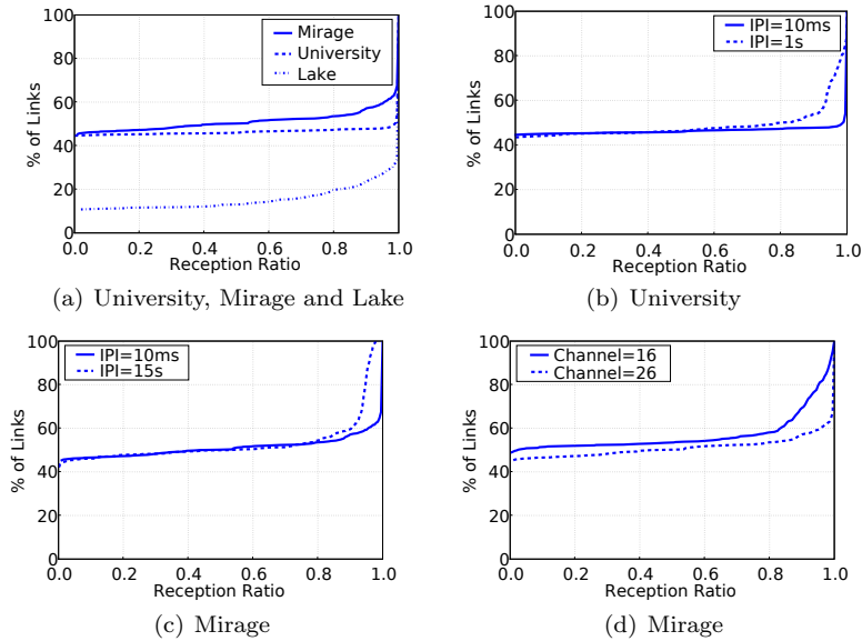
Fig. 3. (a-c) show cumulative distribution functions (CDFs) of link qualities in the three testbeds for channel 26 at different IPIs. The percentage of intermediate links is small compared to good and bad links. It increases as the inter-packet interval increases. (d) shows CDFs of link qualities in Mirage on channels 16 and 26. Channel affects the percentage of perfect links and the percentage of intermediate links.
