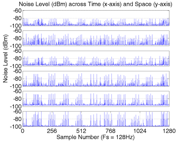
Fig. 15. Sampled signal strength over 10s and across six nodes.
