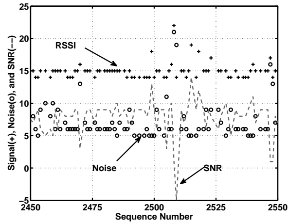
Fig. 25. Signal power (+), noise power (o), and signal-to-noise ratio (- -) versus packet sequence number for a single link from the Roofnet traces. The transmit rate is approximately 78 packets per second. Units of power are reported in dBm with an unknown offset. Signal and noise both vary significantly over time.
