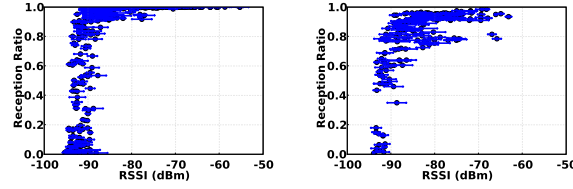
(d) Mirage, IPI = 15s, Channel 26. (e) University, IPI = 10s, Channel 26.
