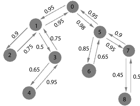
Fig. 1. The Conceptual Model. The graph does not show temporal and spatial correlation observed reception ratios. It does not show if the channel of operation is relevant to protocol performance. It assumes that the observed reception ratio is the same for both data and acknowledgement packets.
