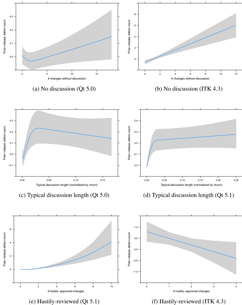
Fig. 10 The estimated count of post-release defects in a component for varying participation metrics. The blue line indicates the values of our model fit on the original data, while the grey area shows the 95% confidence interval based on models fit to 1,000 bootstrap samples.
