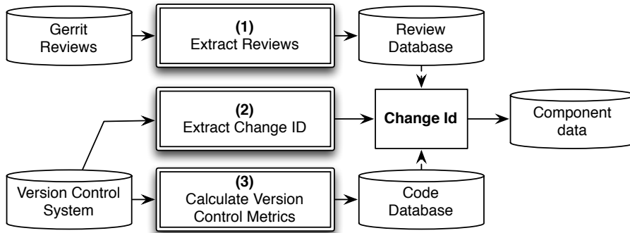
Fig. 2 Overview of our data extraction approach.
