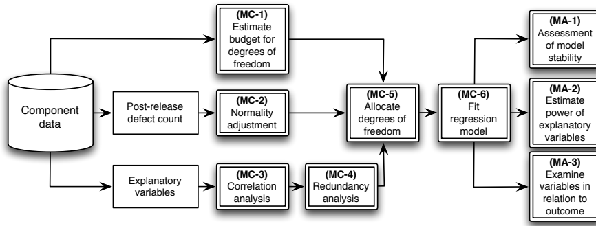
Fig. 3 Overview of our Model Construction (MC) and Model Analysis (MA) approach.
