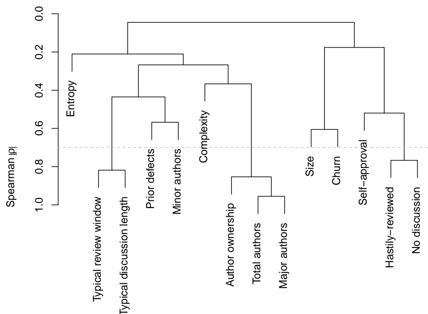
Fig. 8 Hierarchical clustering of variables according to Spearman's |\rho| in Qt 5.0 (RQ2).
