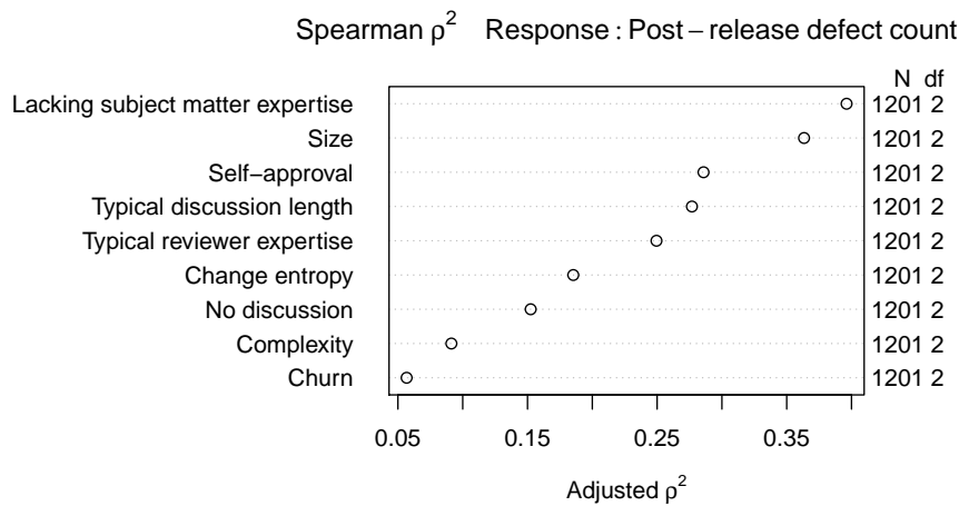
Fig. 12 Dotplot of the Spearman multiple \rho^2 of each explanatory variable and the post-release defect count in Qt 5.0. Larger values indicate a more potential for non-monotonic relationship (RQ3).
