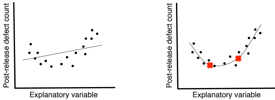
Fig. 4 An example of a non-monotonic relationship that would benefit from knots. The plot on the left shows that a linear fit would not fit the relationship well, whereas the plot on the right has been allocated two knots (red 'X' shapes), and allows each region between the knots to have a different fit to improve the accuracy of the overall fit.
