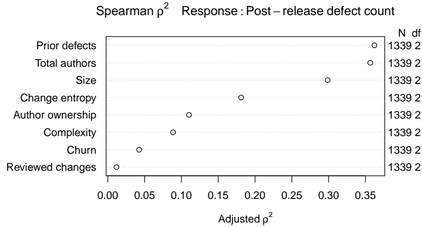
Fig. 6 Dotplot of the Spearman multiple \rho^2 of each explanatory variable and the post-release defect count in Qt 5.0. Larger values indicate a more potential for non-monotonic relationship (RQ1).
