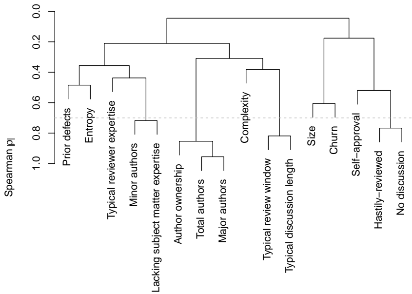
Fig. 11 Hierarchical clustering of variables according to Spearman's |\rho| in Qt 5.0 (RQ3).
