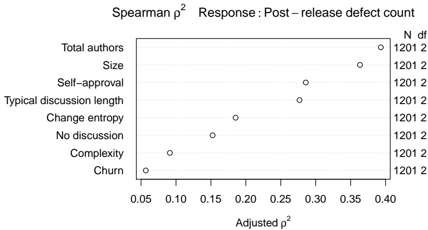
Fig. 9 Dotplot of the Spearman multiple \rho^2 of each explanatory variable and the post-release defect count in Qt 5.0. Larger values indicate a more potential for non-monotonic relationship (RQ2).
