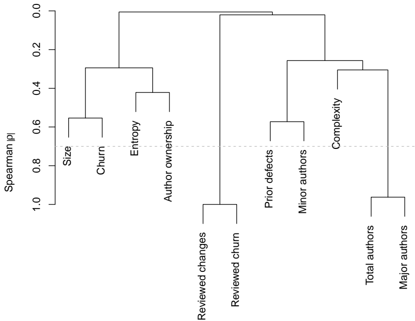
Fig. 5 Hierarchical clustering of variables according to Spearman's |\rho| in Qt 5.0 (RQ1).
