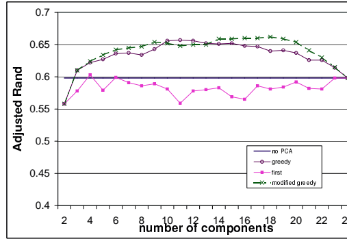
Figure 14: Average adjusted Rand index against the number of components using k-means and Euclidean distance on the mixture of normal distributions of the ovary data.
