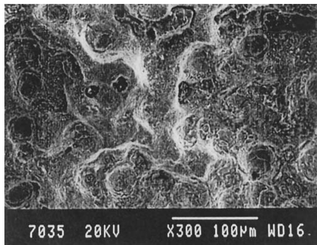
Figure 4 Transgranular fracture surface of a low cycle fatigue specimen tested at 700°C with a strain rate of 10 -3 s -1 .
