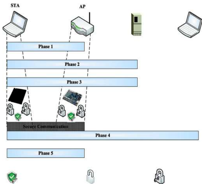
Fig. 2. IEEE 802.11i modified phases of operation.
