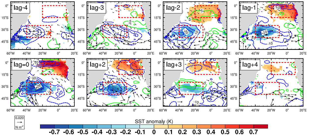
FIG. 8. Composite evolution maps of the anomalies of HadISST monthly SST (K; color scale), Q_{net} ( W m^{-2} ; contours), and winds stress ( N m^{-2} ; arrows) based on the SAOD index fixed at lag = 0, corresponding to June. Only statistically significant ( P \leq 0.05 ) SST anomalies are shown, while significant ( P \leq 0.05 ) wind stress anomalies are represented by thick black arrows. The Q_{net} is contoured at an interval of 5 W m^{-2} ; positive anomalies shown by green contours indicate that the ocean mixed layer is gaining heat, and the negative anomalies (dashed blue contours) show that the ocean mixed layer is losing heat. The top (bottom) two rows of panels are based on the ORAS3 (GECCO2) dataset. All composites are based on the period 1960–2009.
