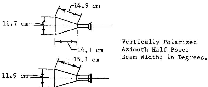
Figure 28. 15 db Gain Horn Used in the Second Test for Measuring Quiet Zone Reflectivity.
