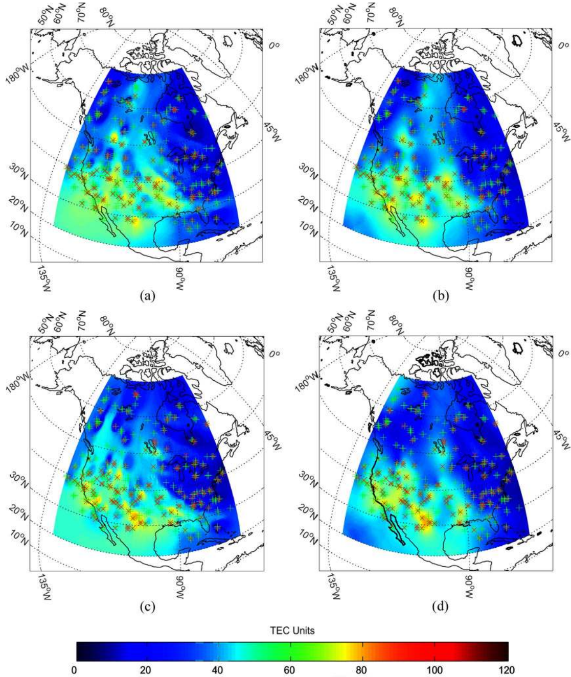
Fig. 10. Example output images produced by ANC and kriging using two sets of the input data from Fig. 8(c). Each set consisted of 25% of the available data ( \times ) and the remaining data ( + ) used to calculate the proportional rmse. (a) and (b) Set 1 results (sparsity of 98.94%) produced by ANC and kriging, respectively. (c) and (d) Set 2 results (sparsity of 98.79%) produced by ANC and kriging, respectively. The proportional rmse values are (a) 0.0640, (b) 0.0533, (c) 0.0503, and (d) 0.0421 TEC units.
