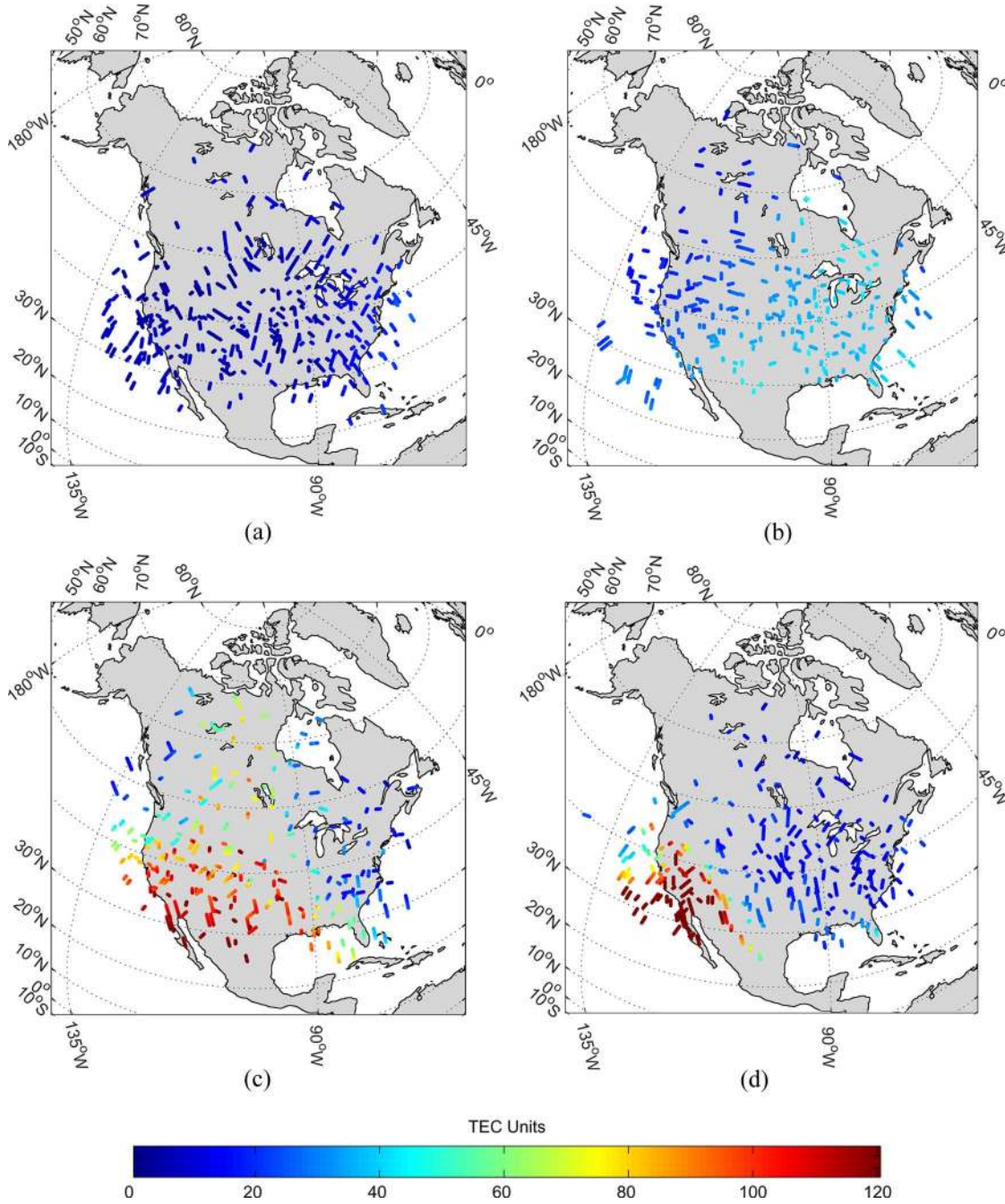
Fig. 8. Example TEC input data for the cross-validation test in Section IV-B. All data are from October 30, 2003 for the time periods (a) 1200–1215 UT, (b) 1600–1615 UT, (c) 2000–2015 UT, and (d) 0000–0015 UT in October 31.
