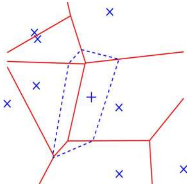
Fig. 1. Voronoi diagram showing (dotted line) new cell overlapping cells from the original tessellation.
