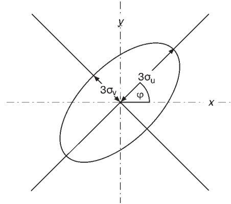
Fig. 3. Example of 2-D Gaussian filtering, as used in ANC, with major and minor axes (of size 3\sigma_u and 3\sigma_v , given by (13) and (14) respectively) rotated by the angle \varphi , given by (11).
