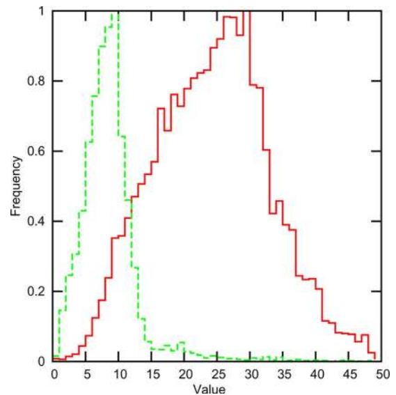
Fig. 4. Normalized histograms of the two types of simulated correlated data described in Section IV-A. (Solid) Multivariate and (dashed) univariate.
