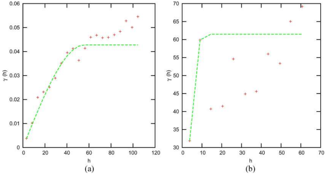
Fig. 2. Semivariograms (+) and (dashed lines) automatically fitted spherical model of (8). (a) Simulated correlated data demonstrating a good fit and (b) degenerate TEC data showing a poor fit.
