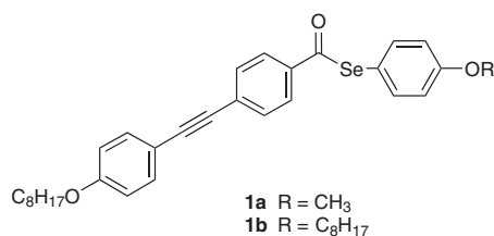
Figure 1. Selenoesters-LC 1a and 1b .
