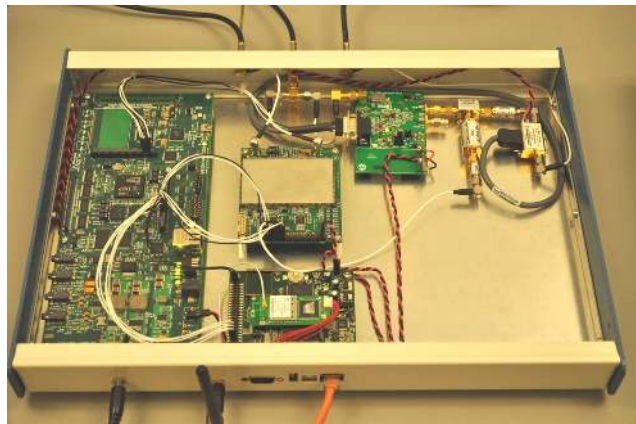
Fig. 3. Picture of the civil GPS spoofer used in the VSD evaluation experiments.
