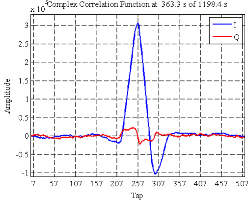
Fig. 6. Plot of the complex correlation function during a spoofing attack on a stationary receiver.
