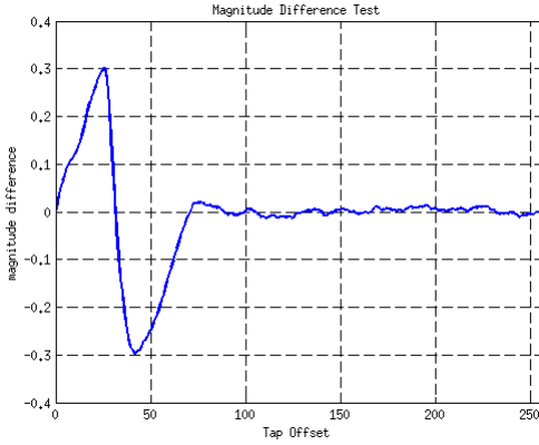
Fig. 8. Plot of MD_{\tau}(t) showing the effect of a spoofing attack on a stationary receiver.
