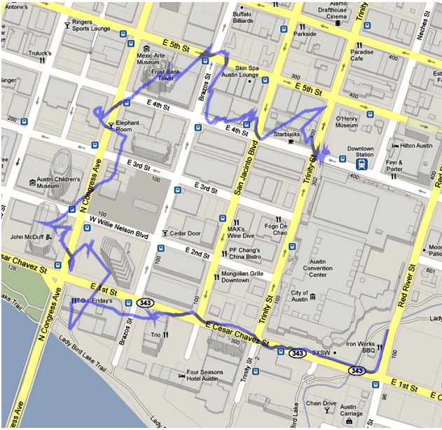
Fig. 5. Map showing a trace of the computed GPS navigation solution for a GPS receiver on a dynamic platform in a challenging dense-urban multipath environment.
