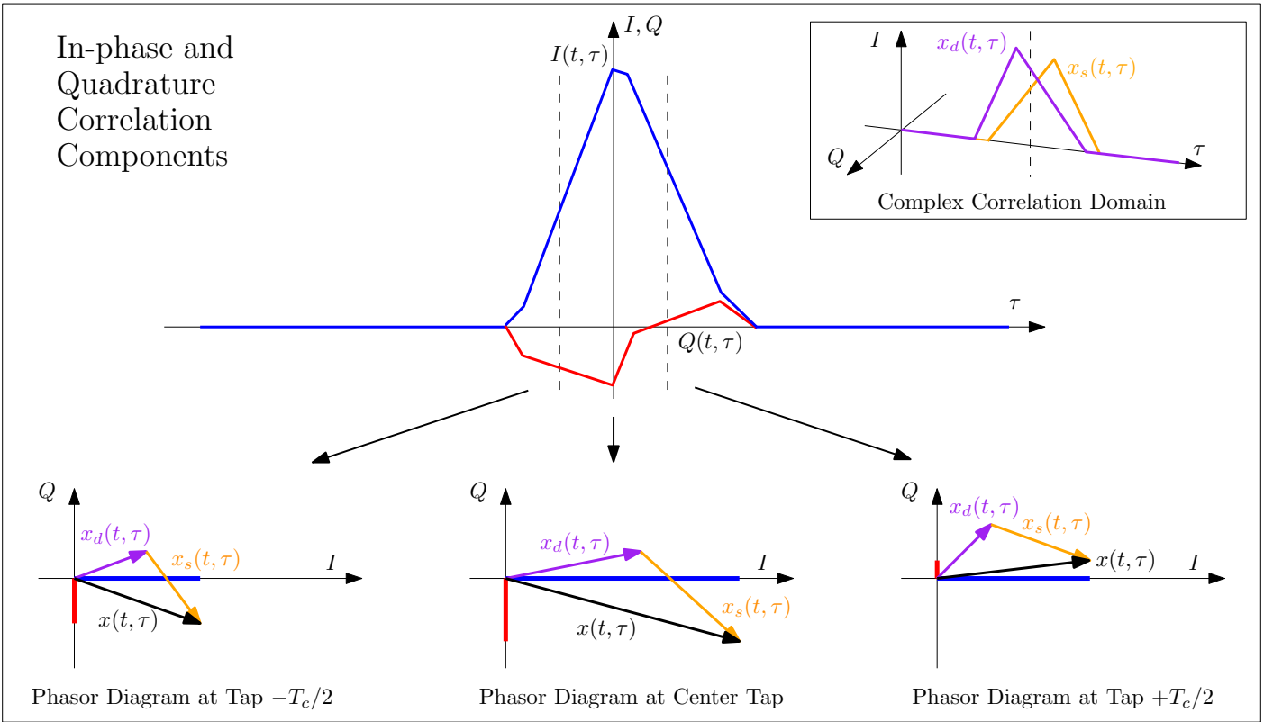
Fig. 2. Figure illustrating the distortions that can be present in the in-phase and quadrature components of x(t, \tau) during a spoofing attack.
