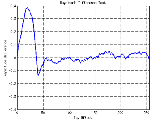
Fig. 9. Plot of MD_{\tau}(t) showing the effect of multipath on a receiver on a dynamic platform.
