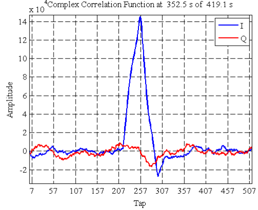
Fig. 7. Plot of the complex correlation function for a non-spoofed receiver on a dynamic platform.
