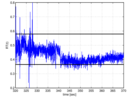
Fig. 15. Plot of RT_{\tau \approx 1/2\mu_s}(t) .
