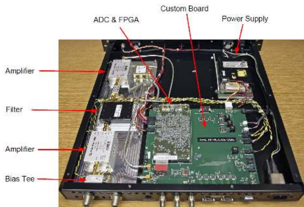
Fig. 4. Picture of the digitizing front-end receiver (figure adapted from Ref. [30] with permission).
