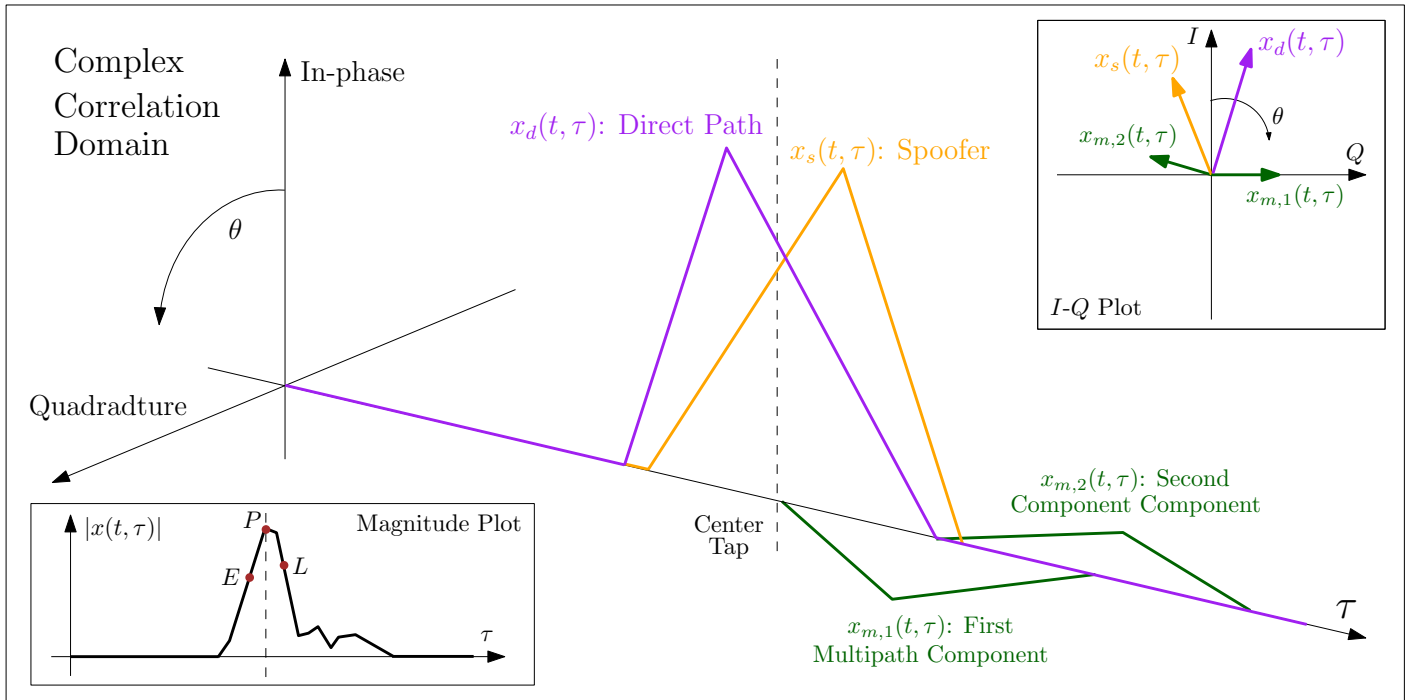
Fig. 1. Figure illustrating the complex correlation domain view of a spoofing attack and the corresponding I - Q and magnitude plots.
