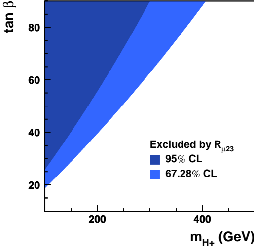
Fig. 11. Regions in the (m_{H^\pm}, \tan \beta) plane in two-Higgs-doublet models excluded by the present result for R_{\mu 23} .
