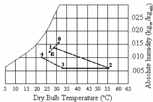
Figure 3. Psychrometric processes.
