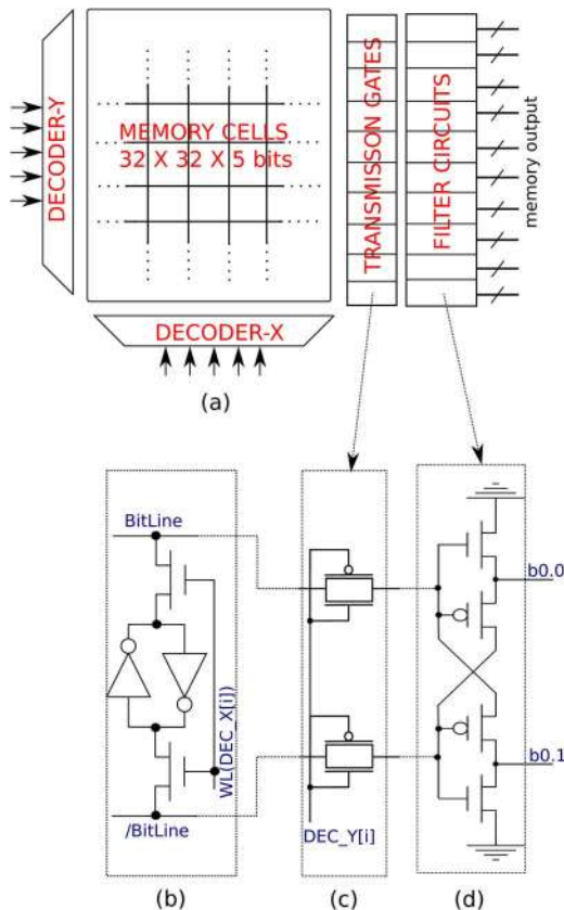
Fig. 3. (a) Memory architecture. (b) A six-transistor standard memory cell. (c) Transmission gate. (d) Memory output filter circuit to produce dual-rail data representation.
