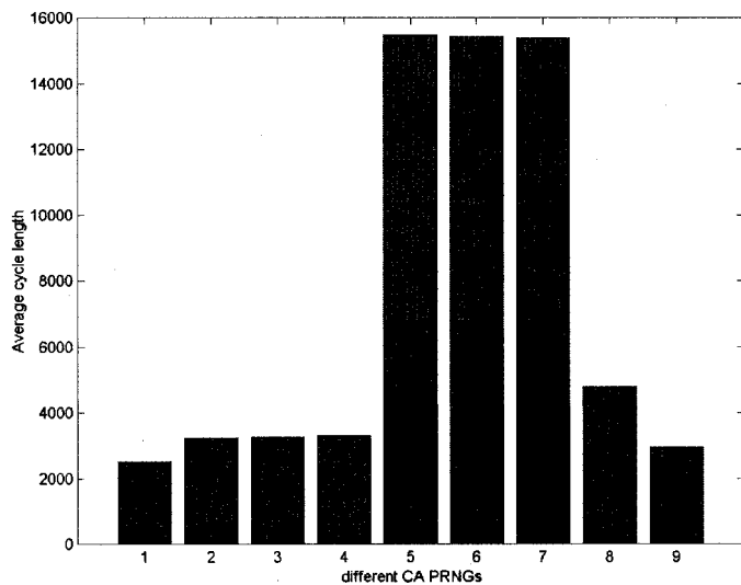
Fig. 12. Average cycle lengths of CA PRNGs. Note: All the tested 1-D CA PRNGs have 16 cells. 1: PCA90-150 PRNG. 2-4: evolved CCA0 PRNGs. 5-7: evolved CCA2 PRNGs. 8: 2-D 4 x 4 CA PRNG. 9: 2-bit PCA90-105 PRNG. Results are based on 20 initial seeds.
