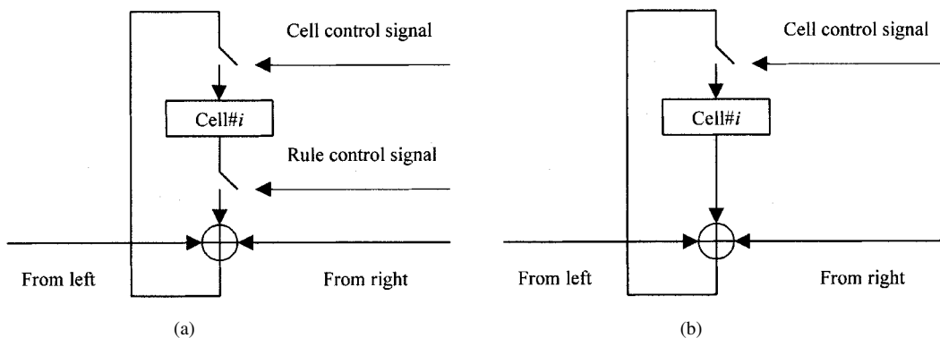
Fig. 2. Controllable cell structure. (a) Programmable controllable cell. (b) Non-programmable controllable cell.
