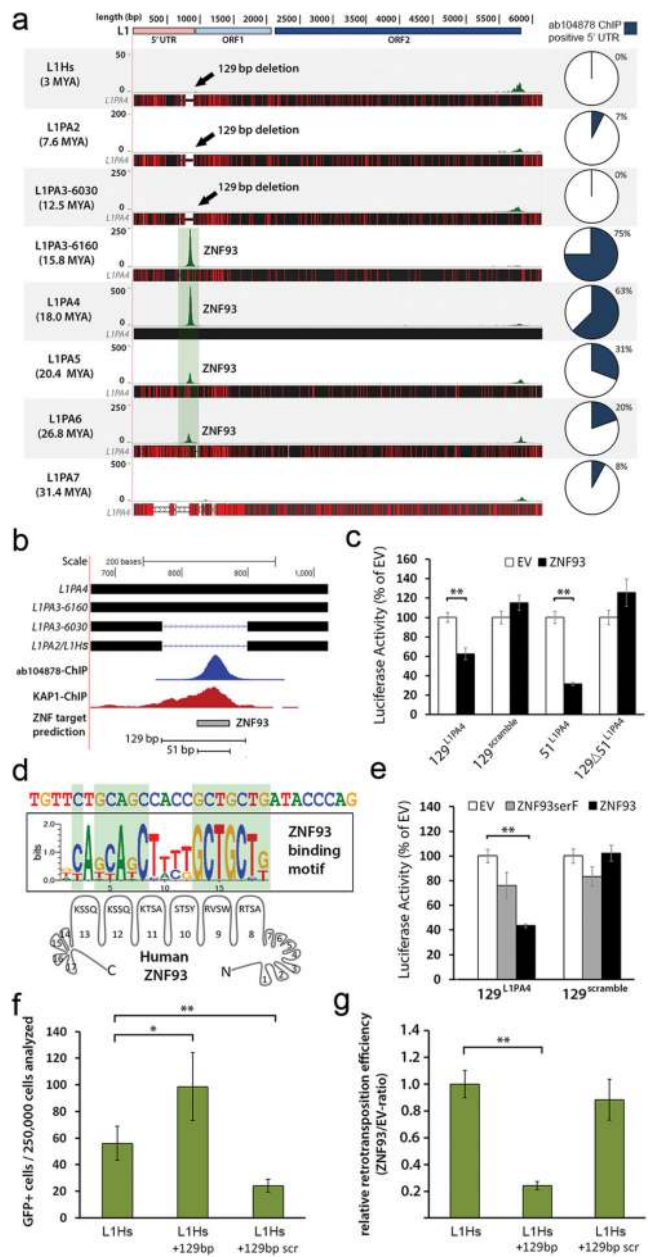
Figure 3. LIPA elements are repressed by primate-specific ZNF93
