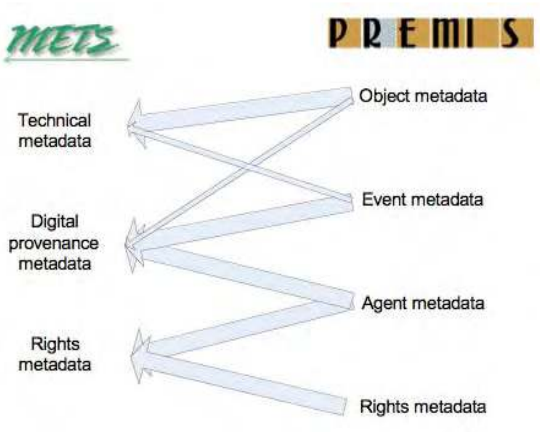
Figure 23. Mapping PREMIS entities to METS metadata sections (Guenther, 2008).
