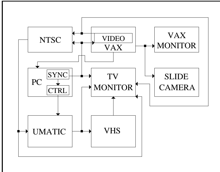
Figure 9: Schematic of the Graphics Equipment
