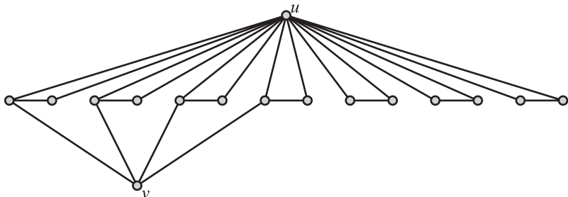
Figure 1: Induced subgraph of G .
