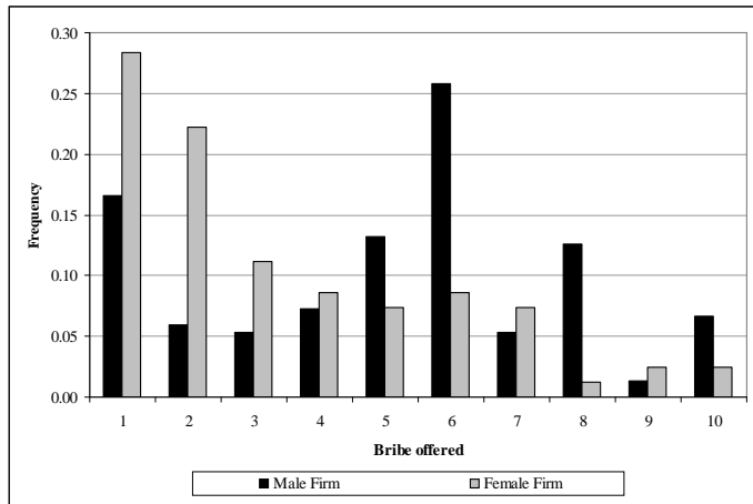
Figure 2: Histogram of bribes offered
