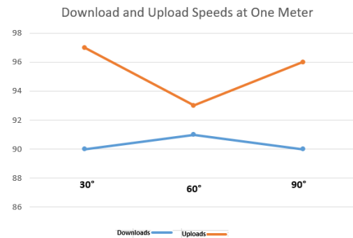
Fig. 14: Download and Upload speed at One Meter via Local FTP Server.
