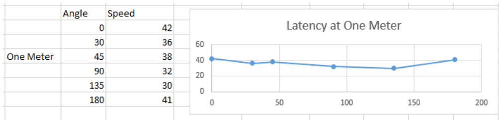
Fig. 10: Latency Speeds at One Meter (Source: Researcher Lab Results)
