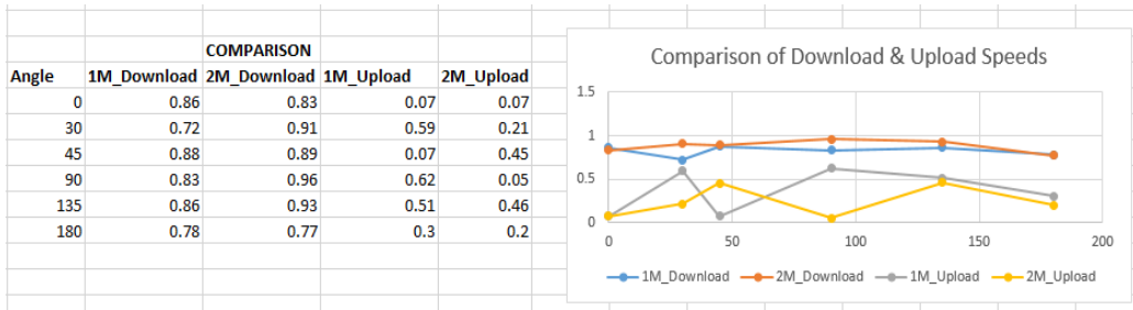
Fig. 13: Upload and Download Speeds Comparison at Respective Angles, One & Two Meters (Source: Researcher Lab Results).
