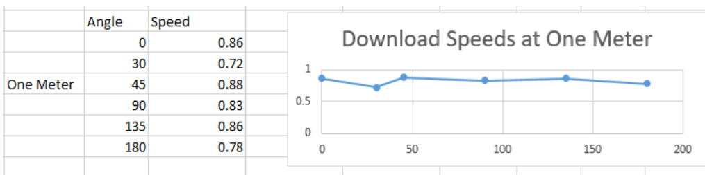
Fig. 6: Download Speeds at One Meter (Source: Researcher Lab Results).
