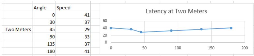
Fig. 11: Latency Speeds at Two Meters (Source: Researcher Lab Results).
