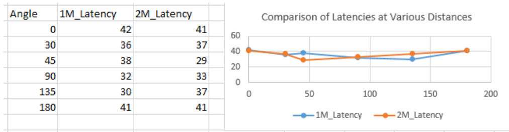
Fig. 12: Latency Speeds Comparison at Respective Angles, One & Two Meters (Source: Researcher Lab Results).
