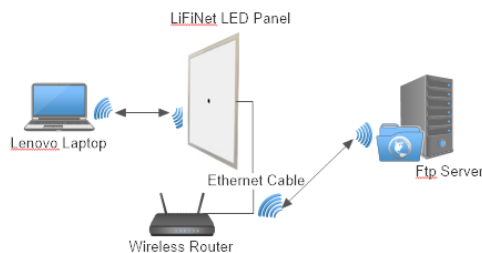
Fig. 3: Schematic LiFi testbed architecture without the internet (Source: authors own visualization).
