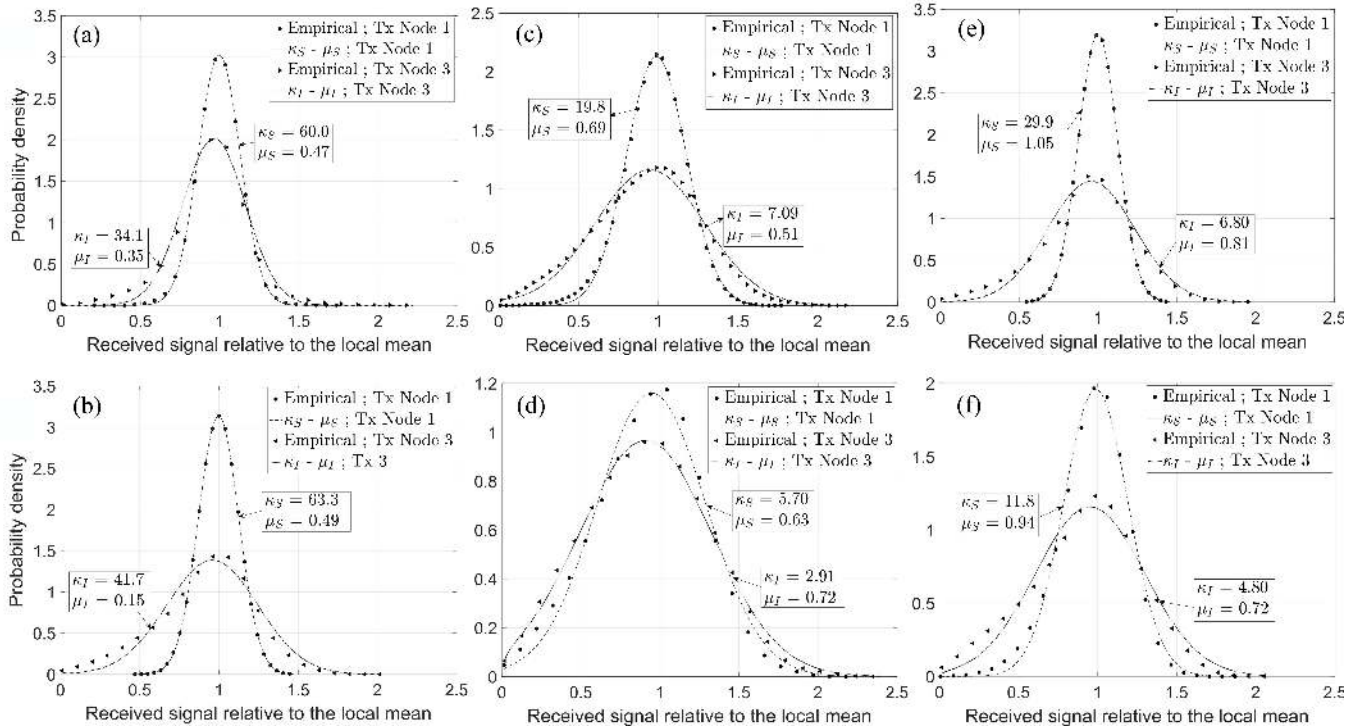
Fig. 4. Empirical envelope pdf of the SoI and interfering links for (a) anechoic chamber scenario 1, (b) anechoic chamber scenario 2, (c) reverberation chamber scenario 1, (d) reverberation chamber scenario 2, (e) laboratory environment scenario 1, and (f) laboratory environment scenario 2 compared to the \kappa - \mu pdf.
