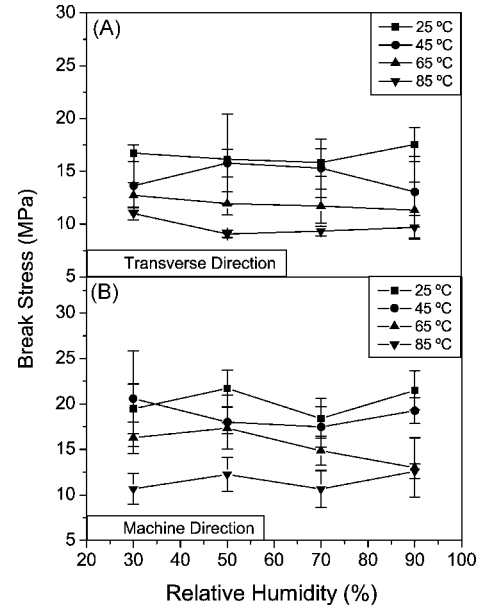
Fig. 10. Break stress as a function of humidity at various temperatures: (A) transverse direction and (B) machine direction.
