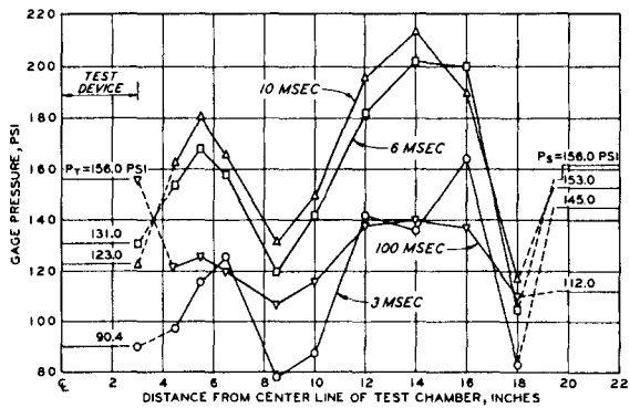
b. VARIATION OF SOIL STRESS WITH TIME AT THE 35-INCH LEVEL
