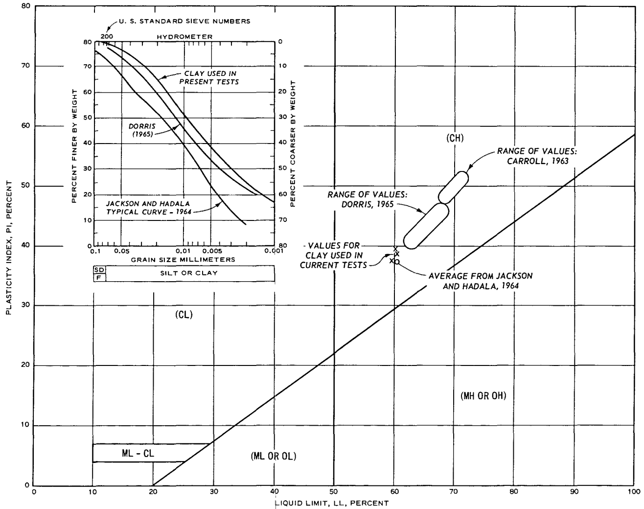
Fig. A-1. Gradation curve and Atterberg limits for buckshot clay
