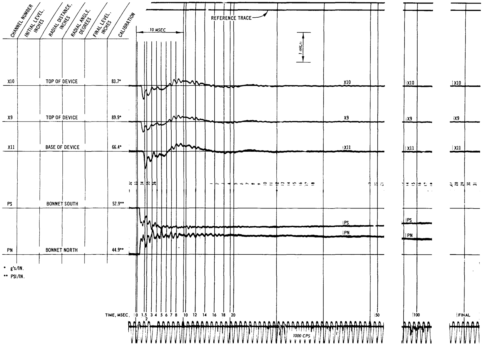
Fig. C-57. Test 24, acceleration and pressure record
