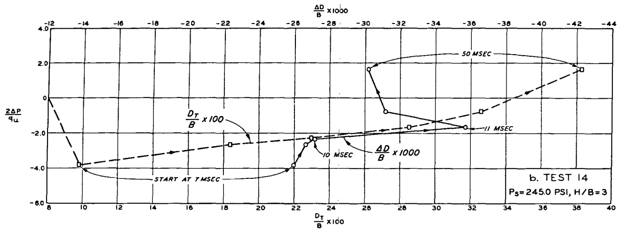
Fig. 52. Dimensionless plot of pressure versus deflection for dynamic Tests 13 and 14
