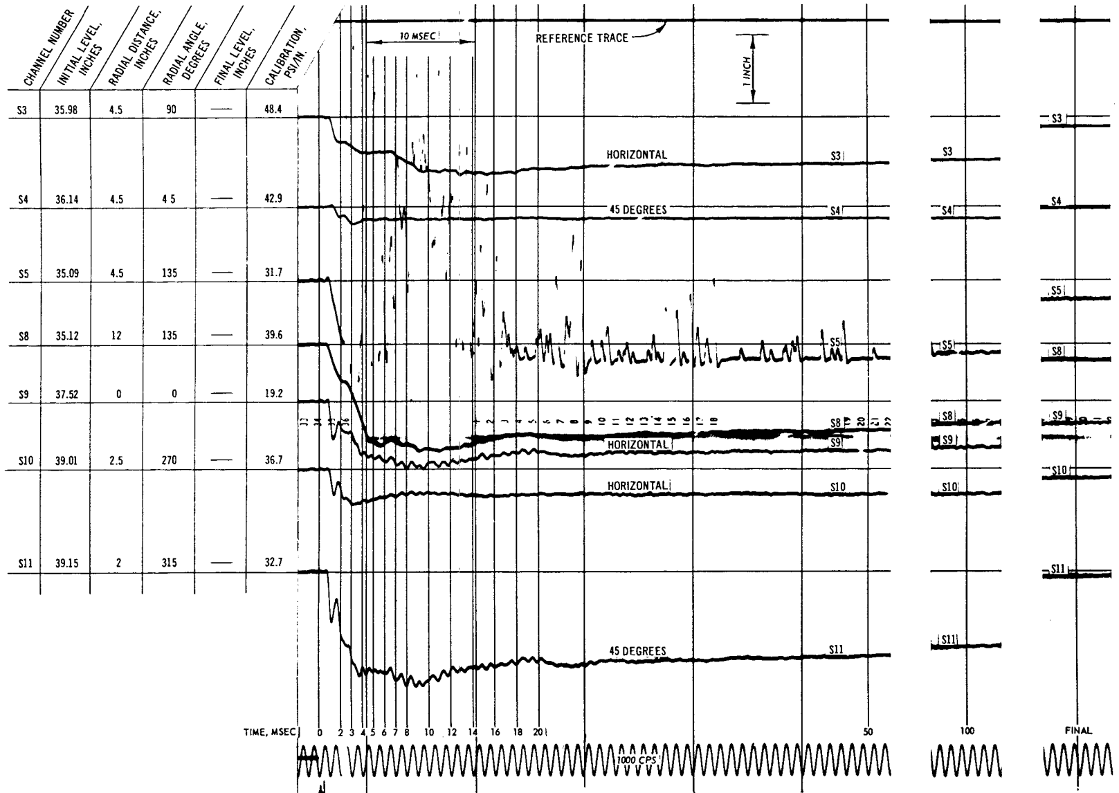
Fig. C-54. Test 24, pressure record
