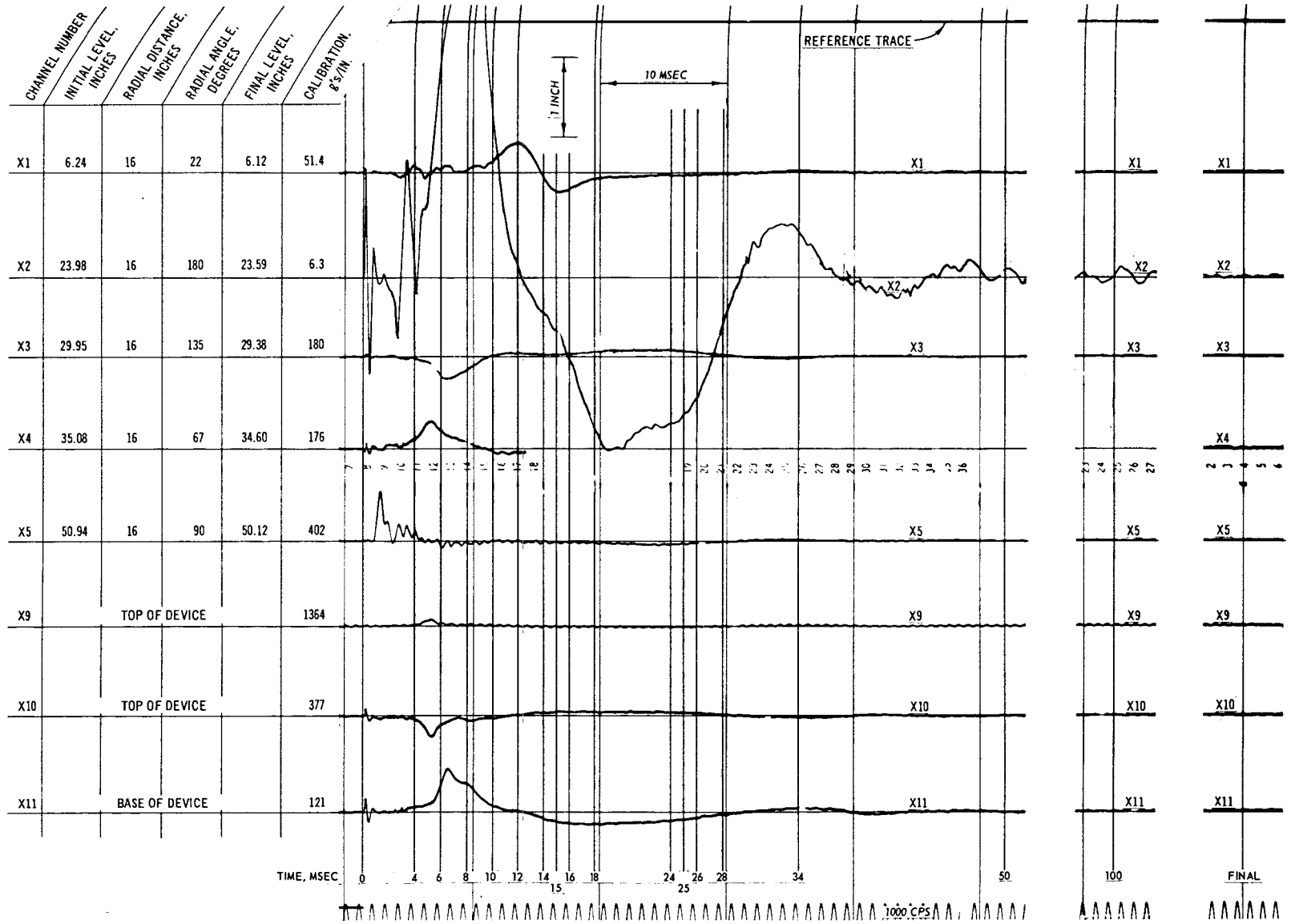
Fig. C-9. Test 12, acceleration record
