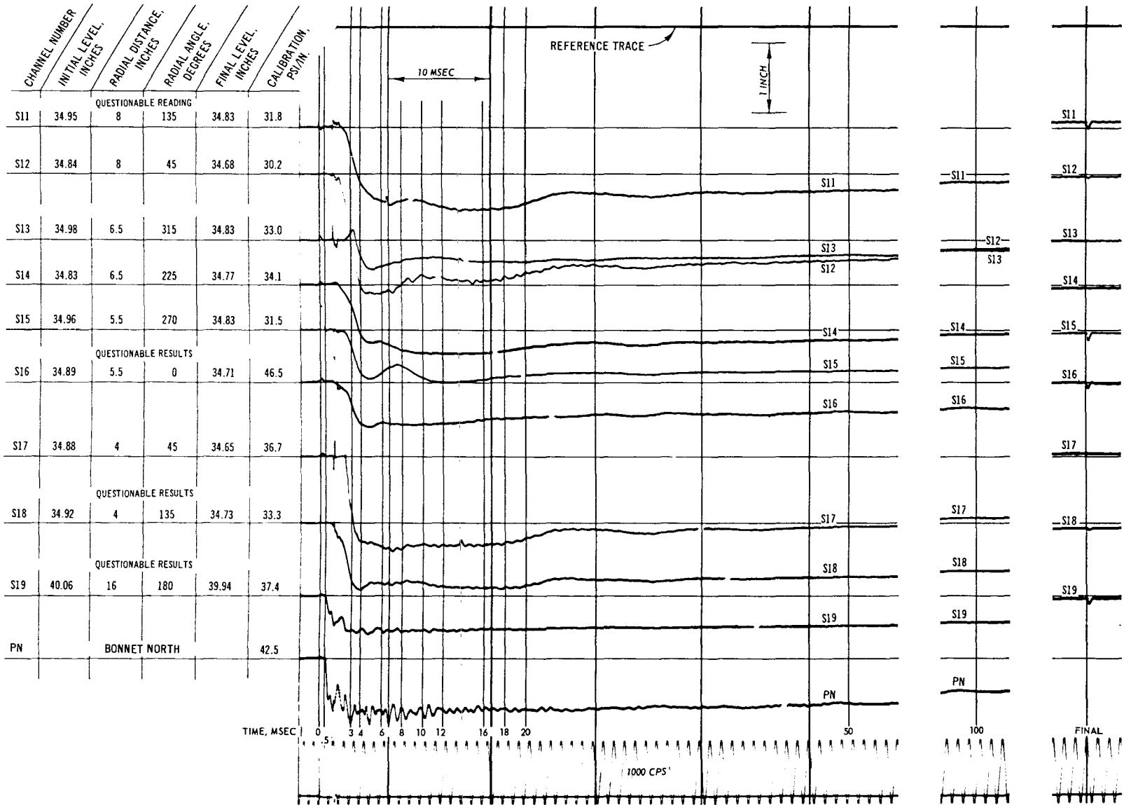
Fig. C-63. Test 26, pressure record (S11-S19)
