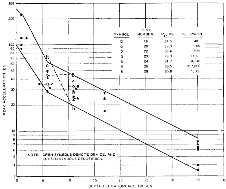
b. Variation with change in structure stiffness; H/B = 1 , P_s \approx 32 to 38 psi
