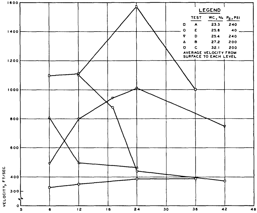
a. PROPAGATION OF INITIAL DISTURBANCE
