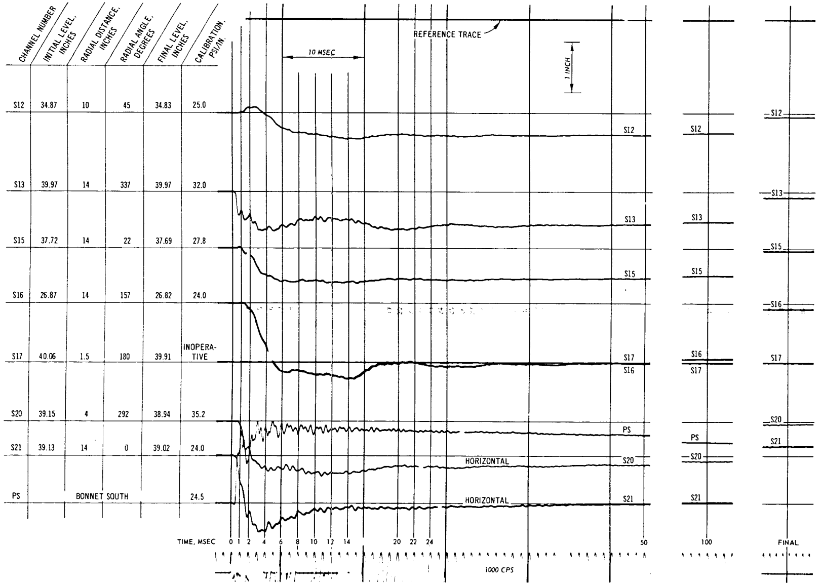
Fig. C-73. Test 28, pressure record (S12-S21)
