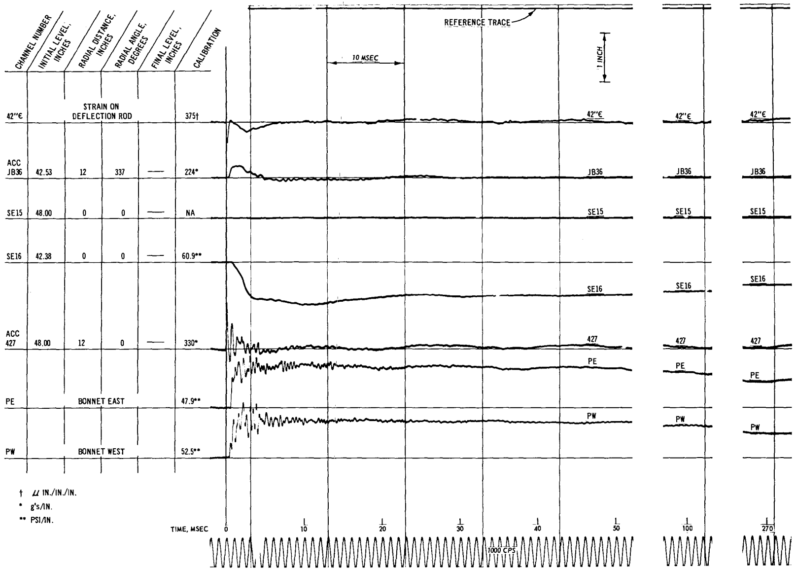
Fig. C-86. Test E, pressure, acceleration, and strain record
