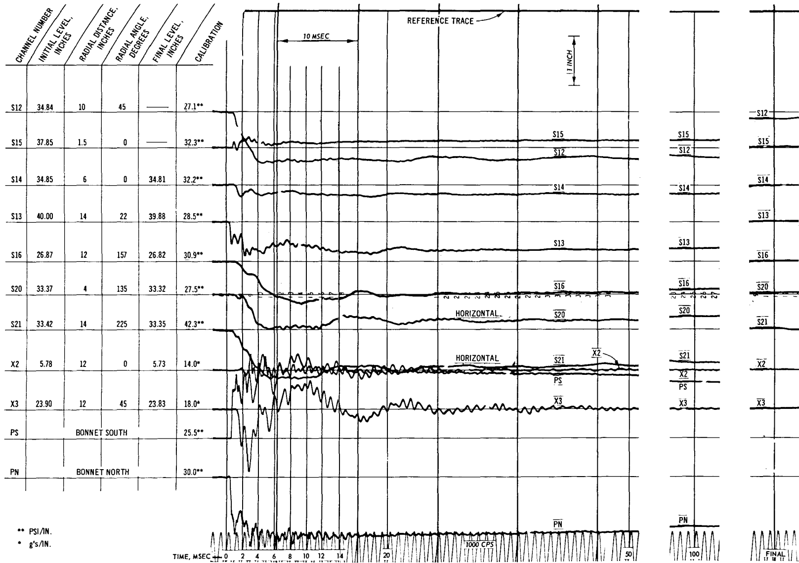
Fig. C-43. Test 21, pressure and acceleration record
