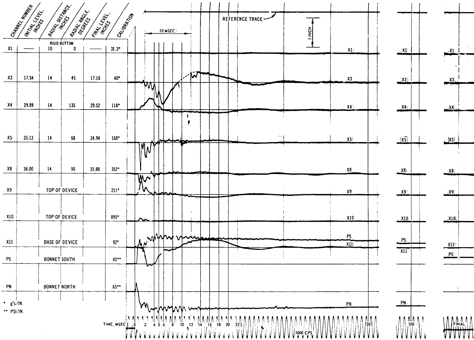
Fig. C-21. Test 15, acceleration and pressure record
