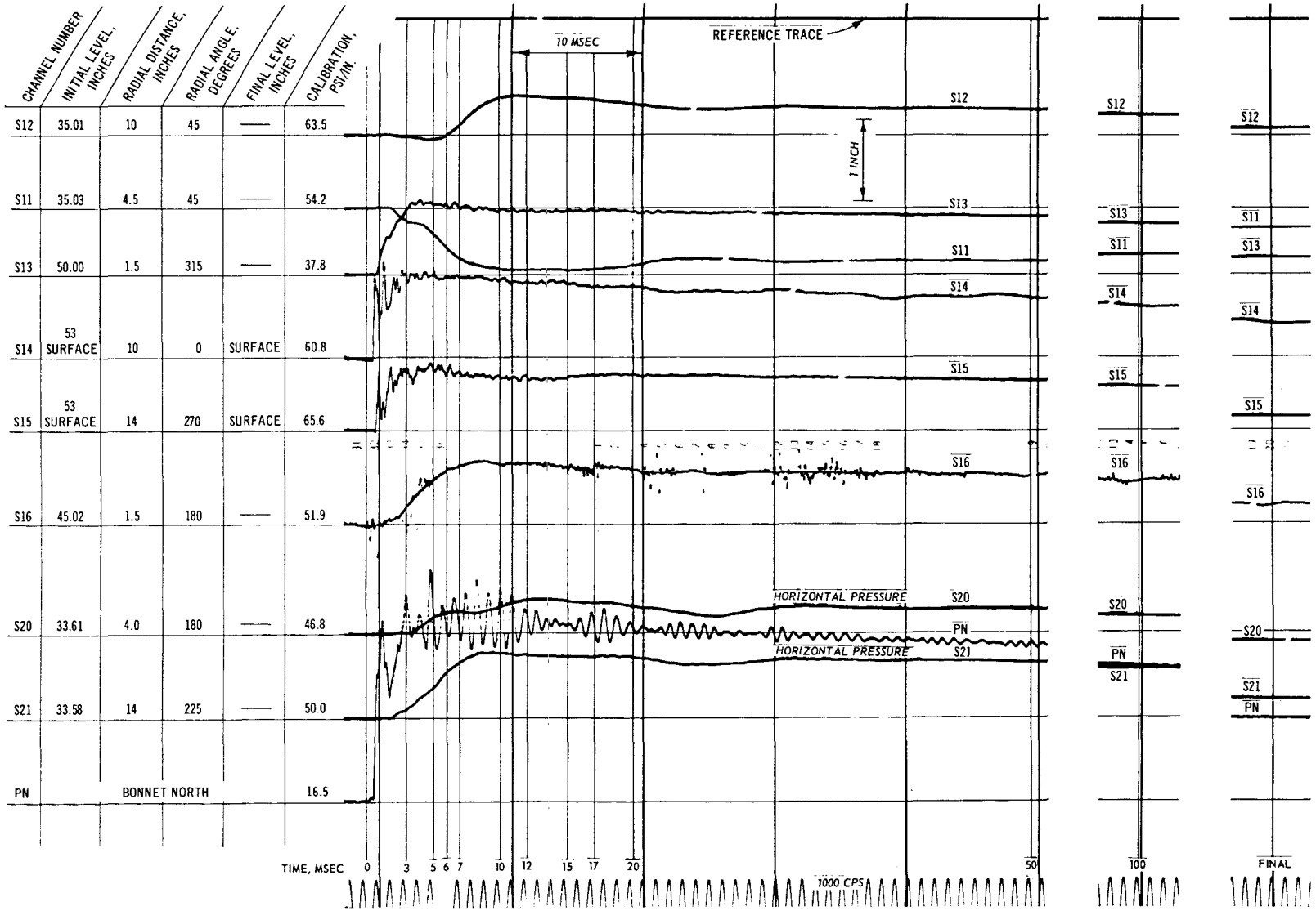
Fig. C-3. Test 11, pressure record (channels S11-S21)
