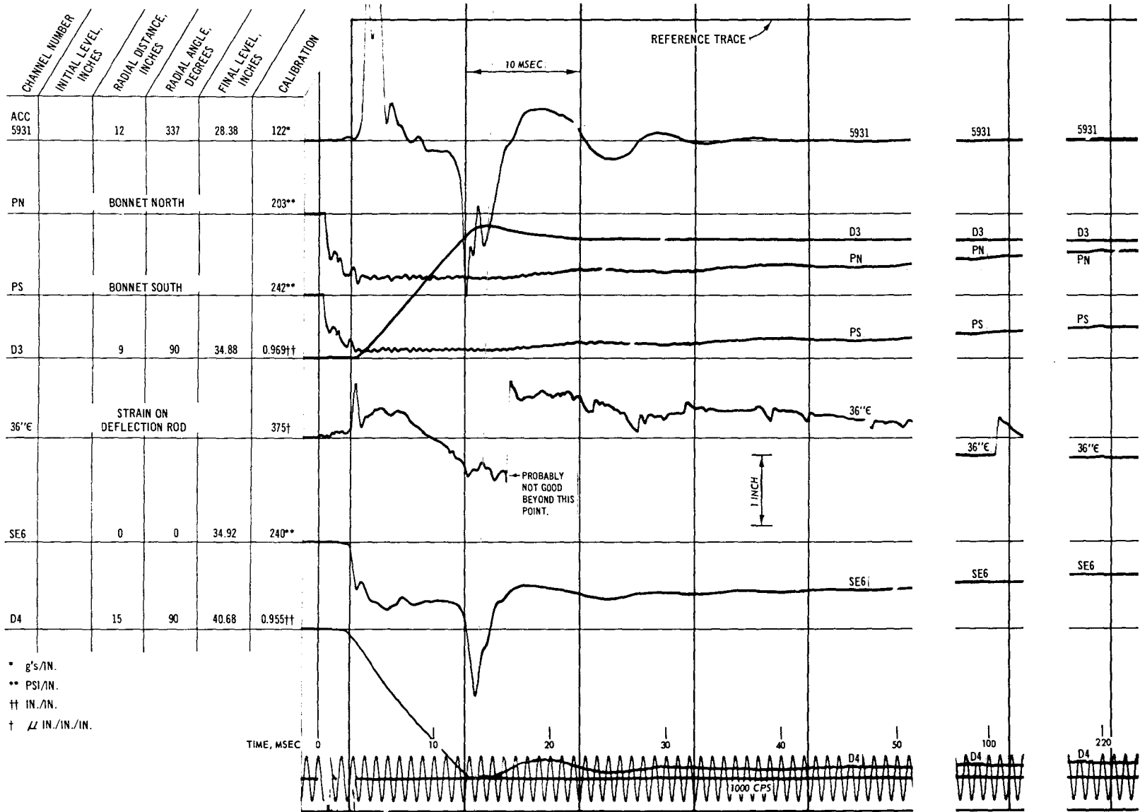
Fig. C-82. Test D, pressure, acceleration, deflection, and strain record
