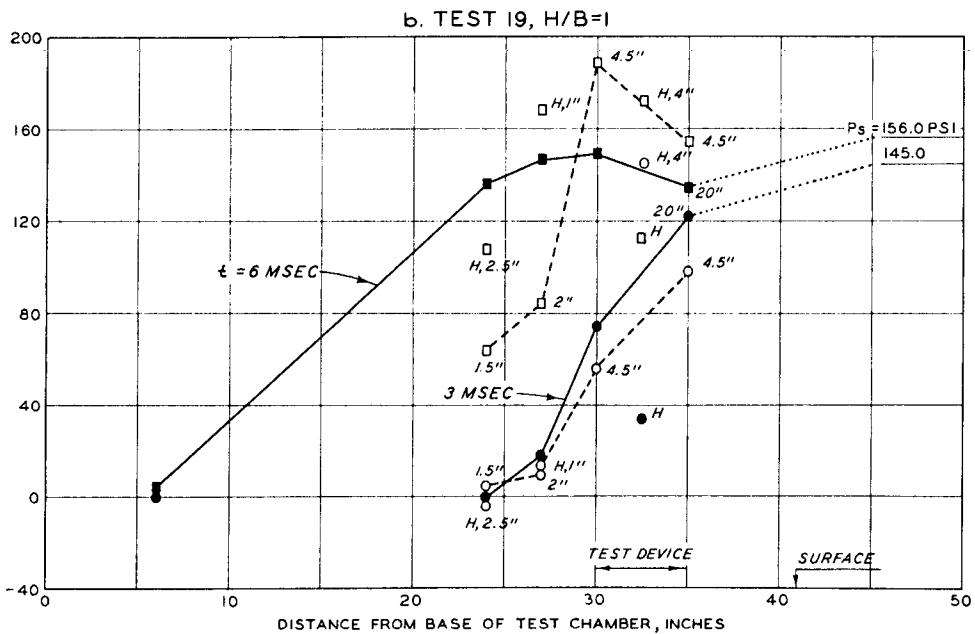
Fig. 65. Variation of soil stress with depth and time, Tests 18 and 19
