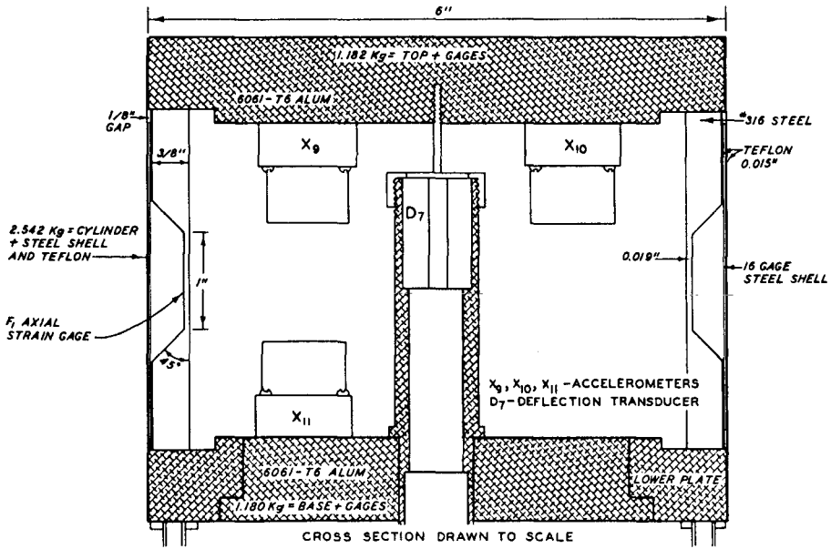
Fig. 14. "Rigid" test device
