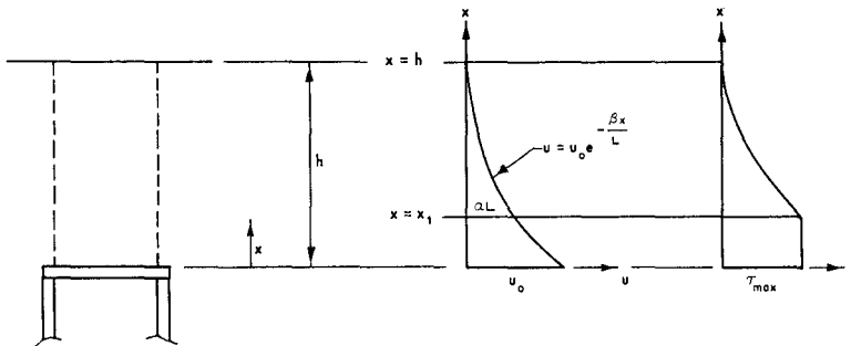
c. VARIATION OF DISPLACEMENT AND SHEARING STRESS WITH DEPTH
