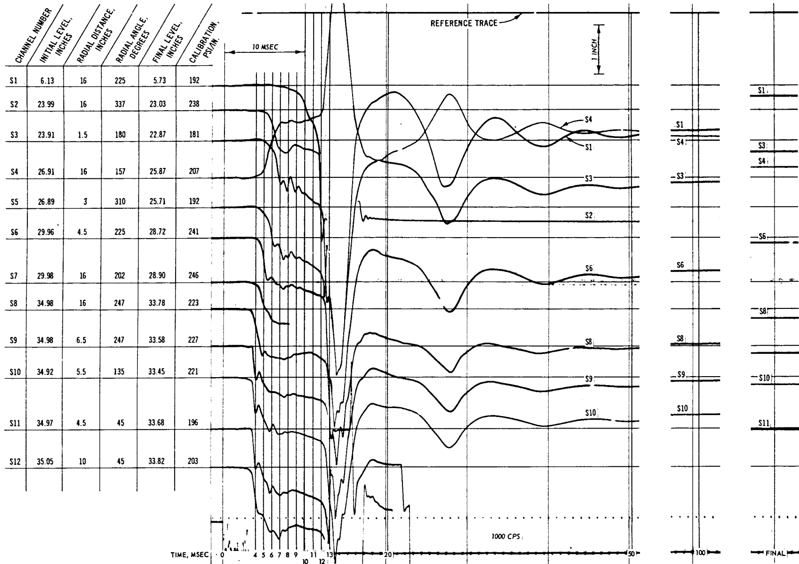
Fig. C-14. Test 14, pressure record (S1-S12)
