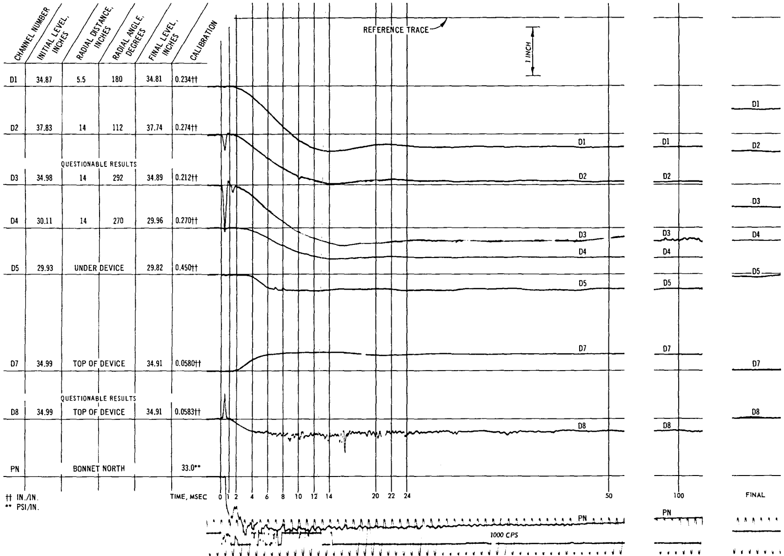
Fig. C-74. Test 28, deflection and pressure record
