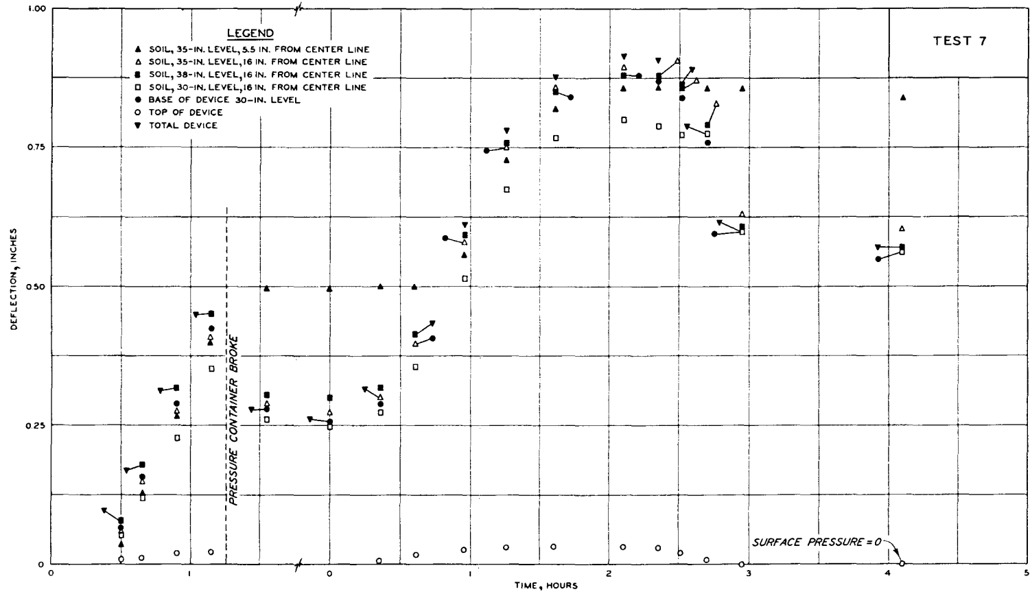
Fig. 39. Soil and structure deflections versus time; Test 7, H/B = 1 , P_S = 37.5 psi
