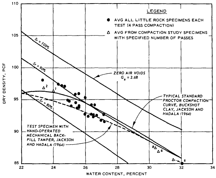
Fig. A-2. Water content-density relations for buckshot clay
