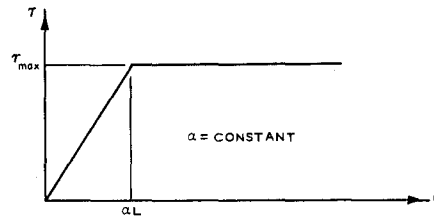
b. ASSUMED VARIATION OF SHEARING STRESS VERSUS DISPLACEMENT
