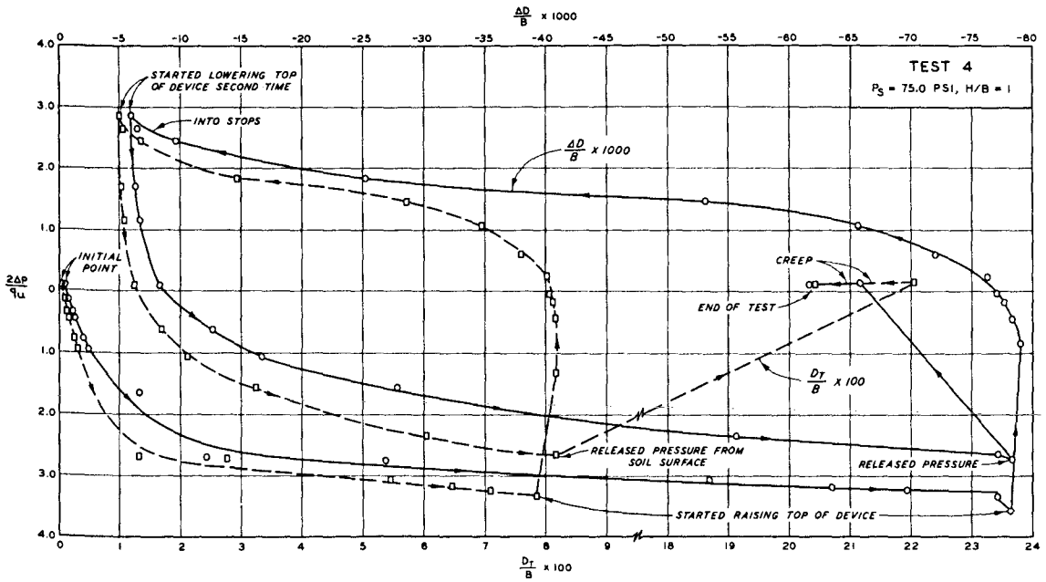
Fig. 23. Dimensionless plot of pressure versus deflection for static Test 4
