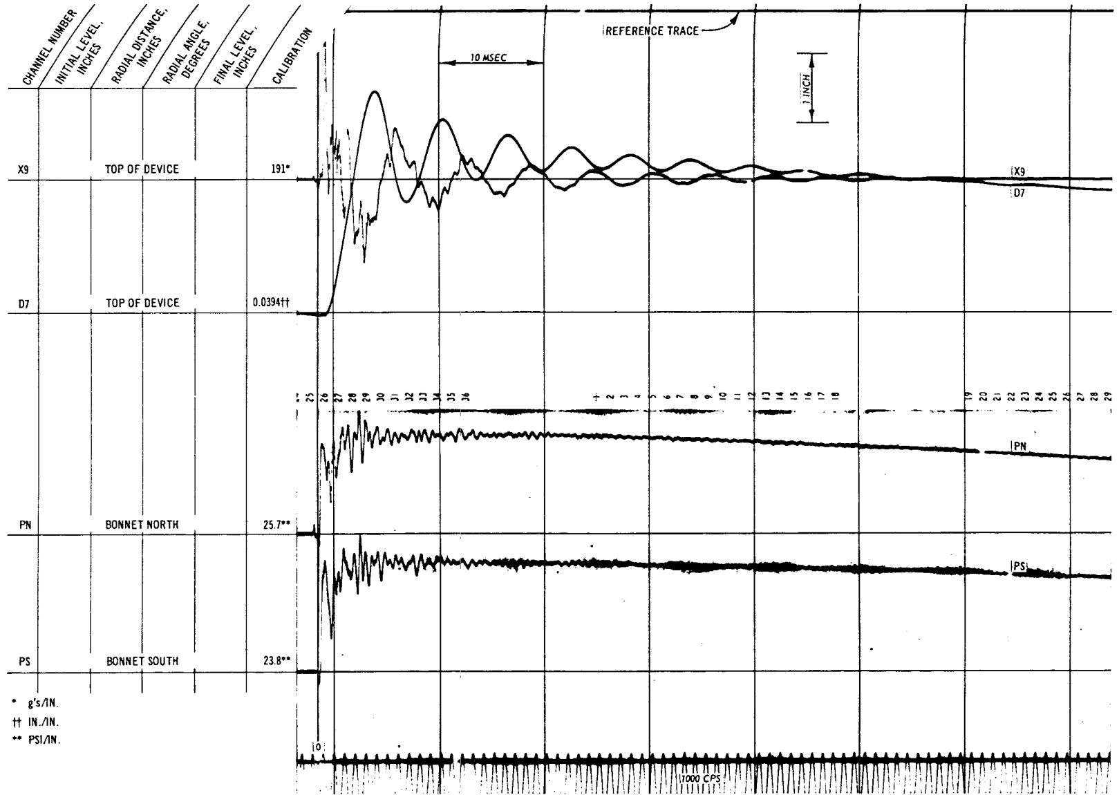
Fig. C-1. Typical dynamic airblast test record for spring-ring test device
