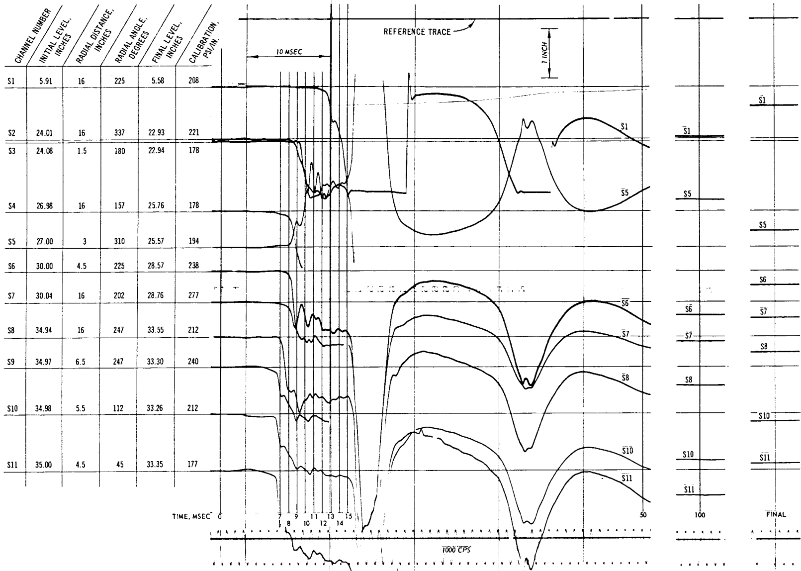
Fig. C-30. Test 18, pressure record (S1-S11)
