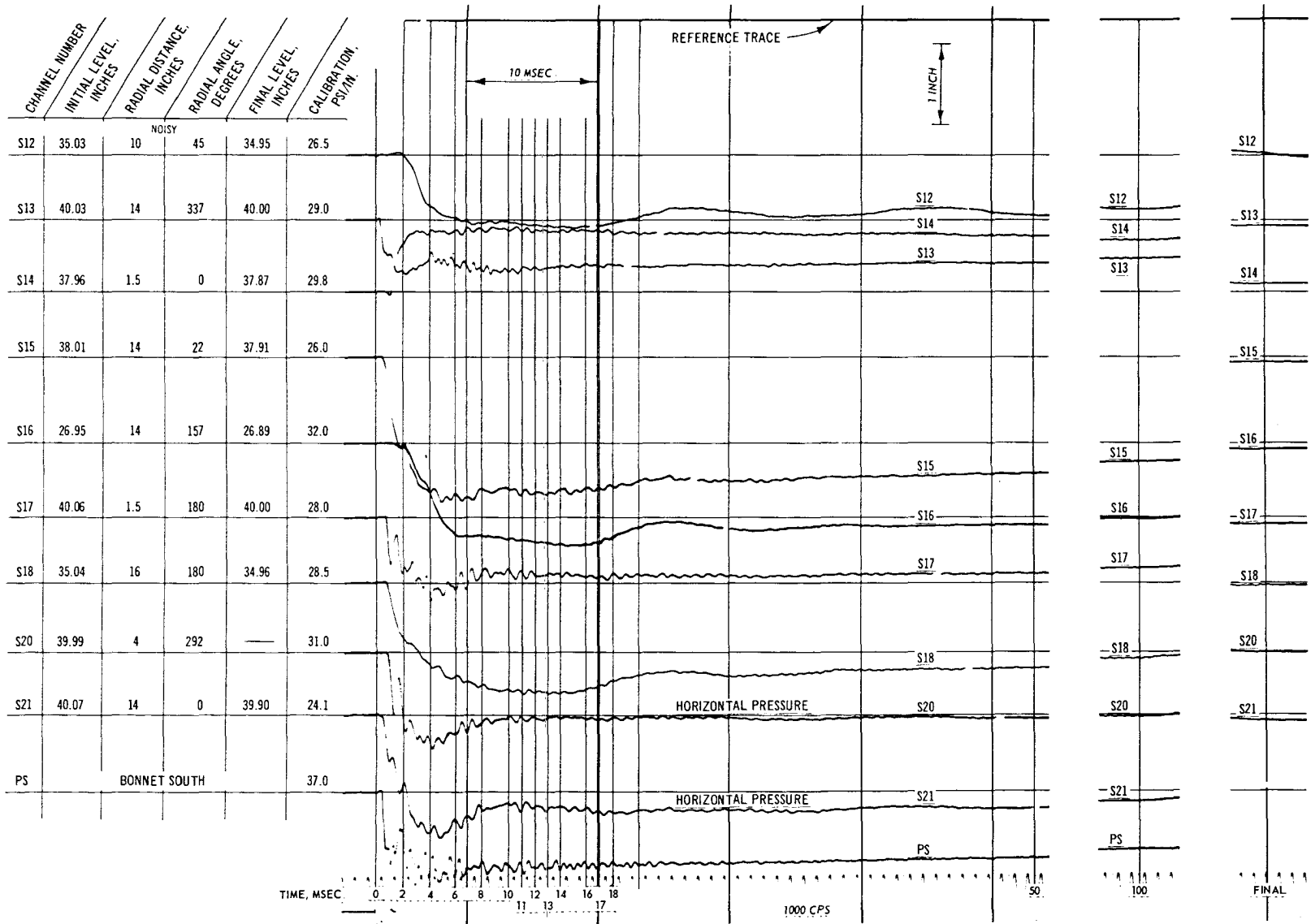
Fig. C-39. Test 20, pressure record (S12-S21)
