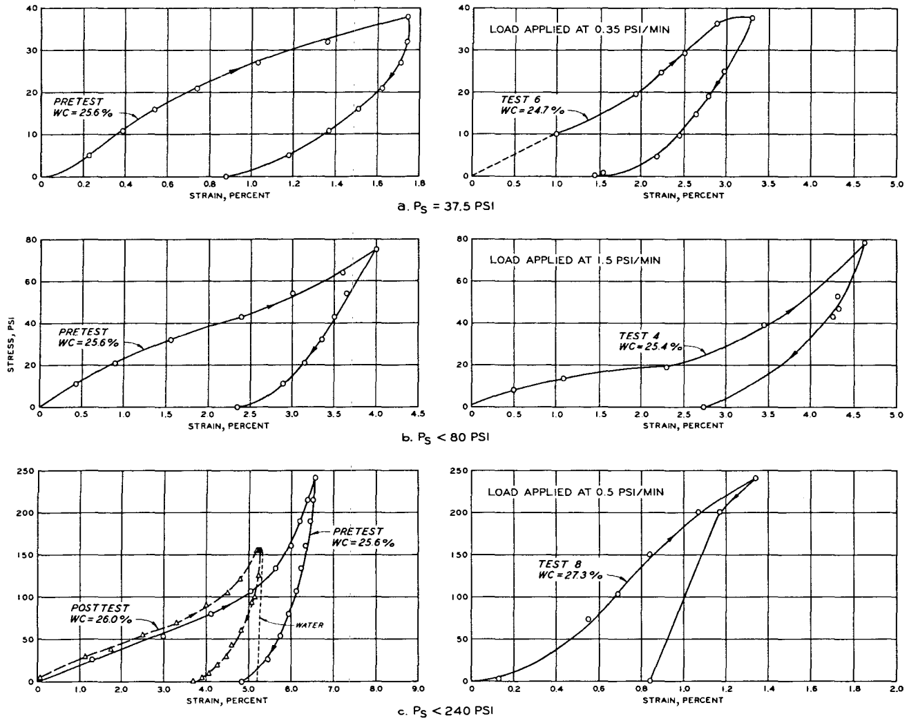
Fig. A-16. Stress-strain curves determined by static one-dimensional tests
