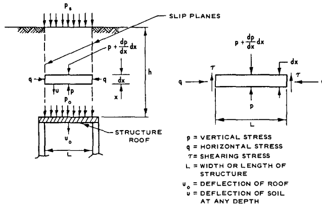
a. ASSUMED FORCE FIELD
