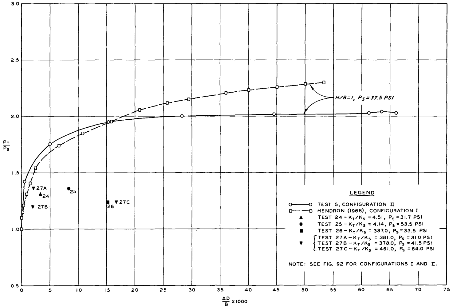
Fig. 93. Passive arching curves, static surface pressure
