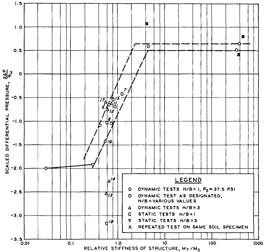
b. RELATION BETWEEN DIFFERENTIAL PRESSURE AND RELATIVE STIFFNESS
