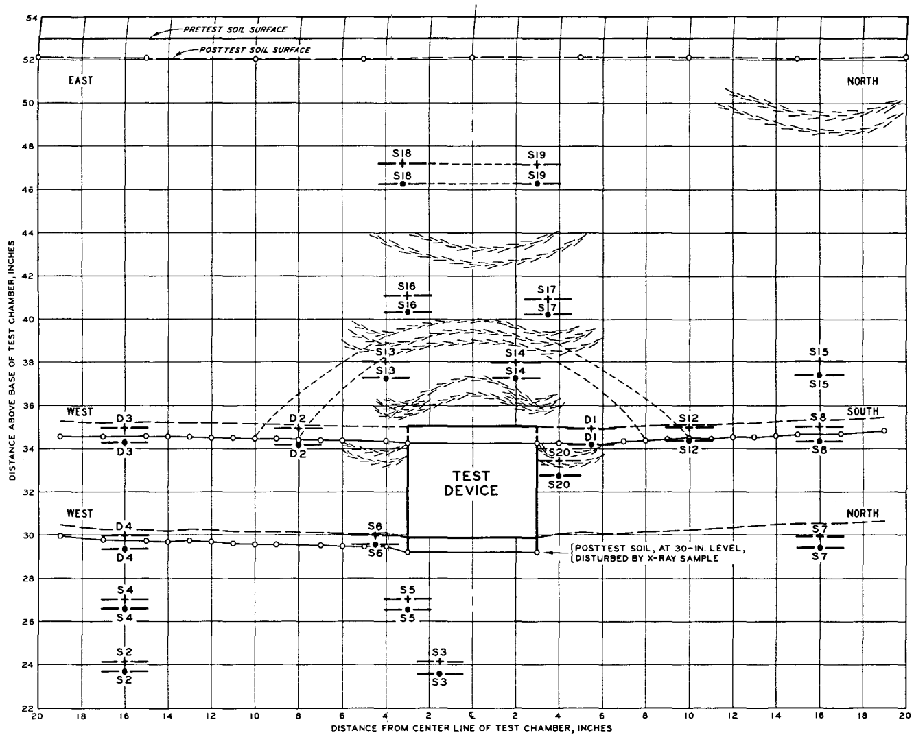
Fig. 45. Sketch of soil deformation patterns found in radiograph and visual inspection, Test 3; H/B = 3 , P_s = 37.5 psi
