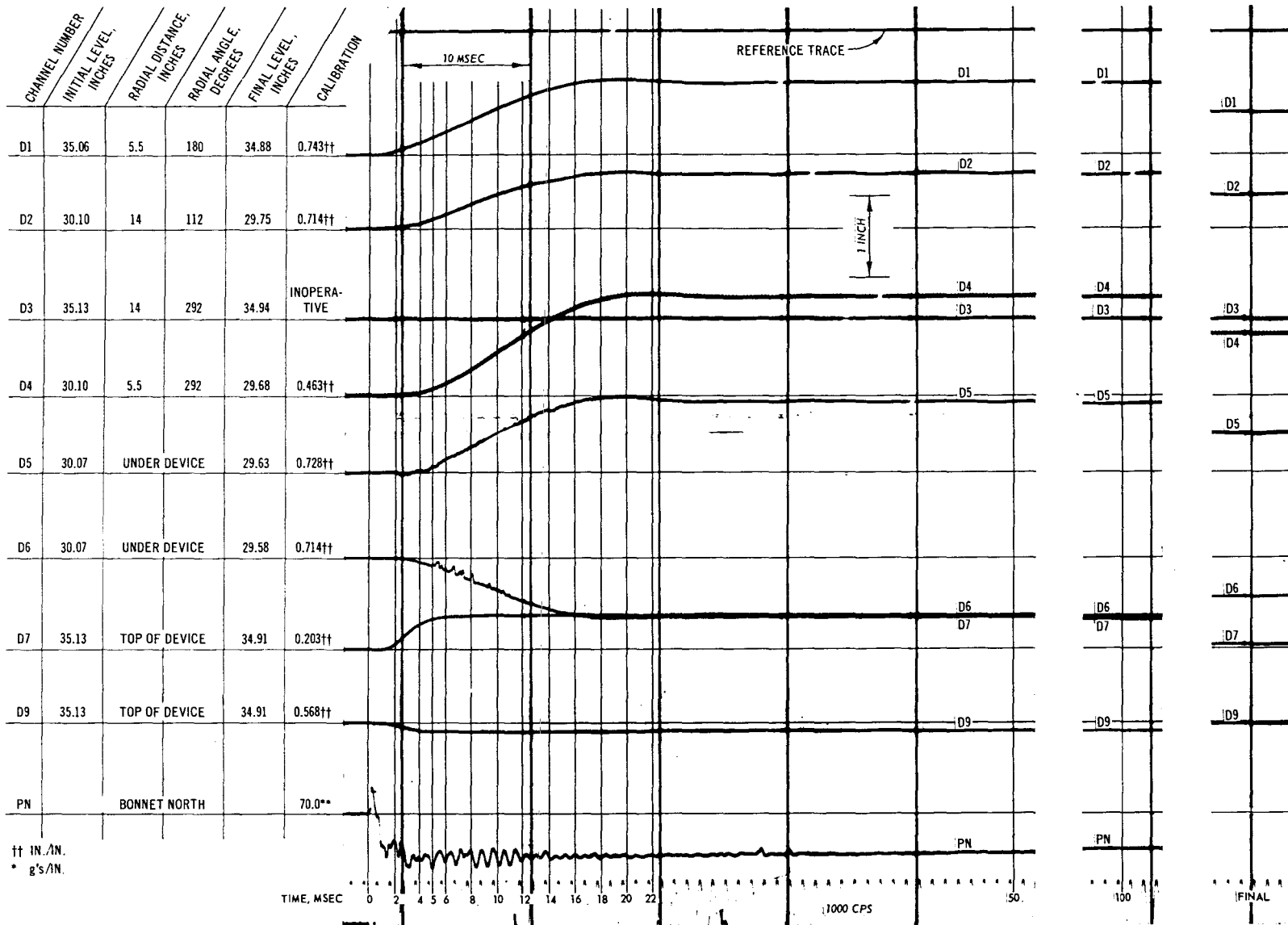
Fig. C-20. Test 15, deflection and pressure record
