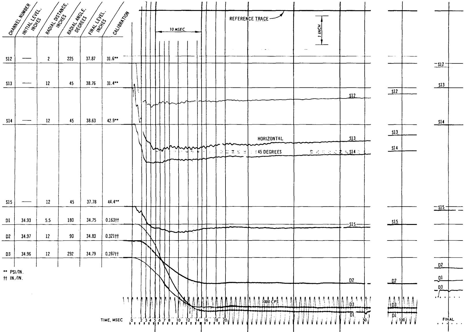
Fig. C-59. Test 25, pressure and deflection record
