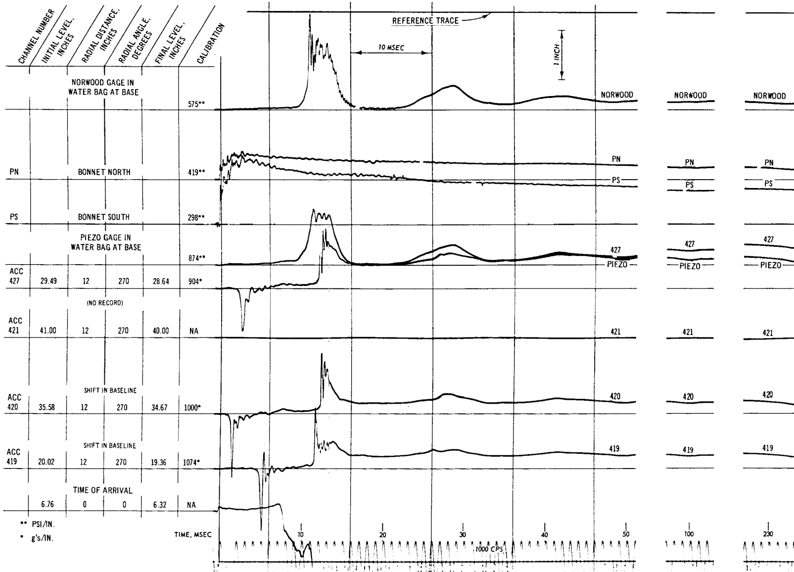
Fig. C-79. Test B, pressure and acceleration record
