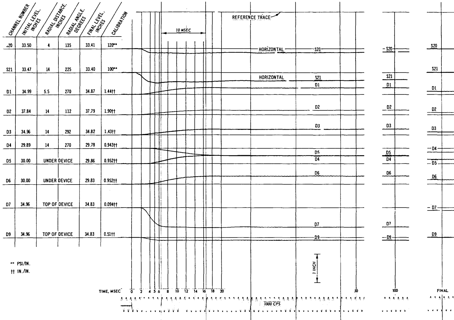
Fig. C-24. Test 16, pressure and deflection record
