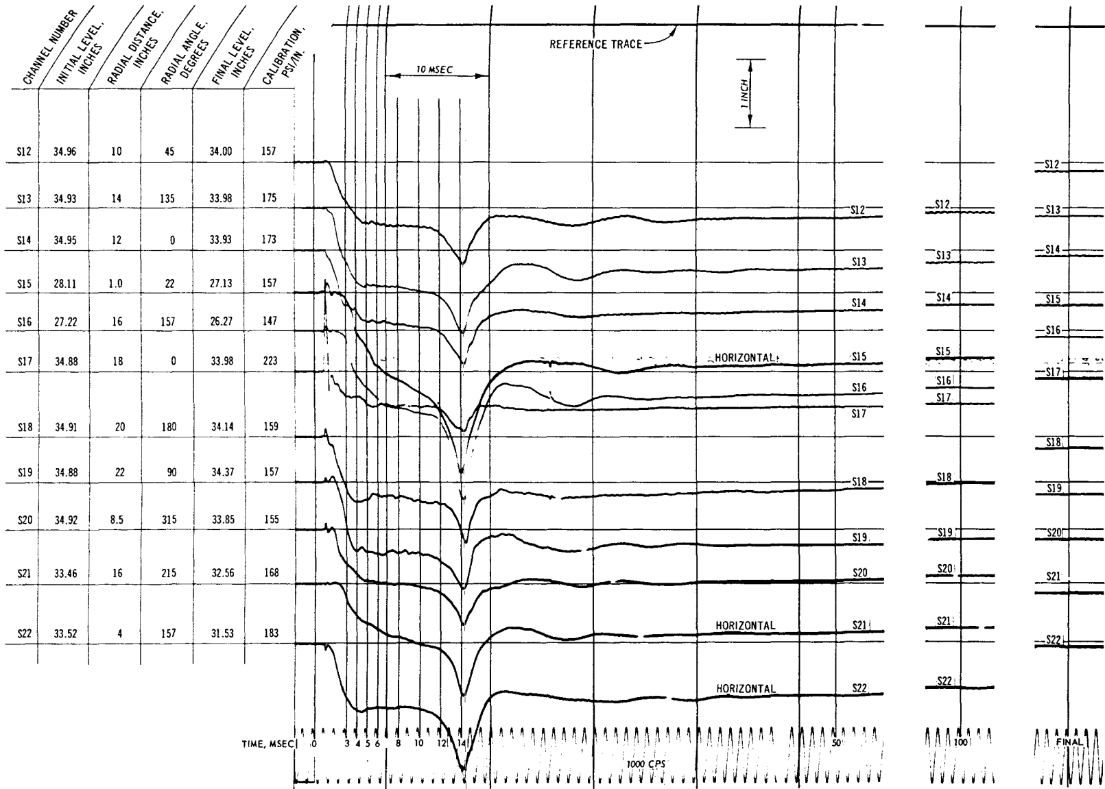
Fig. C-35. Test 19, pressure record (S12-S22)
