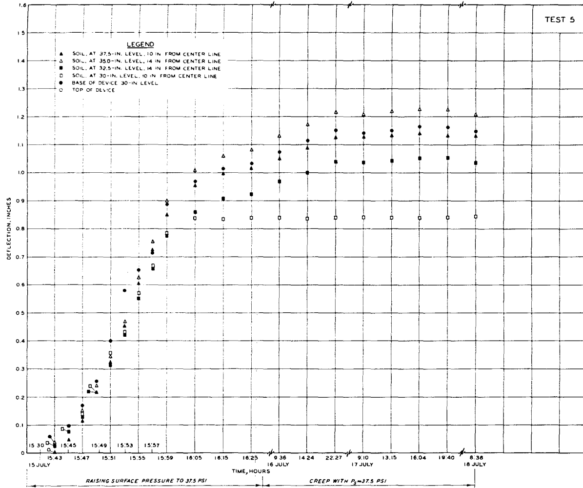
Fig. 37. Soil and structure deflections versus time; Test 5, H/B = 1 , P_s = 37.5 psi
