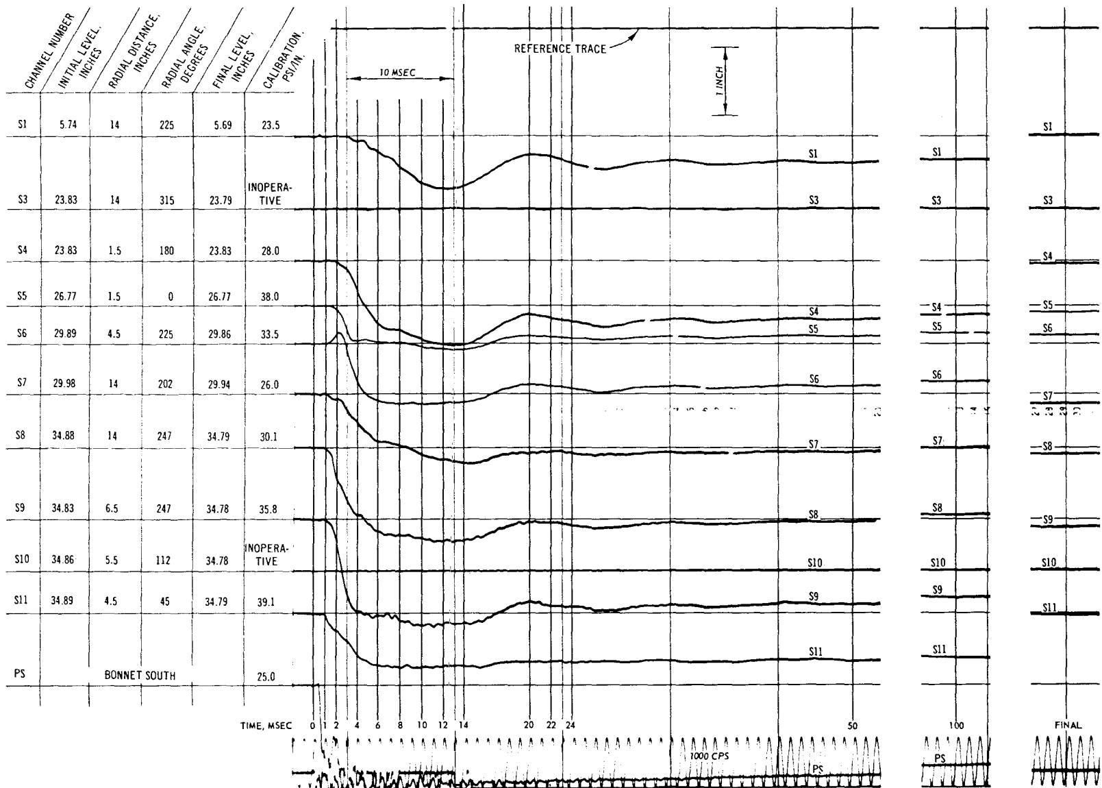
Fig. C-72. Test 28, pressure record (S1-S11)
