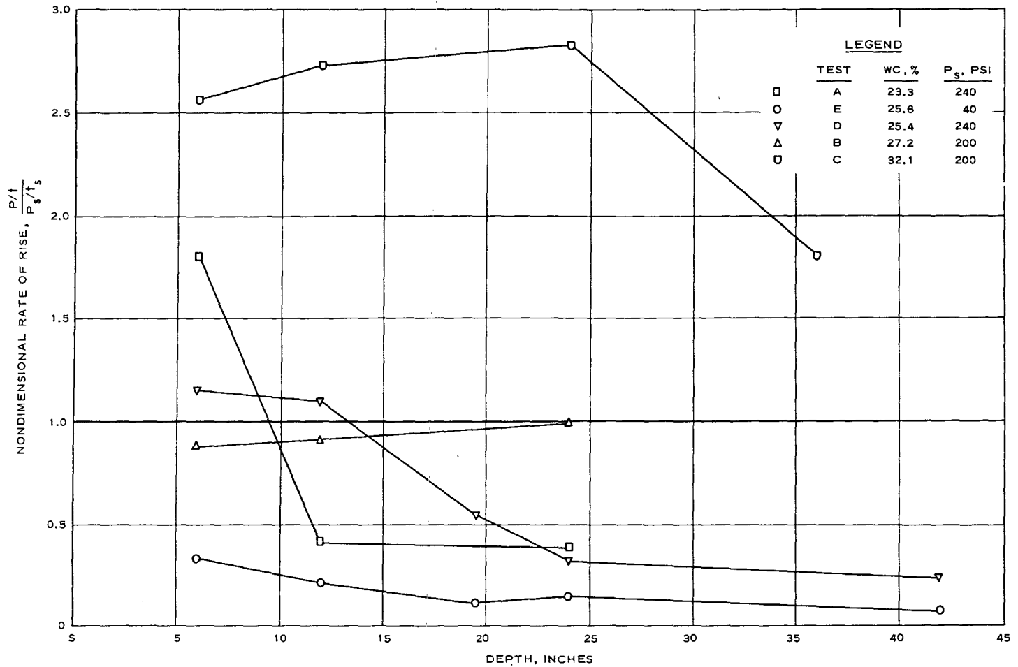
Fig. A-20. Nondimensional rate of rise variation with depth (average of north and south Norwood rates of rise set equal to 1.00)
