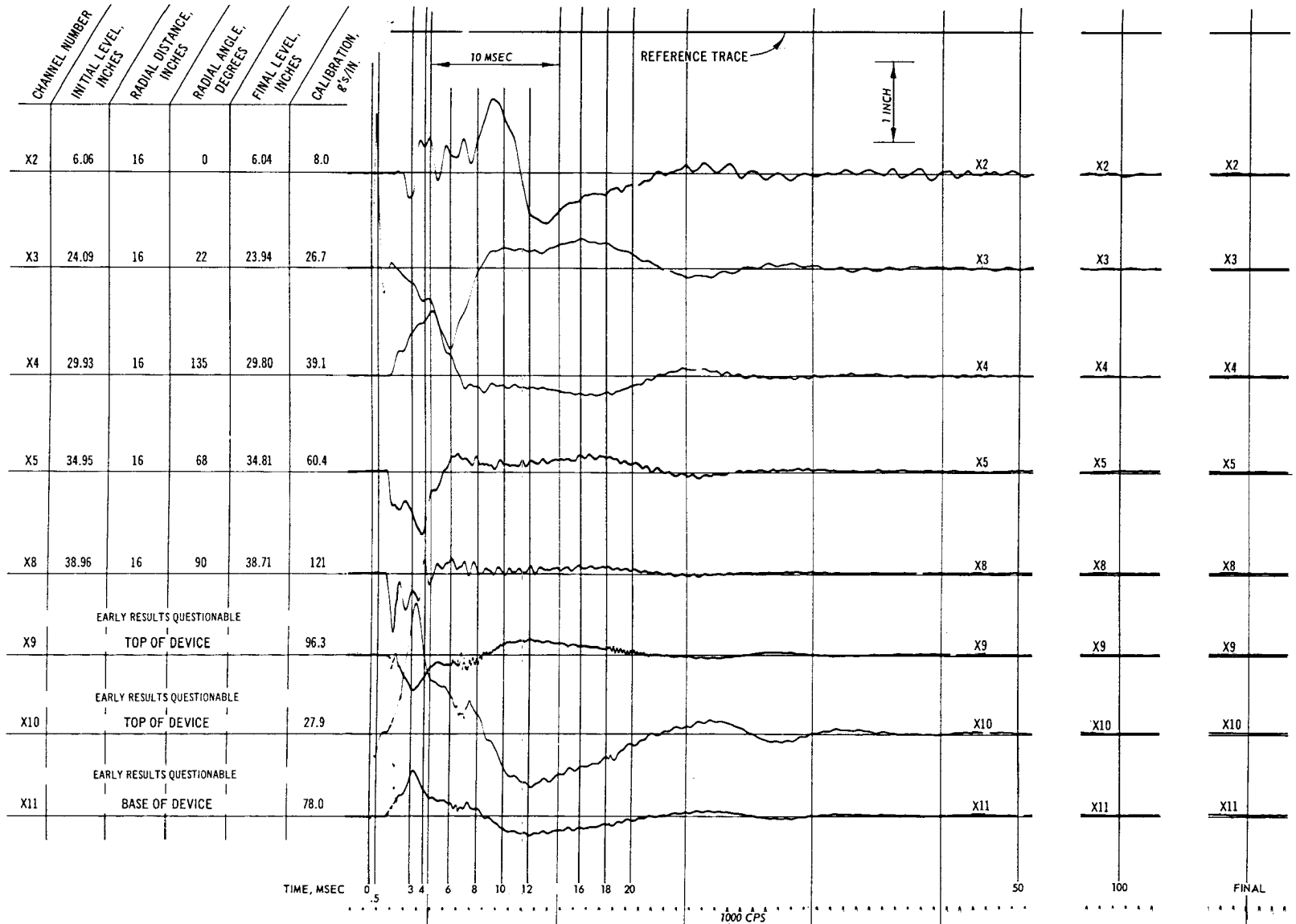
Fig. C-65. Test 26, acceleration record
