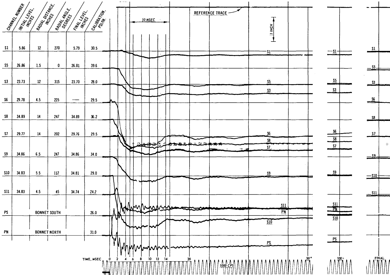
Fig. C-42. Test 21, pressure record
