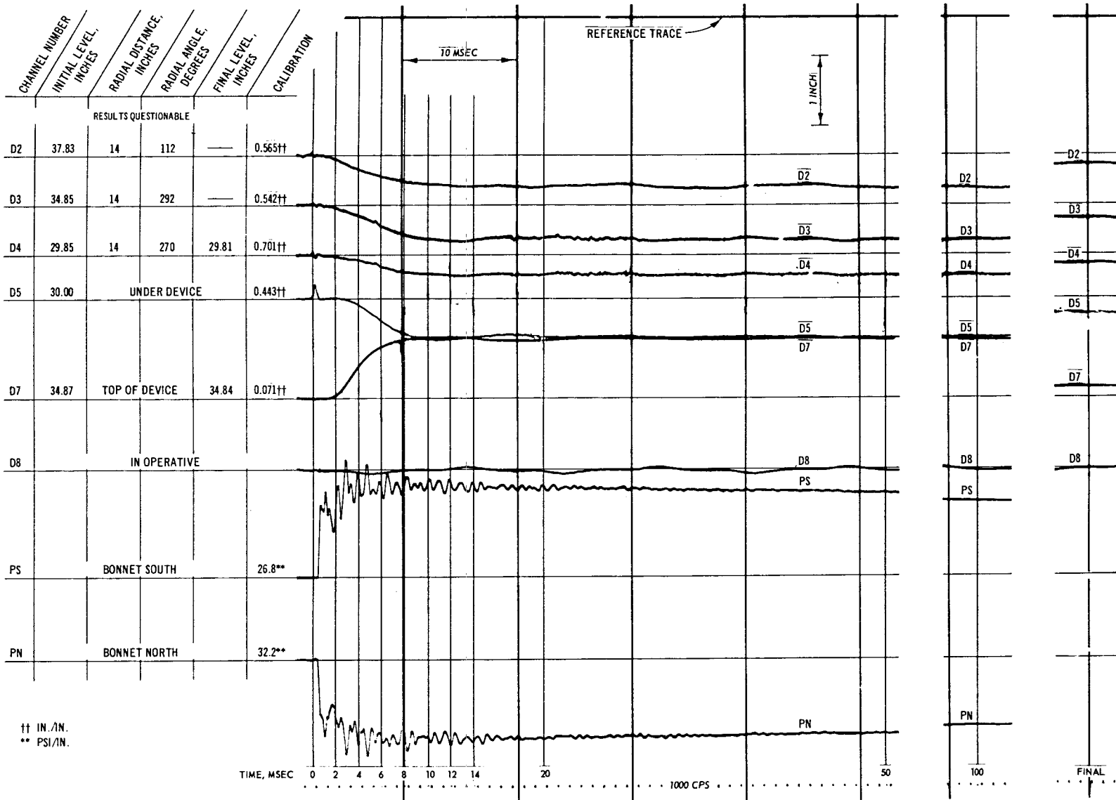
Fig. C-44. Test 21, deflection and pressure record
