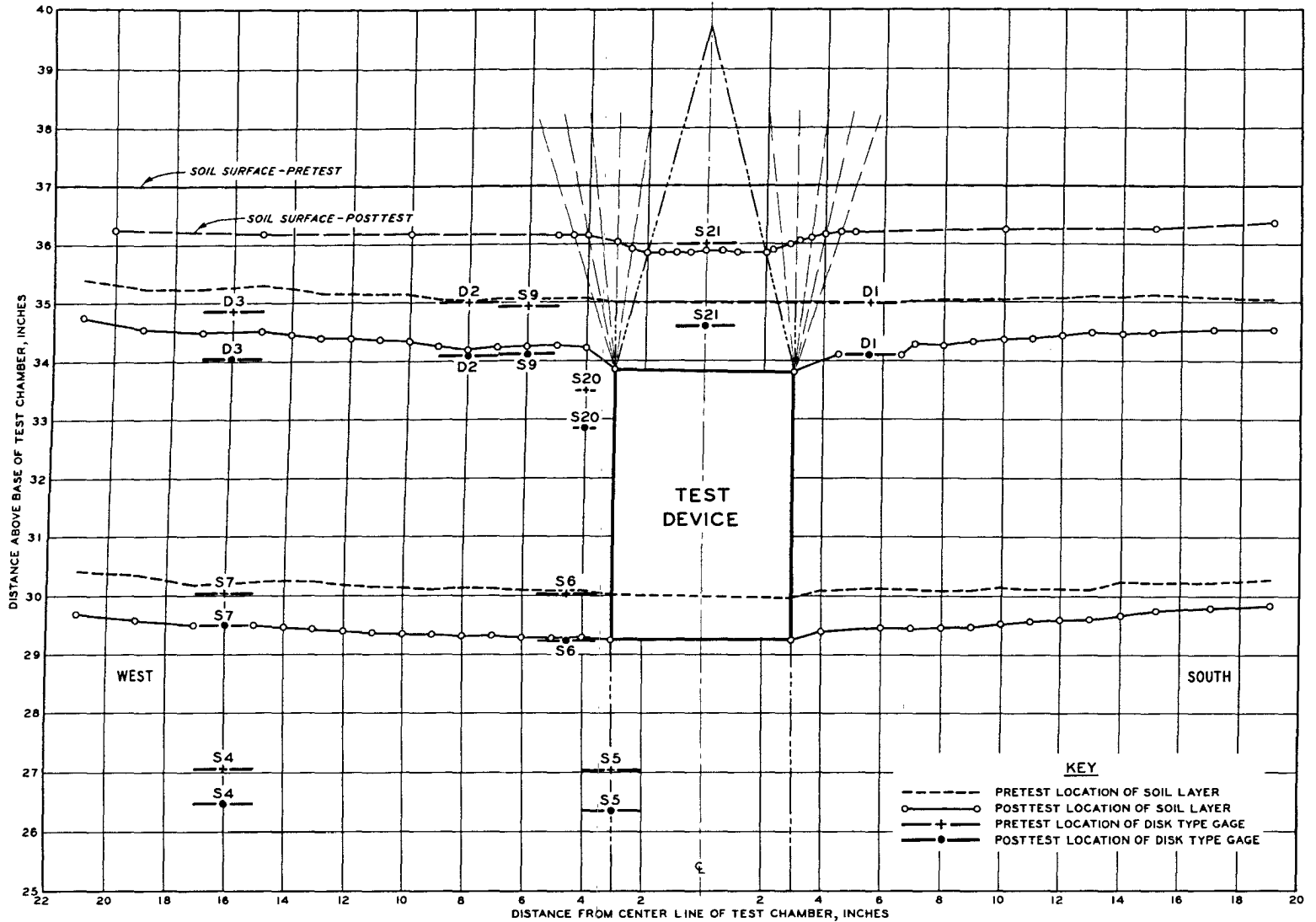
Fig. 42. Cross-section view of soil deformation, Test 1; H/B = 1/3 , P_s = 37.8 psi
