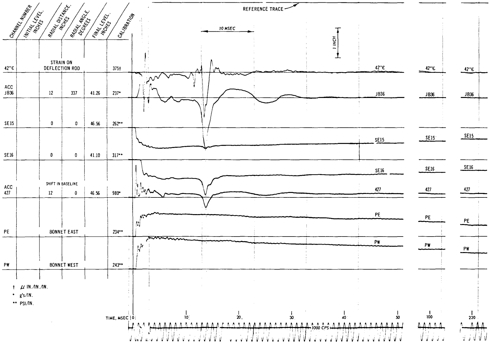
Fig. C-83. Test D, pressure, acceleration, and strain record
