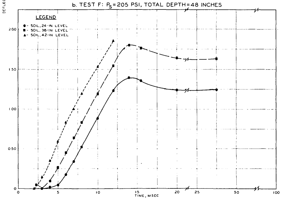
Fig. 75. Soil deflection versus time, preliminary Tests E and F
