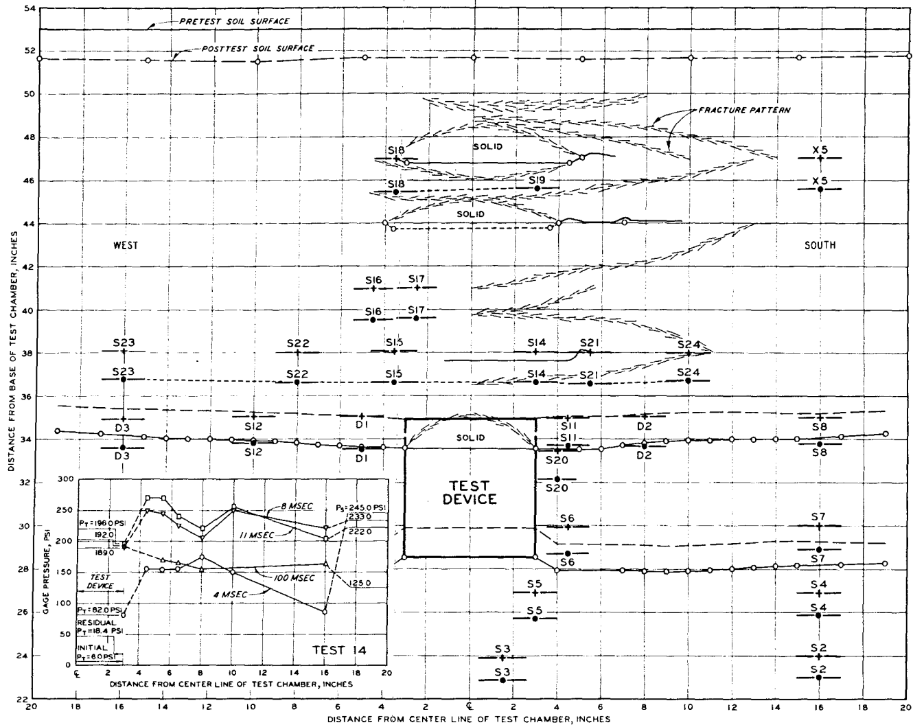
Fig. 82. Cross section of soil deformations, Test 14; H/B = 3 , P_S = 245 psi
