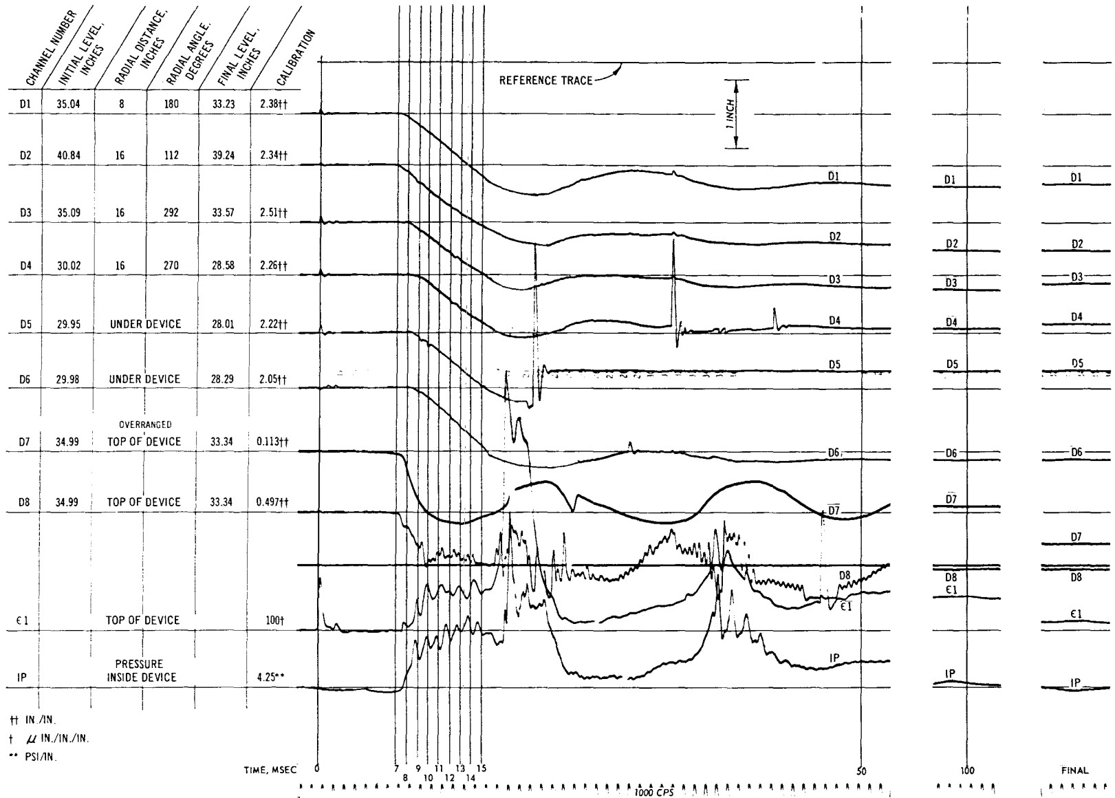
Fig. C-32. Test 18, deflection, strain, and pressure record
