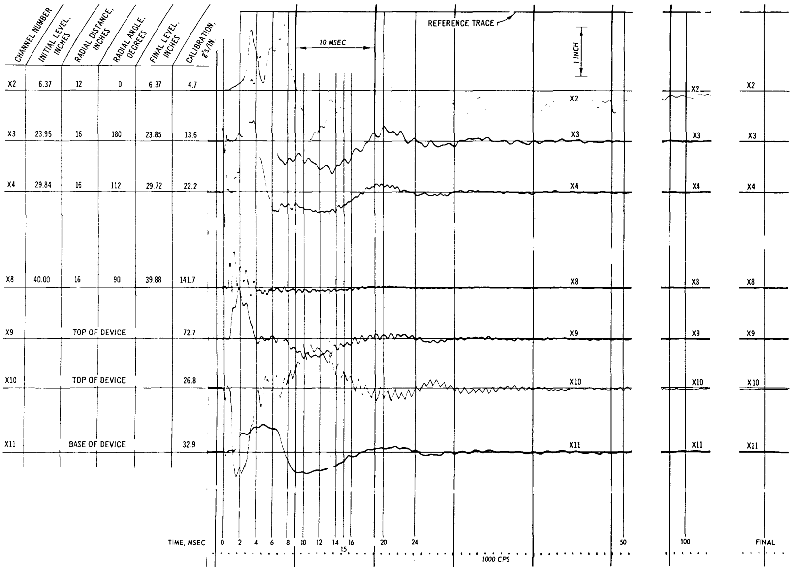
Fig. C-53. Test 23, acceleration record
