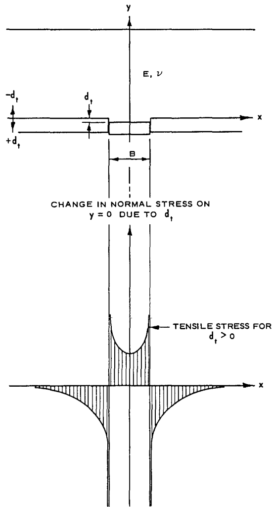
Fig. 4. Distribution of arching stresses from an elastic solution by Finn
