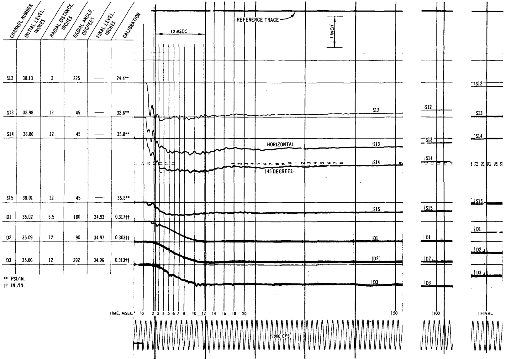
Fig. C-55. Test 24, pressure and deflection record
