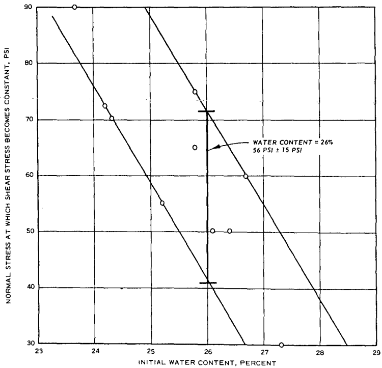
Fig. A-3. Approximate value of stress at which buckshot clay becomes saturated
