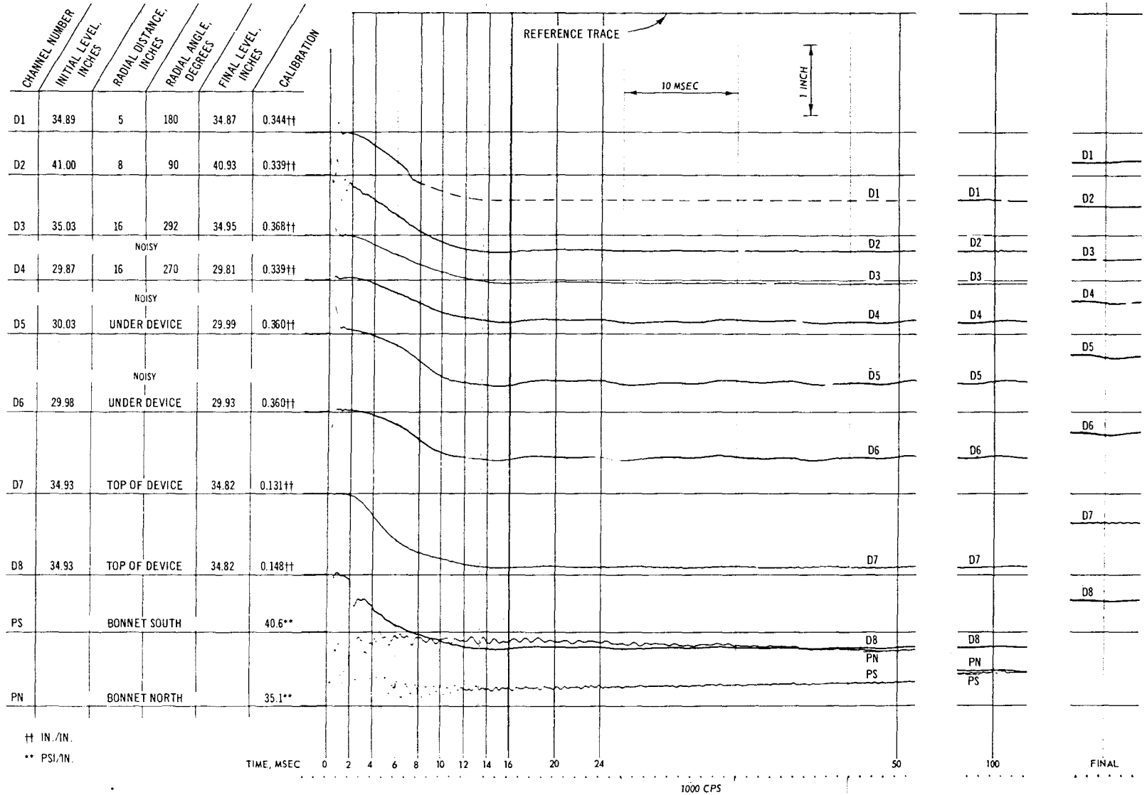
Fig. C-52. Test 23, deflection and pressure record
