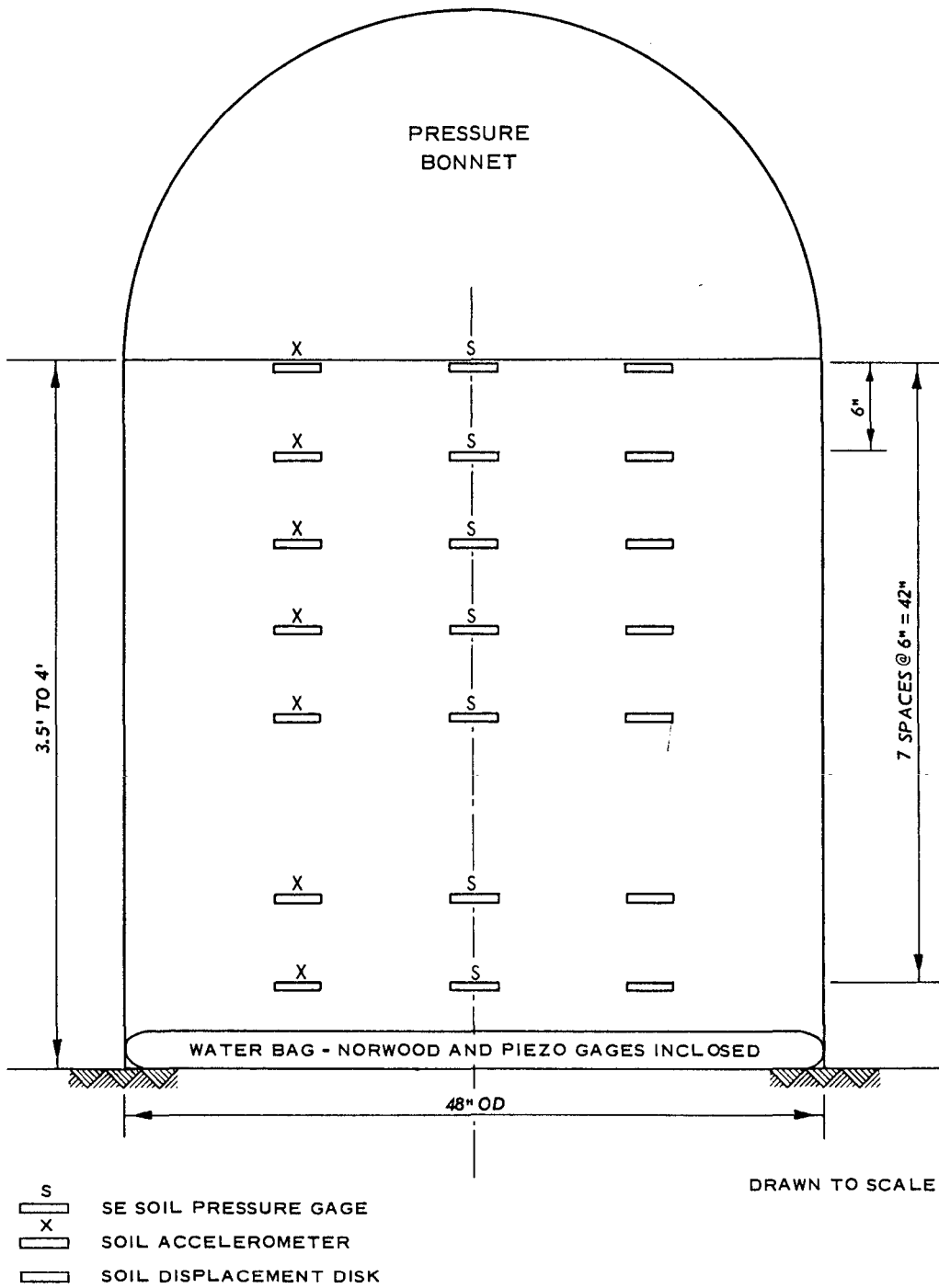
Fig. A-8. Test geometry for preliminary tests in SBLG
