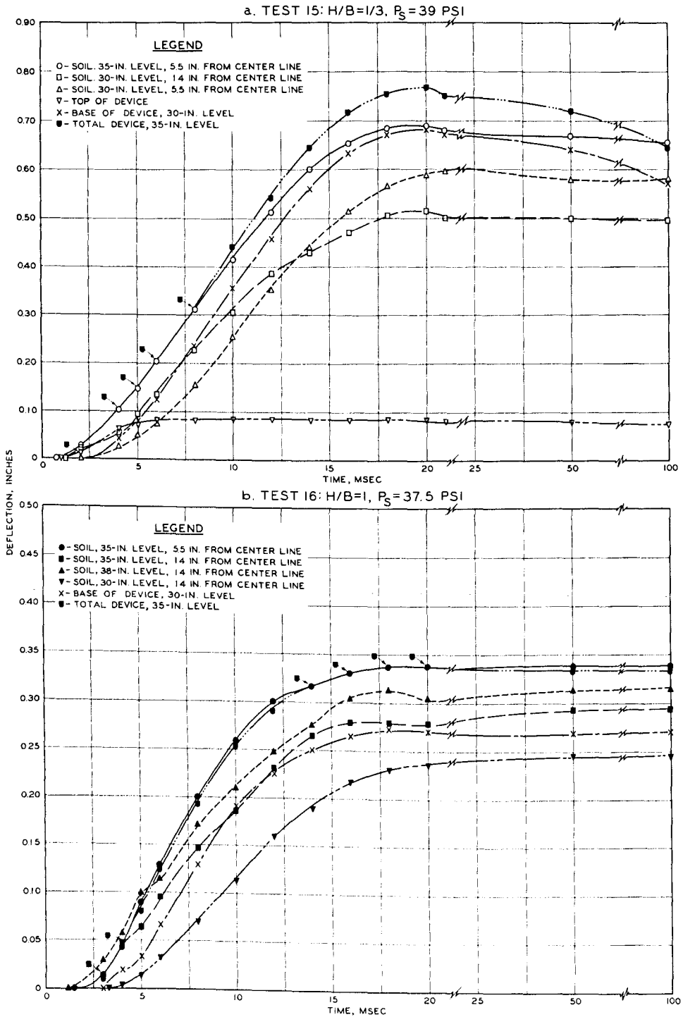
Fig. 72. Soil and structure deflection versus time, Tests 15 and 16
