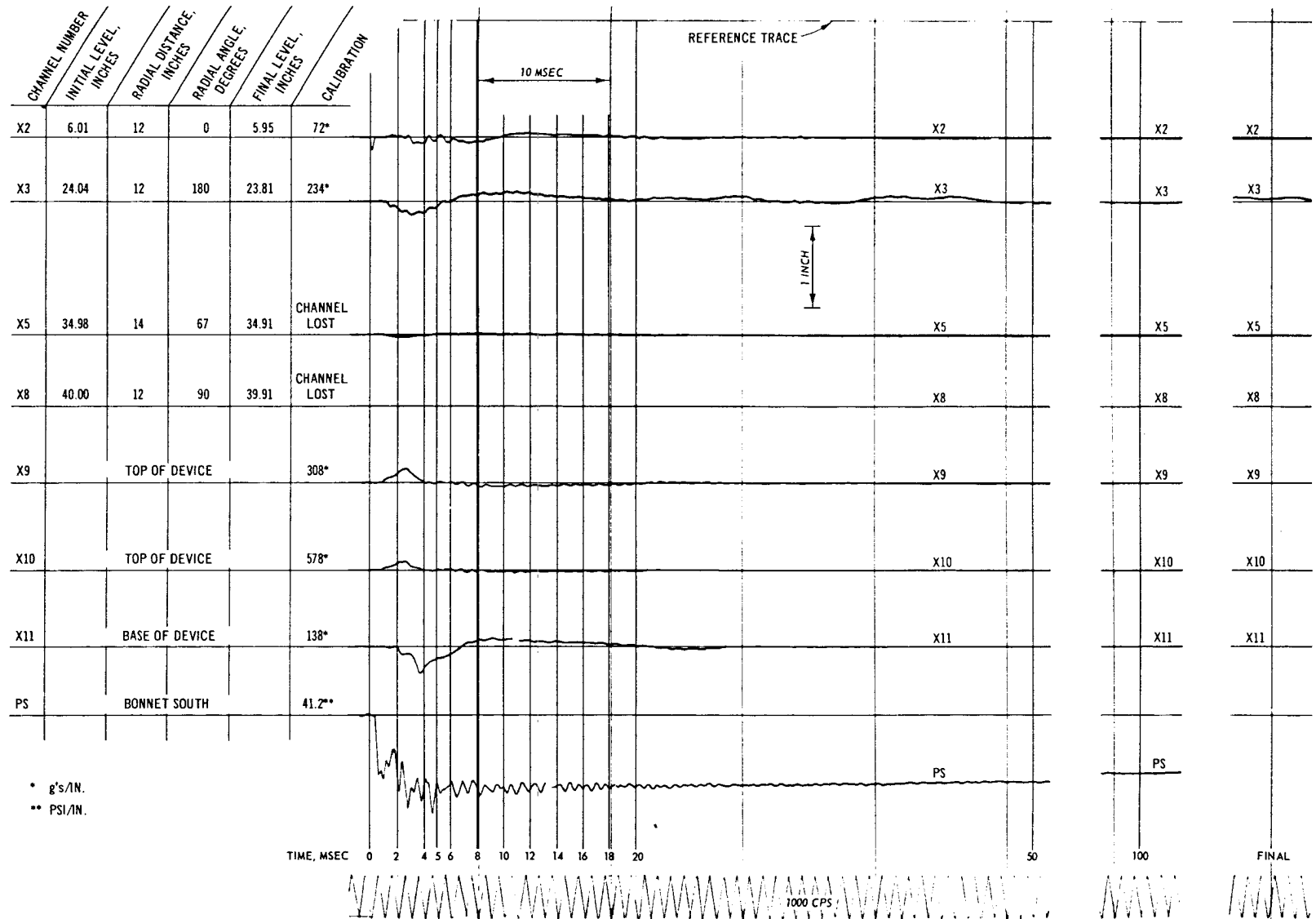
Fig. C-25. Test 16, acceleration and pressure record
