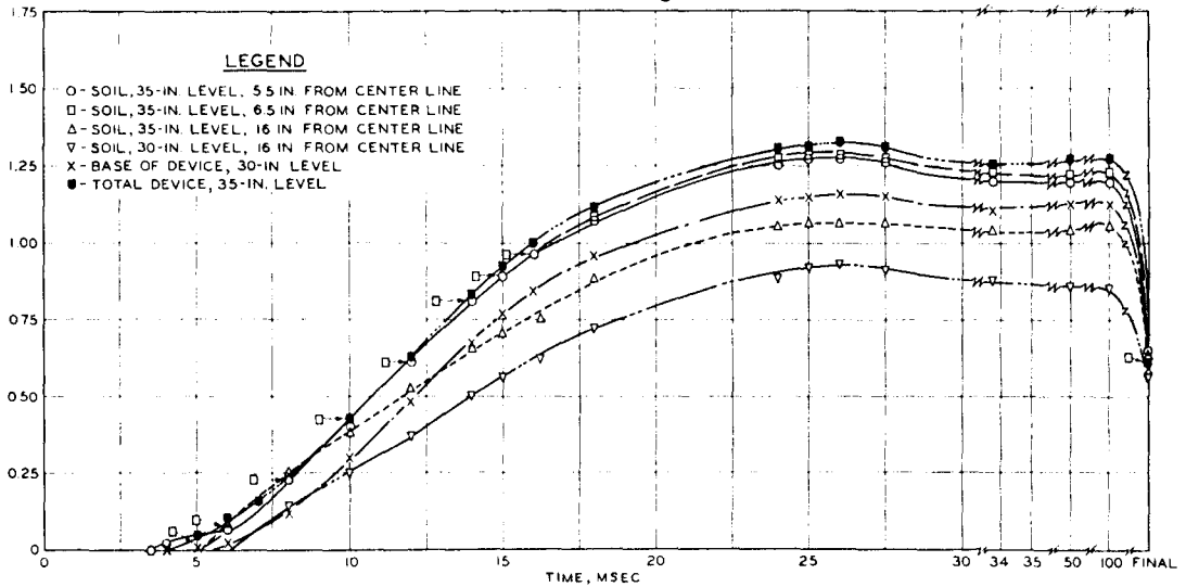
b. TEST 12: H/B=3, P_s = 70 PSI
