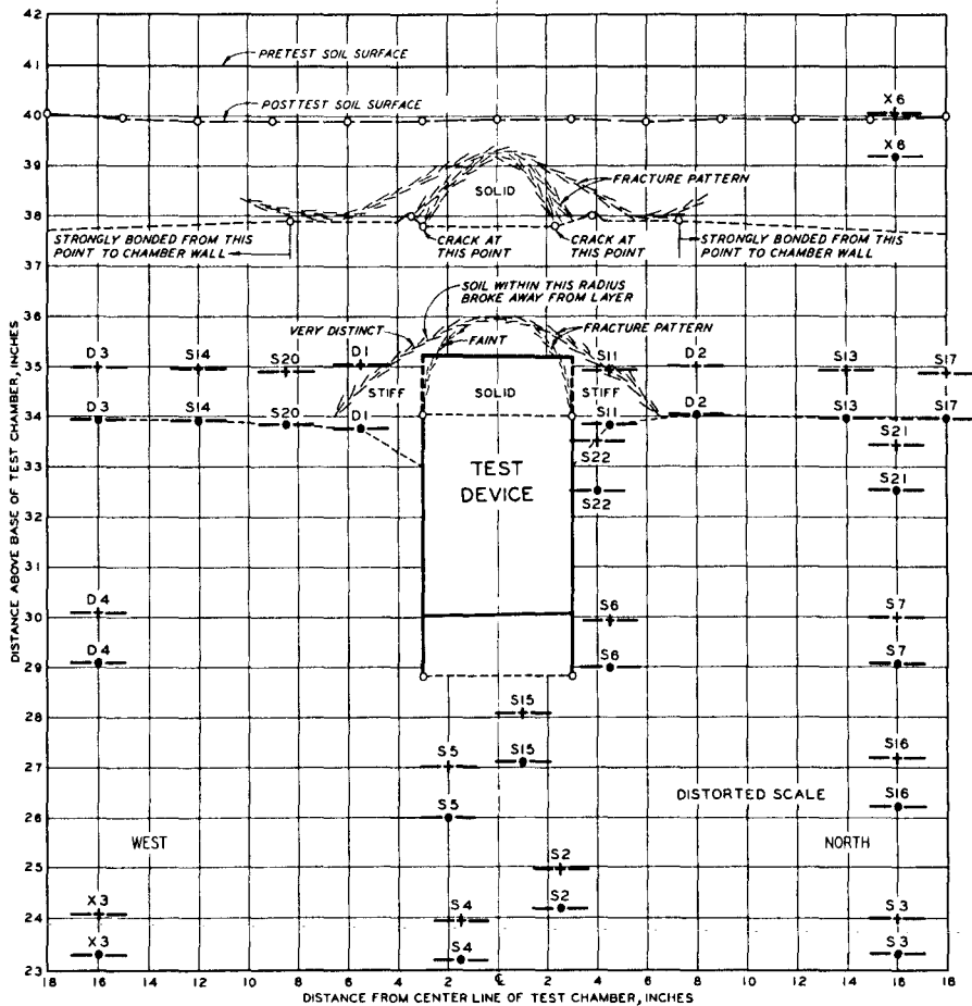
a. CROSS SECTION OF SOIL DEFORMATIONS
