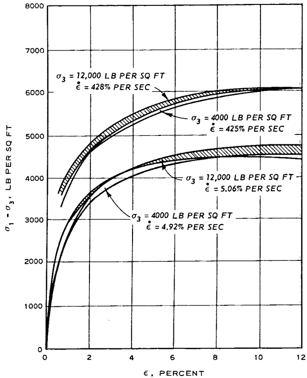
A. BUCKSHOT CLAY STRESS-STRAIN CURVES WC = 27.1 ± 0.3%
