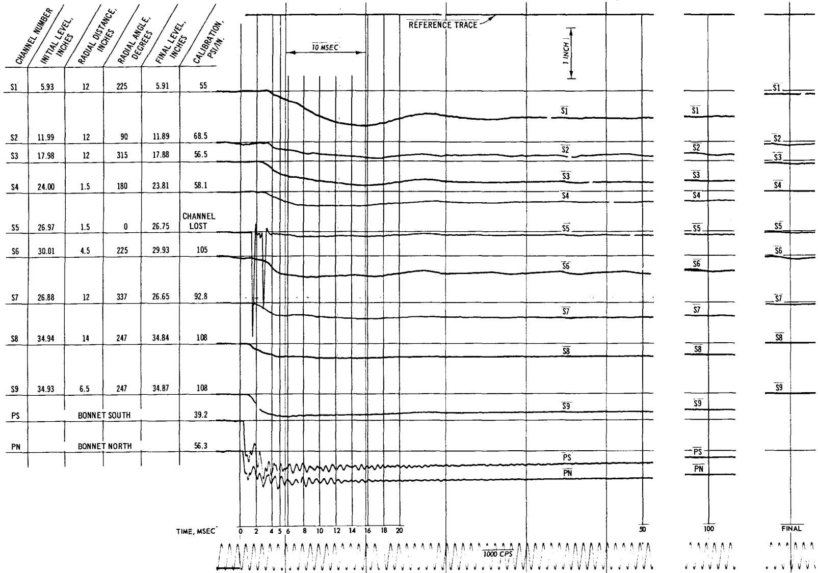
Fig. C-22. Test 16, pressure record (S1-S9)
