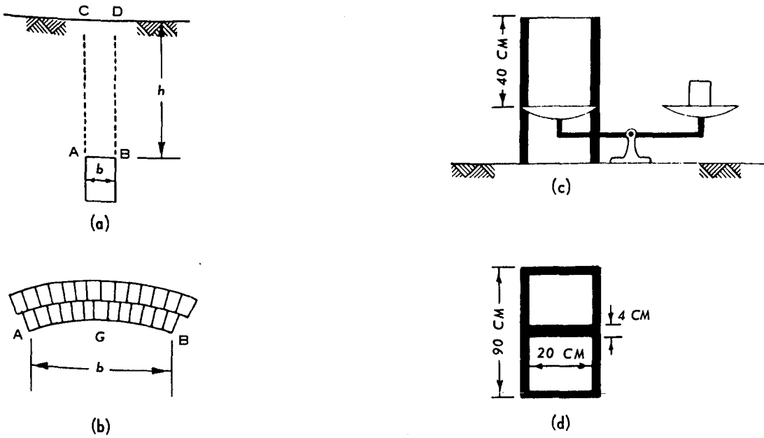
Fig. 1. Analytical and experimental study by Engesser
