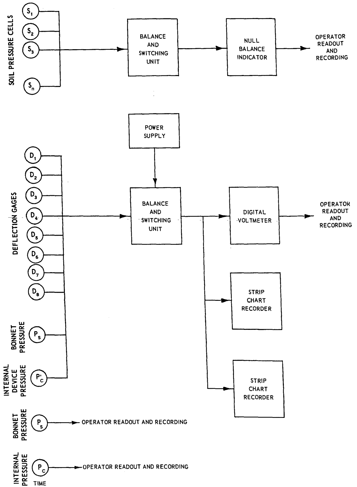
Fig. 18. Block diagram of measurement and control system used for static tests
