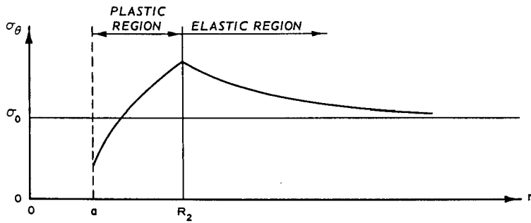
(b) ACTIVE ARCHING - p \ll \sigma_0
