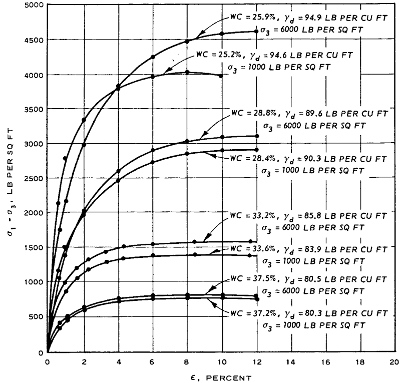
B. BUCKSHOT CLAY UU STRESS-STRAIN CURVES
