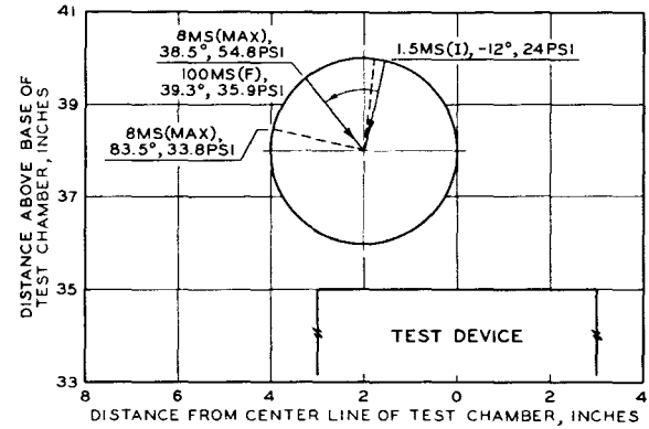
b. DIRECTION OF PRINCIPAL STRESS AND PLANES OF MAXIMUM SHEAR
