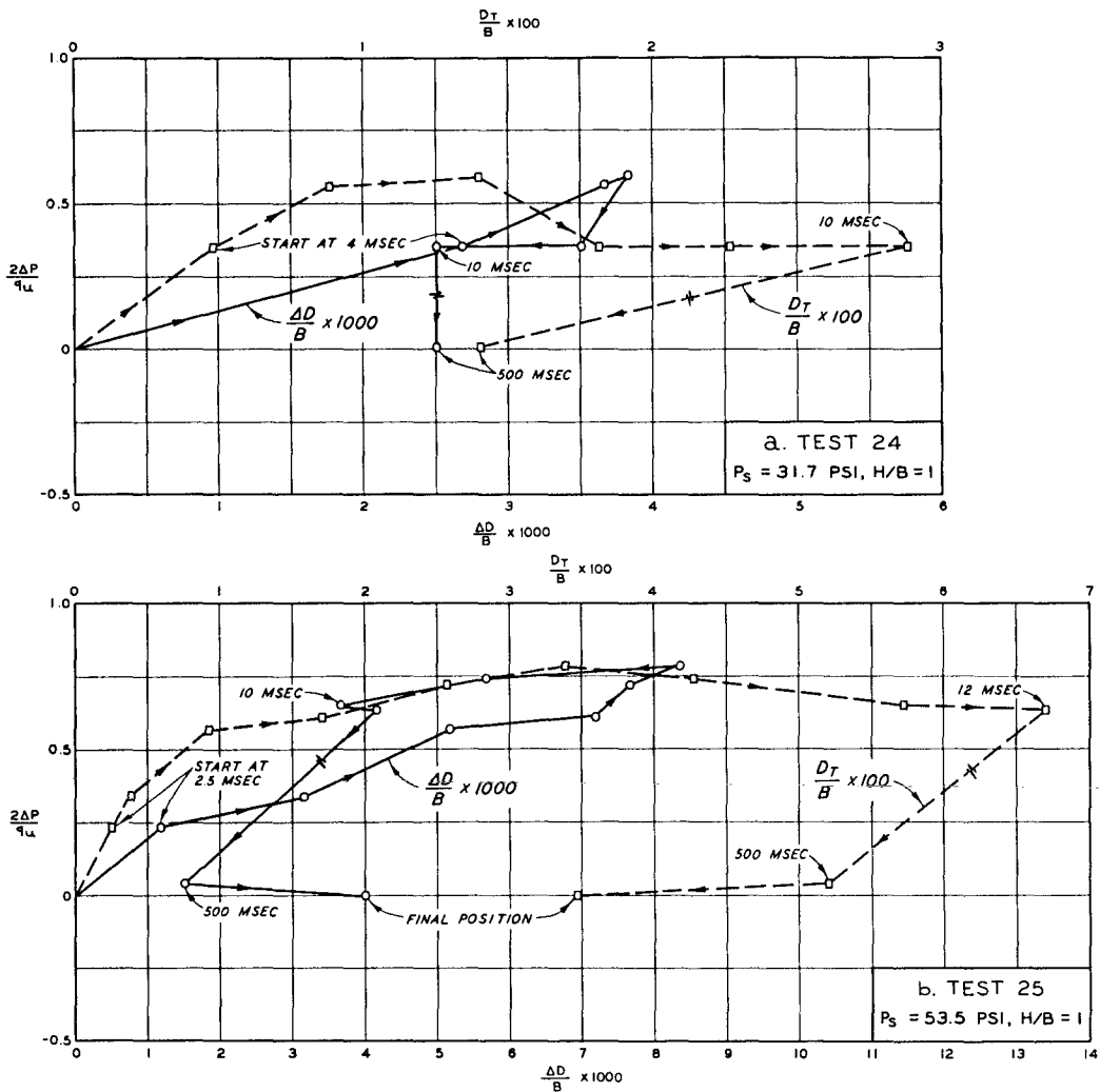
Fig. 57. Dimensionless plot of pressure versus deflection for dynamic Tests 24 and 25
