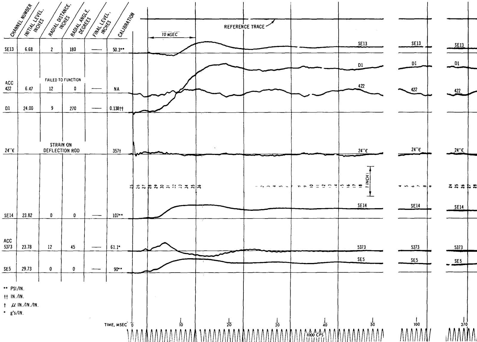
Fig. C-87. Test E, pressure, acceleration, deflection, and strain record
