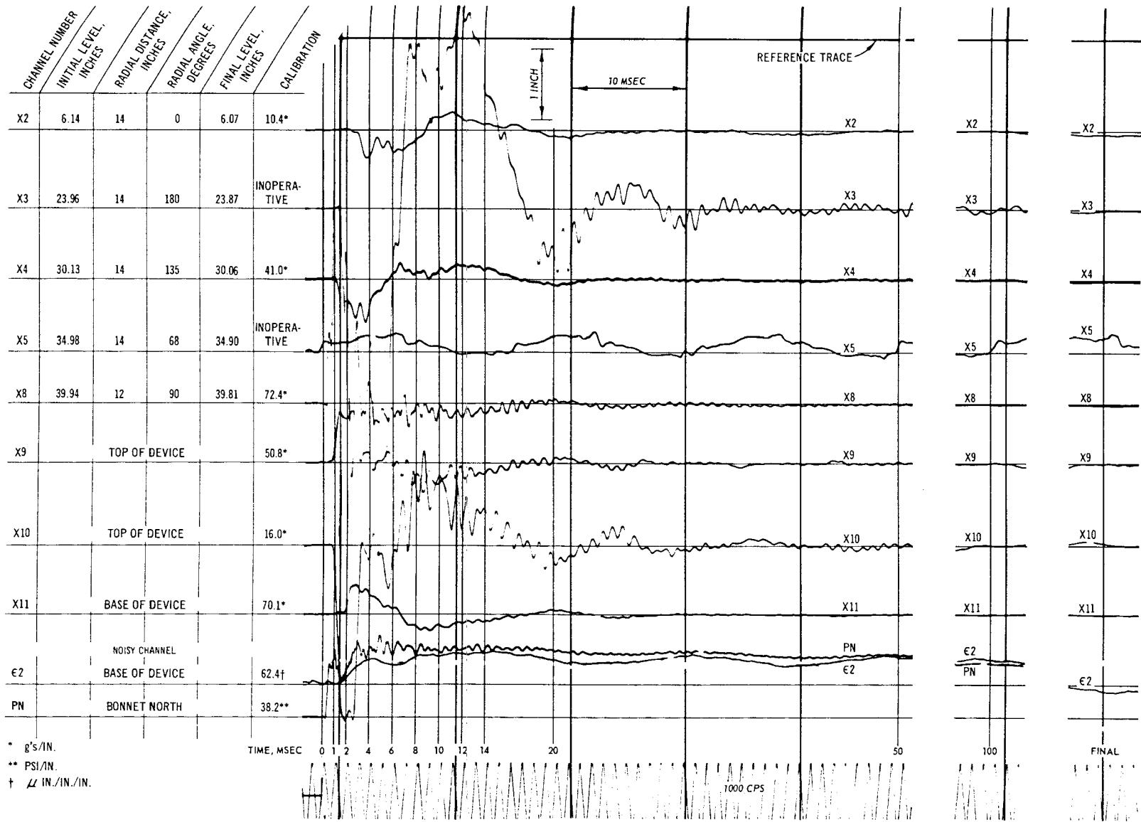
Fig. C-49. Test 22, acceleration, strain, and pressure record
