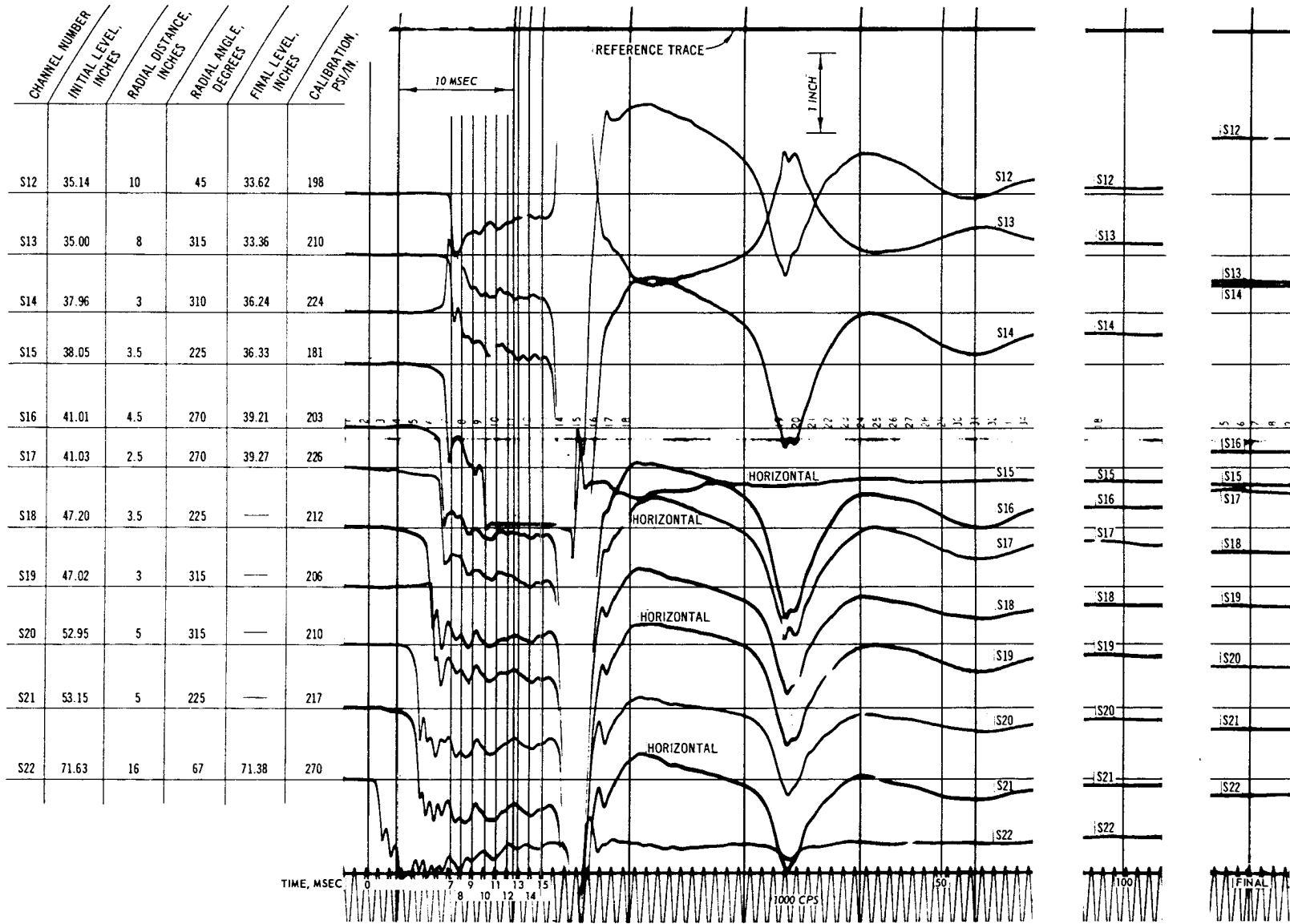
Fig. C-31. Test 18, pressure record (S12-S22)
