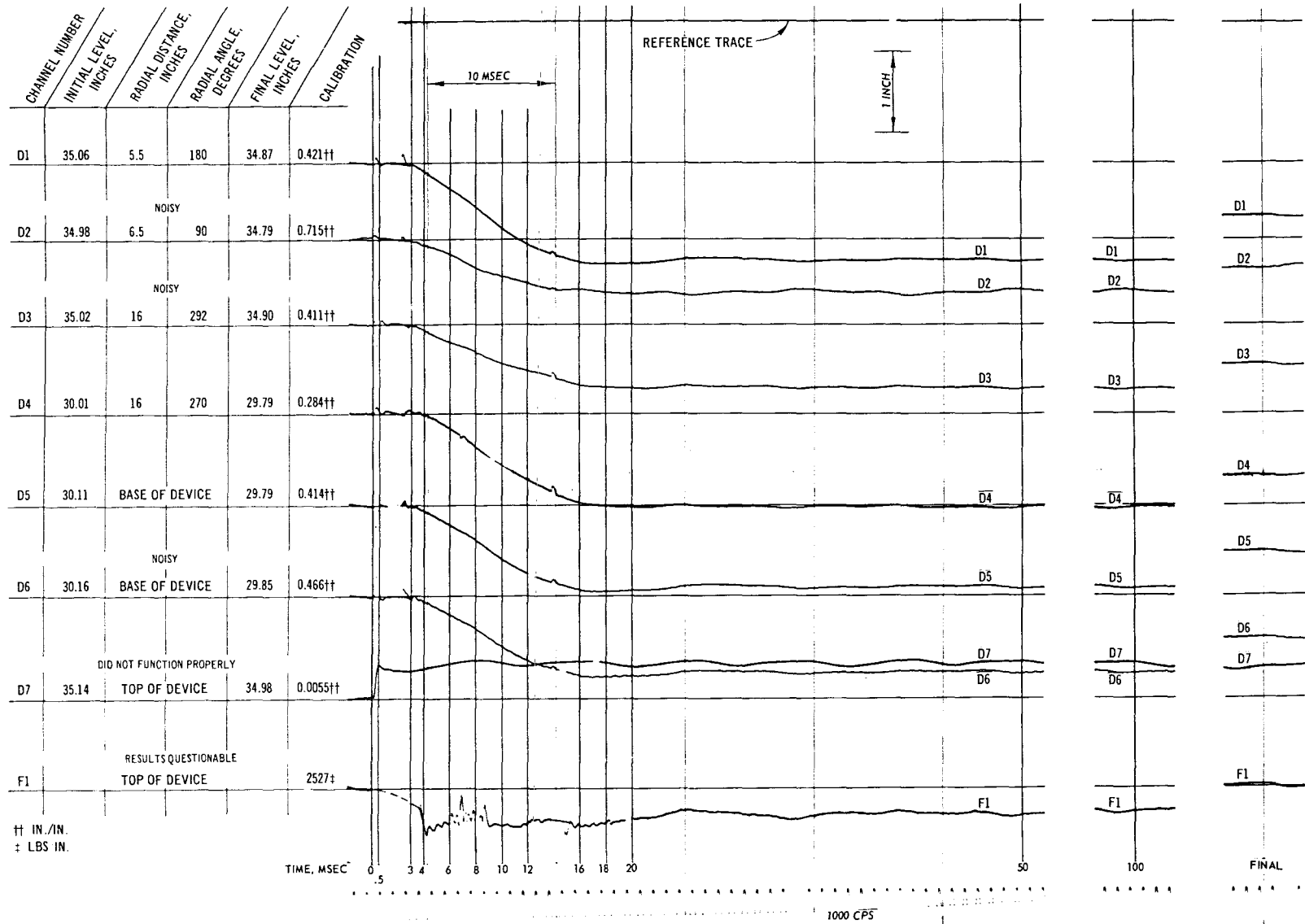
Fig. C-64. Test 26, deflection and force record
