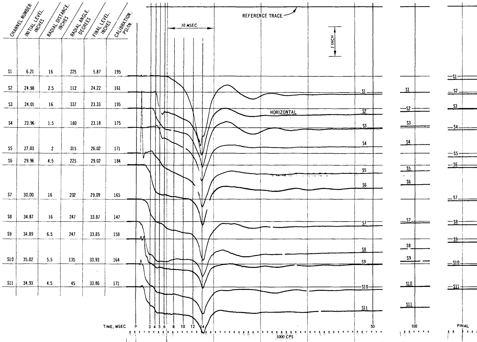
Fig. C-34. Test 19, pressure record (S1-S11)
