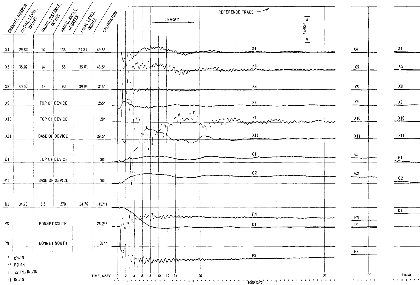
Fig. C-45. Test 21, pressure, acceleration, deflection, and strain record
