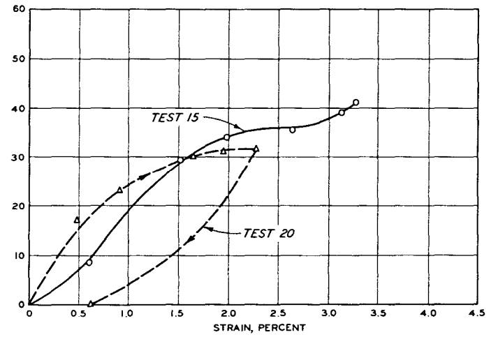
a. LOW PRESSURE TESTS, P_S < 40 PSI
