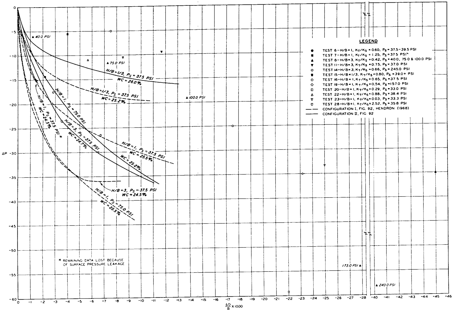
Fig. 94. Active arching, static and dynamic surface pressures, \Delta P versus \frac{AD}{B} \times 1,000
