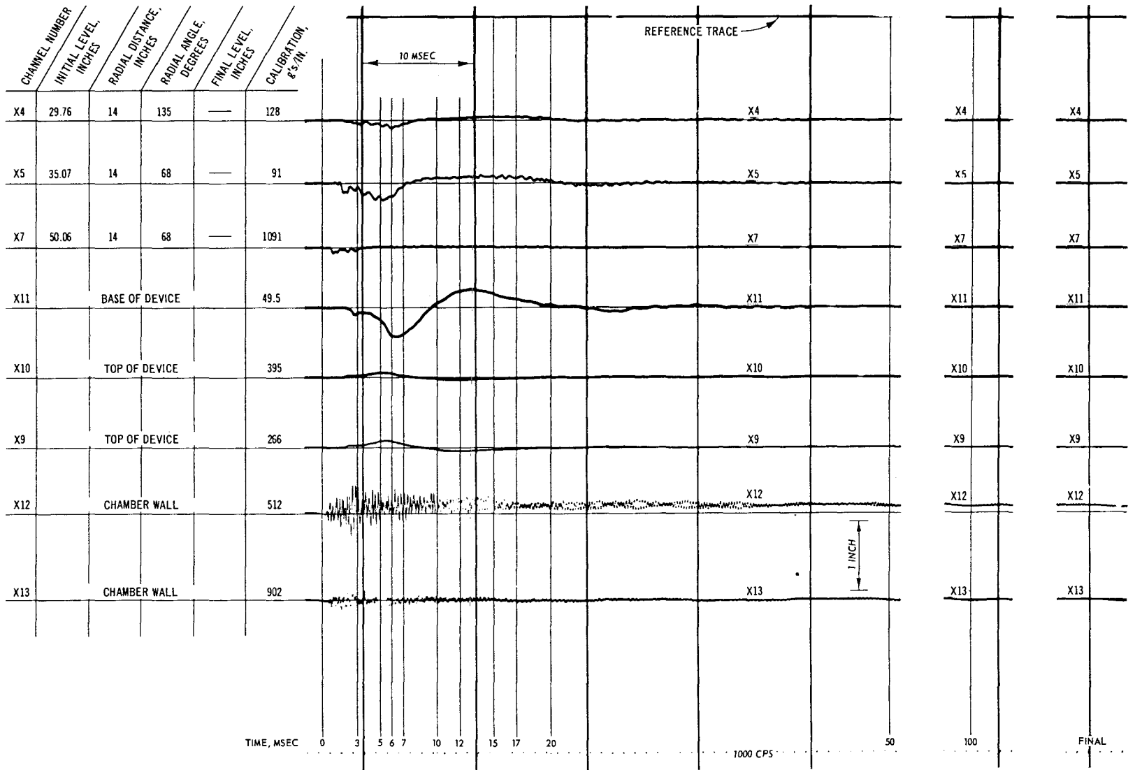
Fig. C-5. Test 11, acceleration record (X4-X13)
