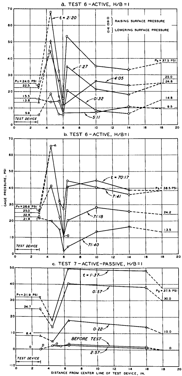
Fig. 28. Change in vertical soil stress at the 35-inch level due to deflection of top of test device, Tests 6 and 7
