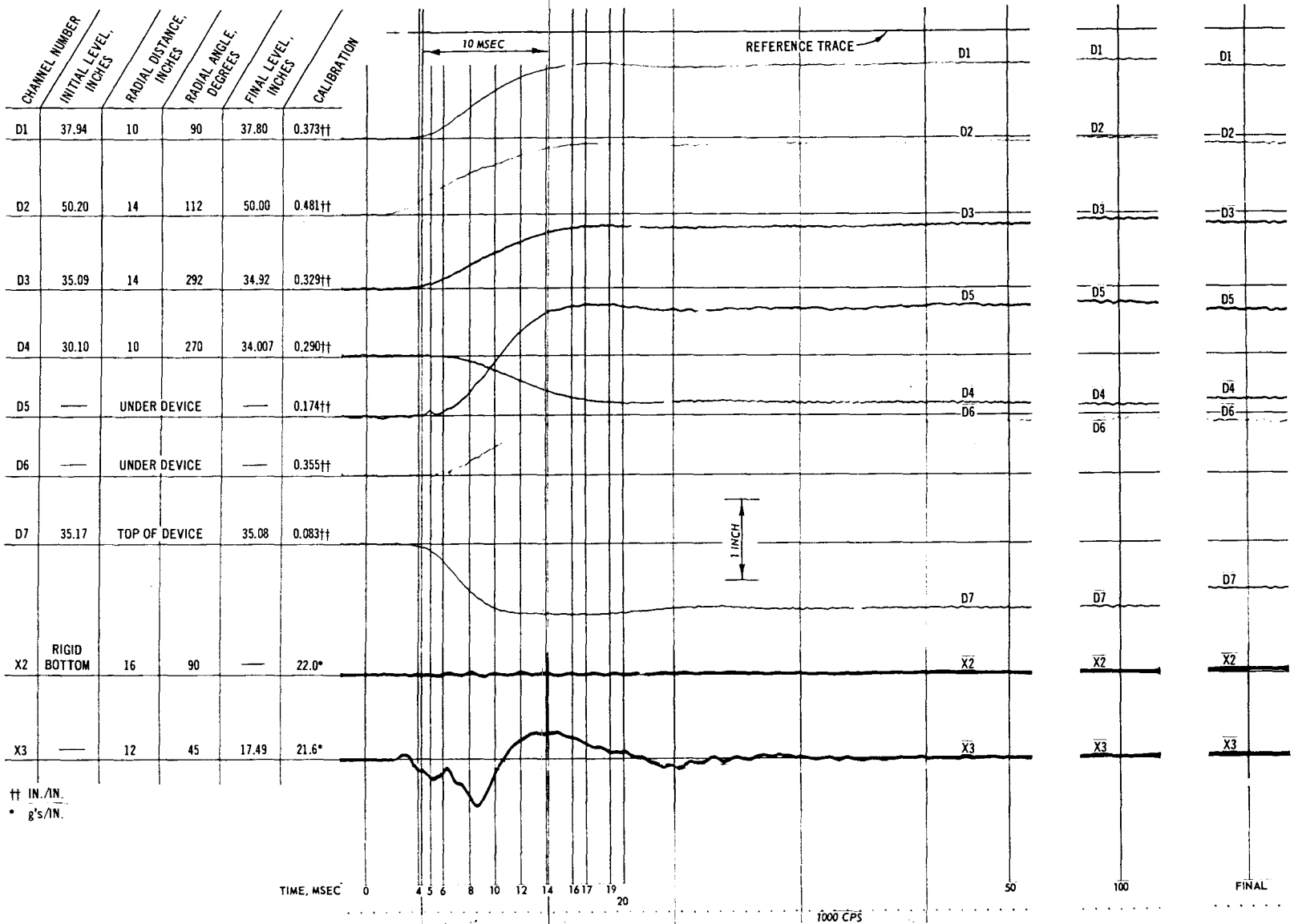
Fig. C-28. Test 17, deflection and acceleration record
