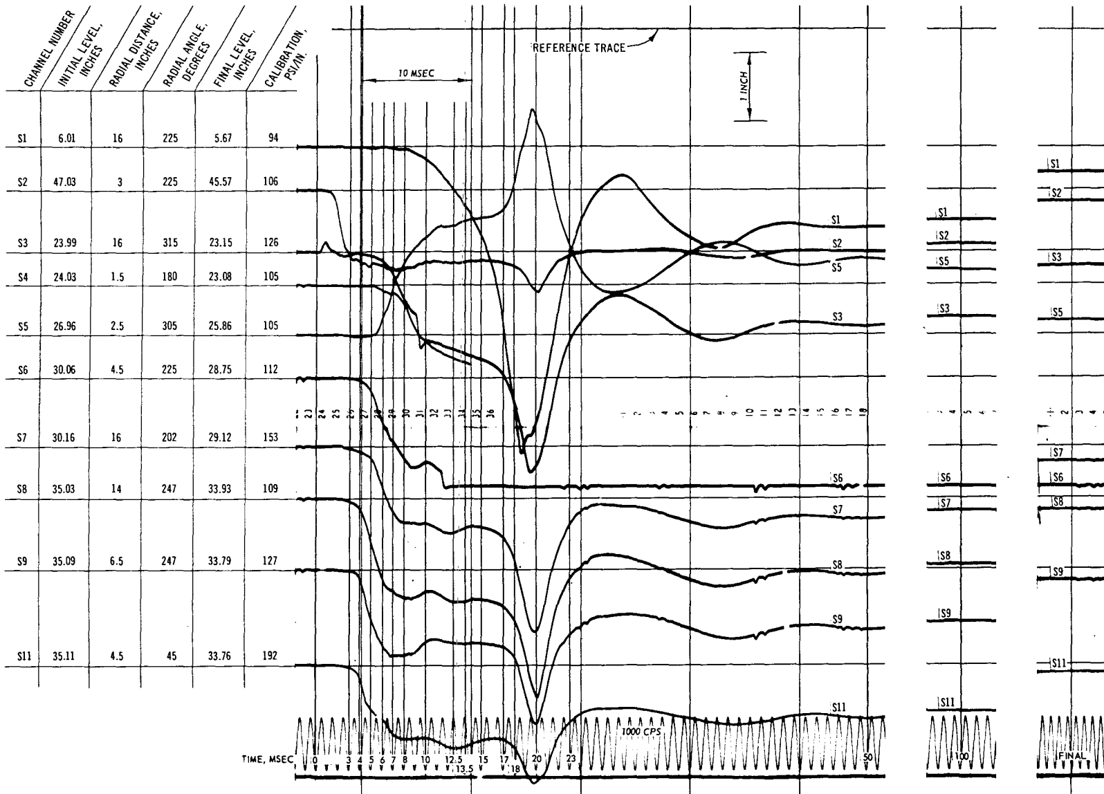
Fig. C-10. Test 13, pressure record (S1-S11)
