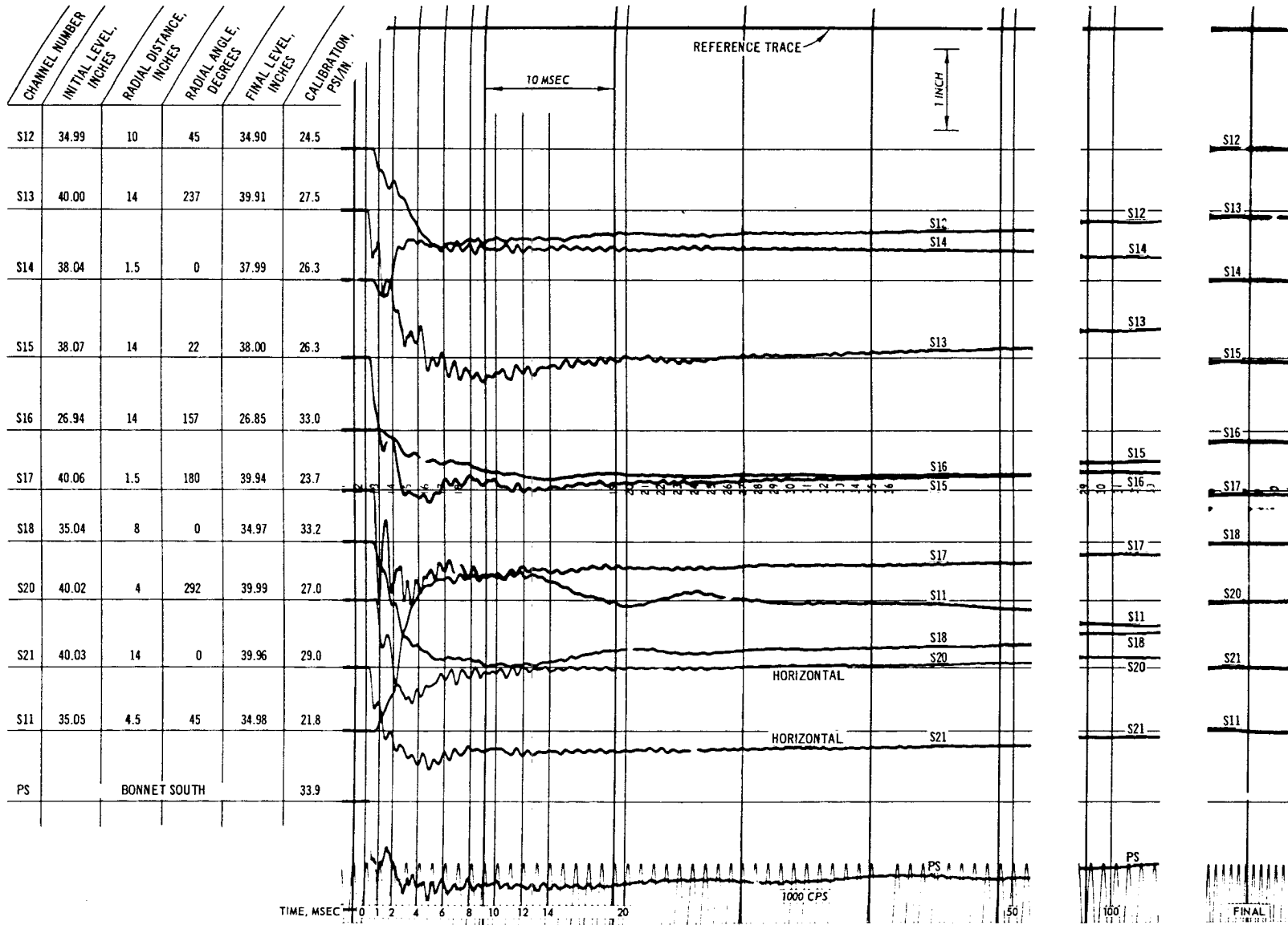
Fig. C-47. Test 22, pressure record (S12-S21, S11)
