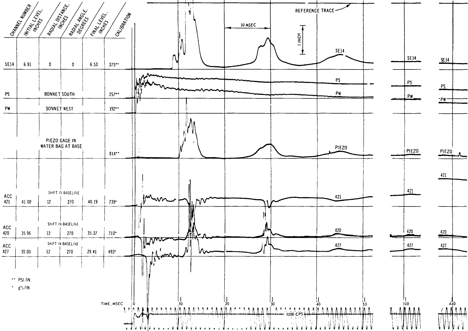
Fig. C-81. Test C, pressure and acceleration record
