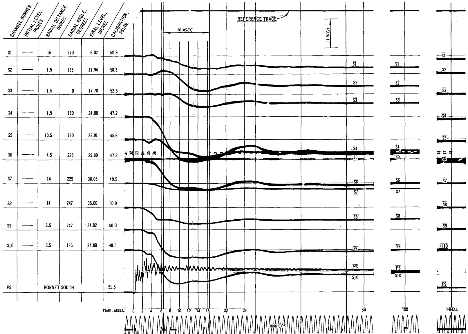
Fig. C-26. Test 17, pressure record (S1-S10)
