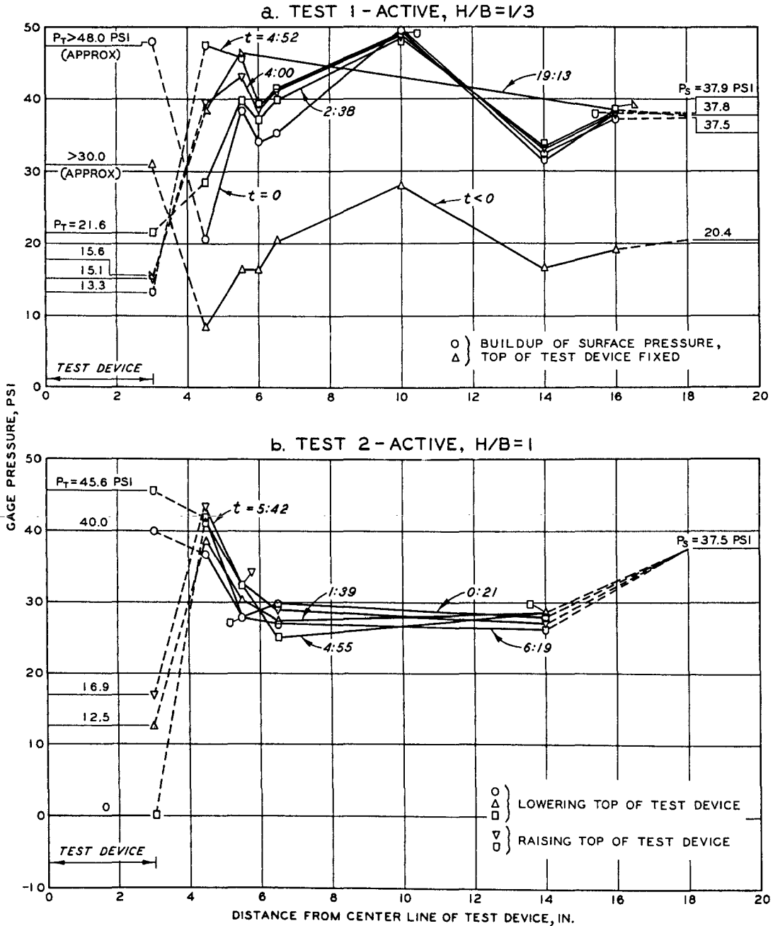
Fig. 26. Change in vertical soil stress at the 35-inch level due to deflection of the top of test device, Tests 1 and 2
