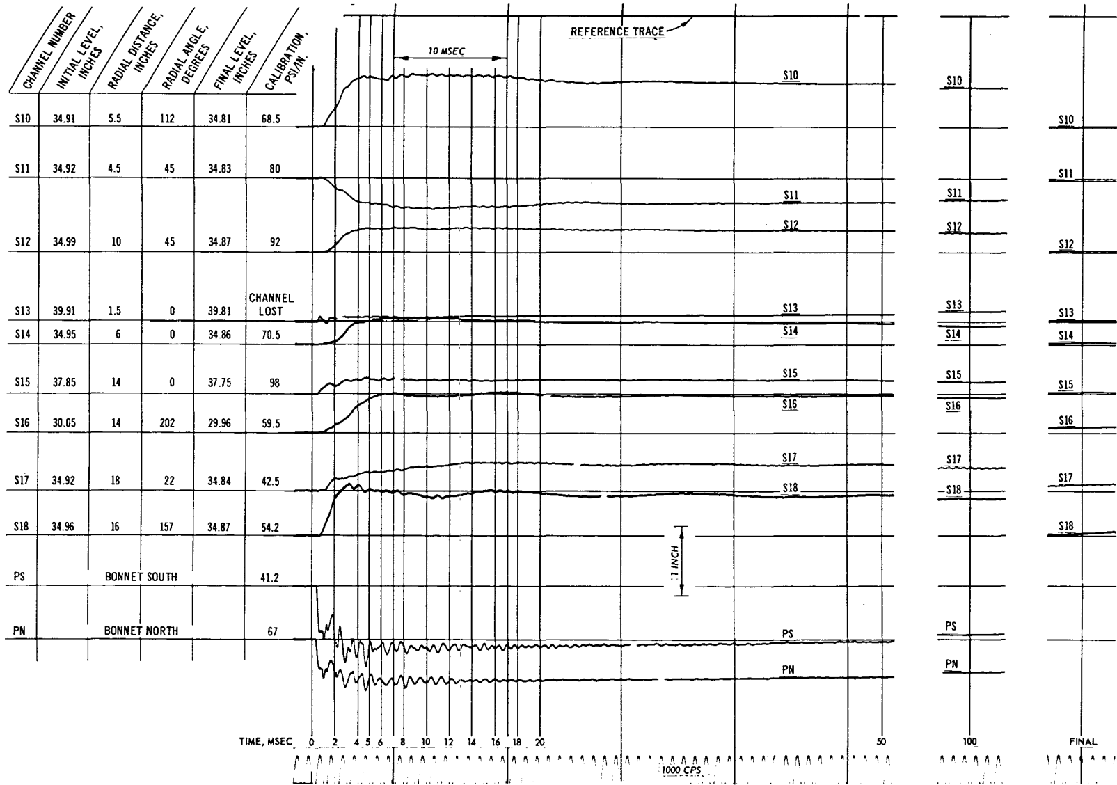
Fig. C-23. Test 16, pressure record (S10-S18)
