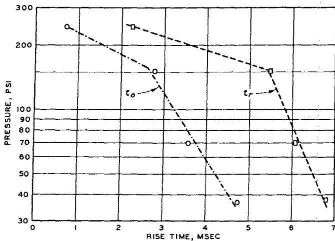
c. VARIATION OF SOIL PRESSURE RISE TIME WITH PEAK SURFACE PRESSURE, H/B = 3
