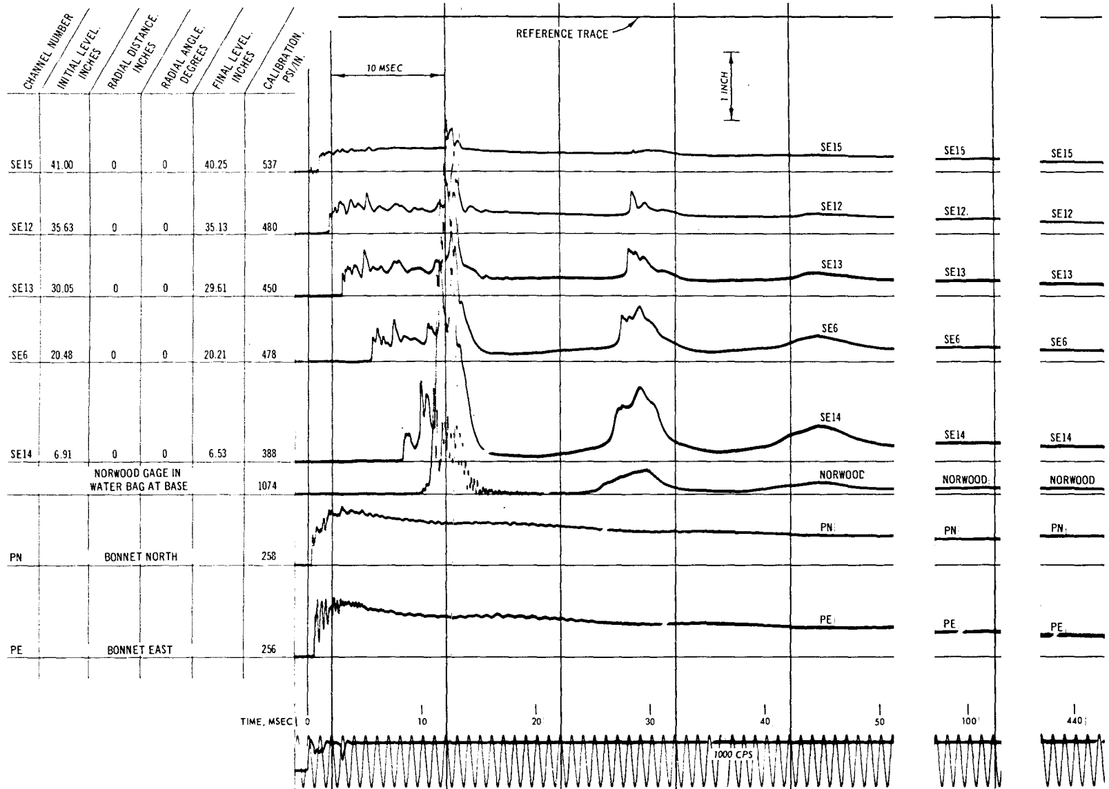
Fig. C-80. Test C, pressure record
