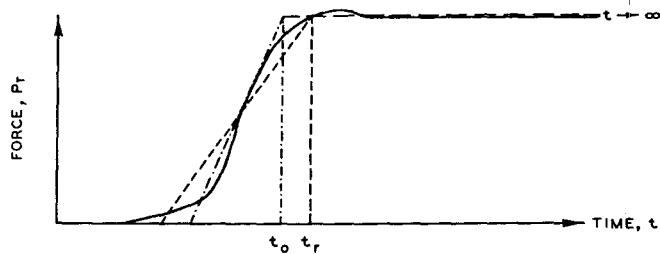
a. ACTUAL AND IDEALIZED FORCE-TIME RELATION
