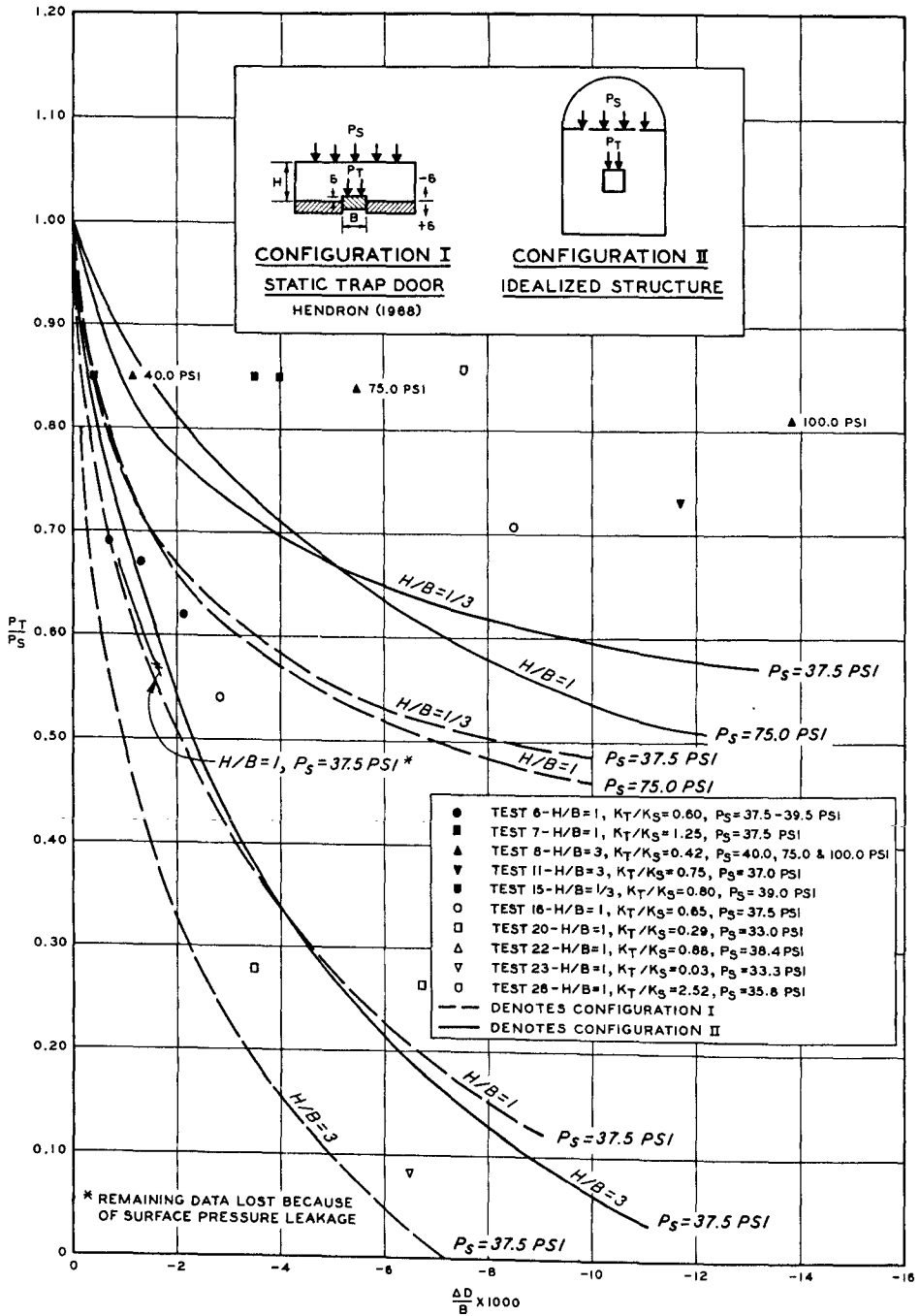
Fig. 92. Active arching curves, static surface pressure
