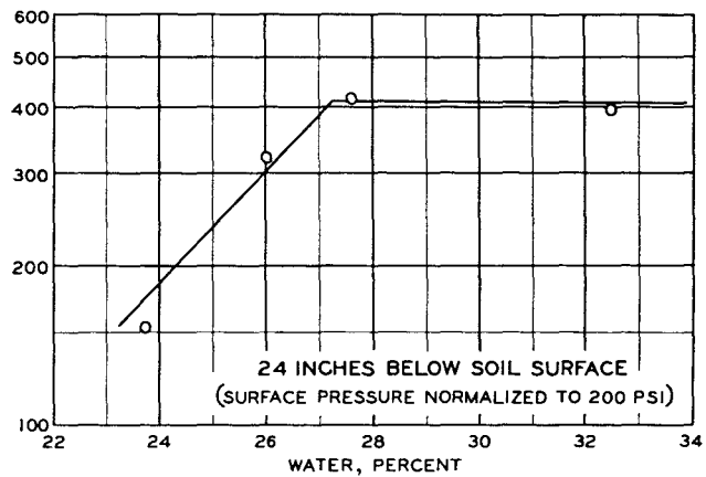
b. PEAK STRESS WAVE VELOCITY VERSUS SOIL WATER CONTENT
