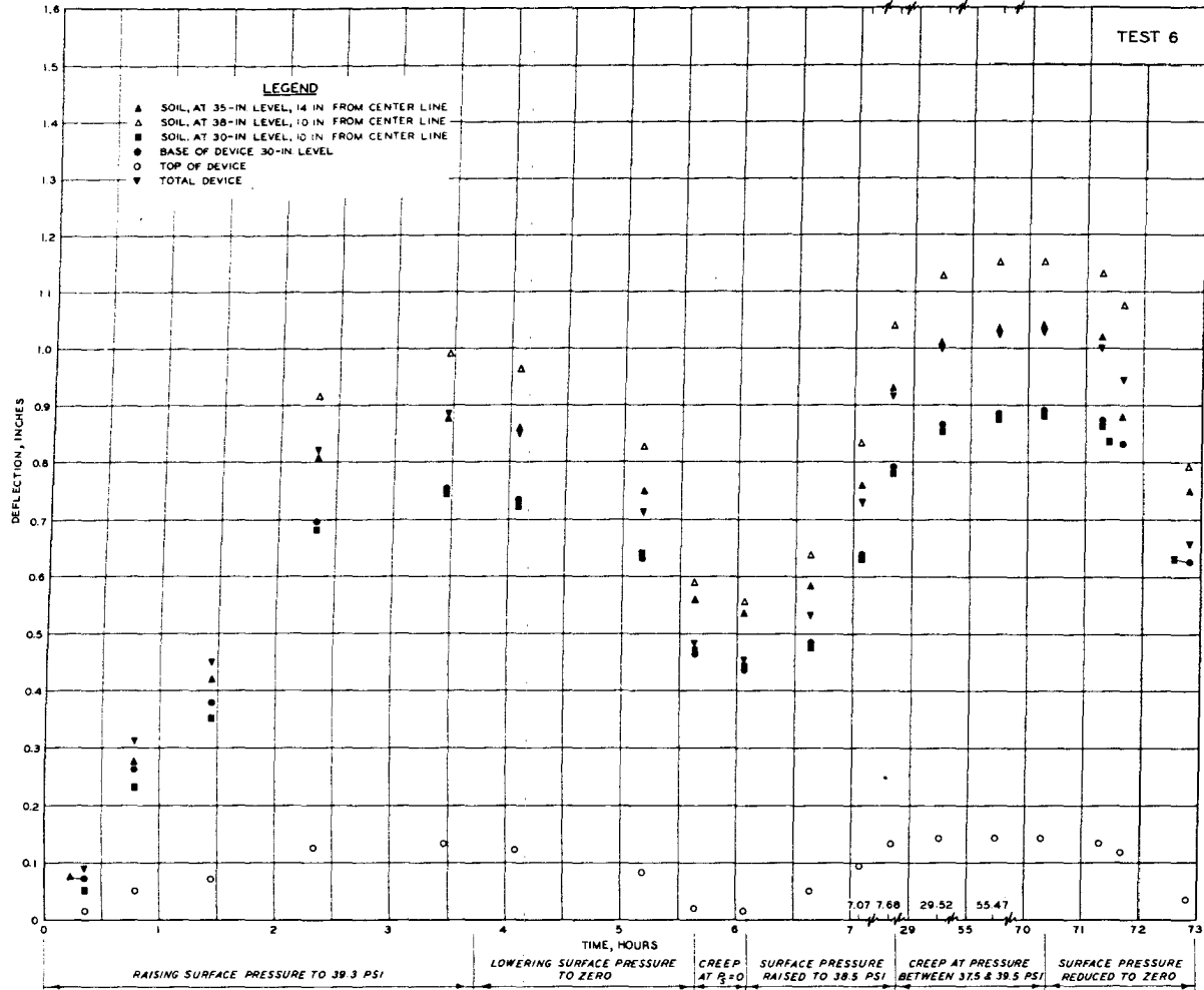
Fig. 38. Soil and structure deflections versus time; Test 6, H/B = 1 , P_S = 39.3 psi
