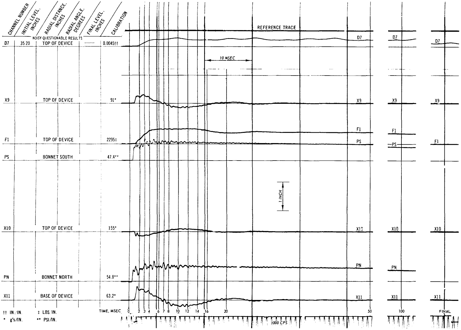
Fig. C-67. Test 27A, deflection, pressure, acceleration, and force record
