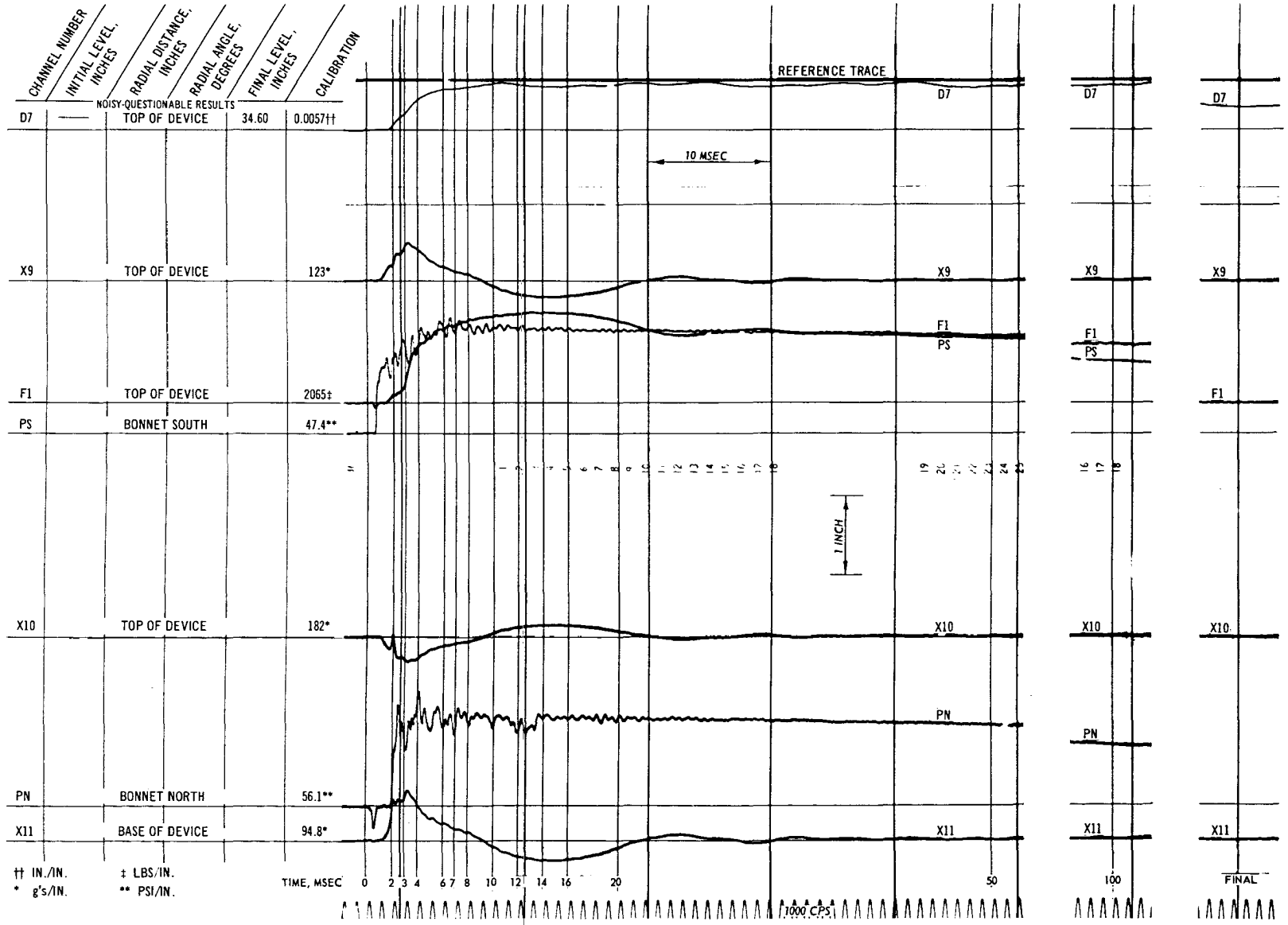
Fig. C-71. Test 27C, deflection, pressure, acceleration, and force record
