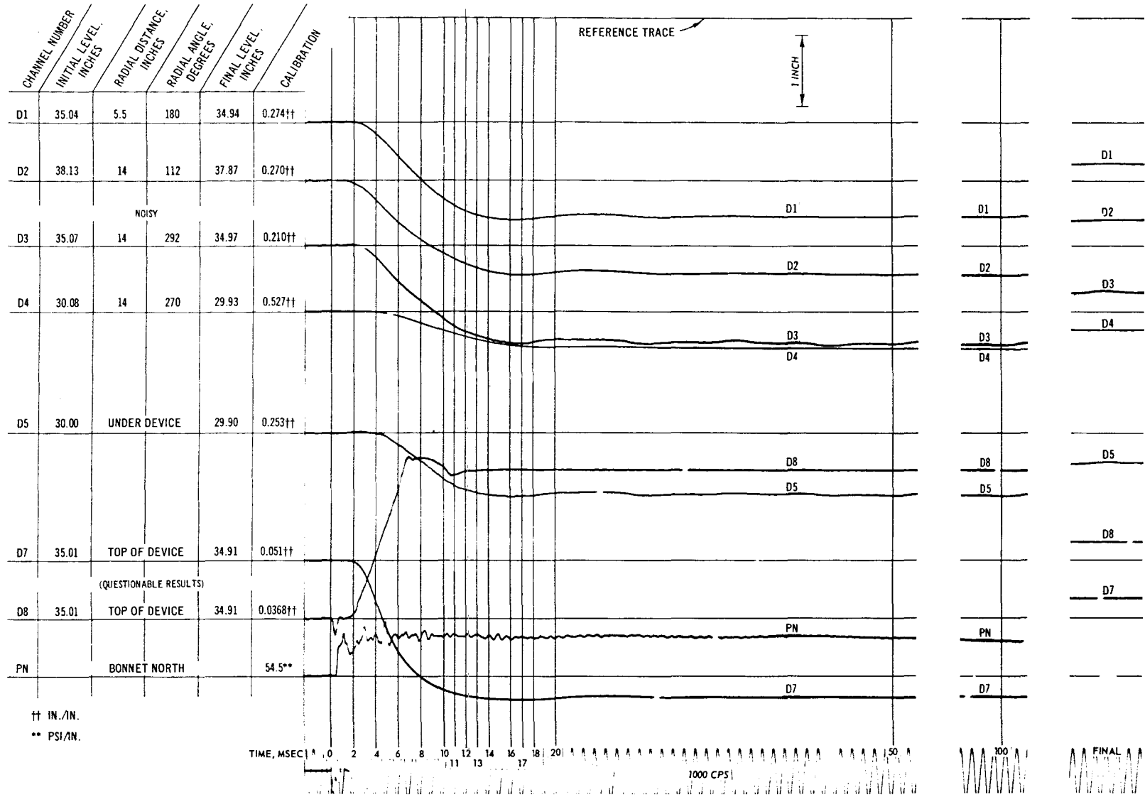
Fig. C-40. Test 20, deflection and pressure record
