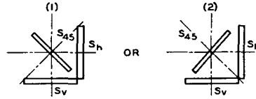
b. PLACEMENT OF SOIL STRESS GAGES
