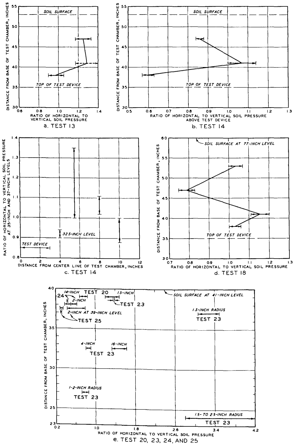
Fig. 68. Variation of horizontal-to-vertical pressure ratio, Tests 13, 14, 18, 20, 23, 24, and 25
