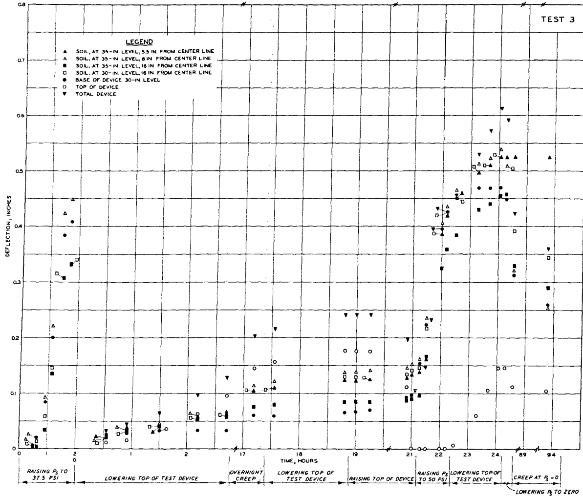
Fig. 36. Soil and structure deflections versus time; Test 3, H/B = 3 , P_S = 37.5 psi
