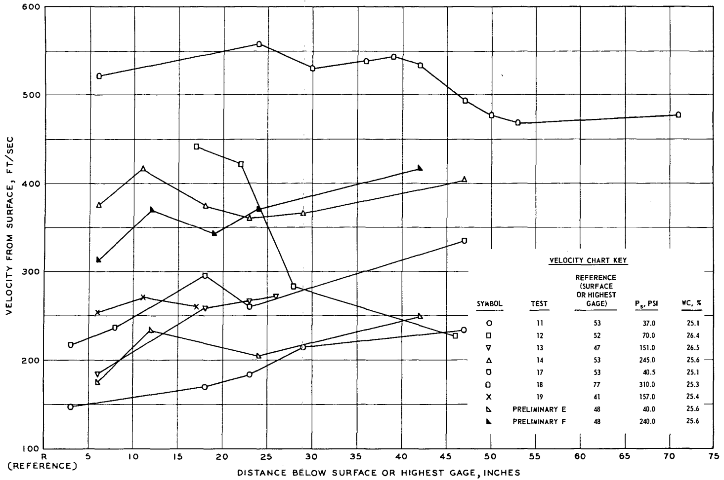
Fig. A-18. Variation of velocity of propagation of first stress peak with surface pressure
