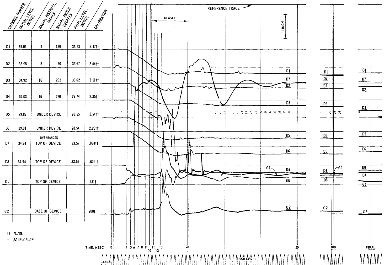
Fig. C-16. Test 14, deflection and strain record
