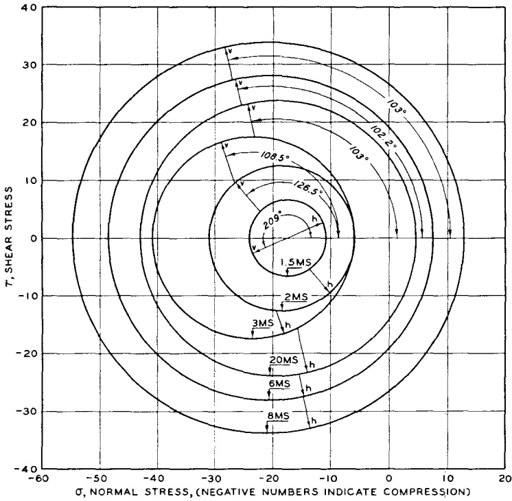
a. MOHR'S CIRCLES OF STRESS, GAGES PLACED AT 2-INCH RADIUS, 38-INCH LEVEL
