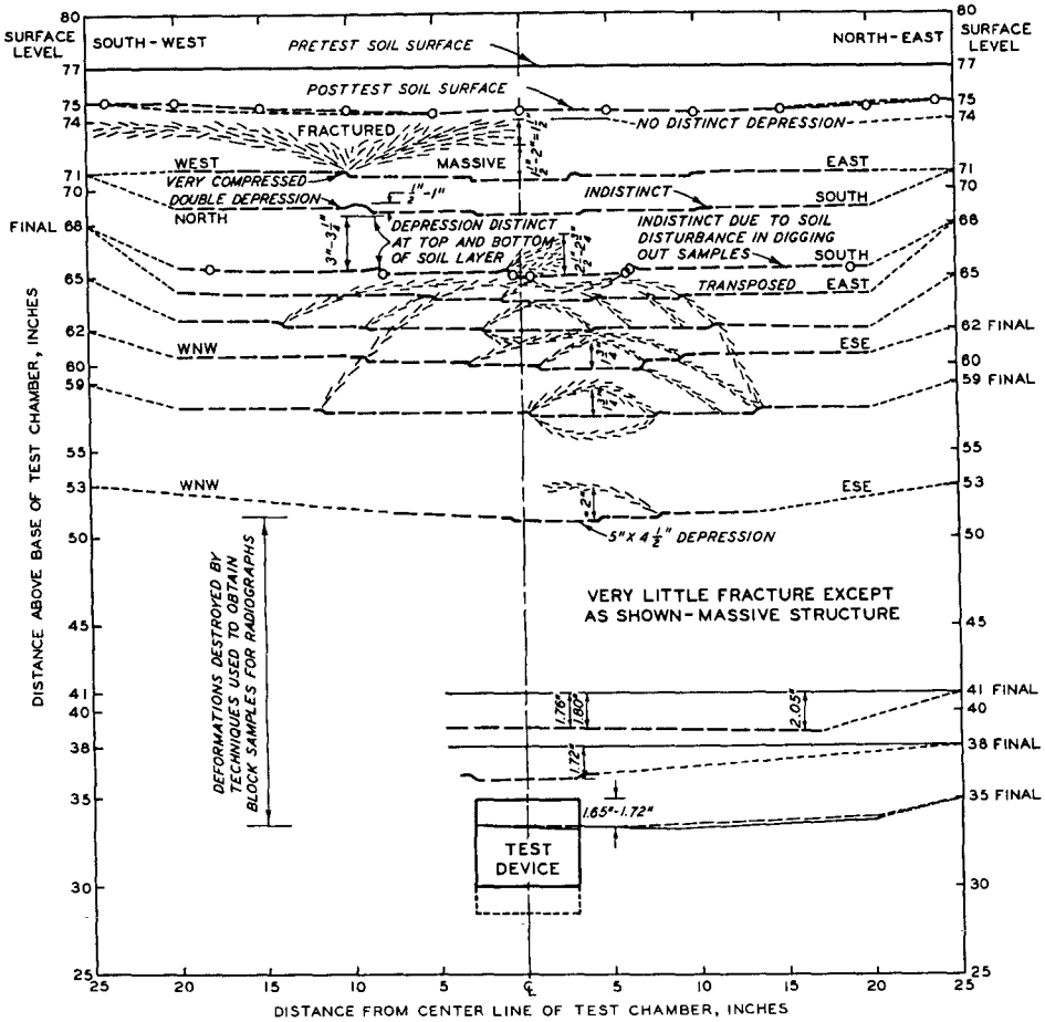
a. CROSS SECTION OF SOIL DEFORMATIONS
