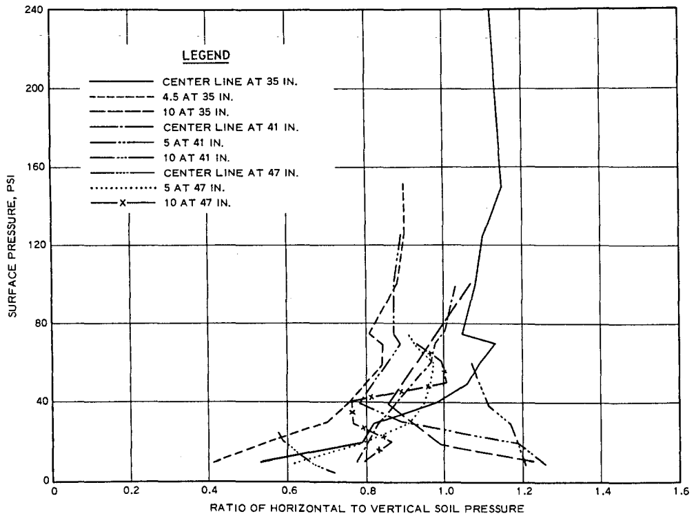
Fig. 32. Variation of horizontal to vertical soil pressure ratio with structural deflection and surface pressure
