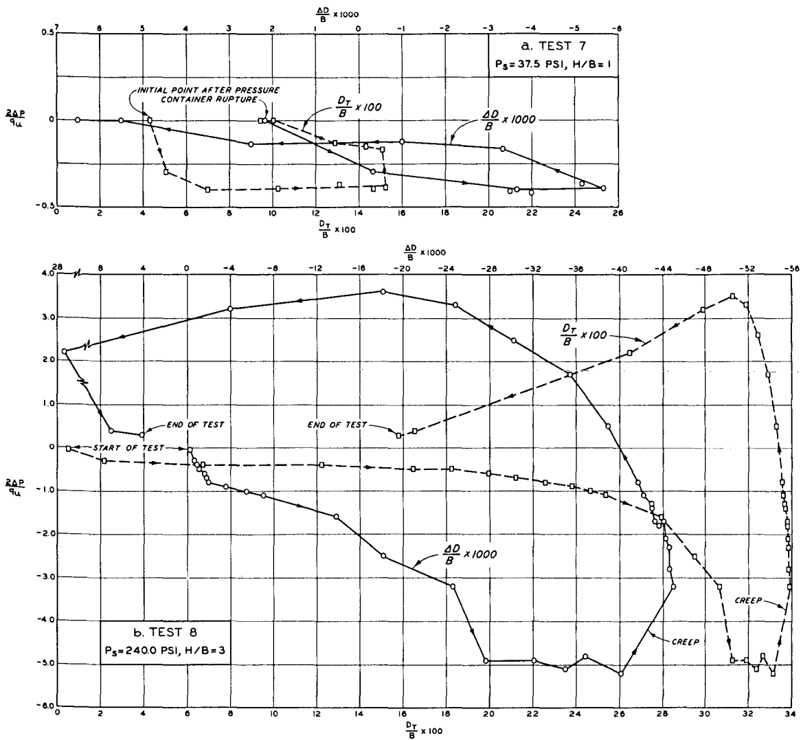
Fig. 25. Dimensionless plot of pressure versus deflection for static Tests 7 and 8
