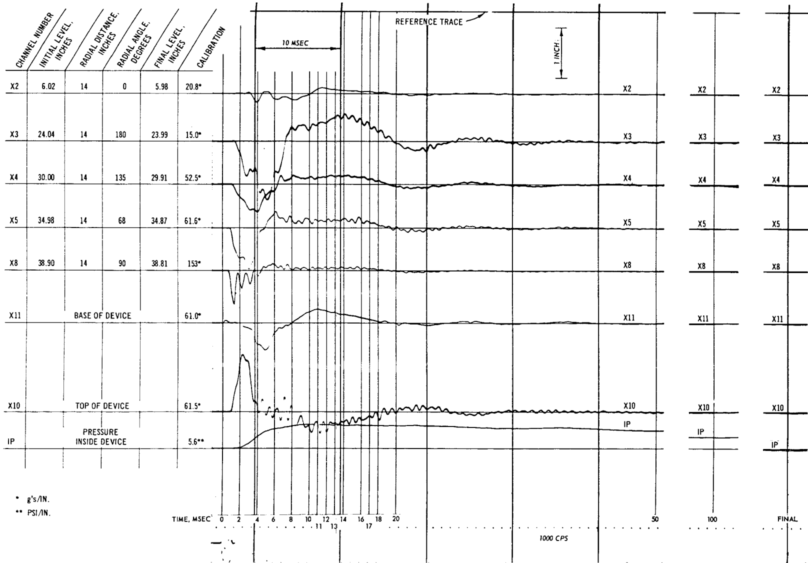
Fig. C-41. Test 20, acceleration and pressure record
