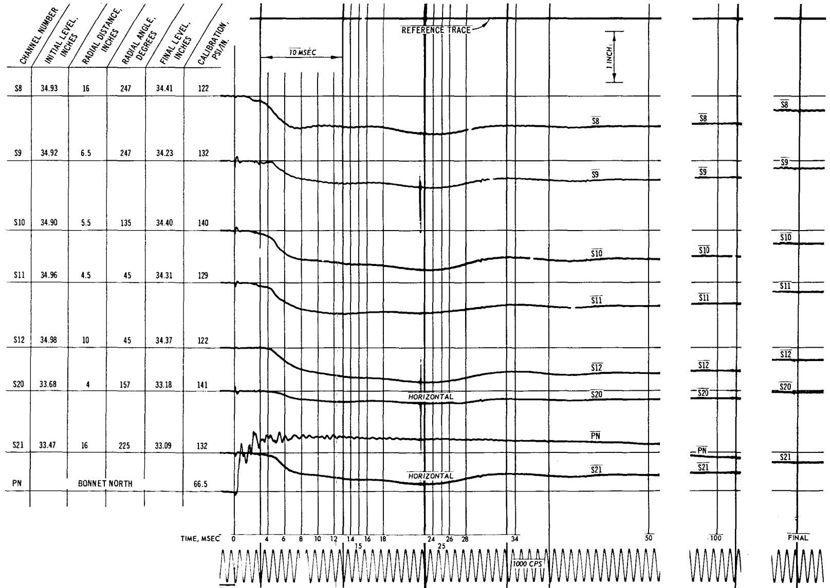
Fig. C-7. Test 12, pressure record (S8-S21)
