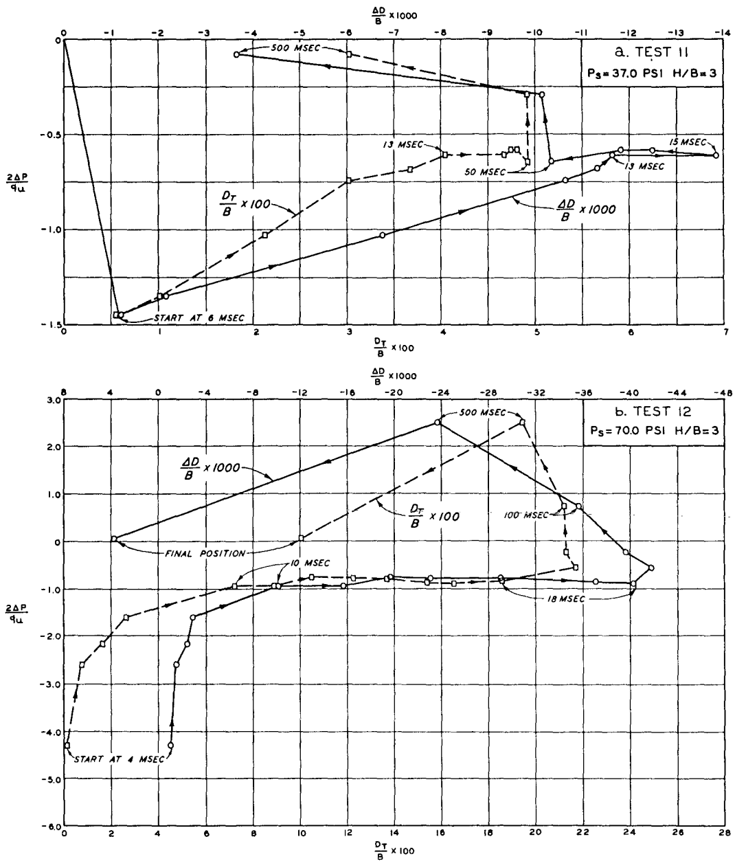
Fig. 51. Dimensionless plot of pressure versus deflection for dynamic Tests 11 and 12
