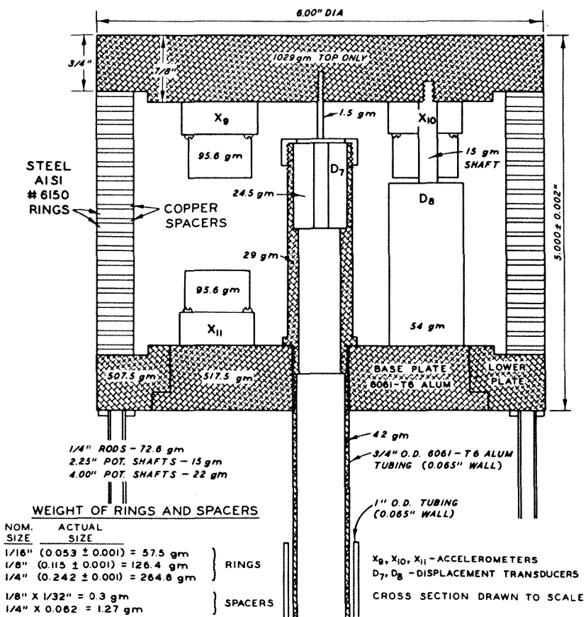
Fig. 12. Spring-ring test device
