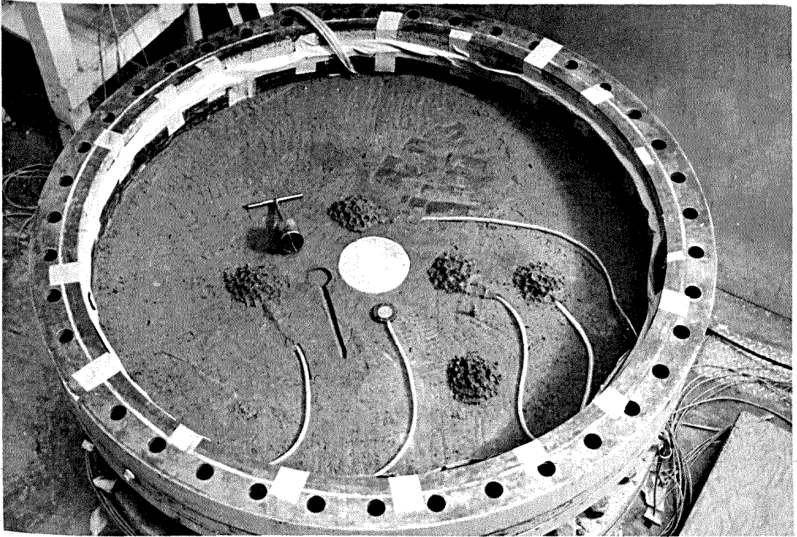
Fig. 16. Soil pressure gage placement at the 35-in. level
