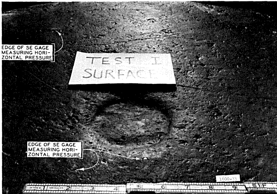
a. Oblique view of soil surface
