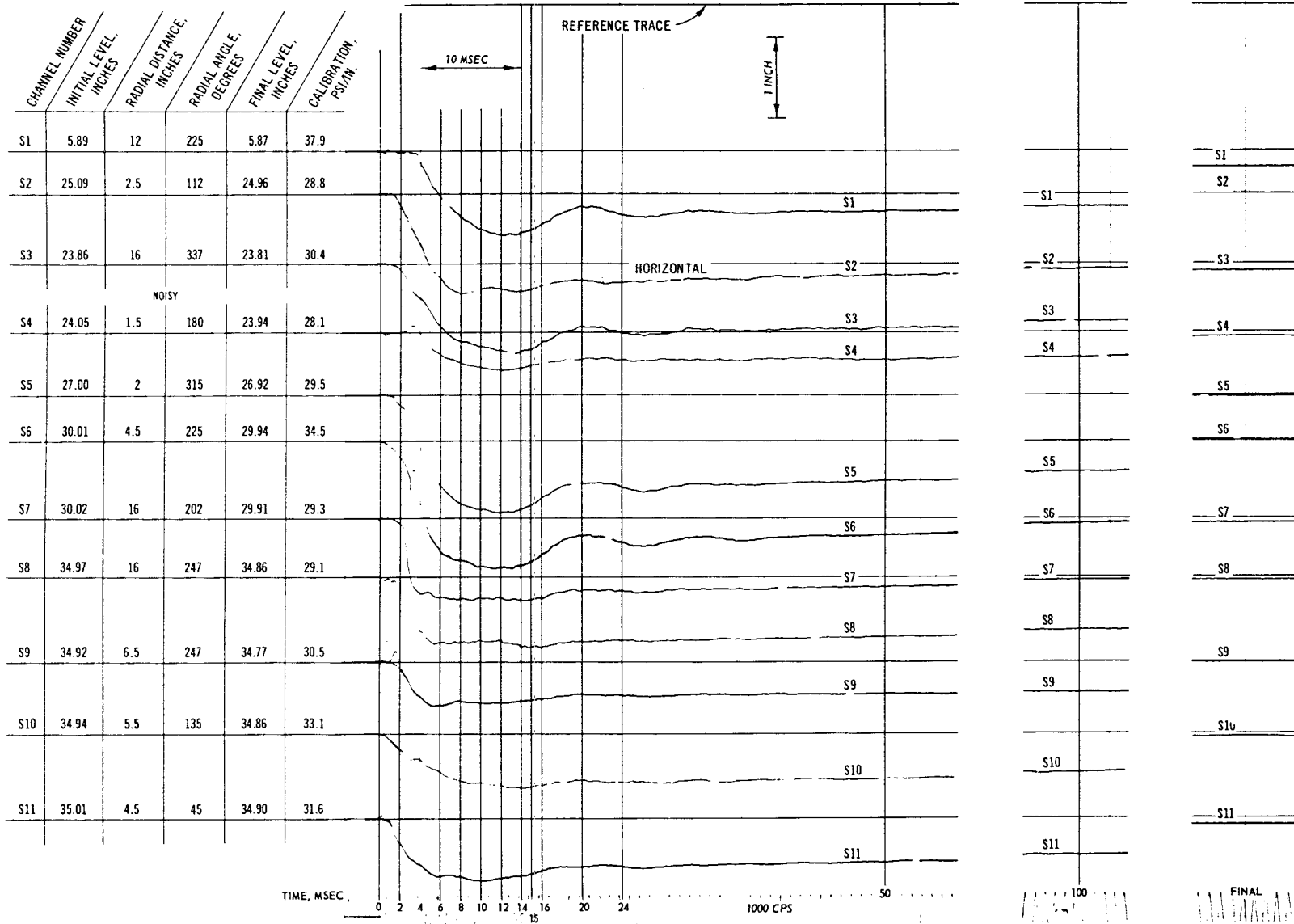
Fig. C-50. Test 23, pressure record (S1-S11)
