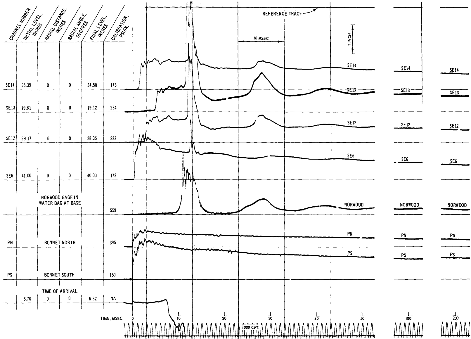
Fig. C-78. Test B, pressure record
