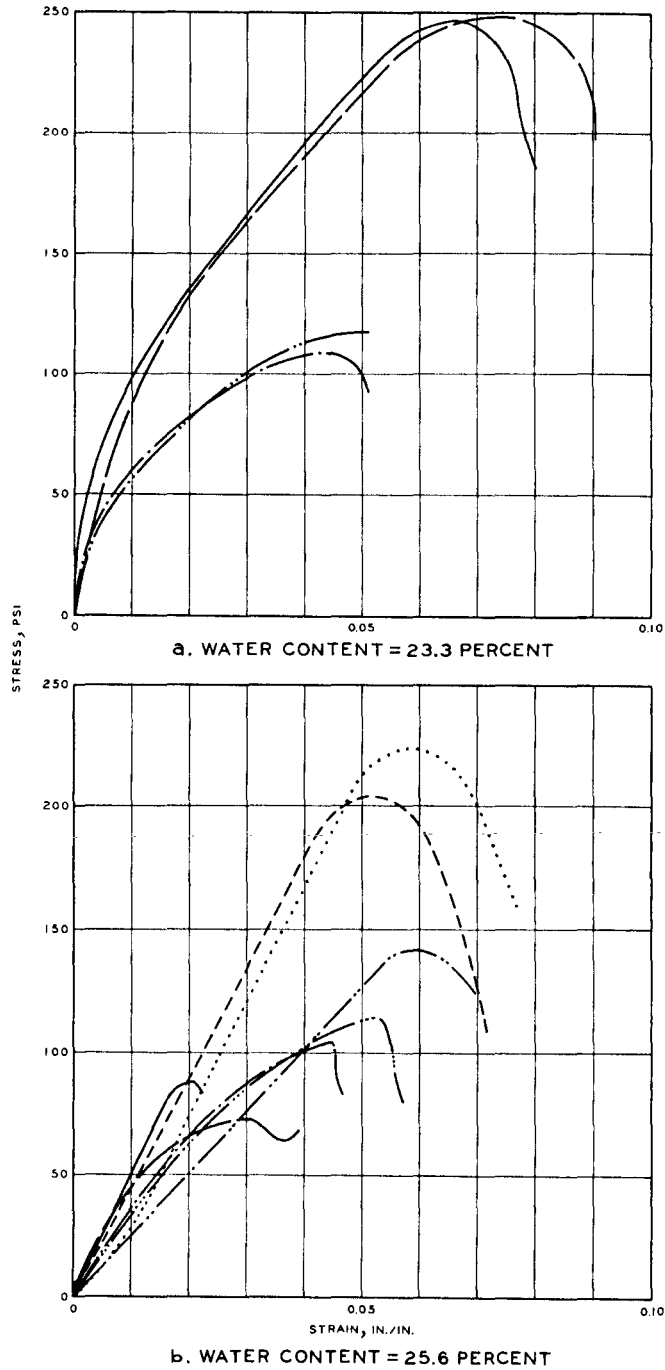
Fig. A-21. Stress-strain curves, buckshot clay, impact loader; water contents, 23.3 and 25.6 percent
