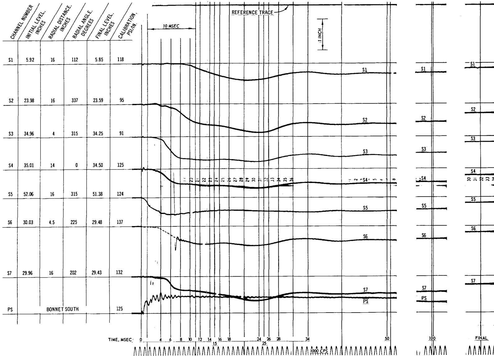
Fig. C-6. Test 12, pressure record (S1-S6)
