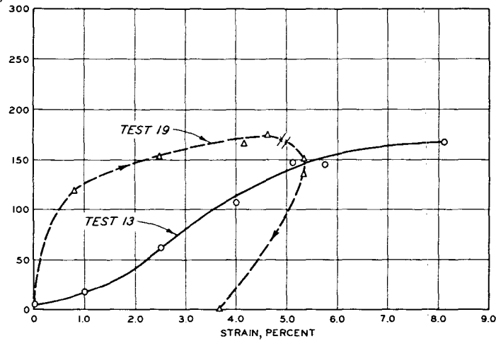
b. HIGH PRESSURE TESTS
