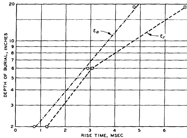
d. VARIATION OF SOIL PRESSURE RISE TIME WITH DEPTH, P_s \approx 37 PSI
