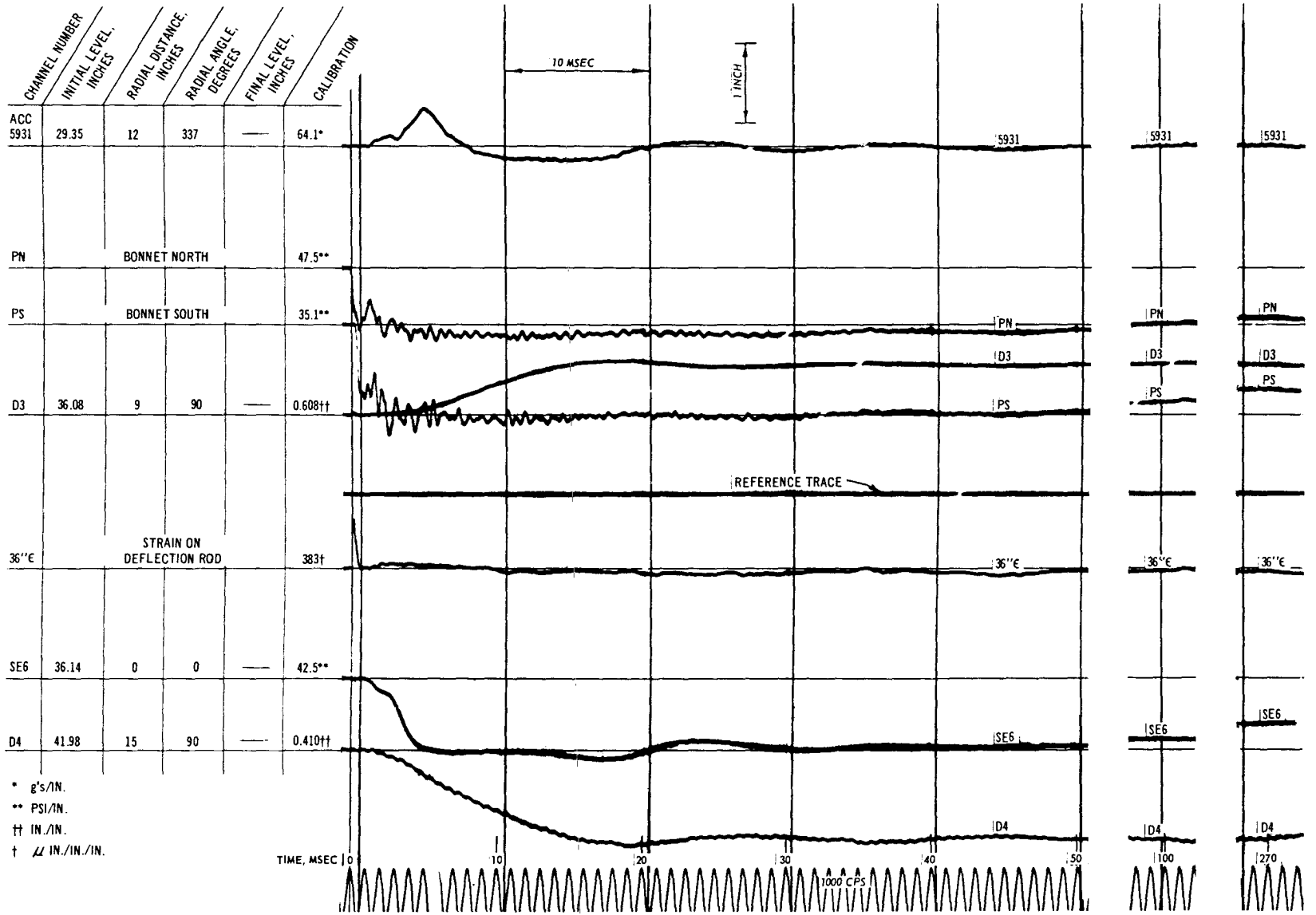
Fig. C-85. Test E, pressure, acceleration, deflection, and strain record
