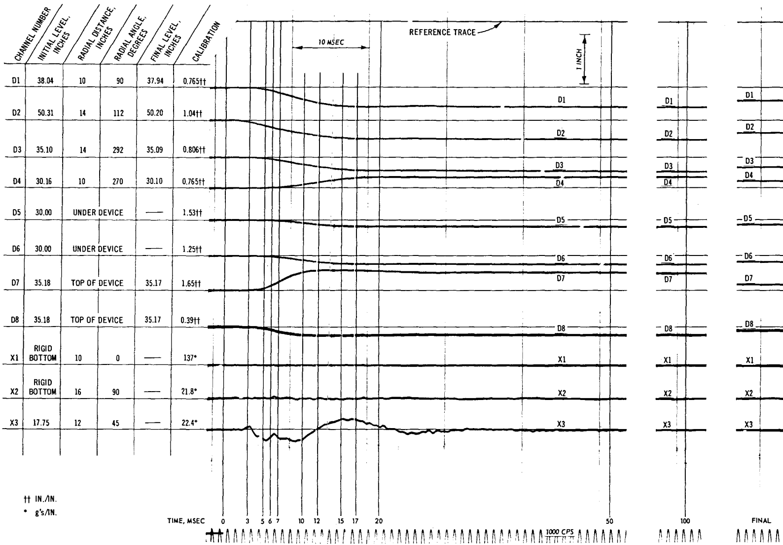
Fig. C-4. Test 11, deflection and acceleration (X1-X3) record
