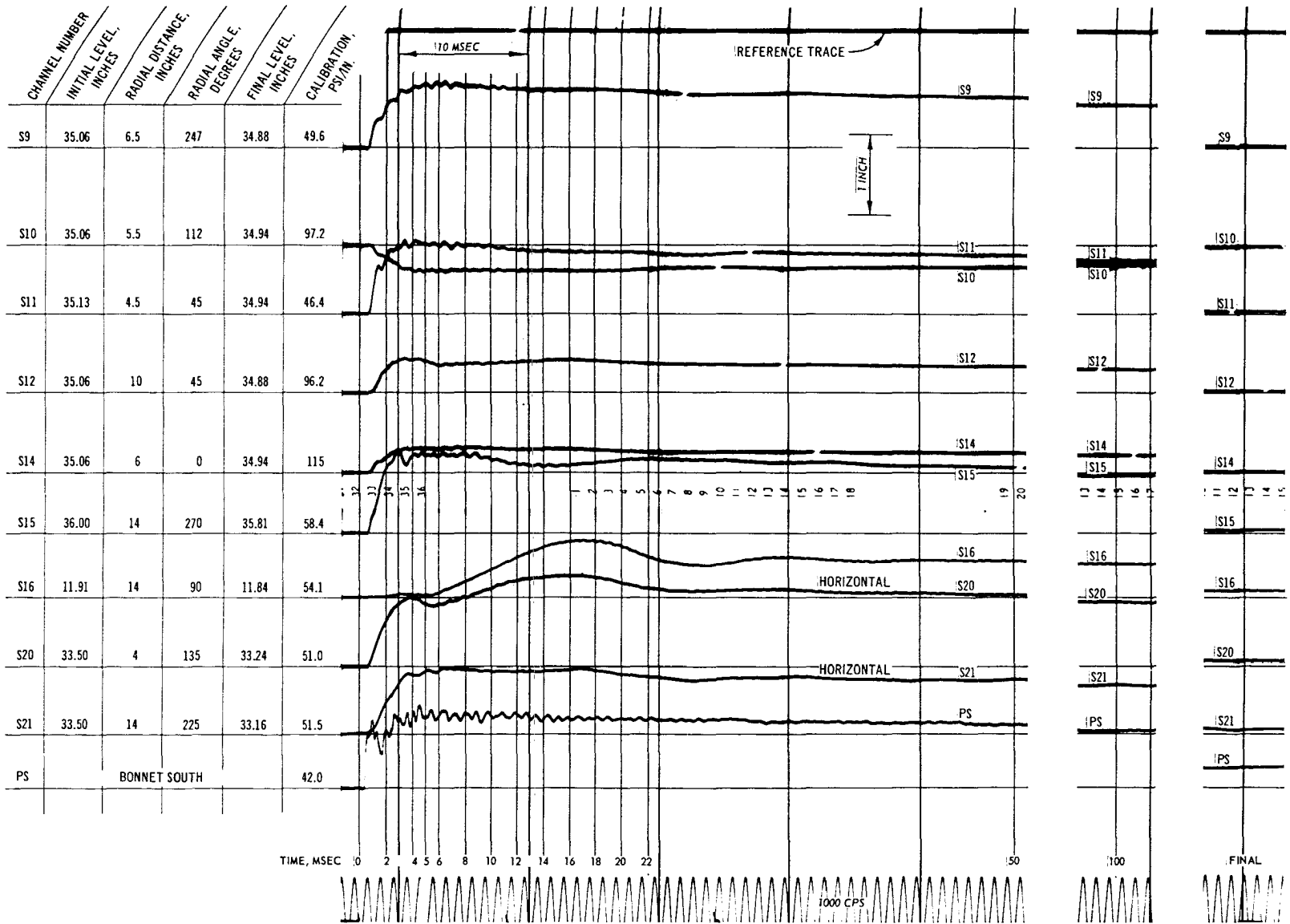
Fig. C-19. Test 15, pressure record (S9-S21)
