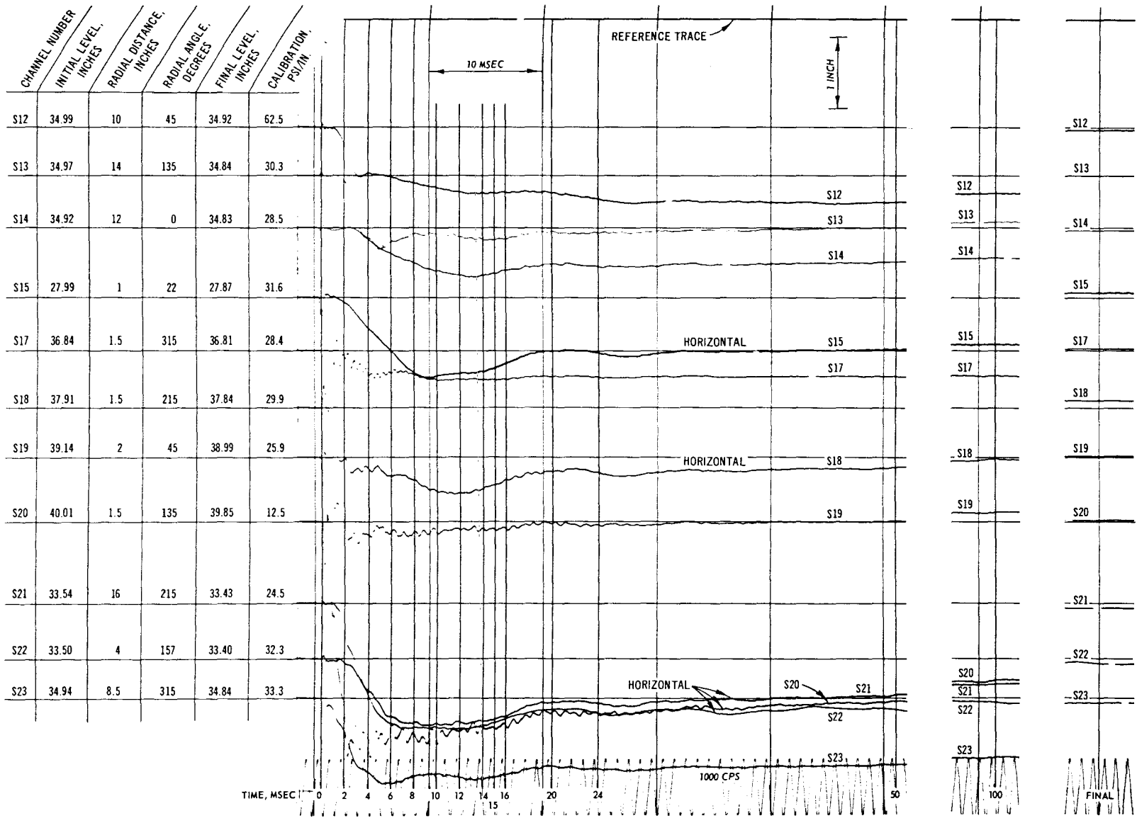
Fig. C-51. Test 23, pressure record (S12-S23)
