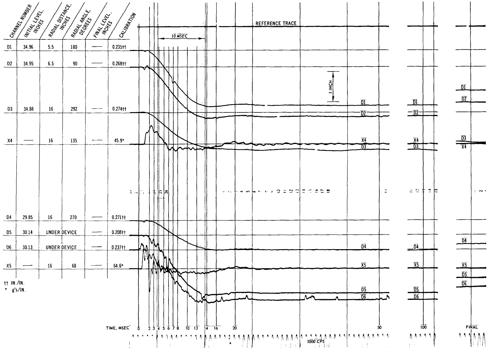
Fig. C-68. Test 27B, deflection and acceleration record
