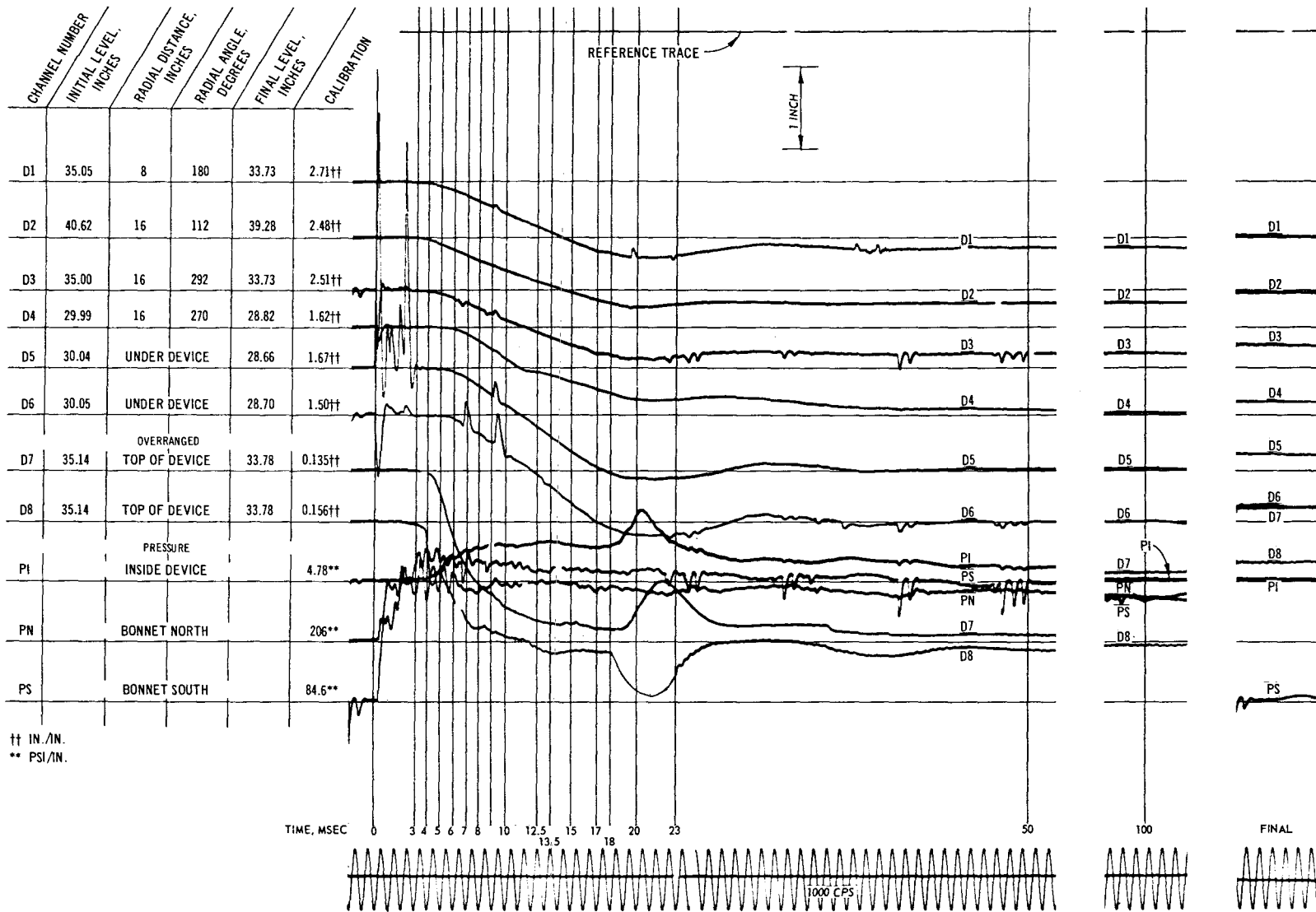
Fig. C-12. Test 13, deflection and pressure record
