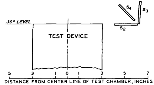
c. TEST 8—CONFIGURATION OF GAGE ARRAY WITH RESPECT TO TEST DEVICE
