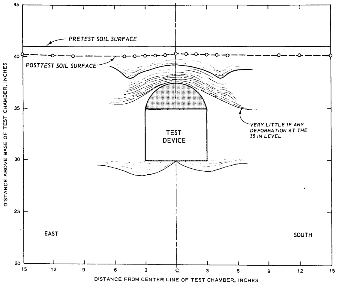
Fig. 90. Hypothetical soil deformations under passive arching conditions
