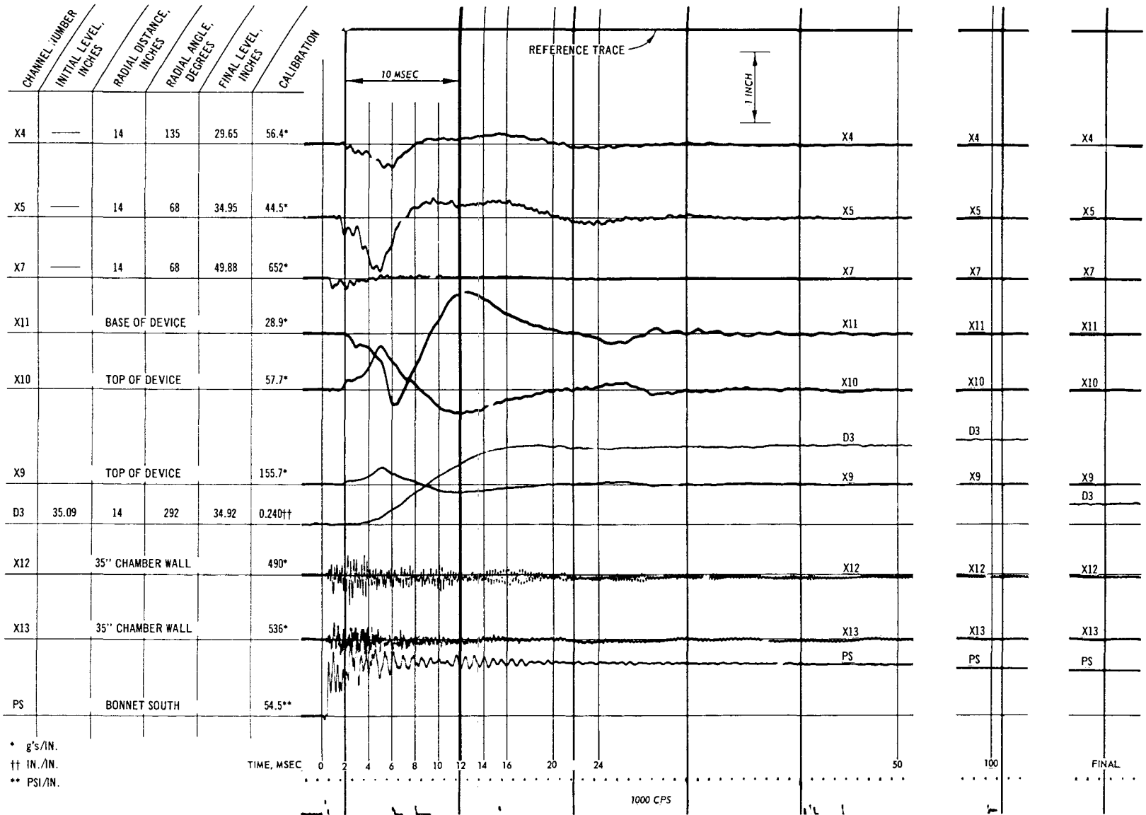
Fig. C-29. Test 17, acceleration, deflection, and pressure record
