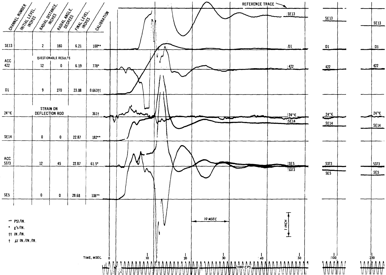
Fig. C-84. Test D, pressure, acceleration, deflection, and strain record
