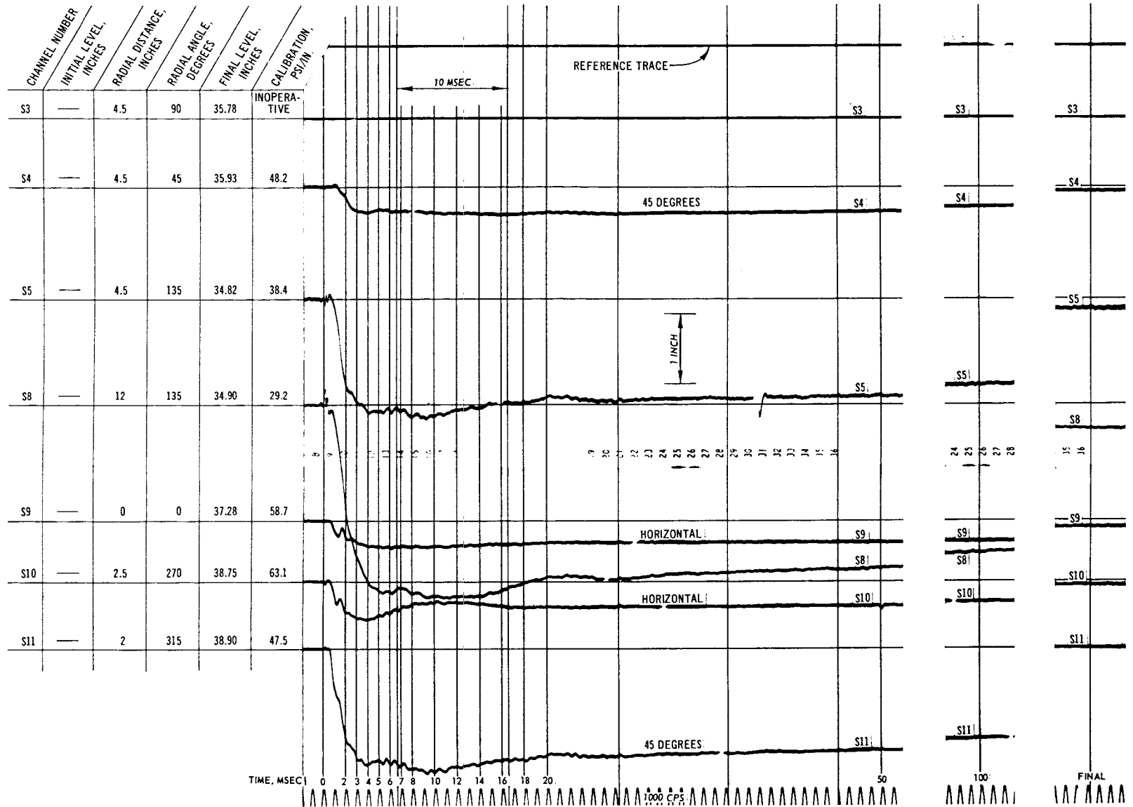
Fig. C-58. Test 25, pressure record
