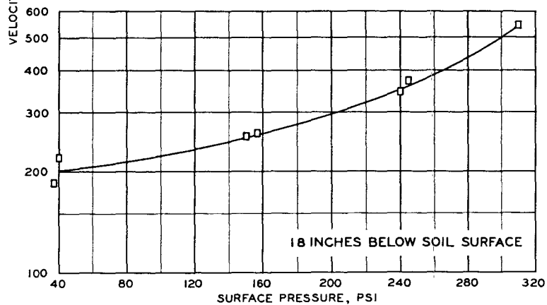
a. STRESS WAVE VELOCITY VERSUS SURFACE PRESSURE
