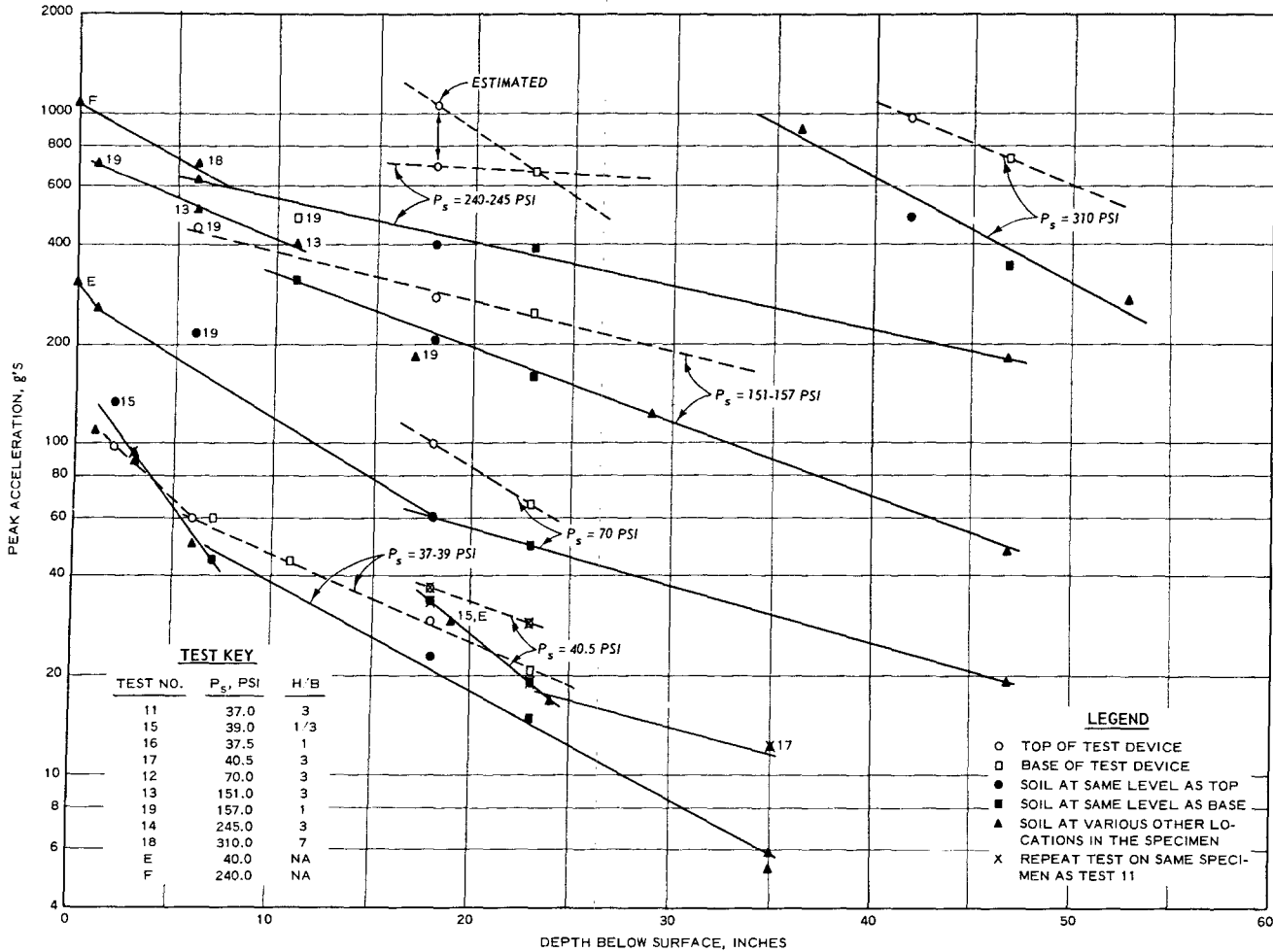
Fig. 76. Variation of soil and structure acceleration with changes in surface pressure and depth of burial at a relatively constant structural stiffness
