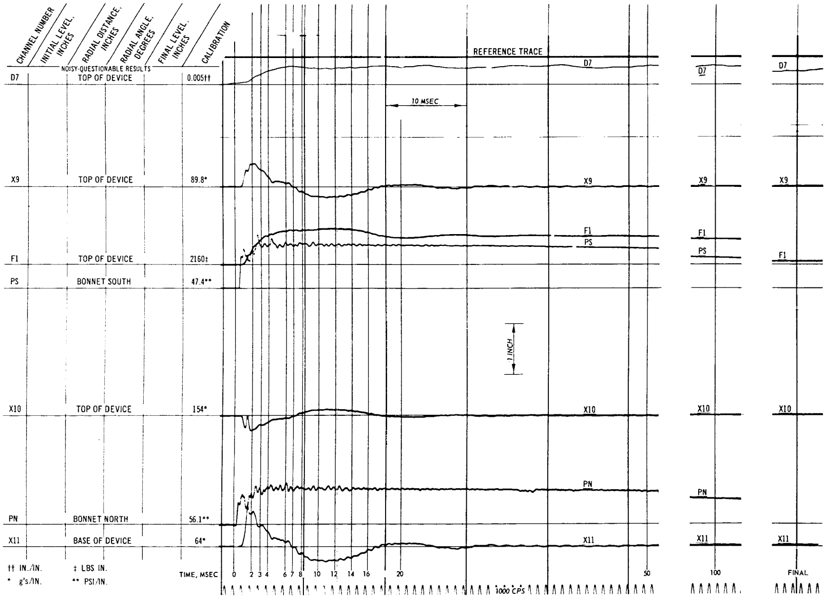
Fig. C-69. Test 27B, deflection, acceleration, pressure, and force record
