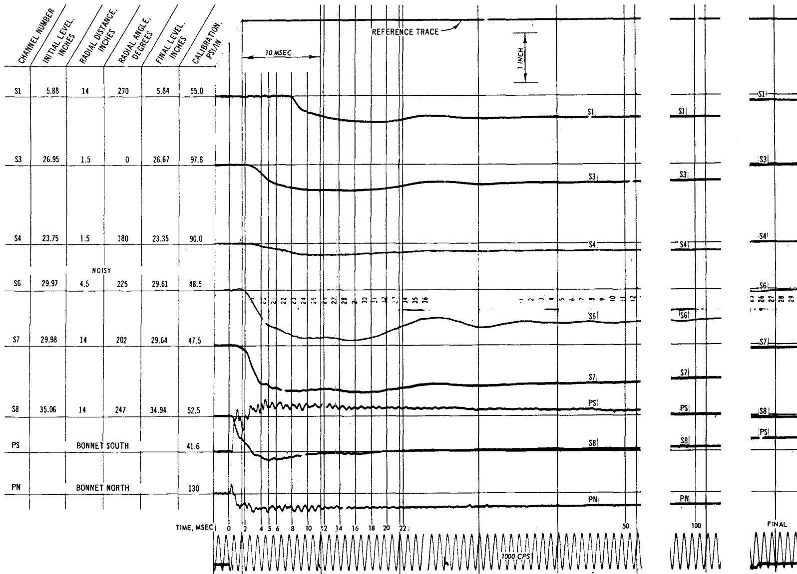
Fig. C-18. Test 15, pressure record (S1-S8)
