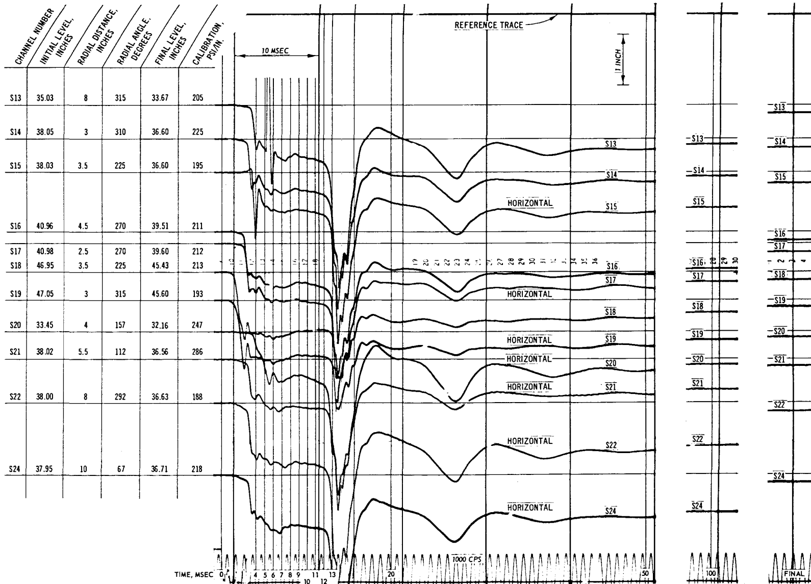
Fig. C-15. Test 14, pressure record (S13-S24)
