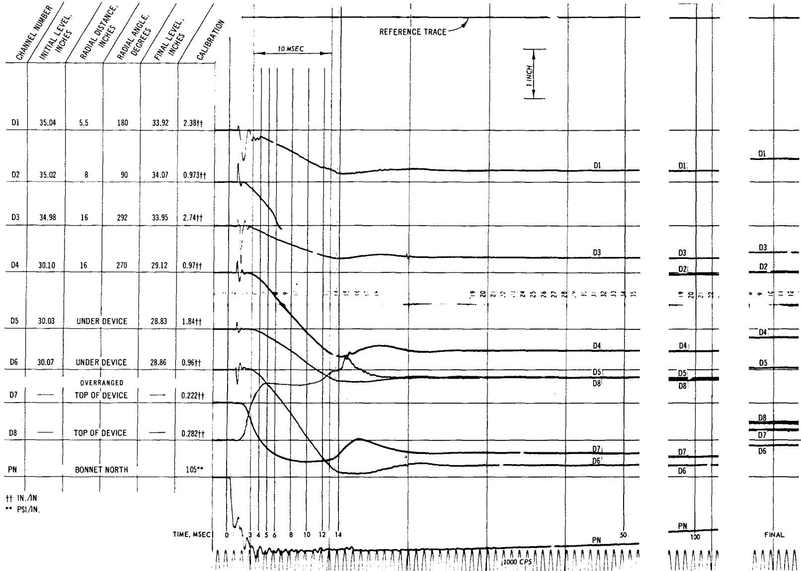
Fig. C-36. Test 19, deflection and pressure record
