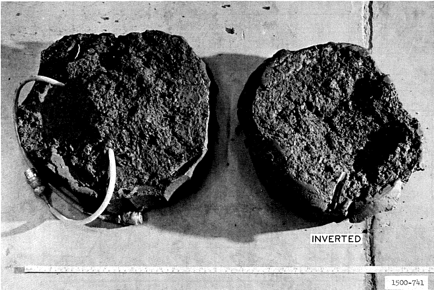
Fig. 91. Soil deformation pattern resulting from a 6-inch plate bearing test; H/B = 3
