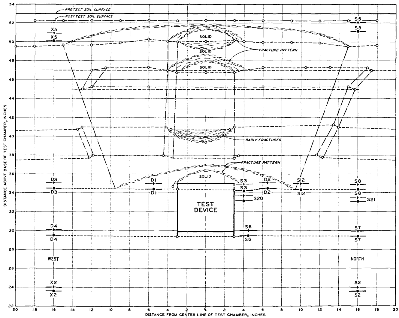
Fig. 79. Cross section of soil deformations, Test 12; H/B = 3 , P_S = 70 psi
