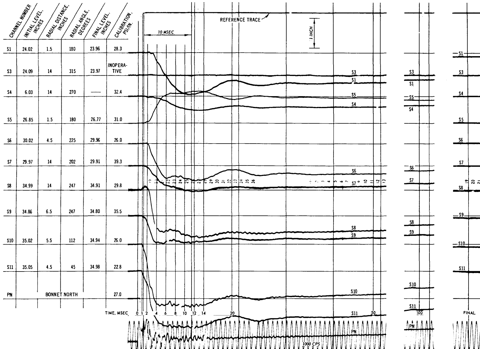
Fig. C-46. Test 22, pressure record (S1-S11)
