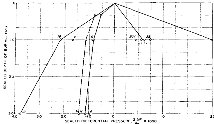
c. VARIATION OF SCALED DIFFERENTIAL PRESSURE WITH DEPTH OF BURIAL AT SCALED DIFFERENTIAL DEFLECTIONS OF \Delta D/B \times 1000 = -50 AND \pm 3.7
