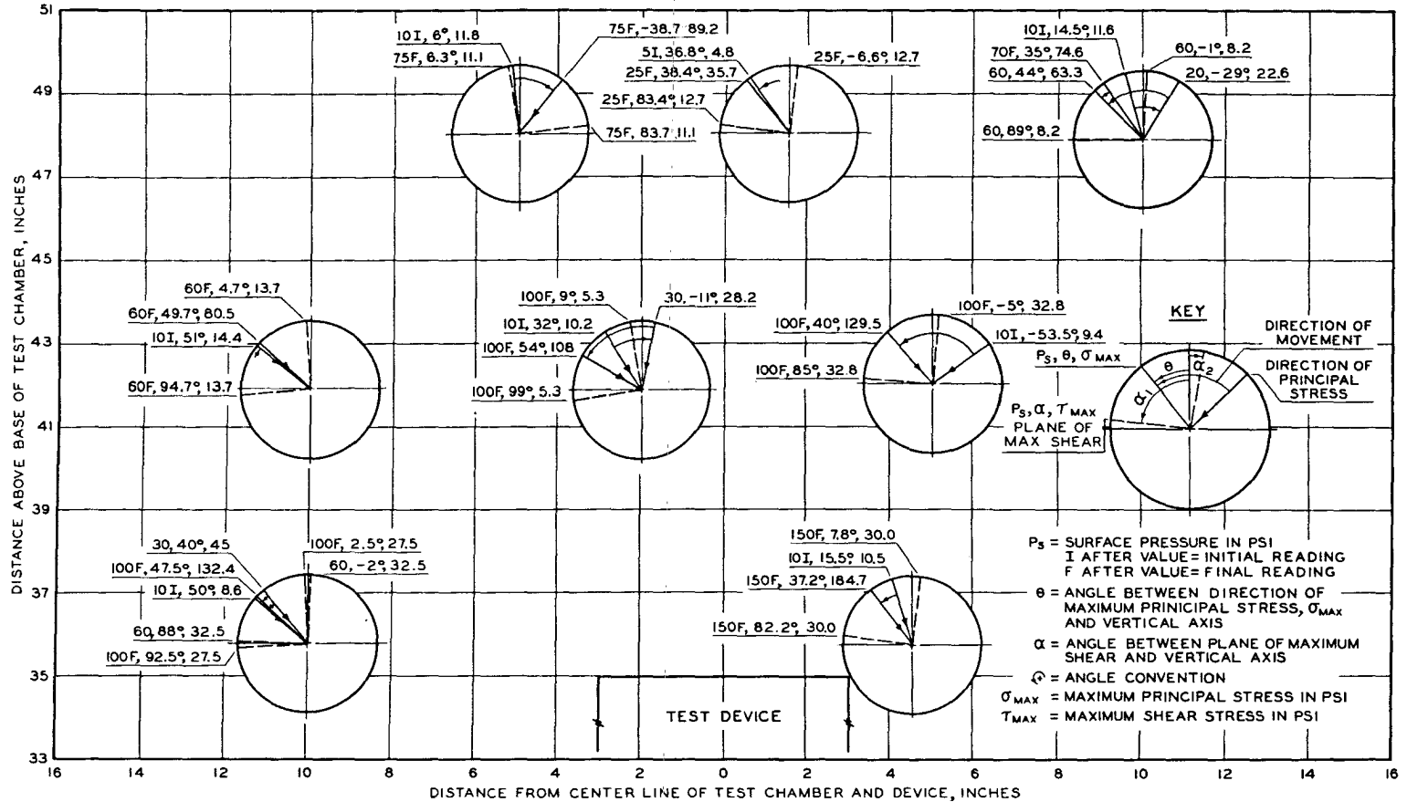
Fig. 34. Directions of principal stresses and location of planes of maximum shear, Test 8
