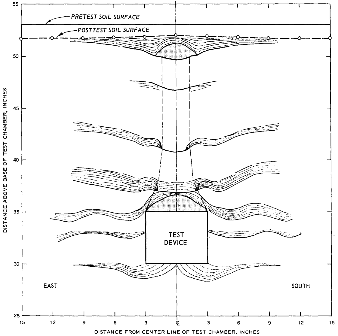
Fig. 89. Composite soil deformation profile under active arching conditions
