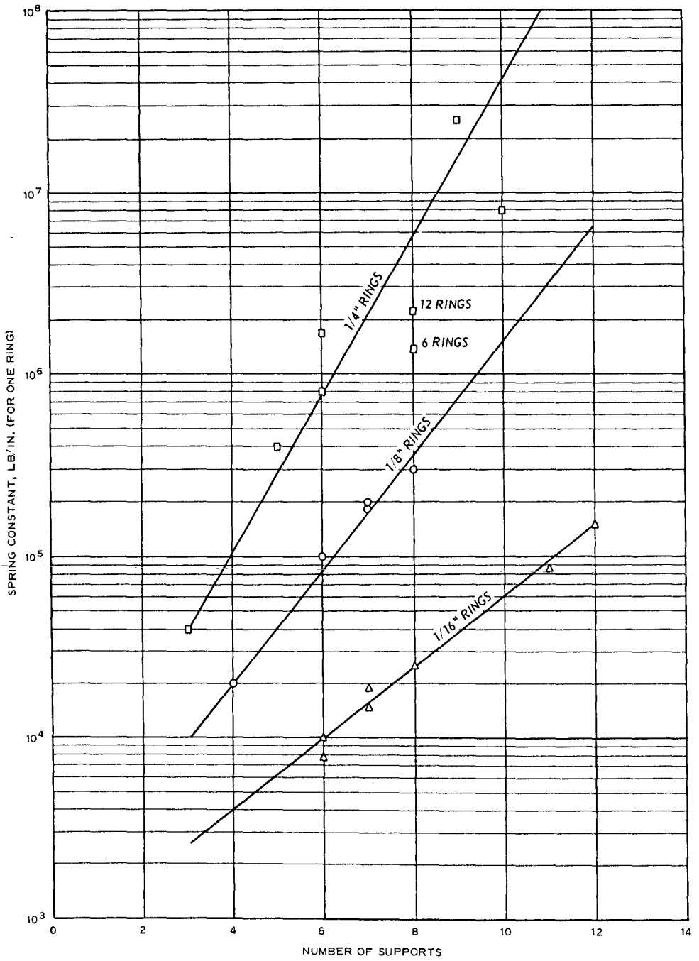
Fig. B-3. Spring constants of individual spring ring
