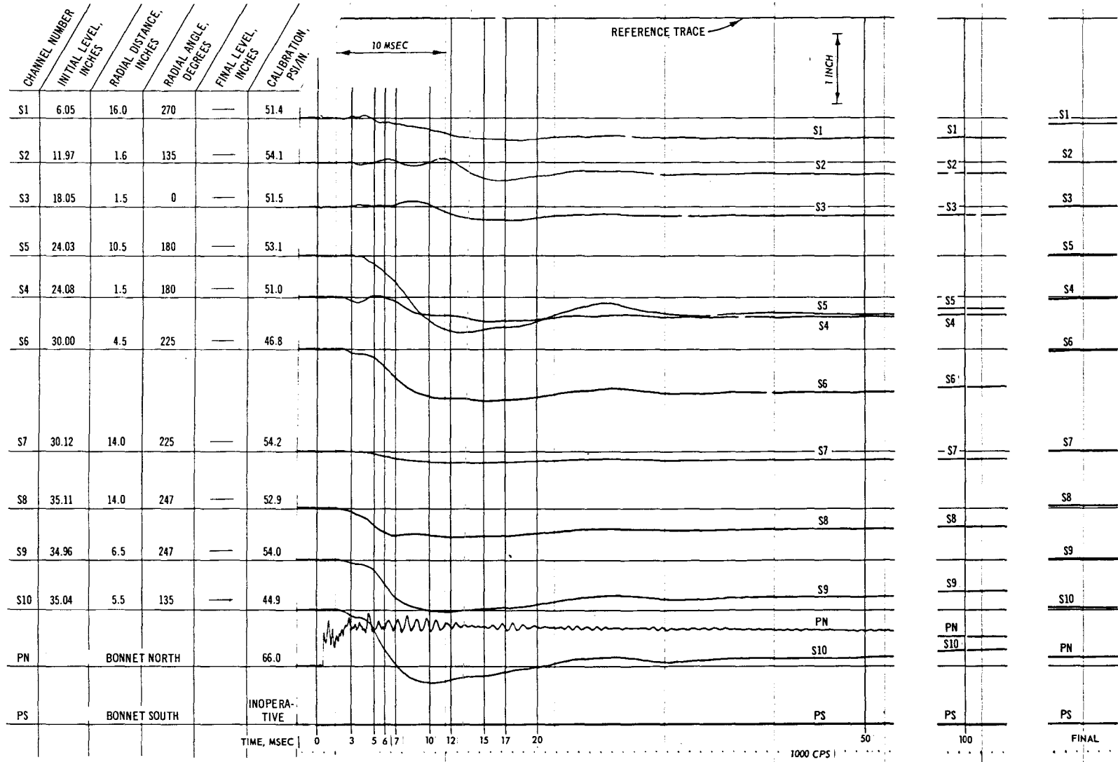
Fig. C-2. Test 11, pressure record (channels S1-S10)
