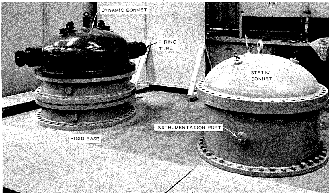
Fig. 7. Small Blast Load Generator facilities (SBLG)
