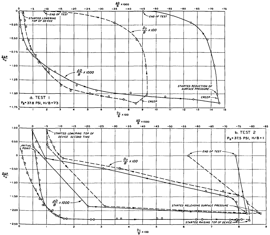
Fig. 21. Dimensionless plot of pressure versus deflection for static Tests 1 and 2
