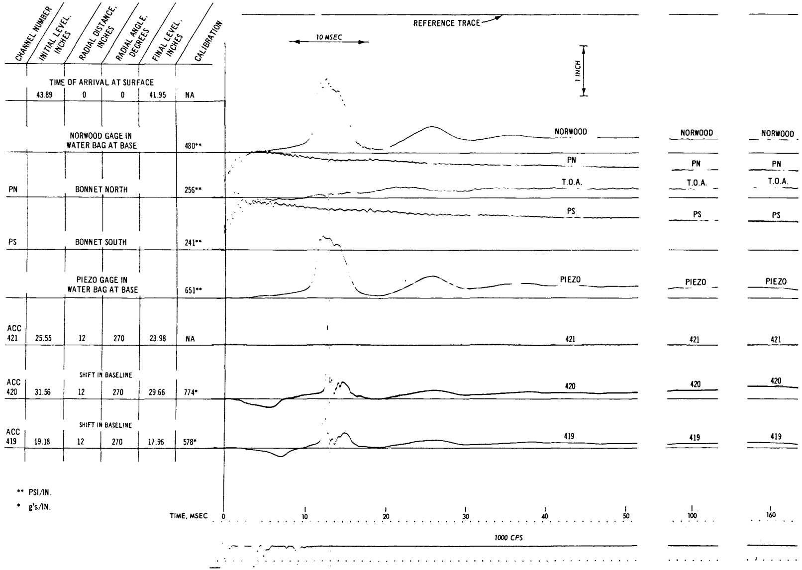
Fig. C-77. Test A, pressure and acceleration record
