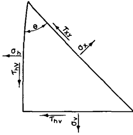
a. STRESS COMPONENTS ACTING ON FACES OF A SMALL WEDGE CUT FROM A BODY WHICH IS IN A STATE OF PLANE STRESS
