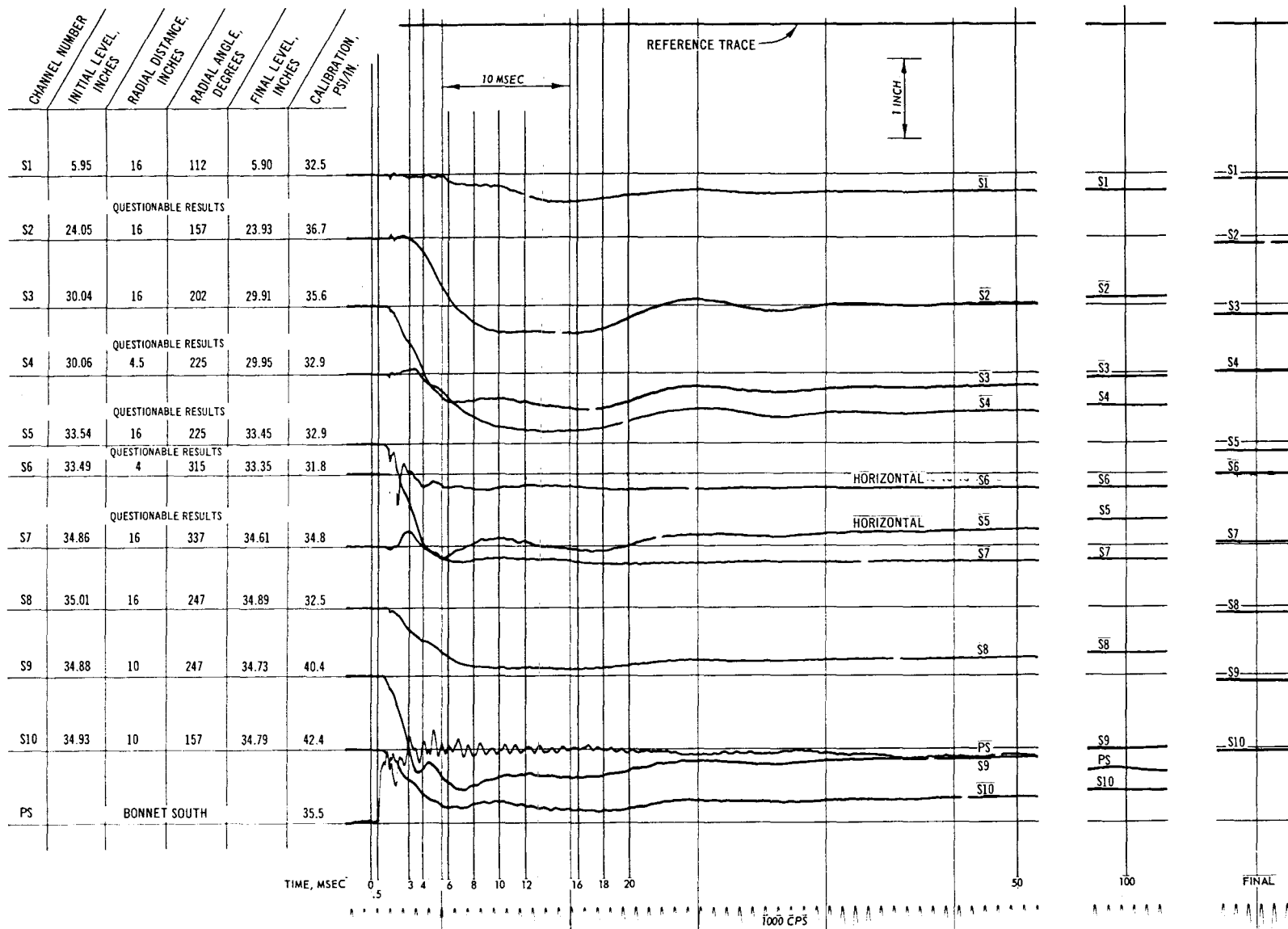
Fig. C-62. Test 26, pressure record (S1-S10)
