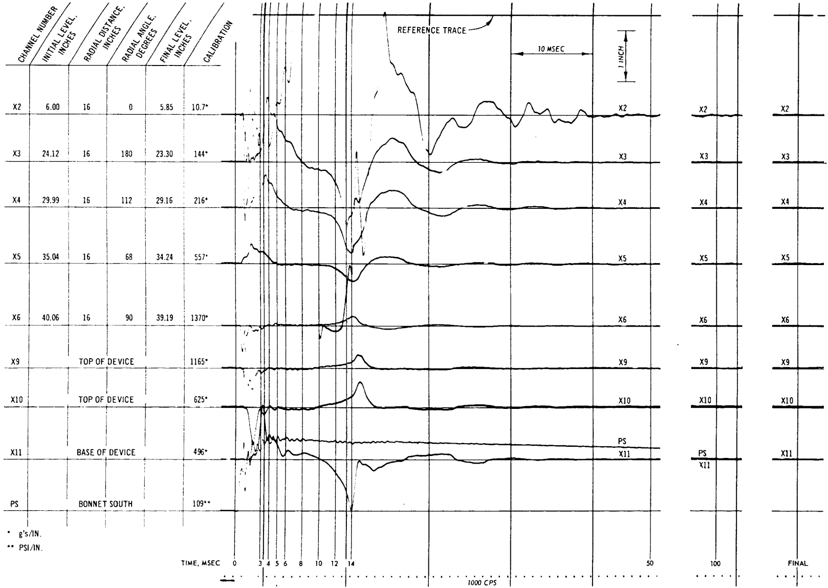
Fig. C-37. Test 19, acceleration and pressure record
