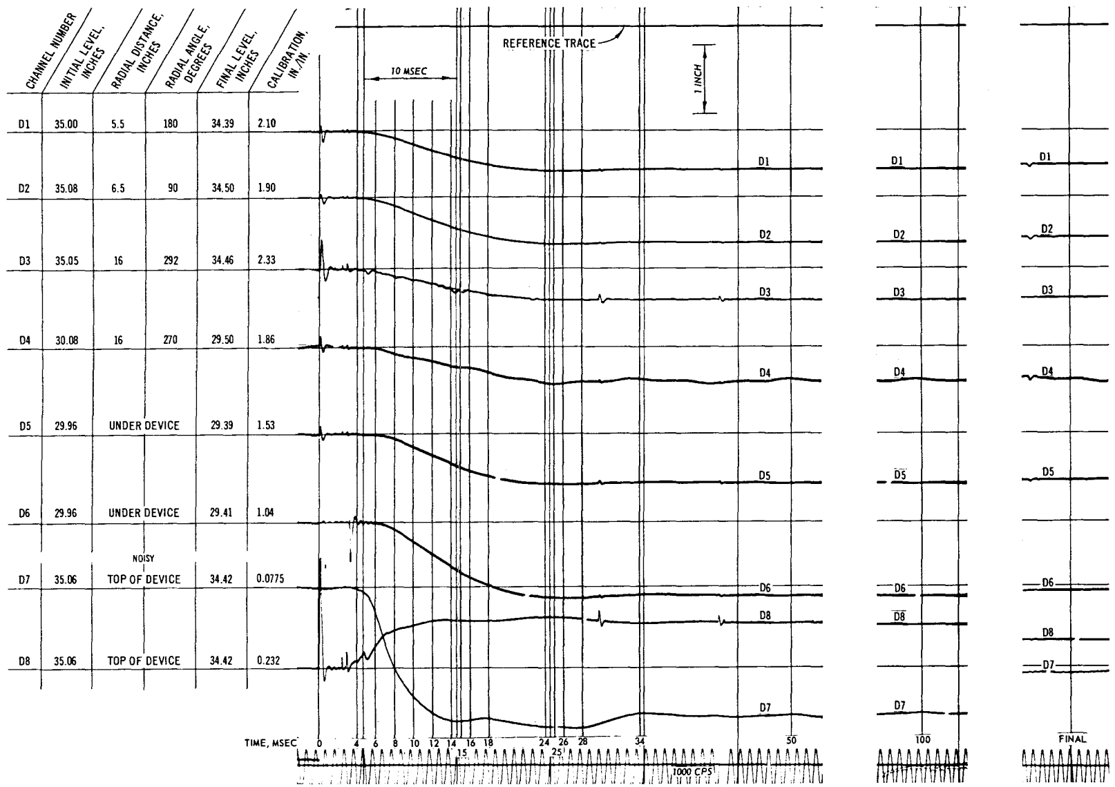
Fig. C-8. Test 12, deflection record
