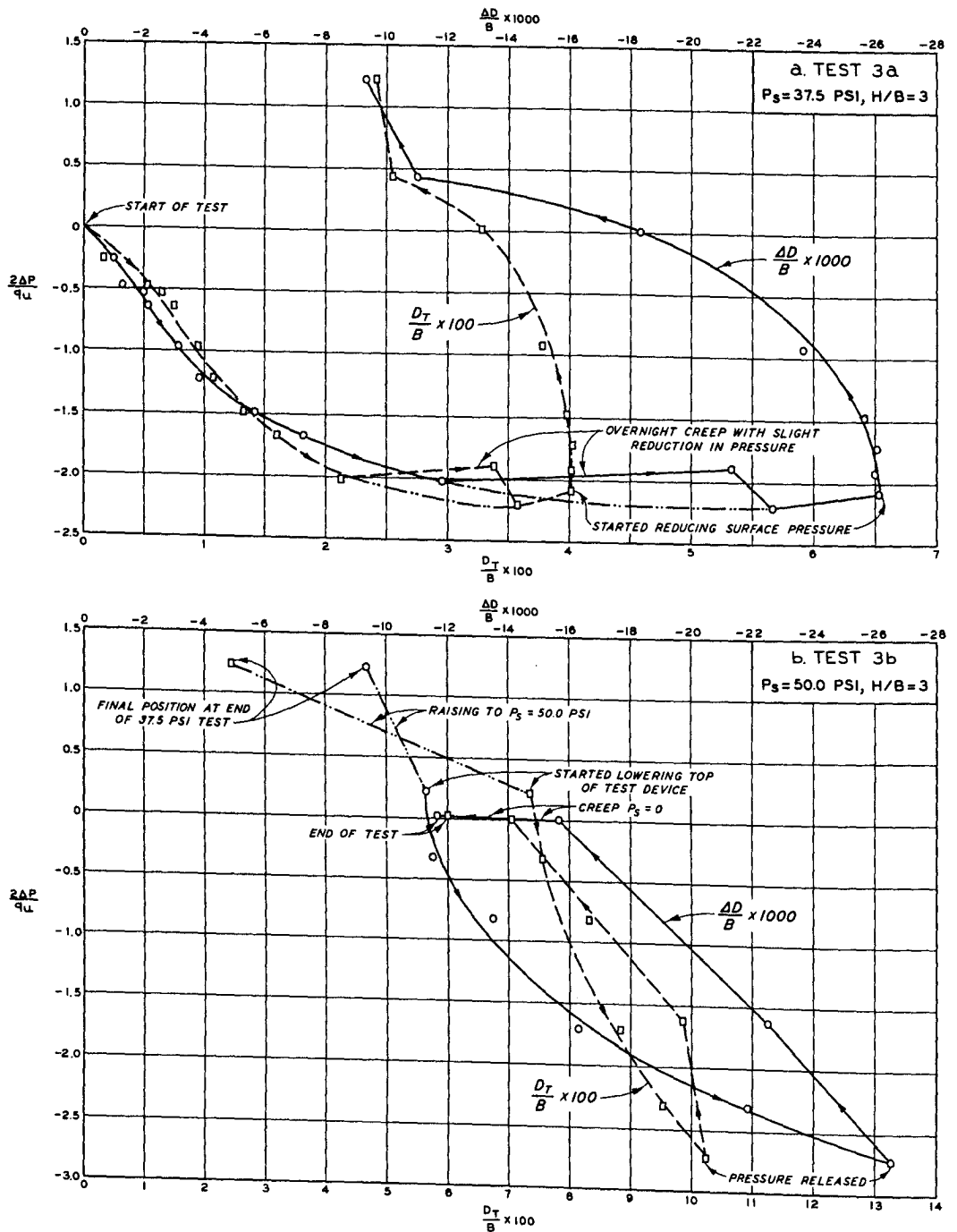
Fig. 22. Dimensionless plot of pressure versus deflection for static Test 3
