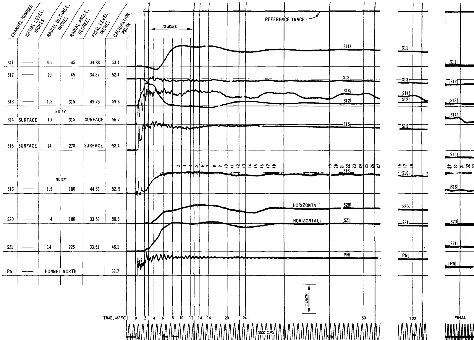
Fig. C-27. Test 17, pressure record (S11-S21)
