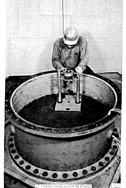
g. TAKING VANE-SHEAR READINGS
