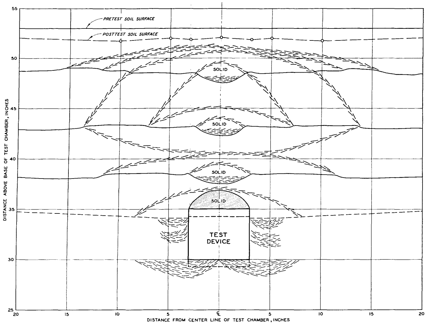
Fig. 96. Composite soil deformation profile under active arching conditions
