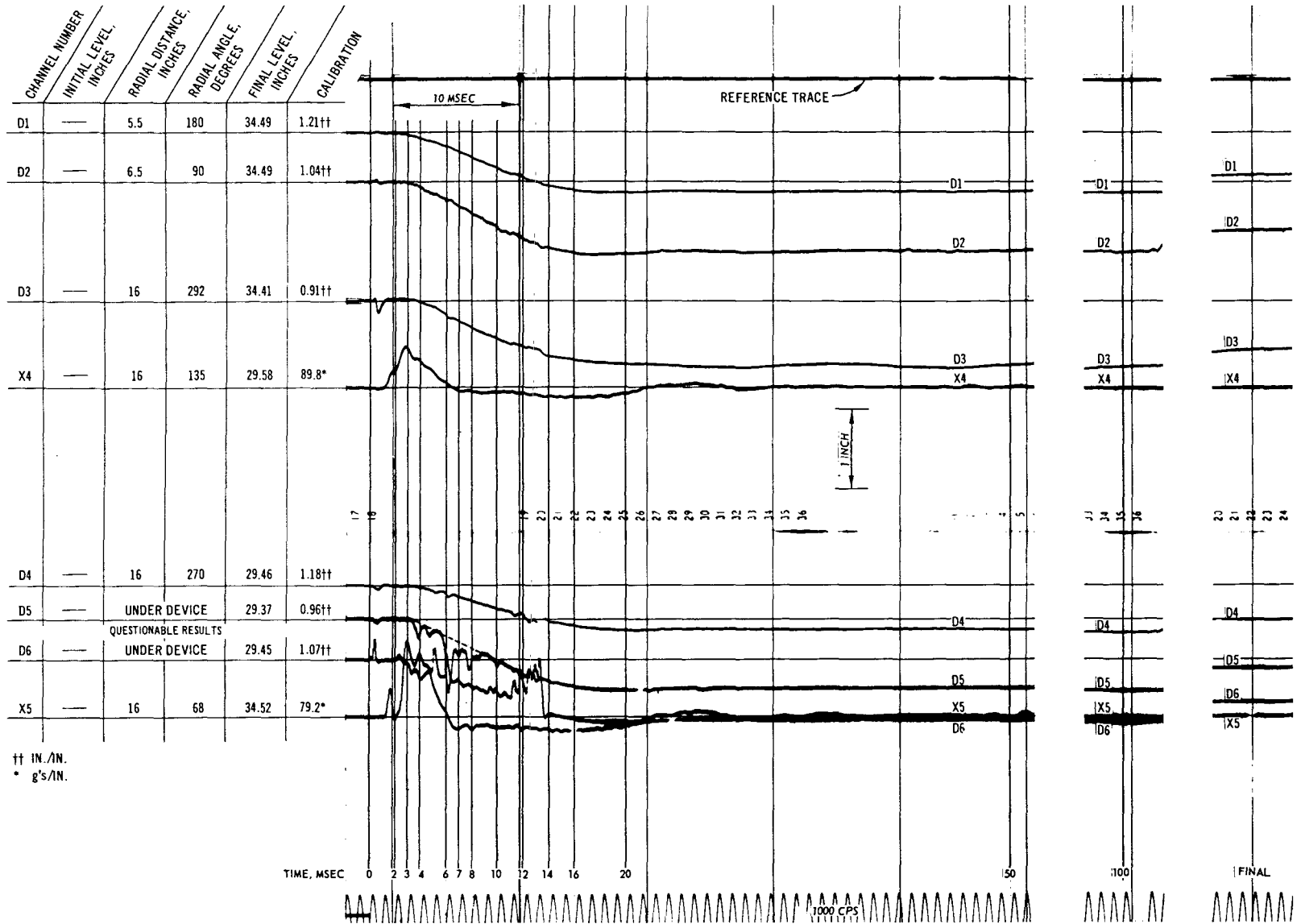
Fig. C-70. Test 27C, deflection and acceleration record
