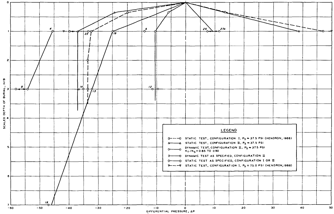
Fig. 97. Differential pressure versus scaled depth of burial, active and passive arching; WC \approx 26\% , B = 6 inches
