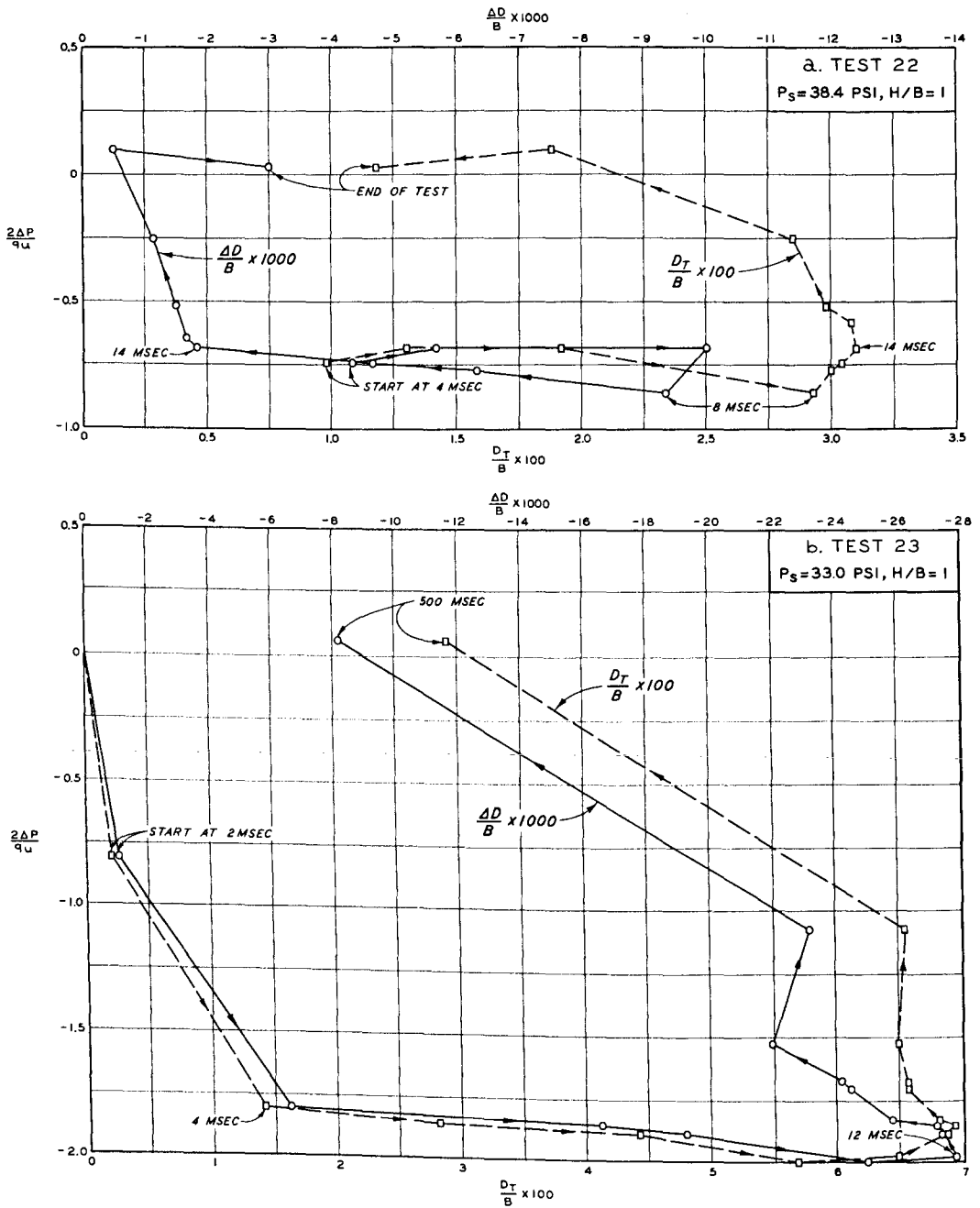
Fig. 56. Dimensionless plot of pressure versus deflection for dynamic Tests 22 and 23
