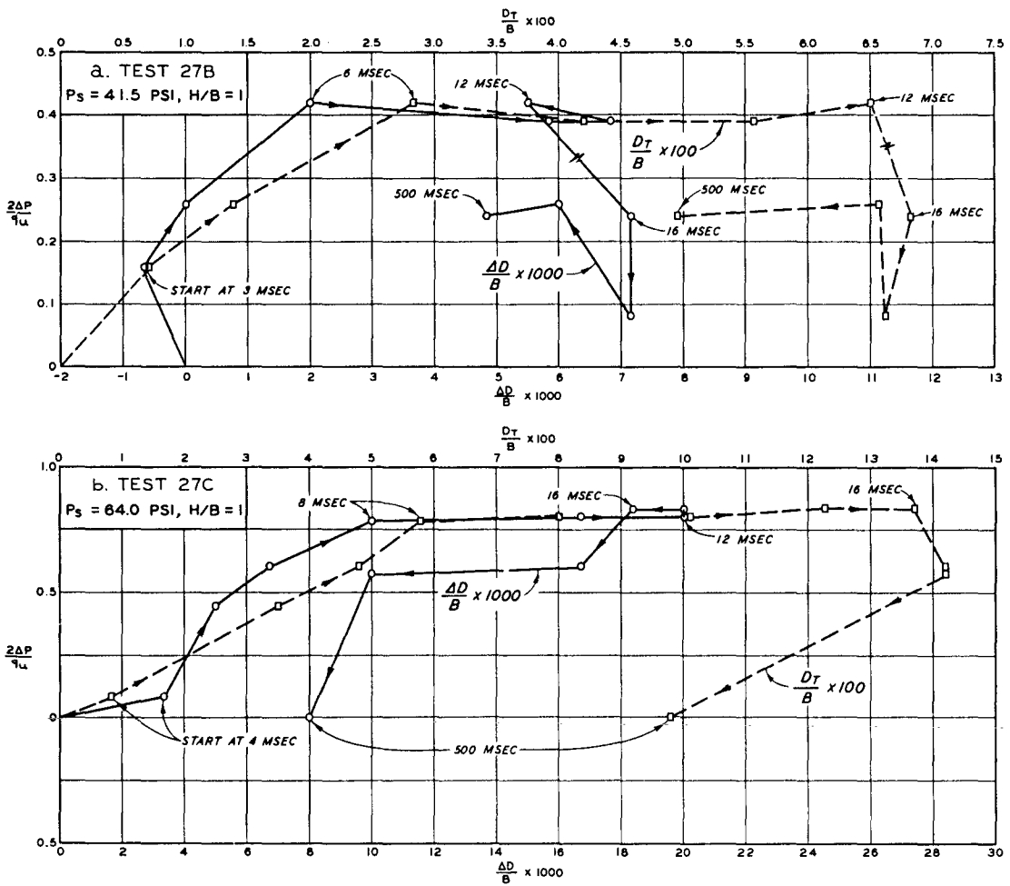
Fig. 59. Dimensionless plot of pressure versus deflection for dynamic Tests 27B and 27C
