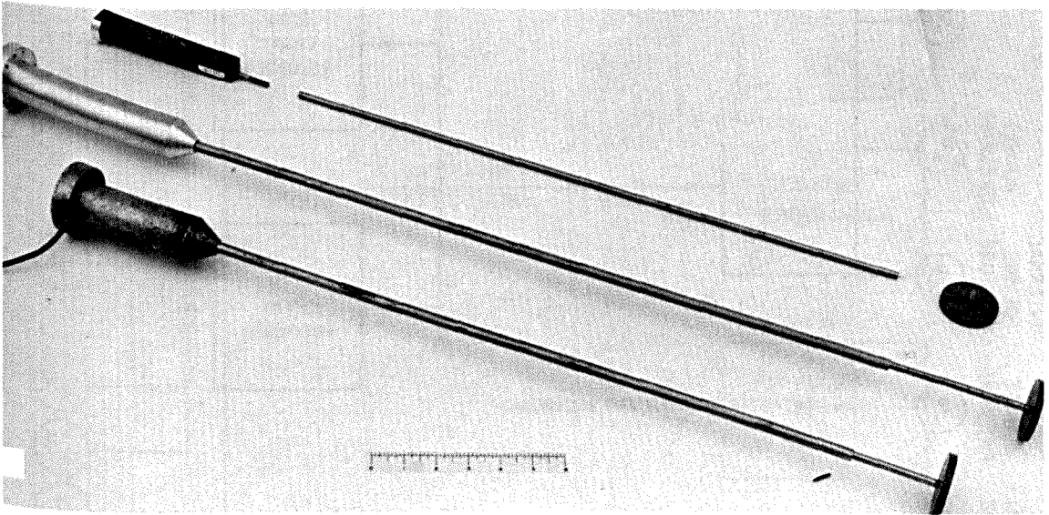
Fig. 17. WES soil deflection measuring device
