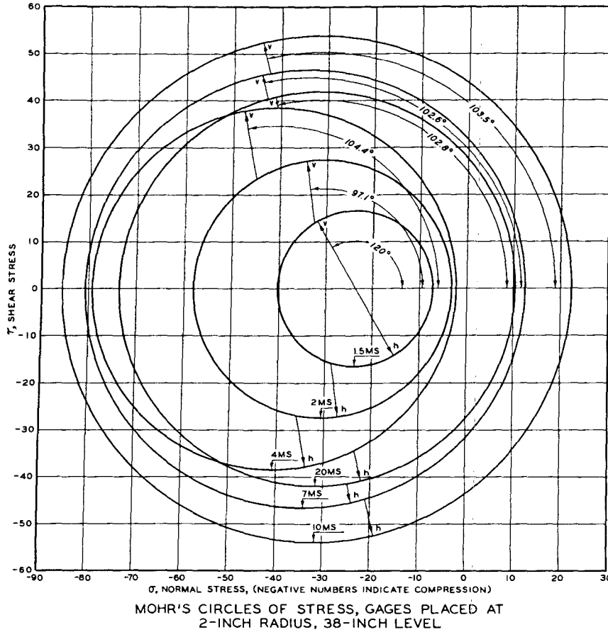
Fig. 70. Determination of direction and magnitude of principal stress, Test 25
