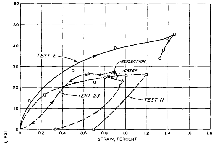
a. LOW PRESSURE TESTS, P_S < 40 PSI
