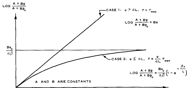
d. VARIATION OF STRESS WITH DEPTH
