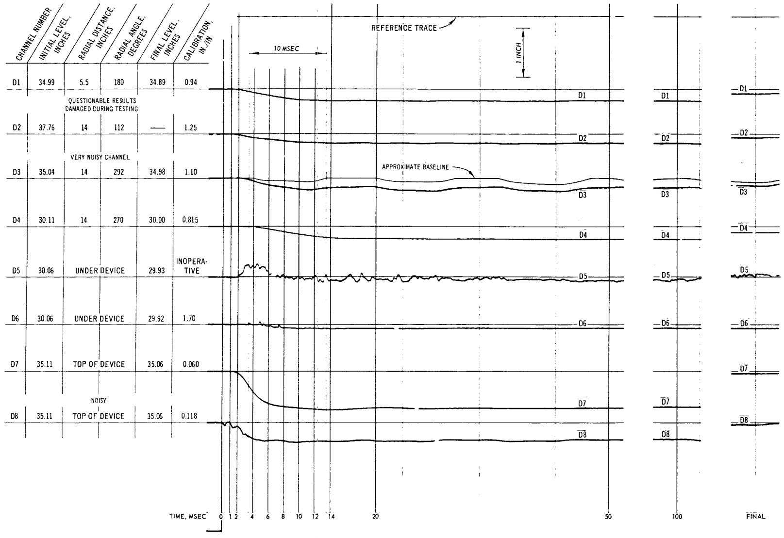
Fig. C-48. Test 22, deflection record
