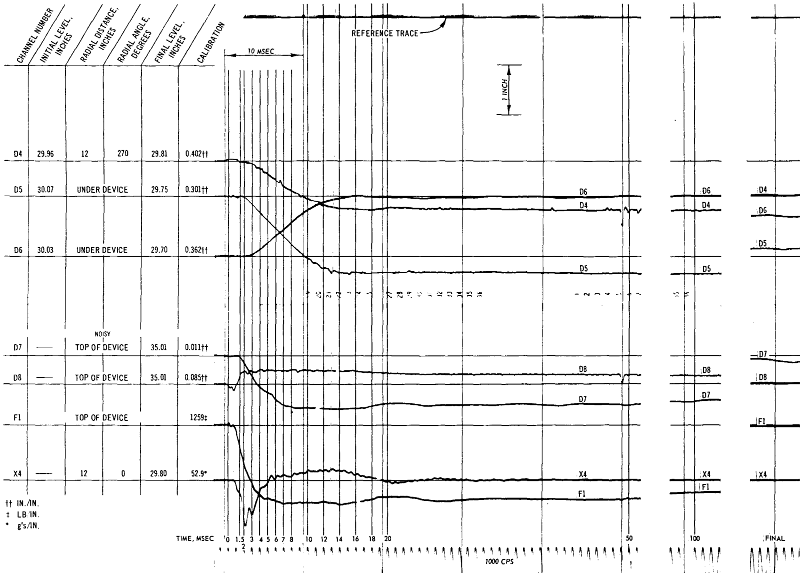
Fig. C-60. Test 25, deflection, force, and acceleration record
