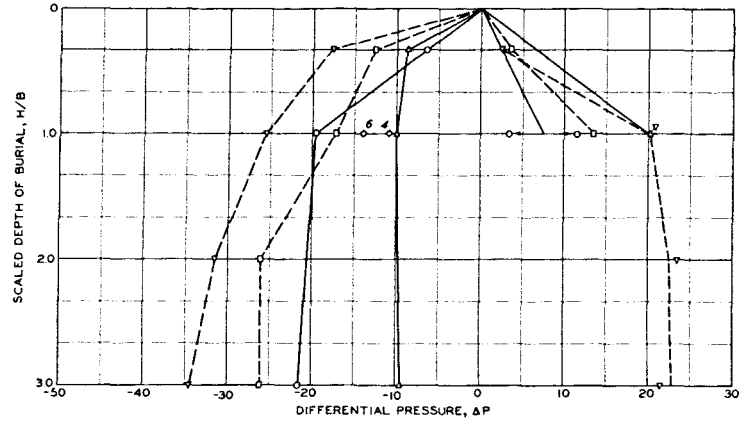
b. VARIATION OF DIFFERENTIAL PRESSURE WITH DEPTH OF BURIAL AT SCALED DIFFERENTIAL DEFLECTIONS OF \Delta D/B \times 1000 = \pm 2.0
