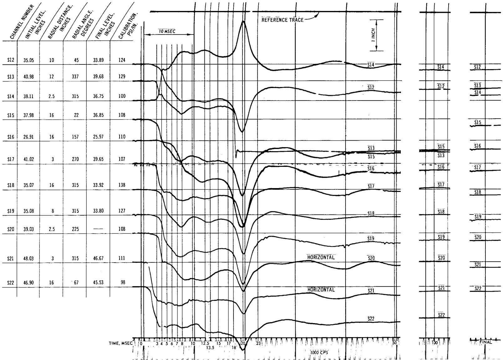
Fig. C-11. Test 13, pressure record (S12-S22)
