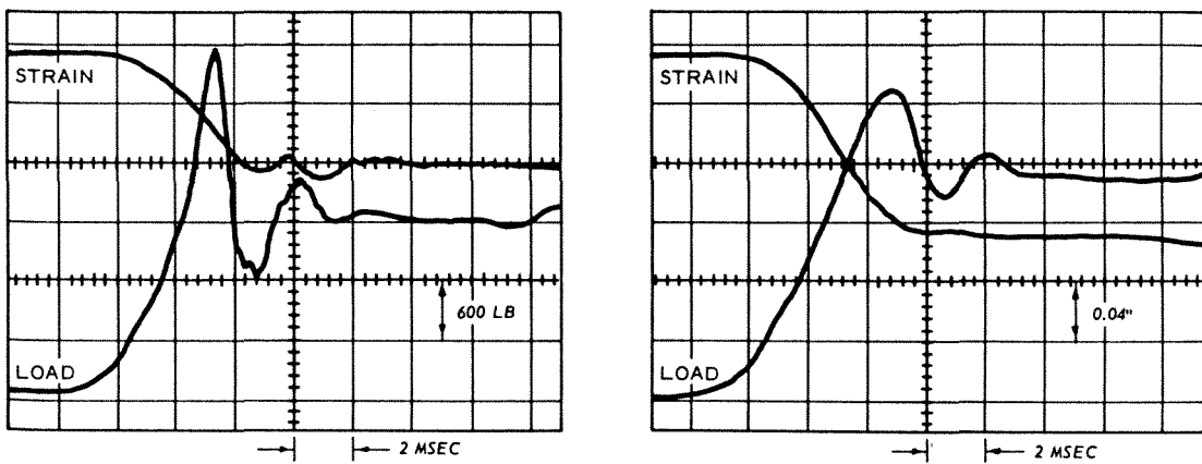
Fig. A-11. Typical oscilloscope records from confined compression tests
