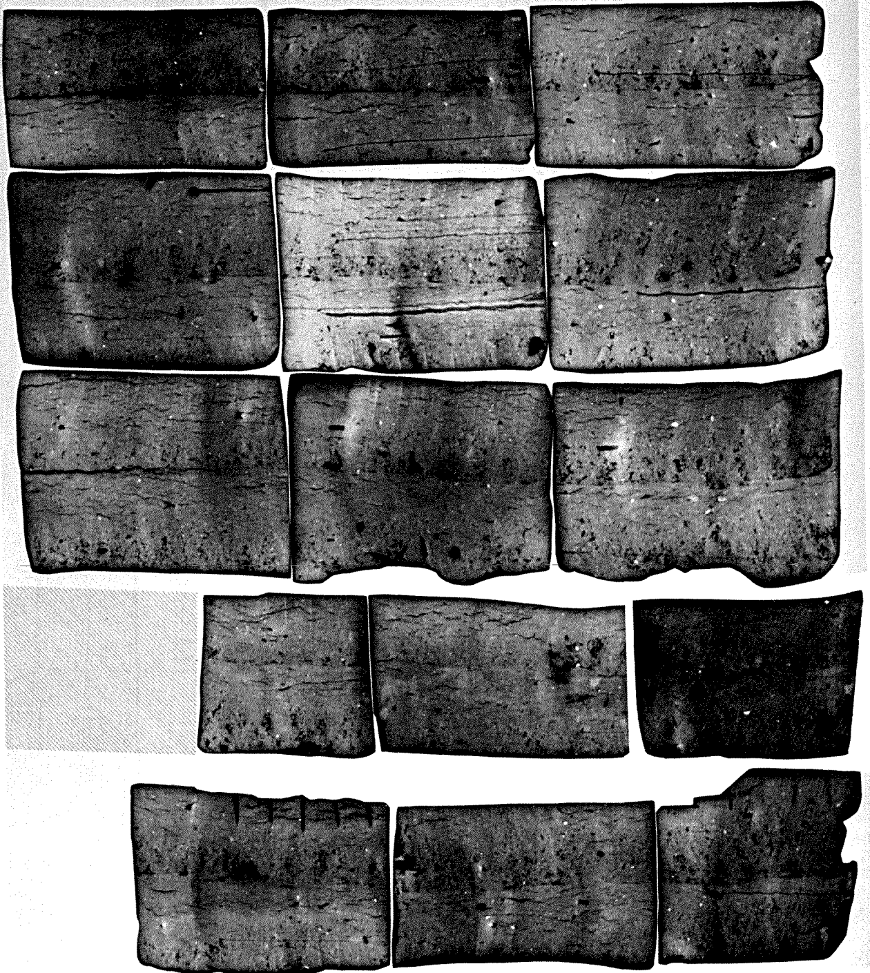
Fig. 44. Radiograph of soil deformation pattern, Test 3; H/B = 3, P_S = 37.5 \text{ psi}
