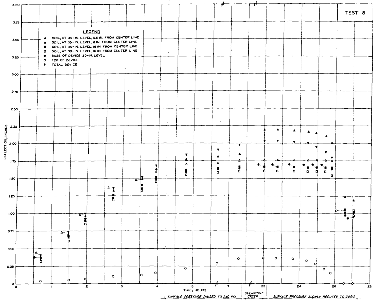
Fig. 40. Soil and structure deflections versus time; Test 8, H/B = 3 , P_S = 240 psi
