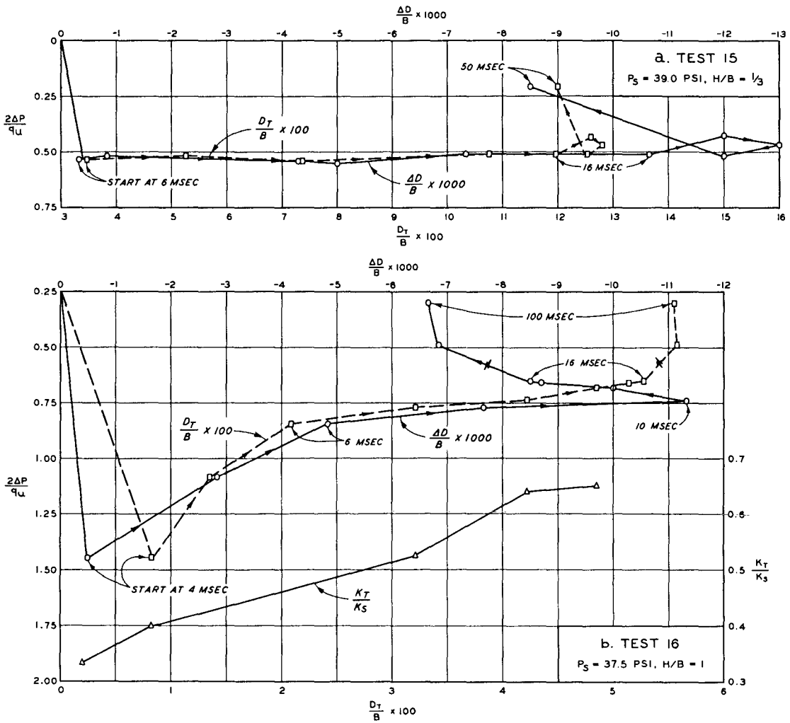
Fig. 53. Dimensionless plot of pressure versus deflection for dynamic Tests 15 and 16
