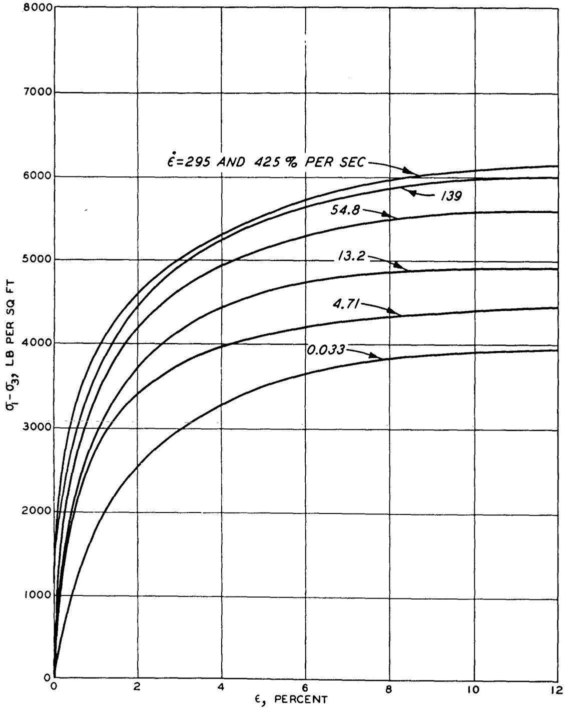
Fig. A-24. Stress-strain curves, buckshot clay (after Carroll)
