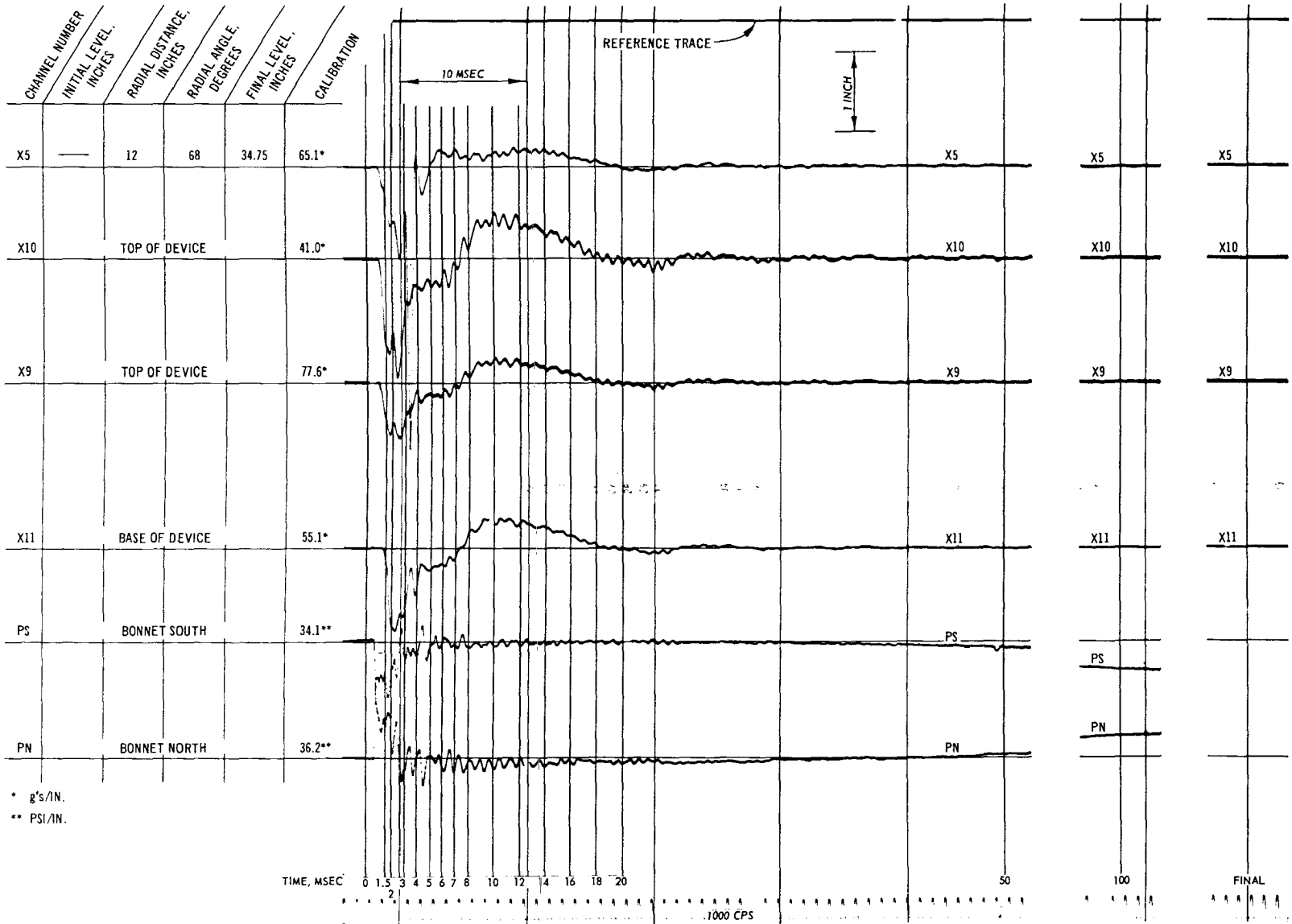
Fig. C-61. Test 25, acceleration and pressure record
