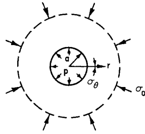
(a) GEOMETRY AND BOUNDARY CONDITIONS
