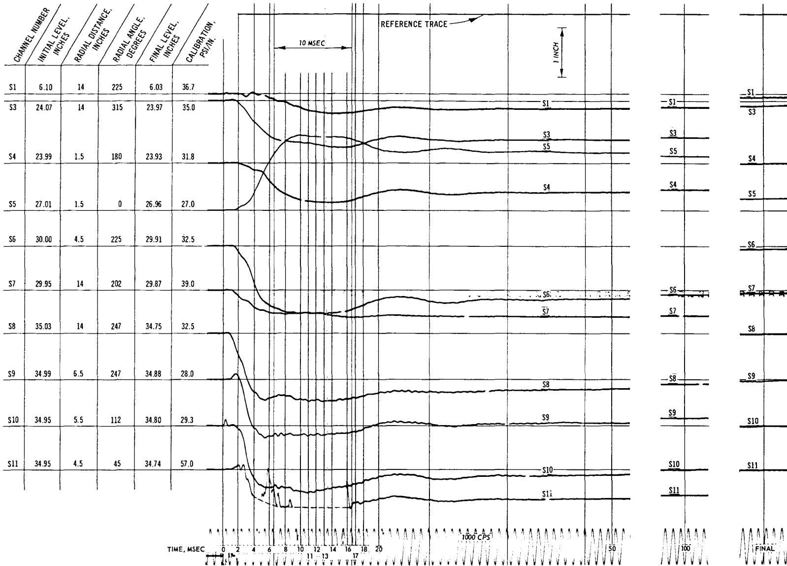
Fig. C-38. Test 20, pressure record (S1-S11)
