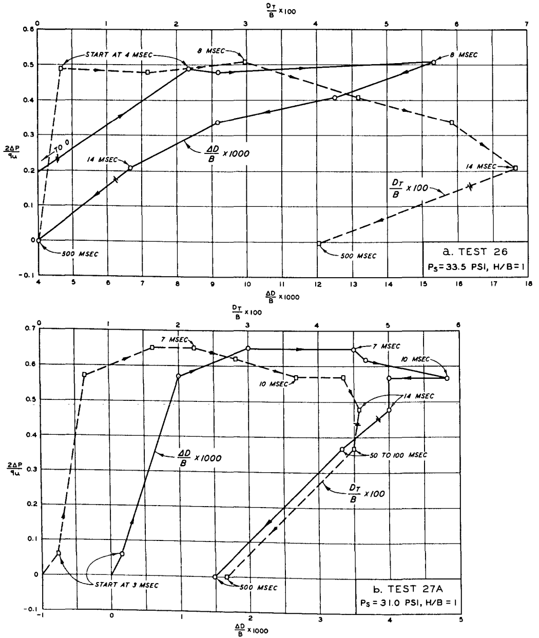
Fig. 58. Dimensionless plot of pressure versus deflection for dynamic Tests 26 and 27A
