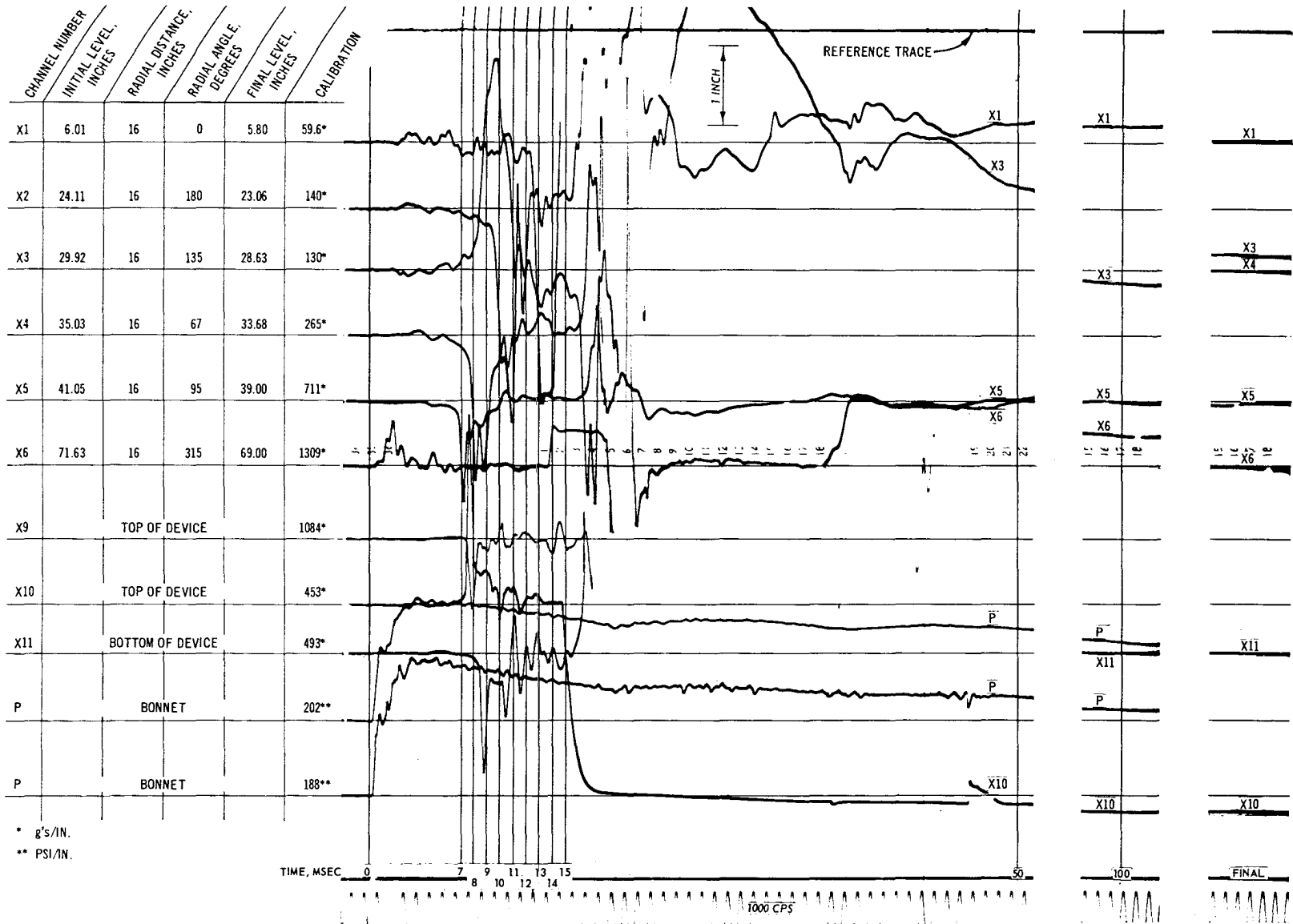
Fig. C-33. Test 18, acceleration and pressure record
