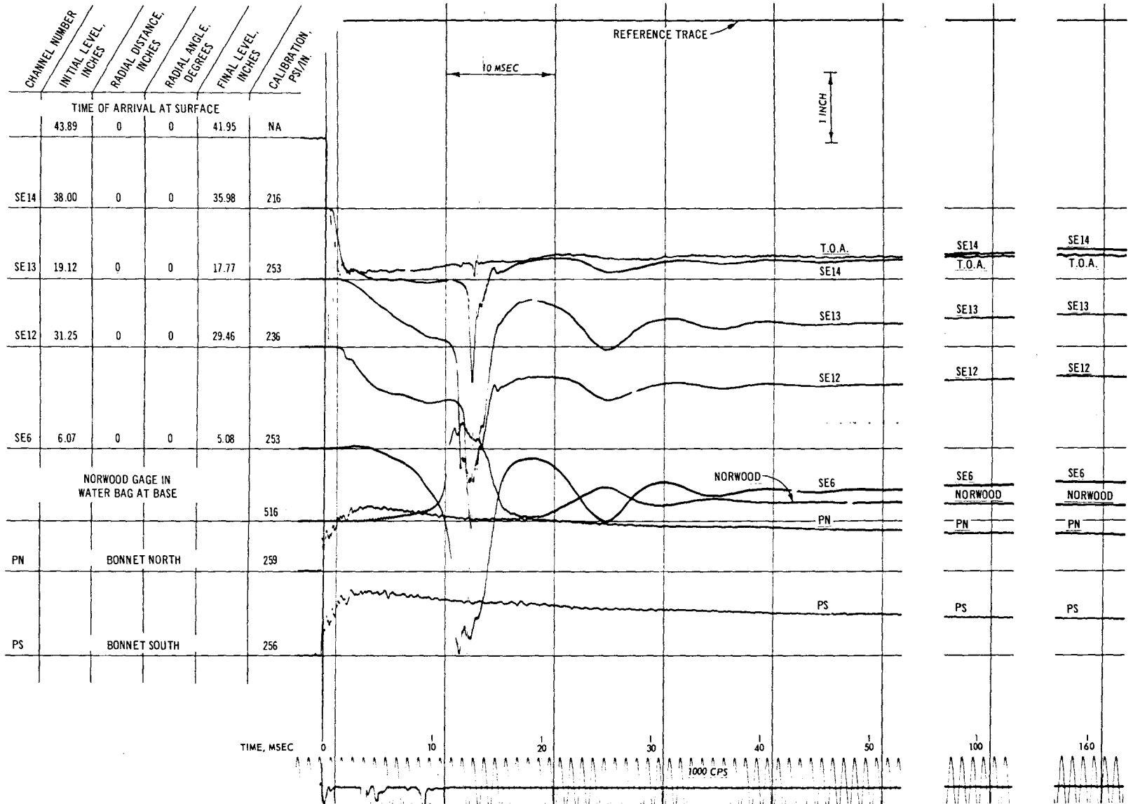
Fig. C-76. Test A, pressure record
