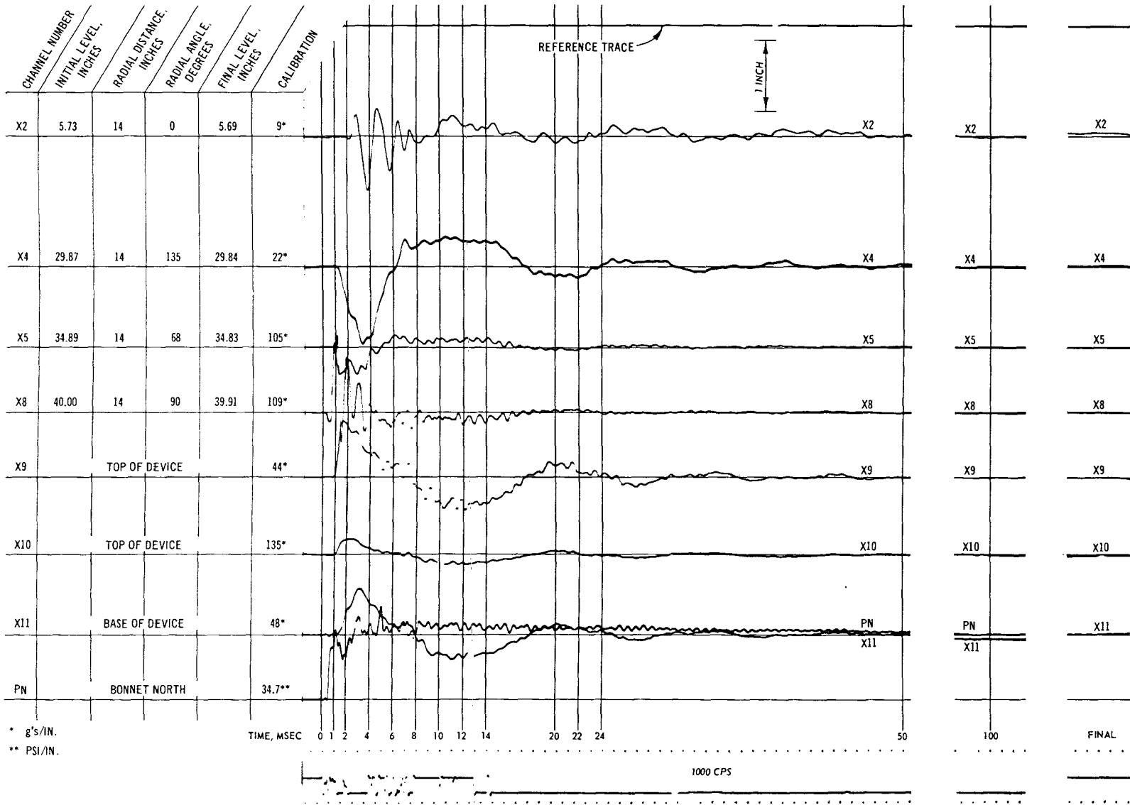
Fig. C-75. Test 28, acceleration and pressure record
