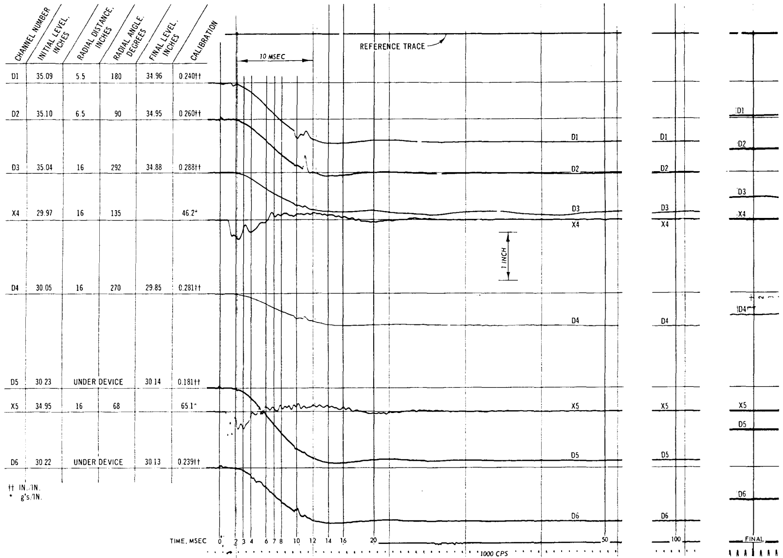
Fig. C-66. Test 27A, deflection and acceleration record
