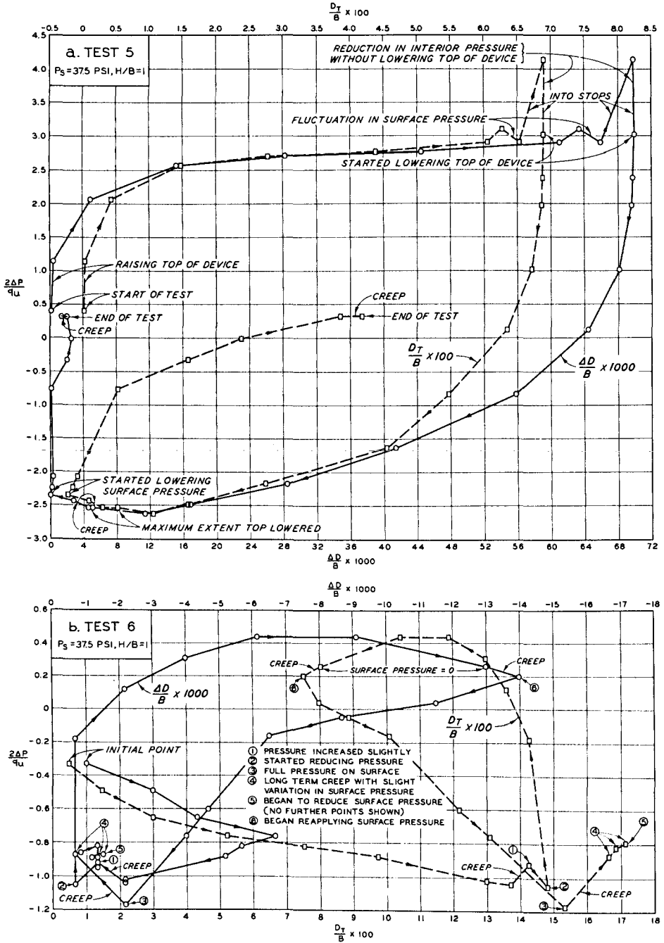
Fig. 24. Dimensionless plot of pressure versus deflection for static Tests 5 and 6
