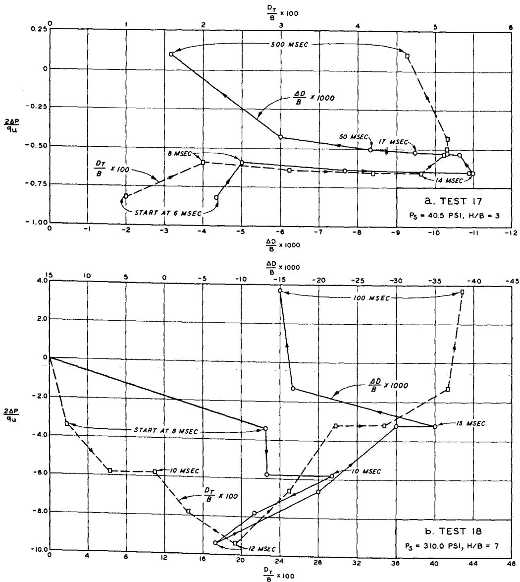
Fig. 54. Dimensionless plot of pressure versus deflection for dynamic Tests 17 and 18
