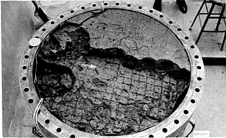
a. Oblique view of 38-inch soil level
