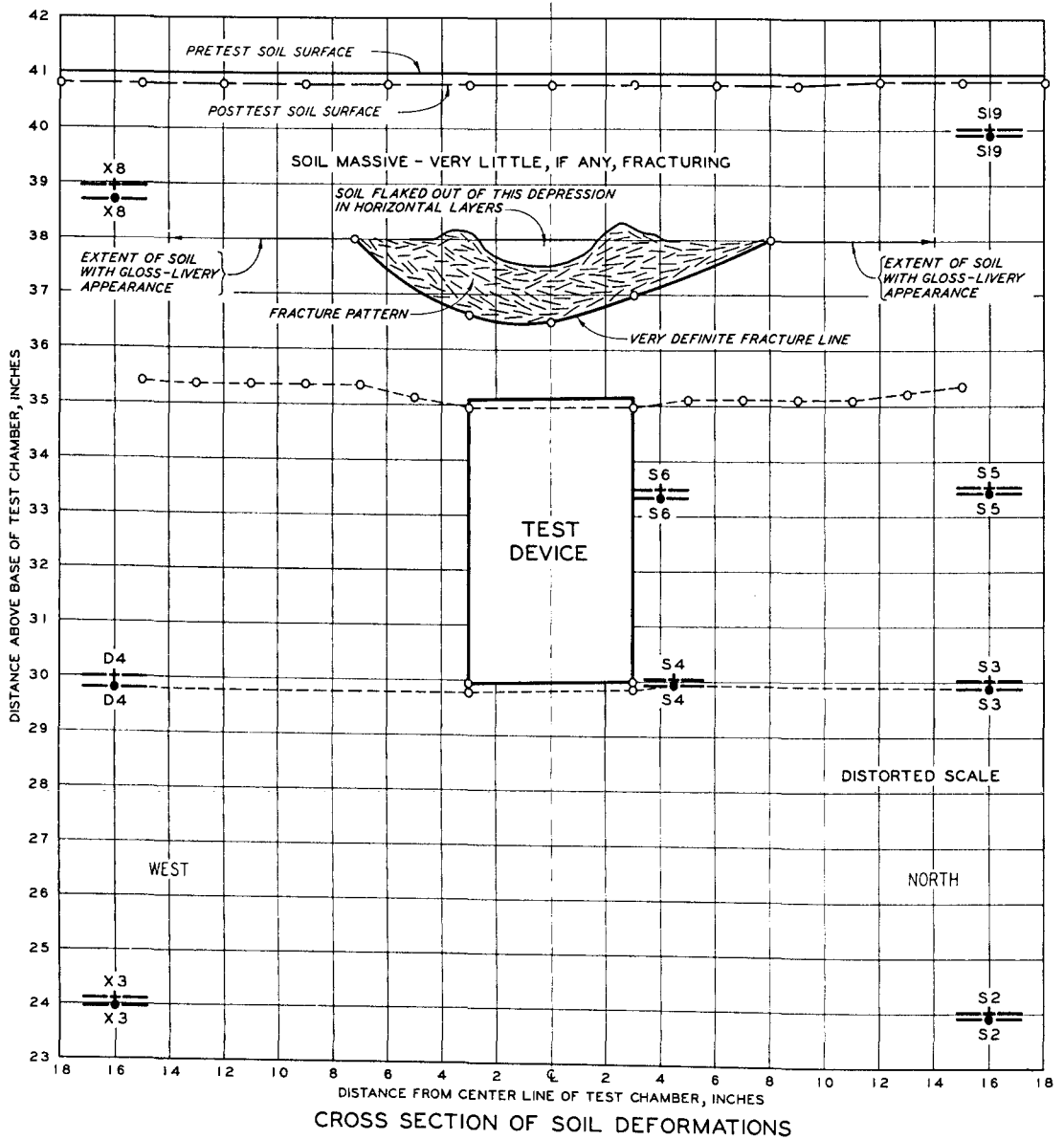
Fig. 88. Cross section of soil deformations, Test 26; H/B = 1 , P_s = 33.5 psi
