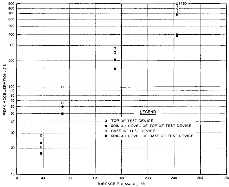
a. Variation with change in surface pressure at constant depth of burial; Tests 11, 12, 13, and 14; H/B = 3
