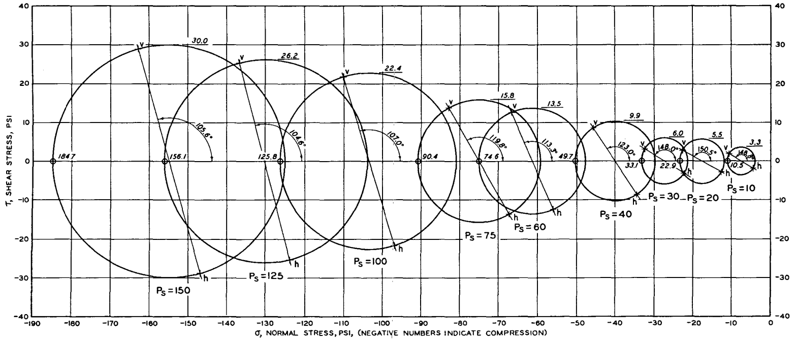
d. TEST 8—MOHR'S CIRCLES OF STRESS, GAGES S_2 , S_3 , AND S_4 , 4.5-INCH RADIUS AT 35-INCH LEVEL
