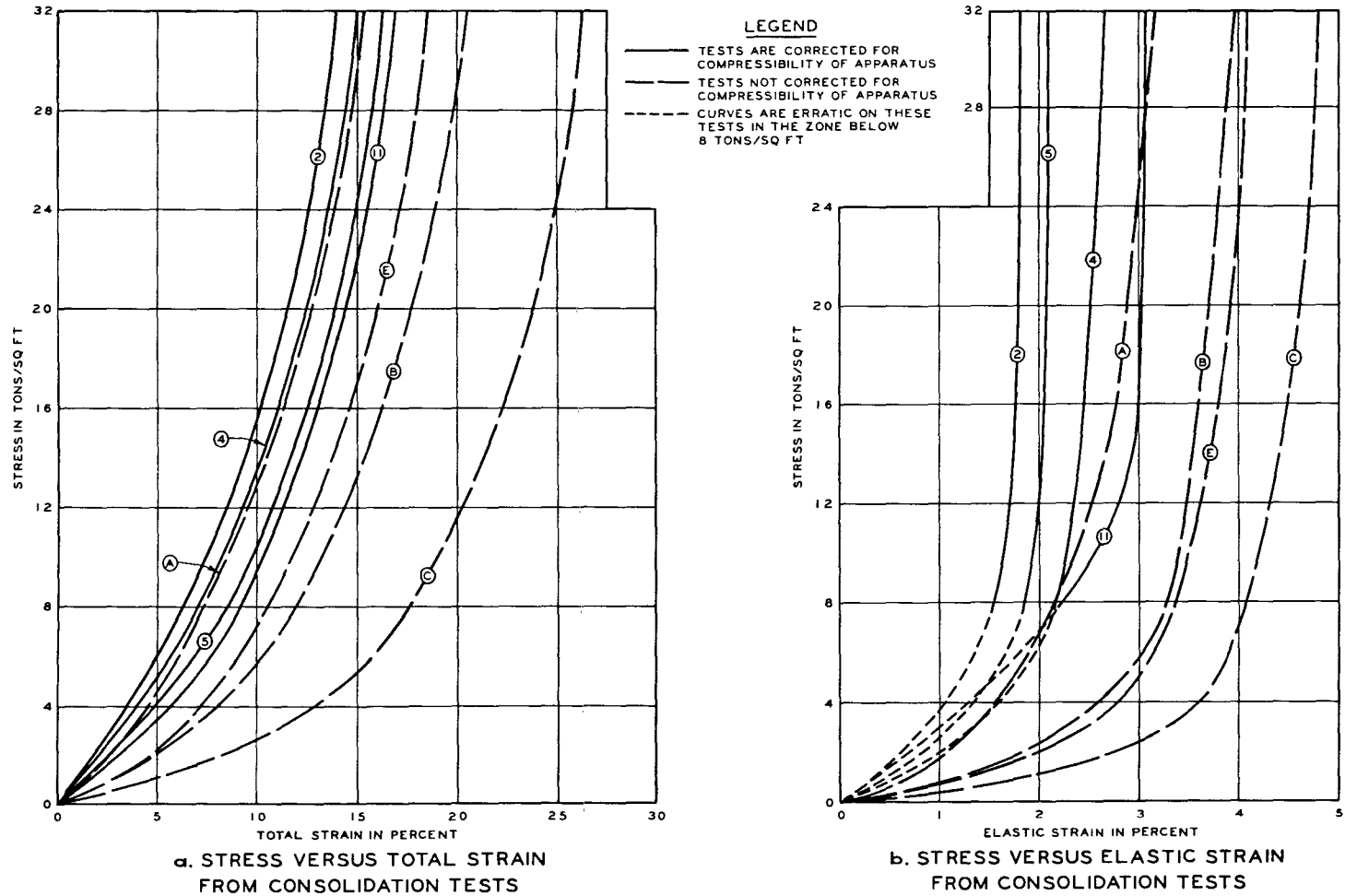
Fig. A-15. Stress-strain curves constructed from consolidation test results
