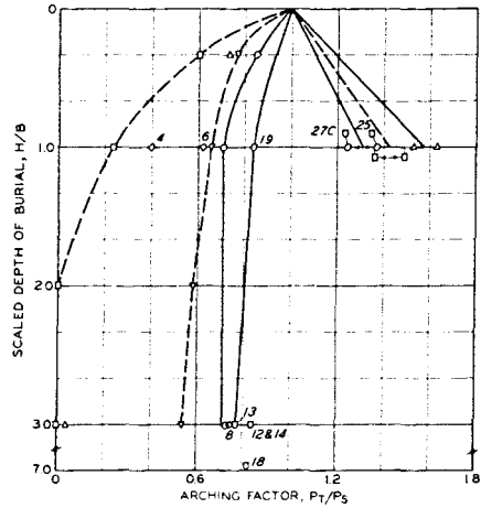
a. VARIATION OF RELATIVE LOAD ON THE STRUCTURE WITH DEPTH OF BURIAL; WC ≈ 26% AND B=6 INCHES
