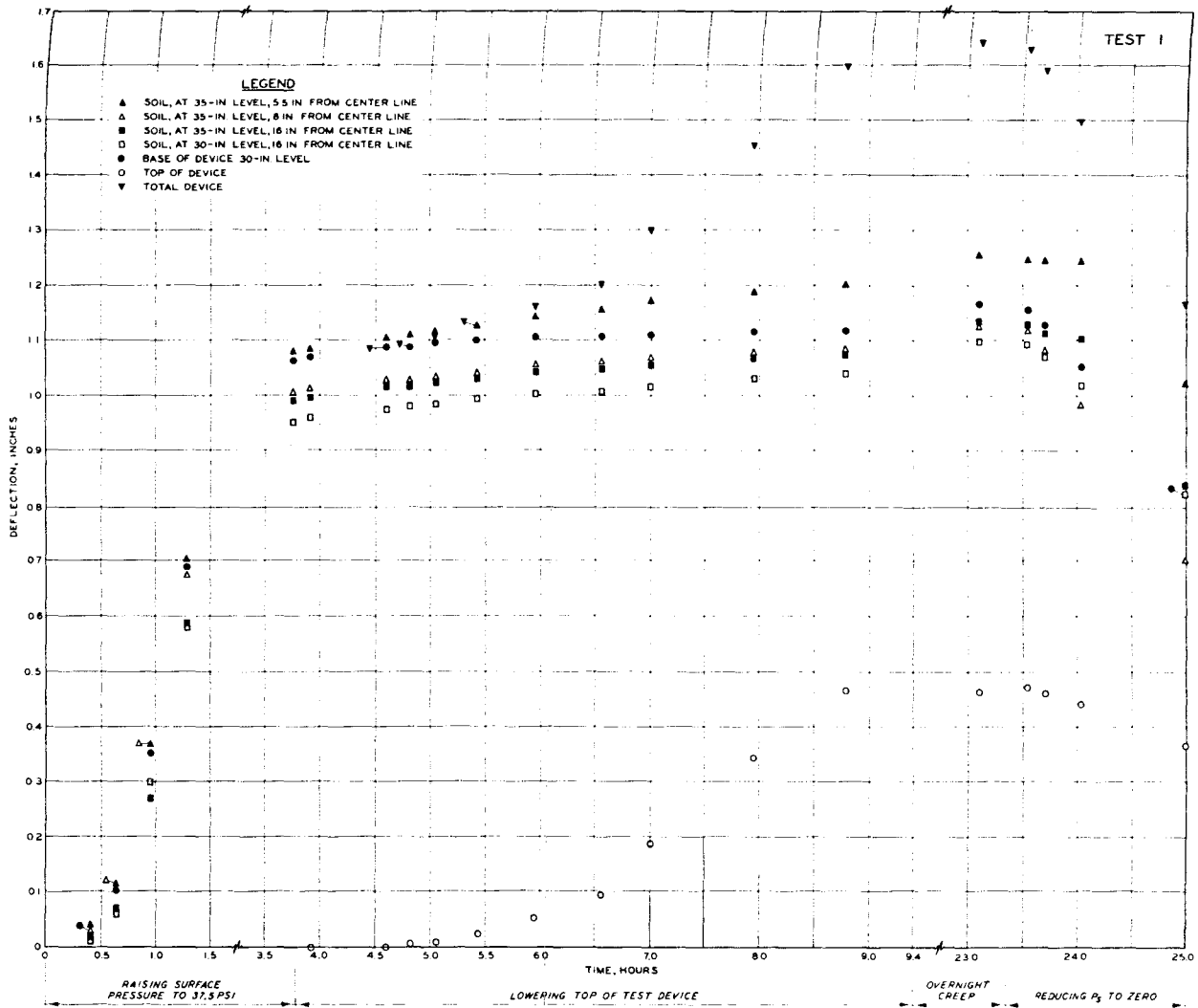
Fig. 35. Soil and structure deflections versus time; Test 1, H/B = 1/3 , P_s = 37.5 psi
