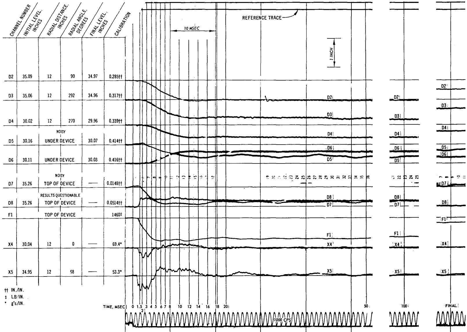
Fig. C-56. Test 24, deflection, force, and acceleration record
