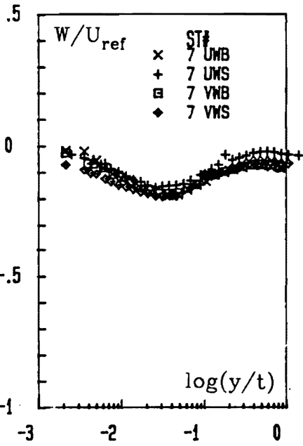
Figure 20w. U,V,W mean velocity components measured with two different LDV techniques presented in tunnel coordinates.: UV, UW and VW show the LDV beam system used to obtain the data. Extensions B and S denote the measurements taken with Burst Spectrum Analyzer and fast sampling rate swept-spectrum analyzer, respectively. Station numbers are also shown in the figures.
