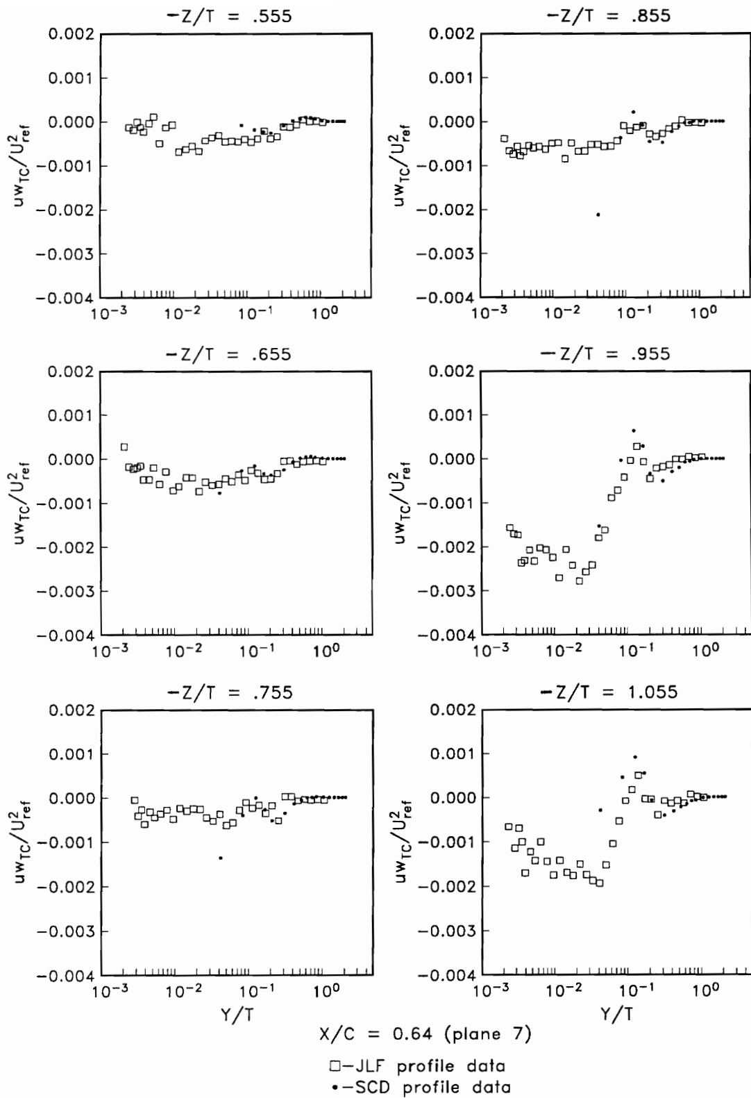
Figure 4.72. Profiles of \overline{u w_{TC}} / (U_{ref})^2 , Plane 7
