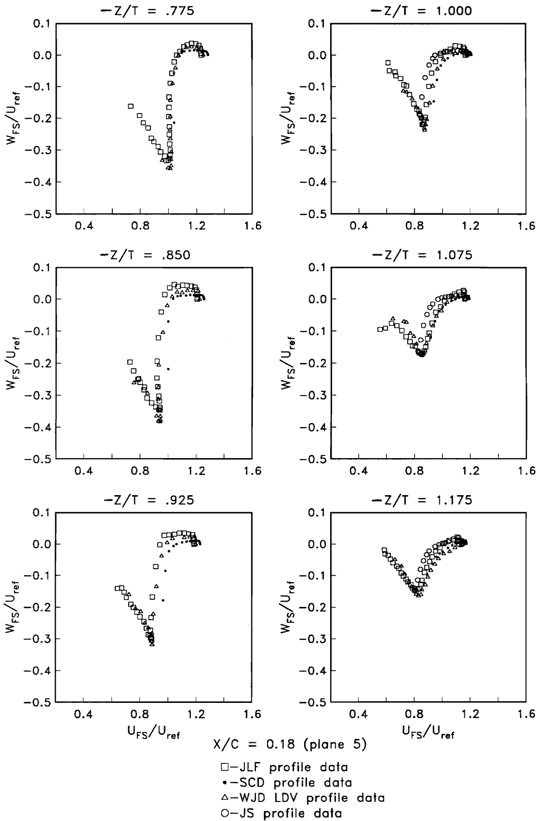
Figure 4.77. Boundary Layer Hodograph Plots, Plane 5
