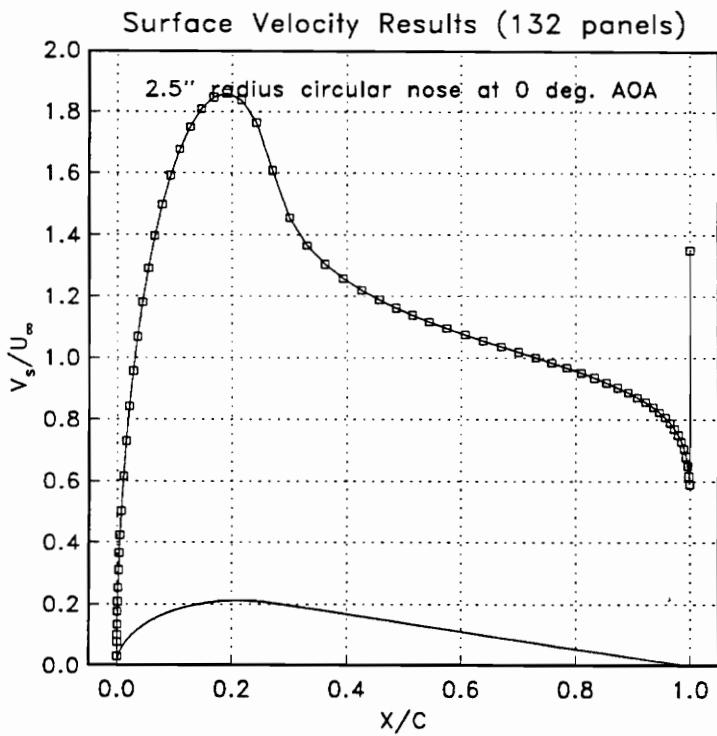
Figure 6.5a,b. Baseline and Teardrop Appendage Velocity Results, 0° AoA
