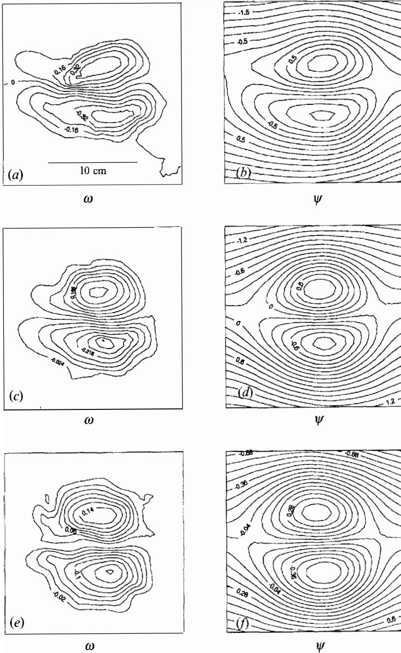
FIGURE 13. Contour plots of vorticity \omega (left column) and corresponding stream function \psi (right column) for a dipole created by a laminar injection of fluid. The dipole moves to the right. (a, b) t = 33 s, (c, d) 64 s and (e, f) 121 s. Experimental parameters: Q = 0.58 ml s^{-1} , \delta t = 25 s and N = 3.0 rad s^{-1} .
