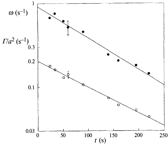
FIGURE 18. Graphical representation of the decay of the mean normalized circulation \Gamma/a^2 ( \circ ) and the mean extremal vorticity \omega = \frac{1}{2}(\omega_{max} - \omega_{min}) ( \bullet ). Both data sets are least-square fitted by exponential functions of the form e^{-\alpha t} , with \alpha a free parameter. Experimental parameters: see figure 8.
